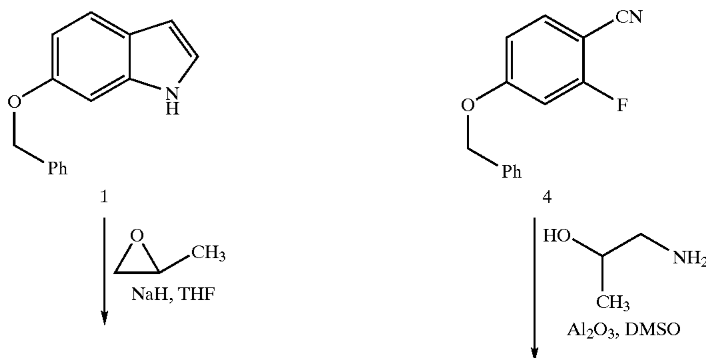
SCHEME 1
