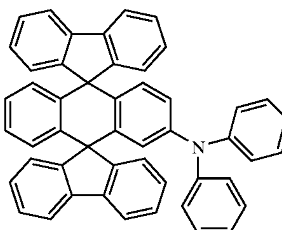
Chemical Compound 11
