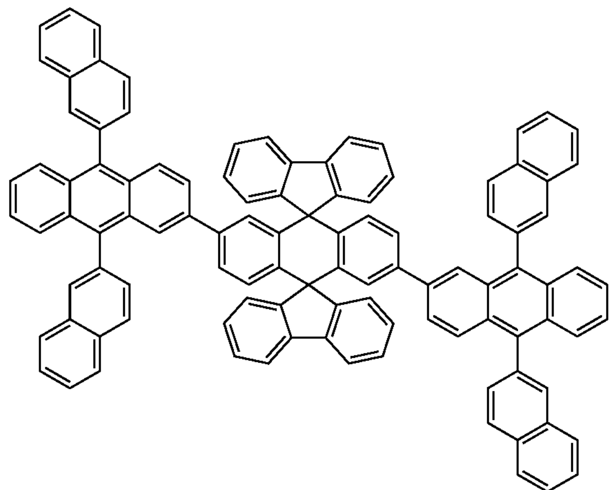
Chemical Compound 123
