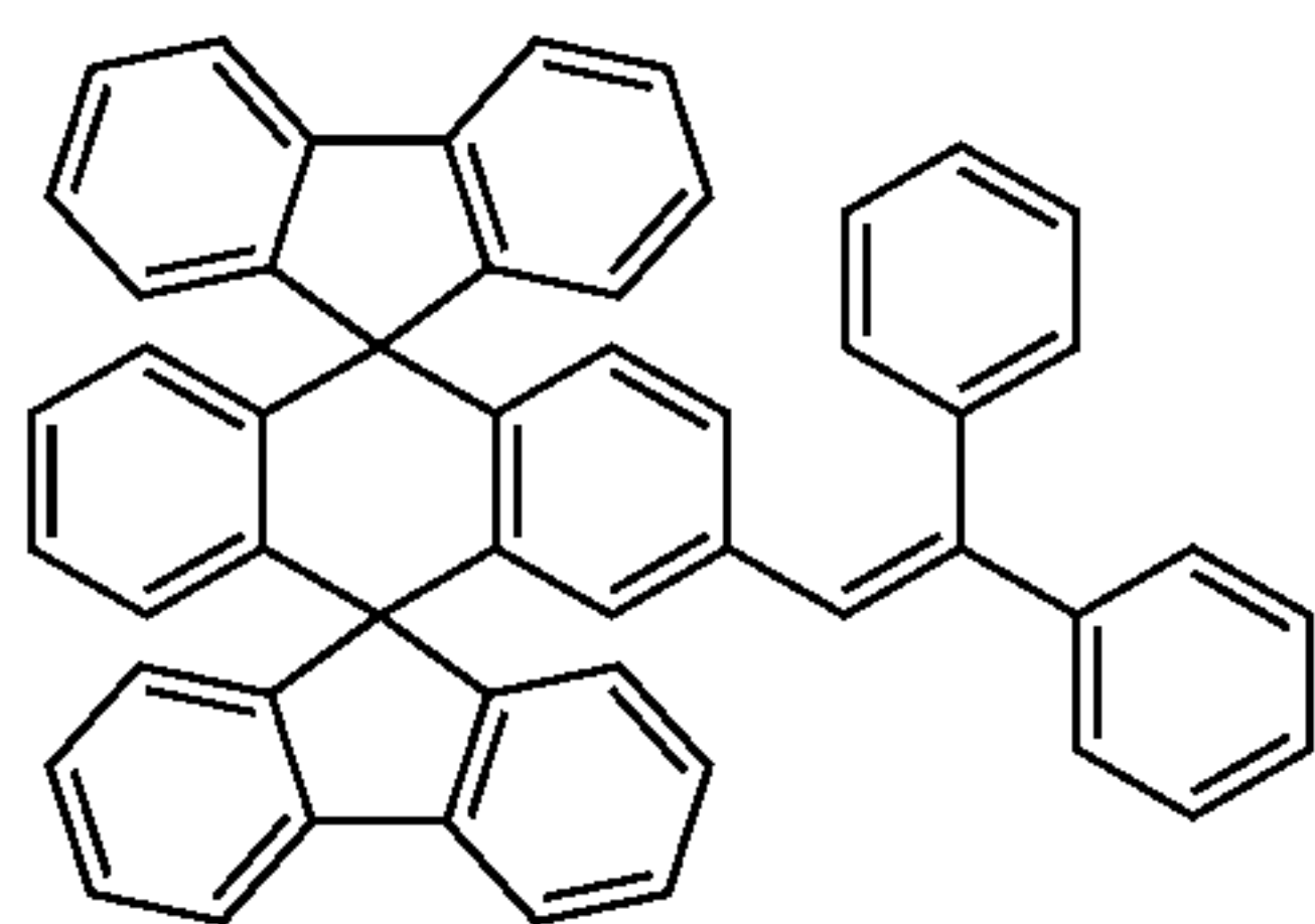
Chemical Compound 106
