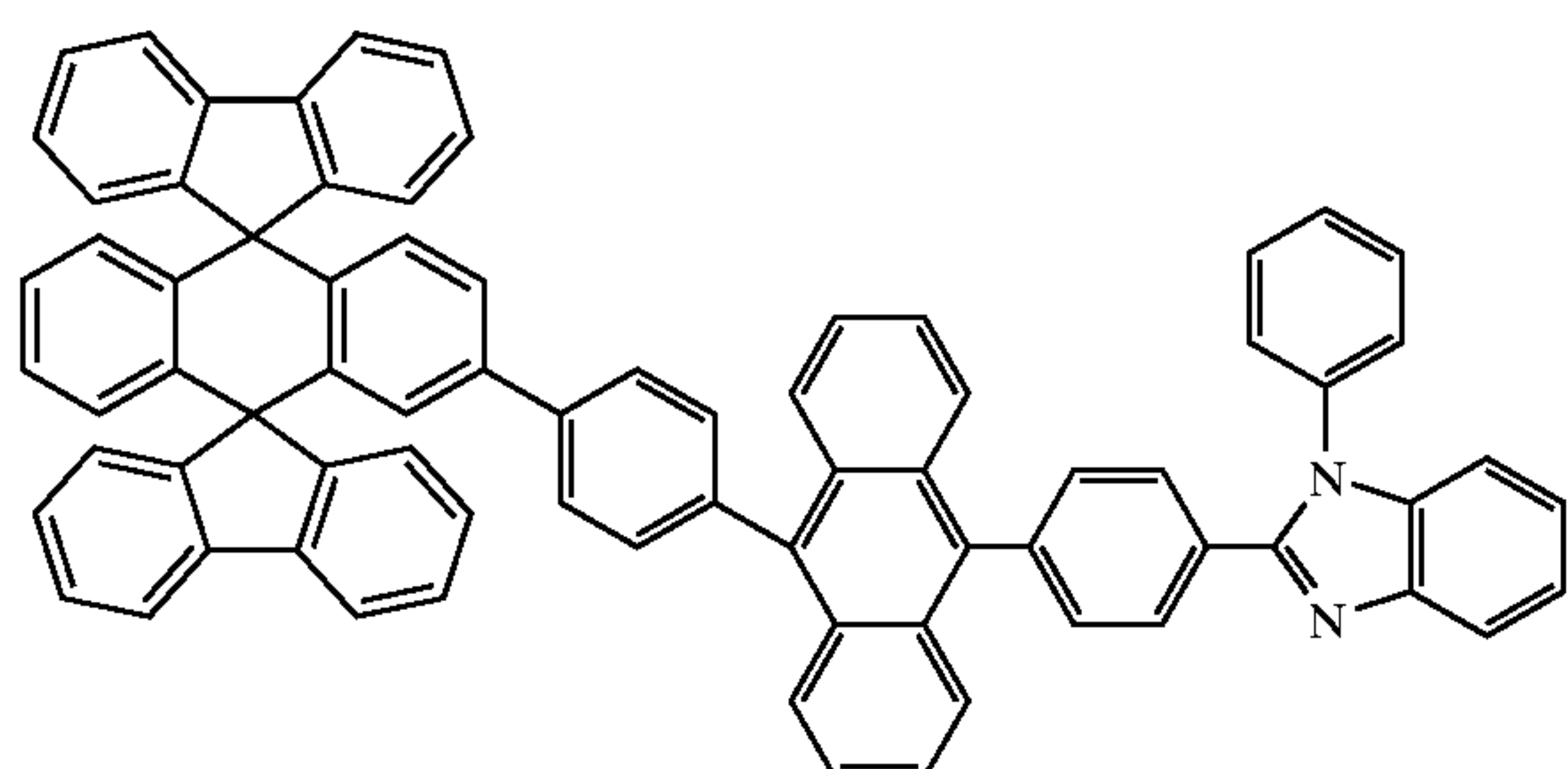
Chemical Compound 210
