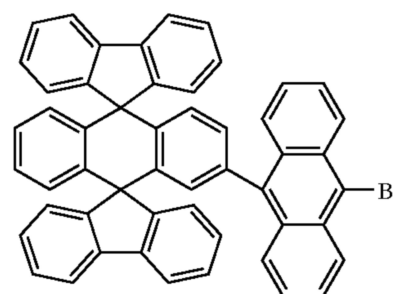
Chemical Compound 5
