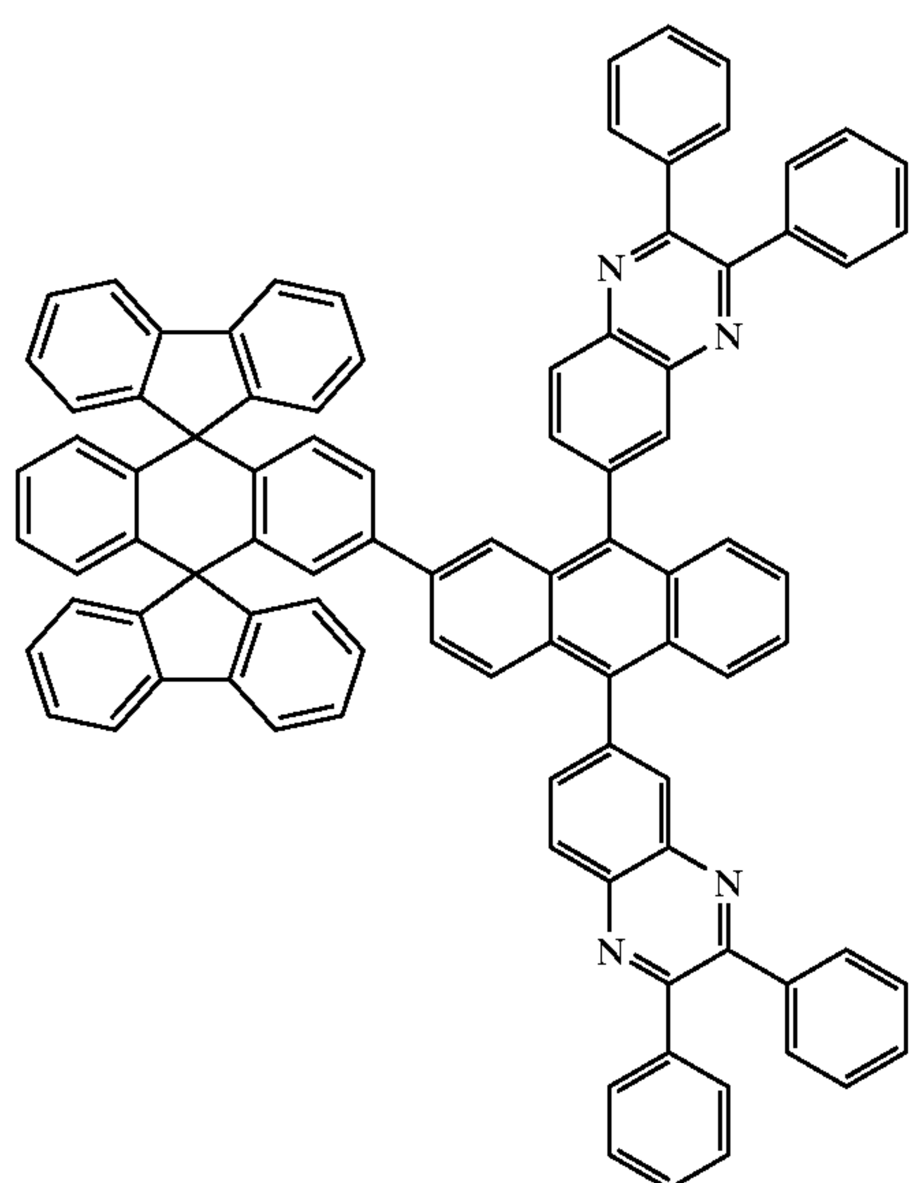
Chemical Compound 212
