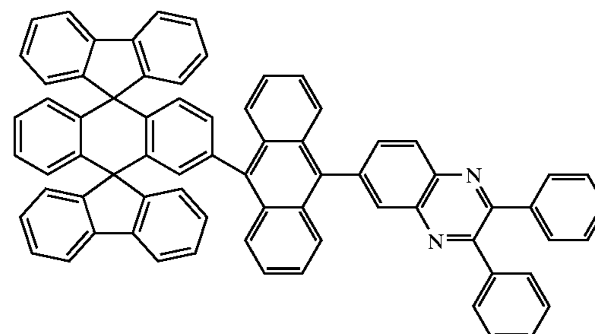
Chemical Compound 203
