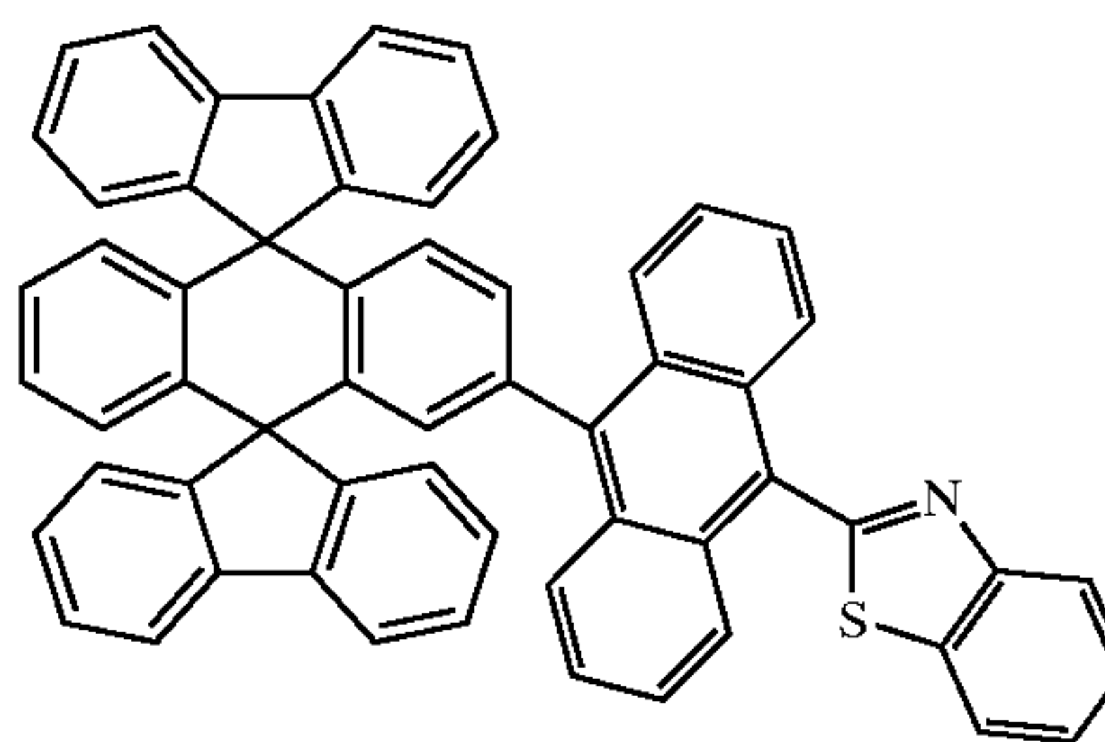
Chemical Compound 214
