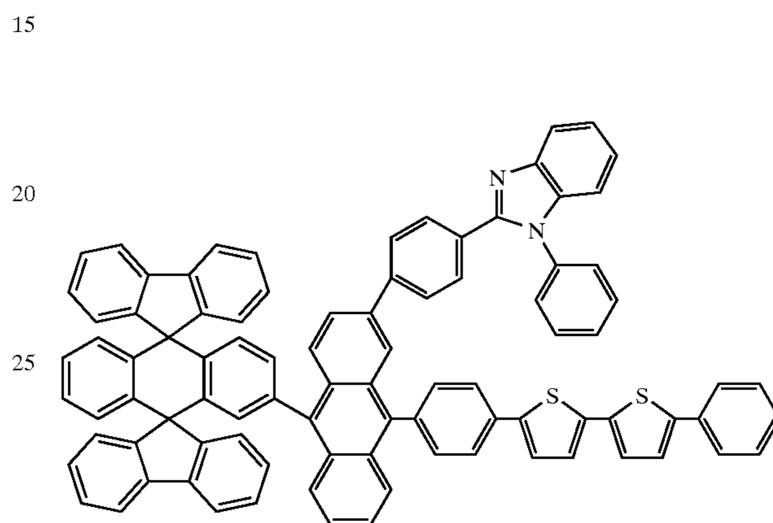
Chemical Compound 132
