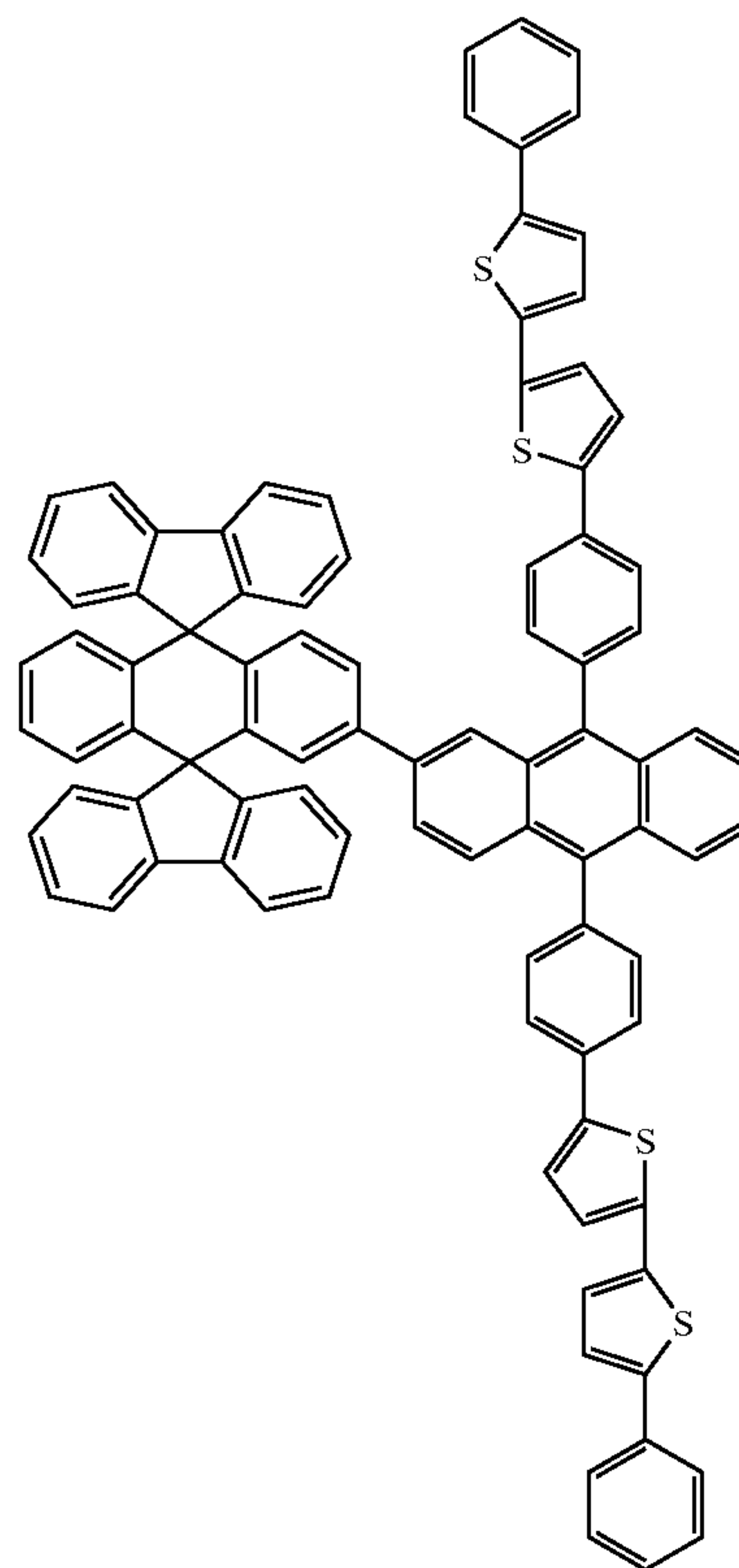
Chemical Compound 129
