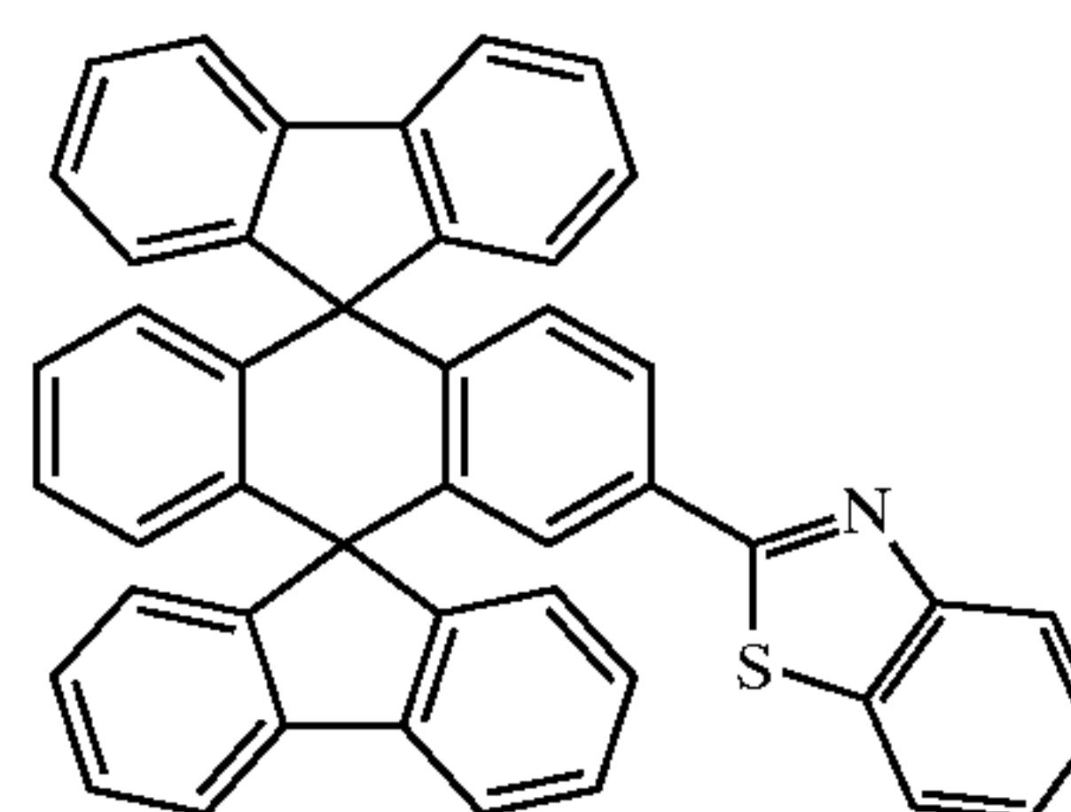
Chemical Compound 215
