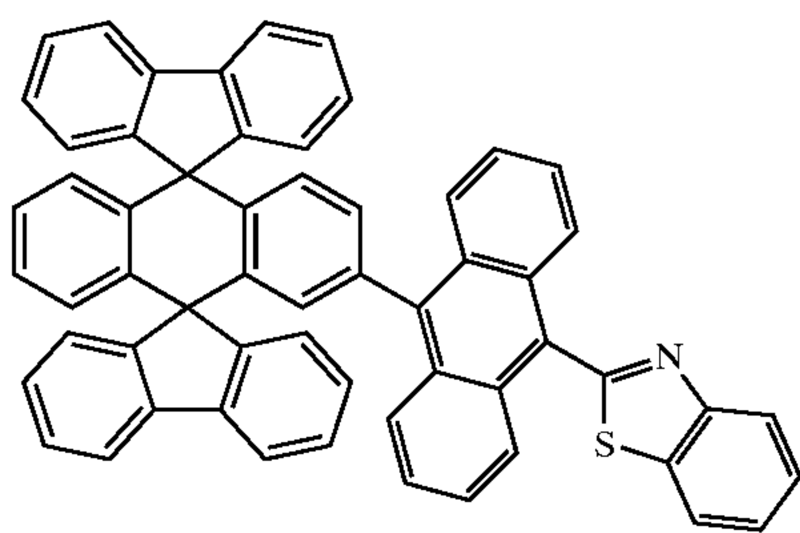
Chemical Compound 214
