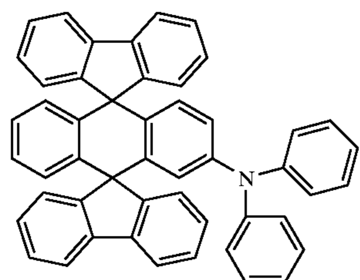
Chemical Compound 11
