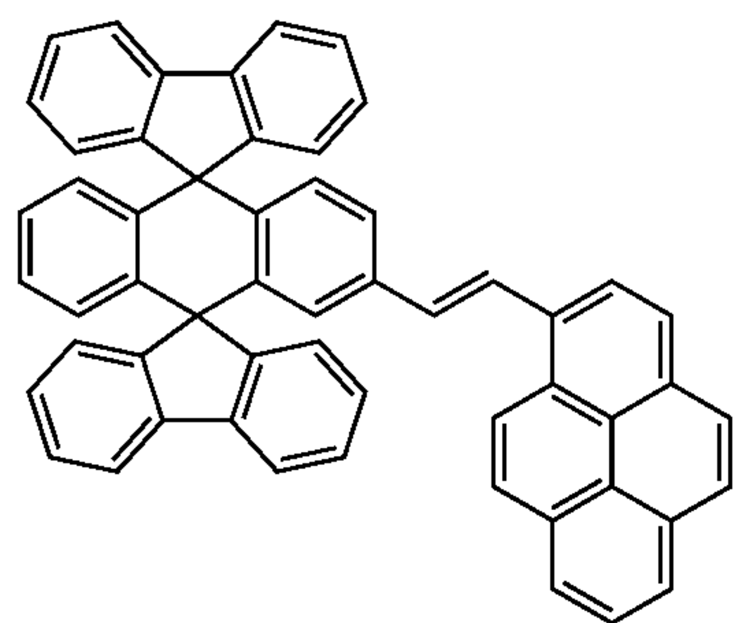
Chemical Compound 103
