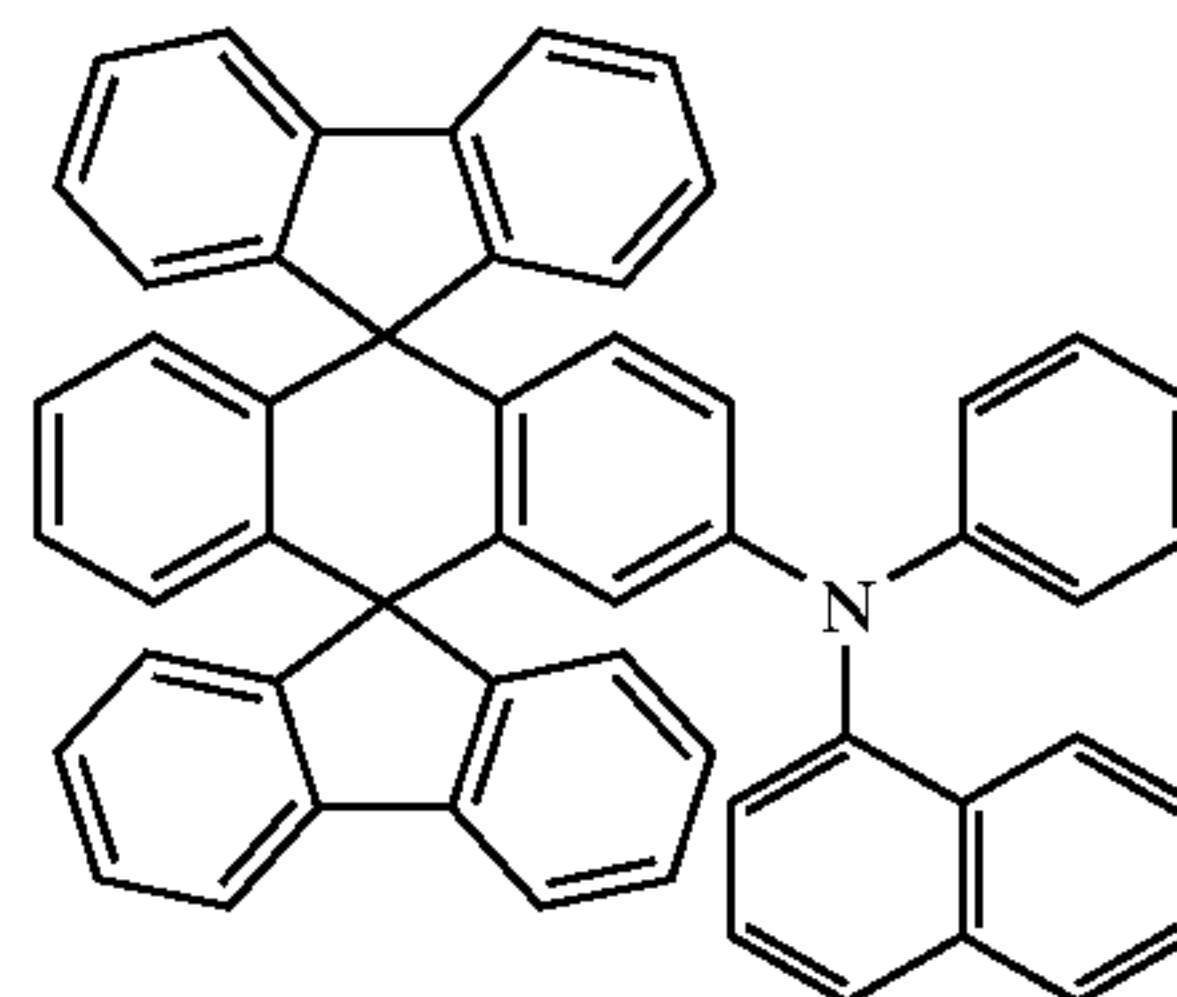
Chemical Compound 301
