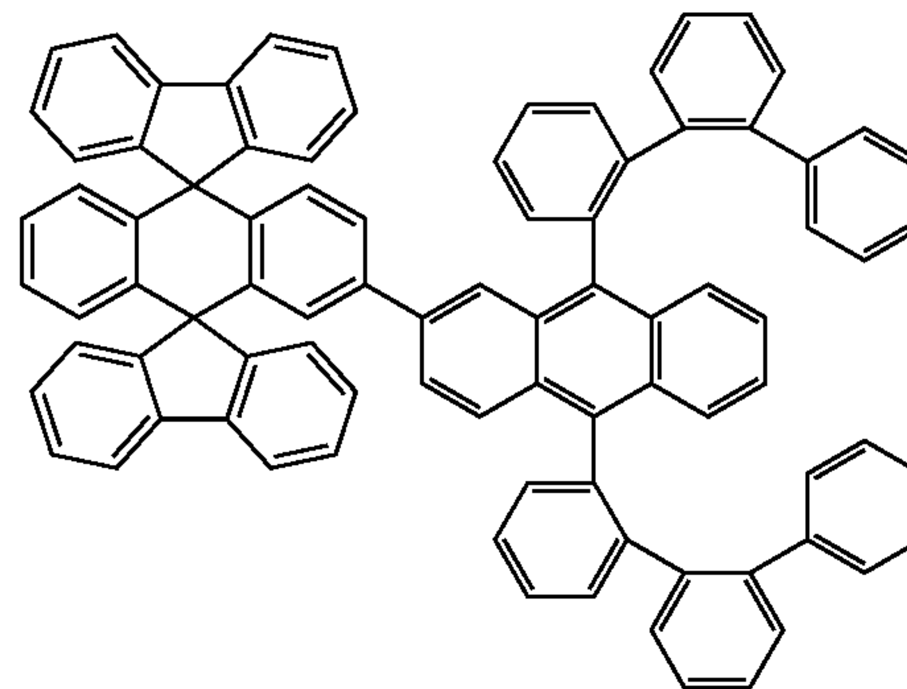
Chemical Compound 136
