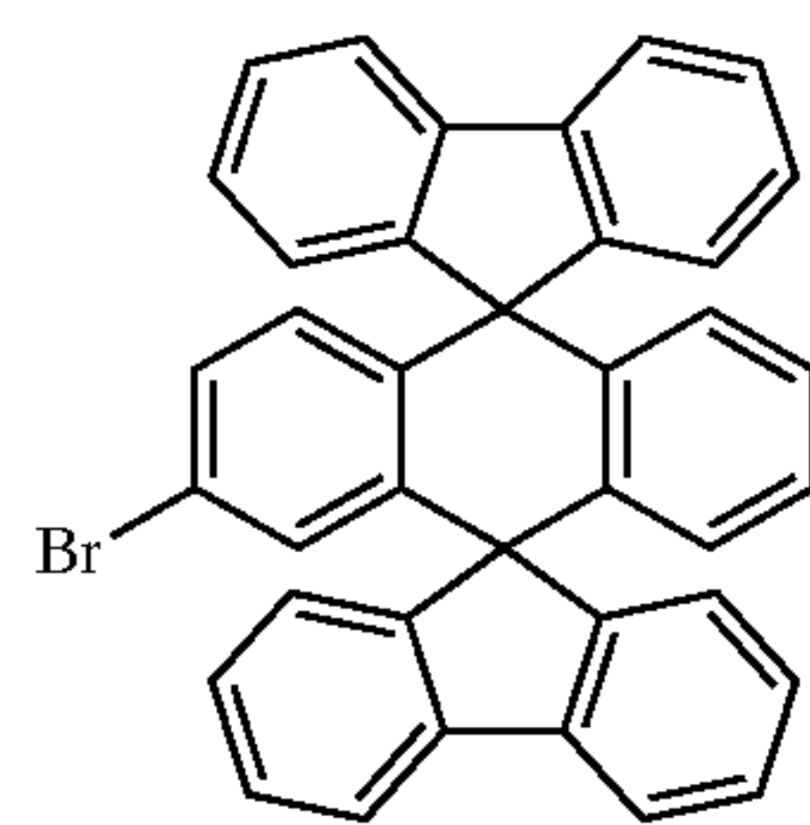
Chemical Compound 1
