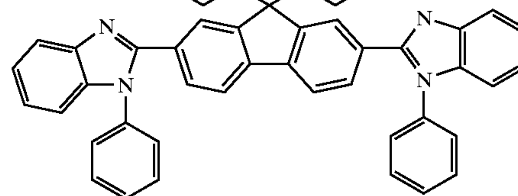
Chemical Compound 219
