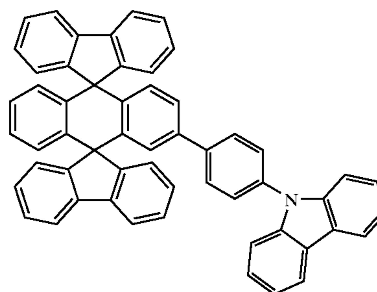
Chemical Compound 406
