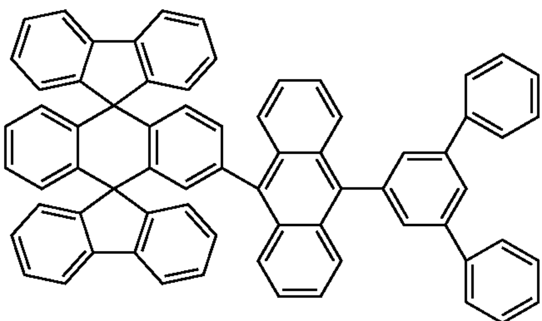
Chemical Compound 113
