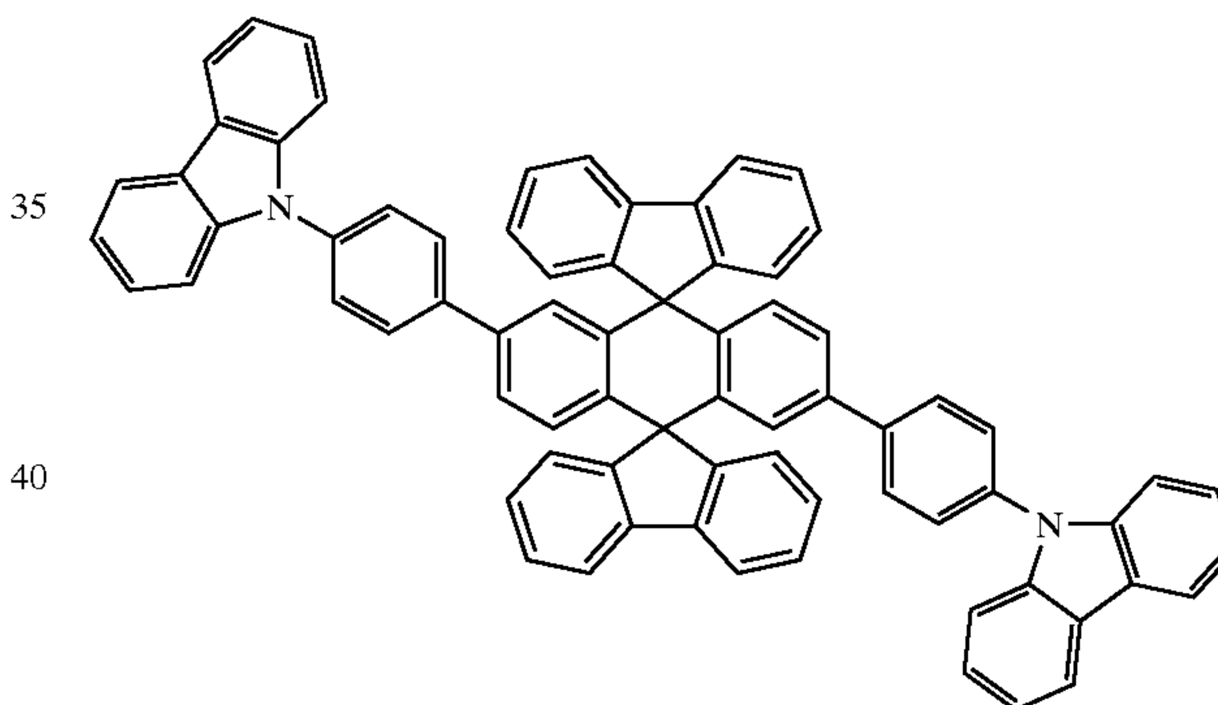
Chemical Compound 402
