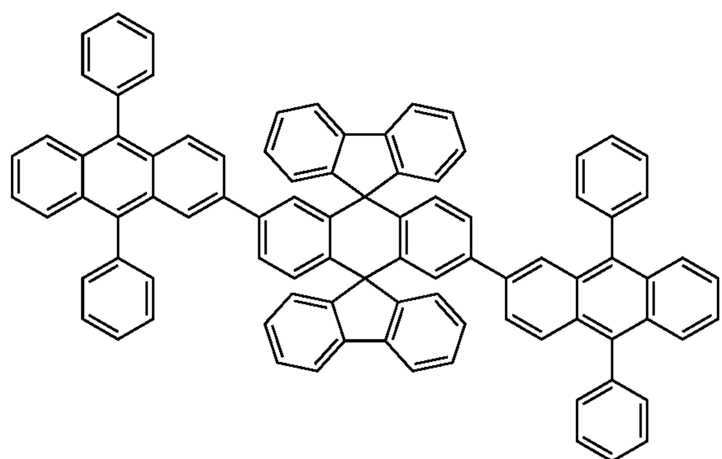
Chemical Compound 122
