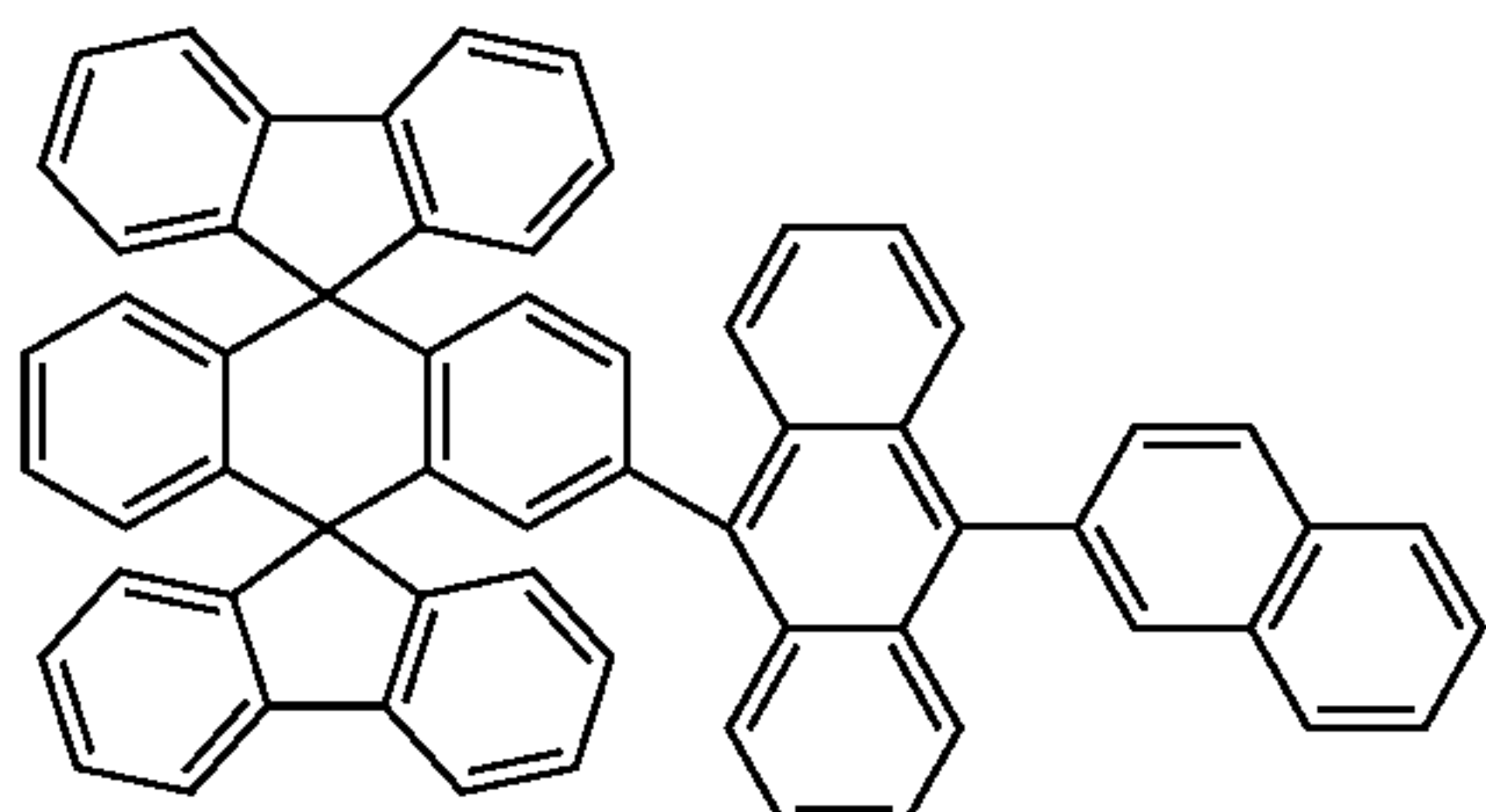
Chemical Compound 110
