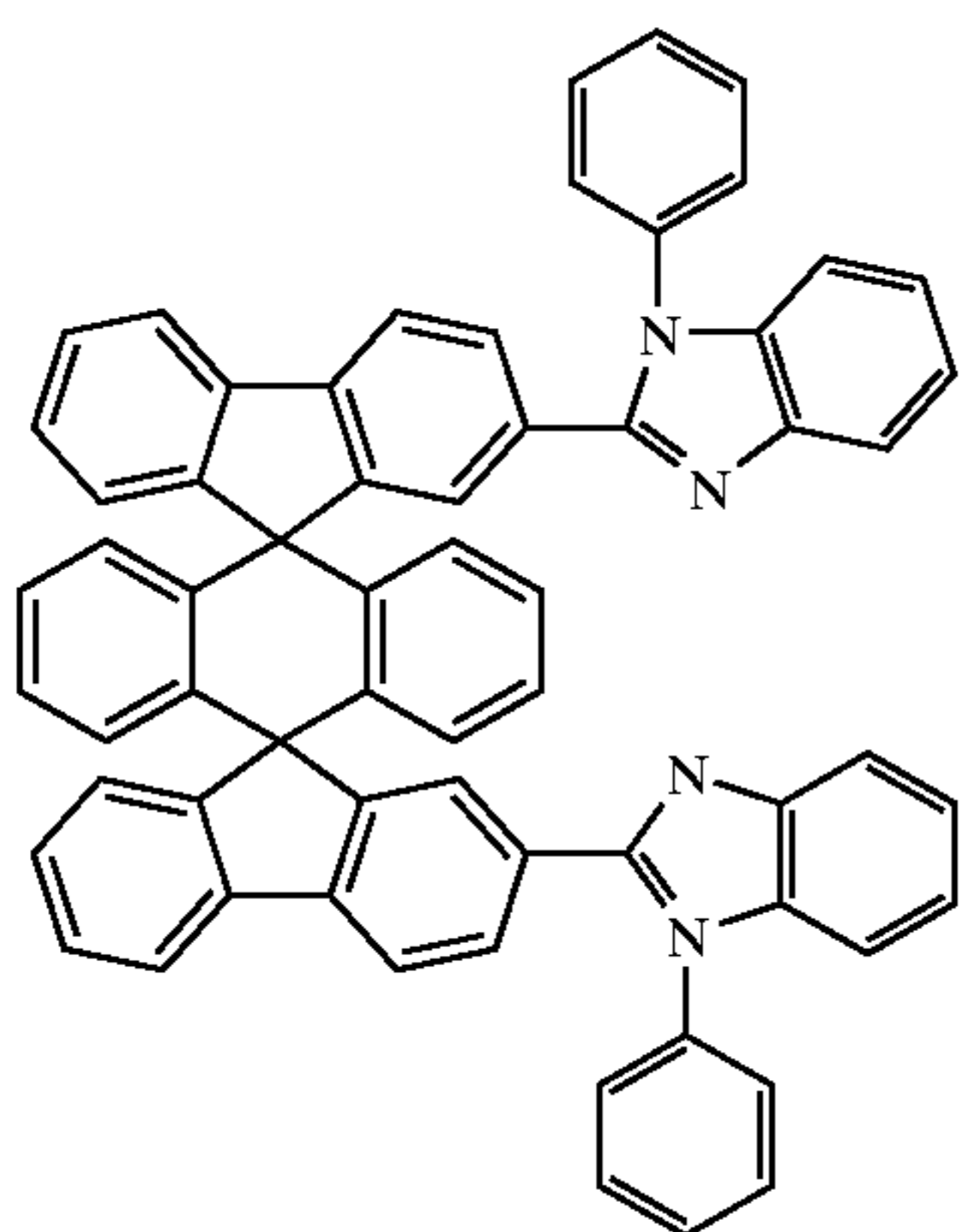
Chemical Compound 221
