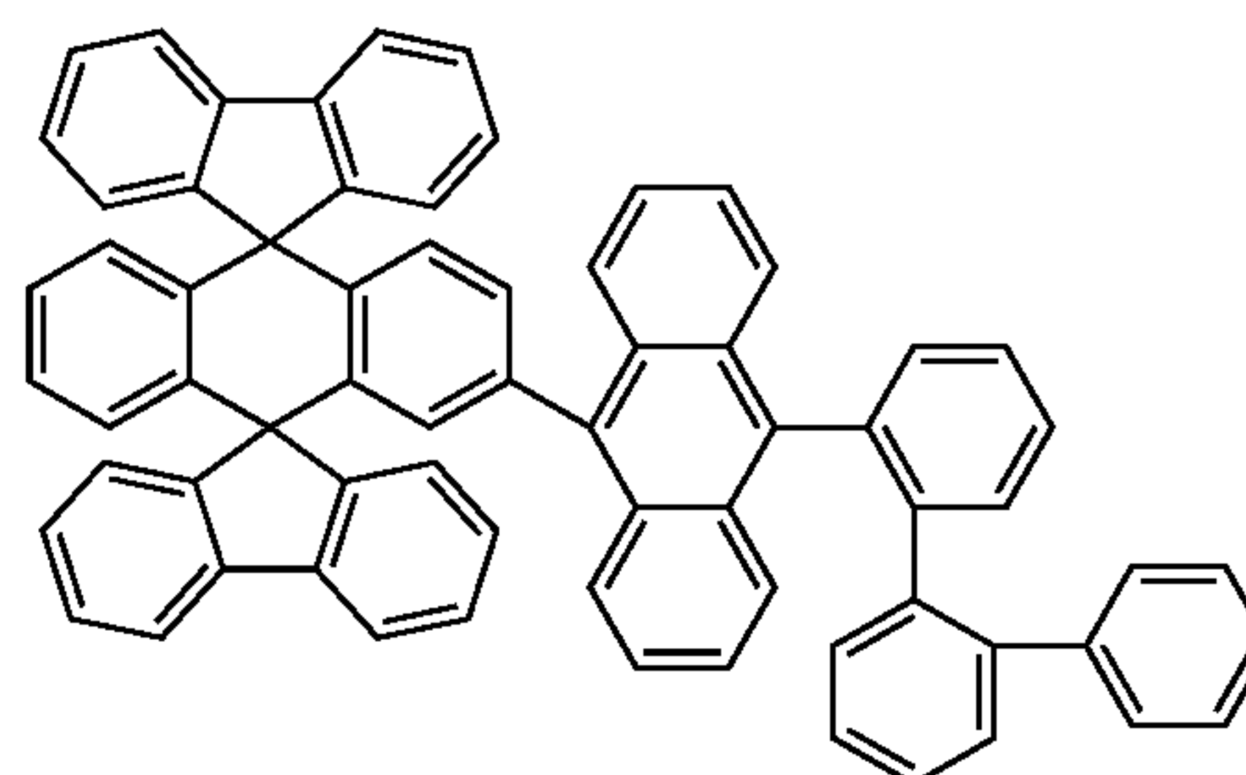
Chemical Compound 112
