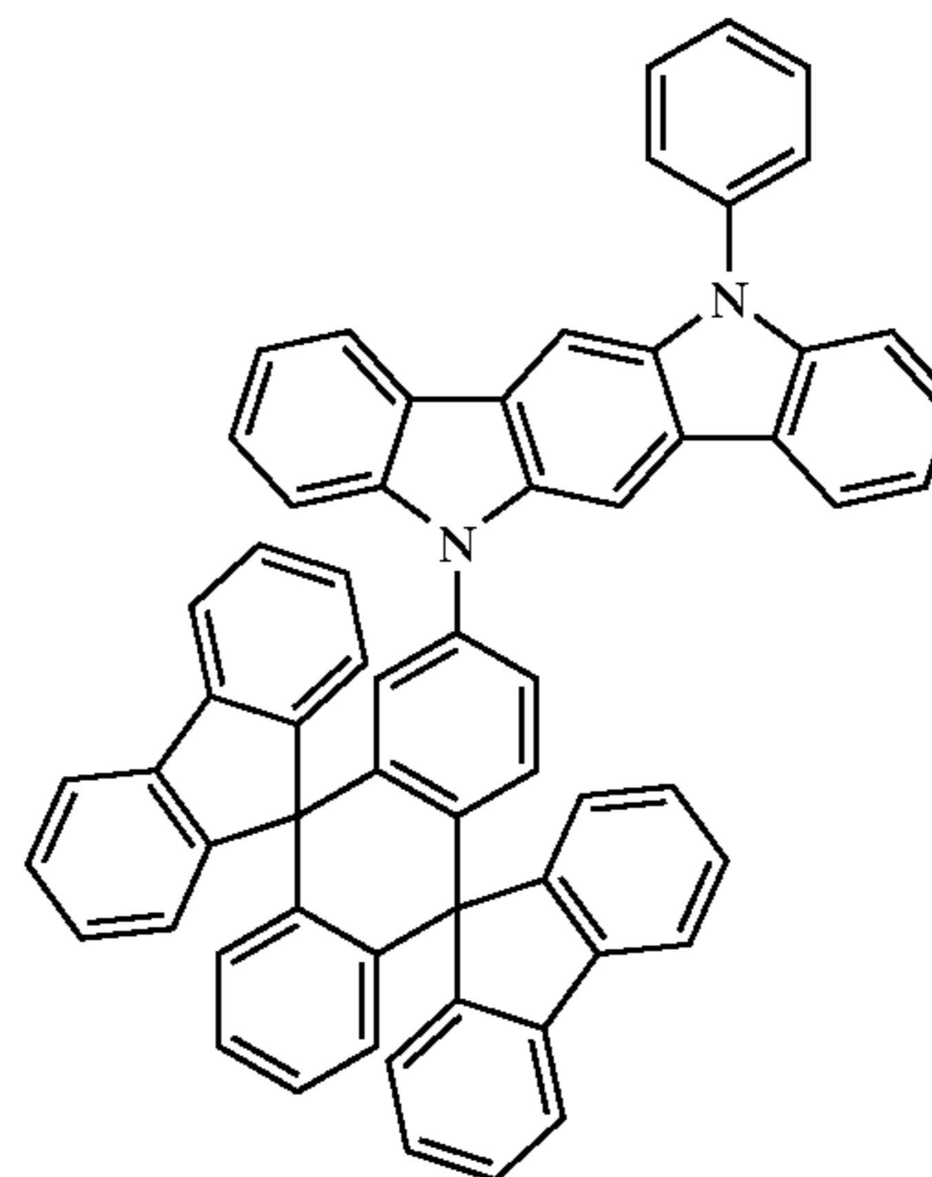
Chemical Compound 410
