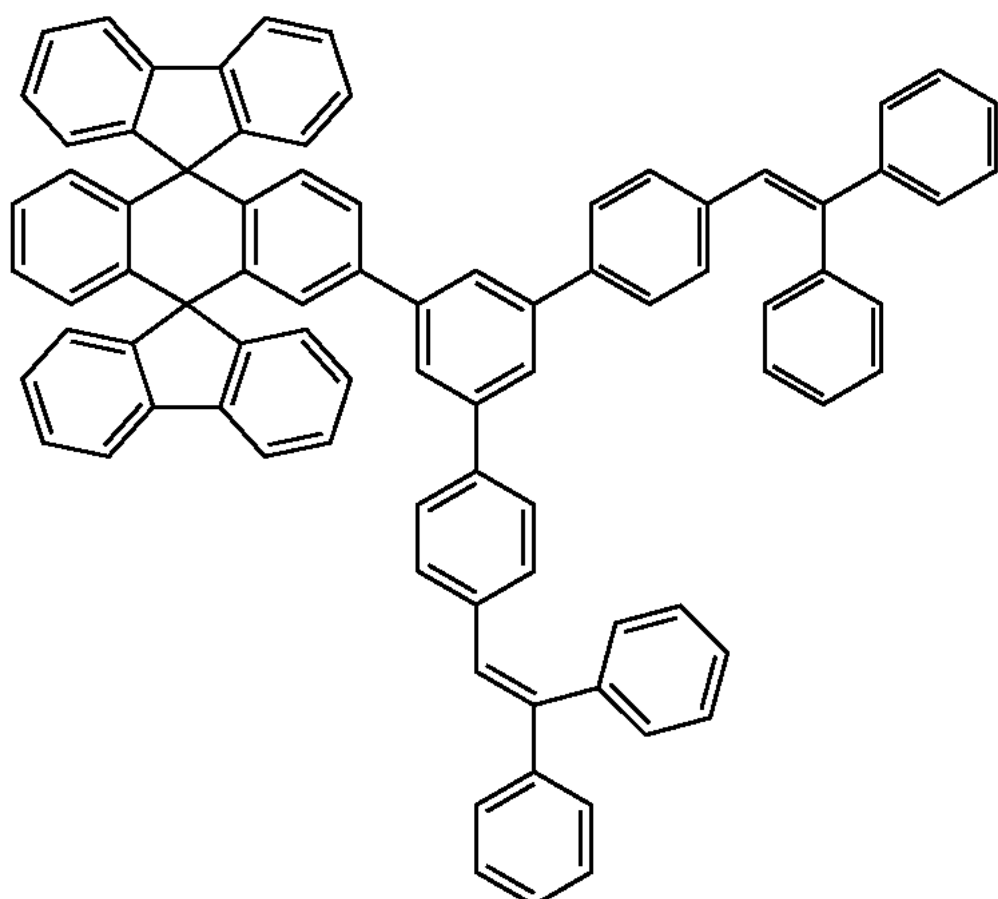
Chemical Compound 108
