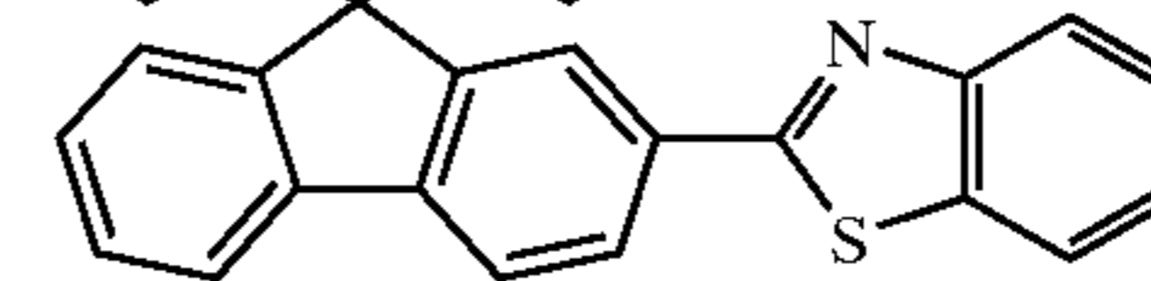
Chemical Compound 220
