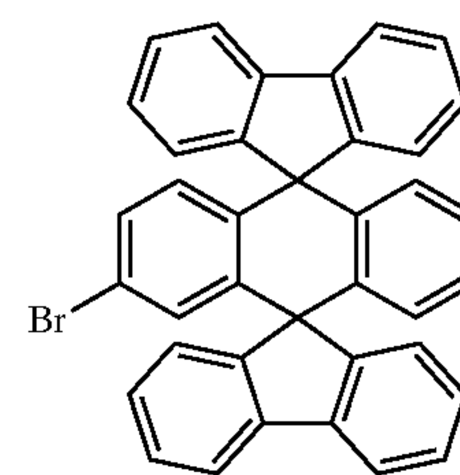
Chemical Compound 1
