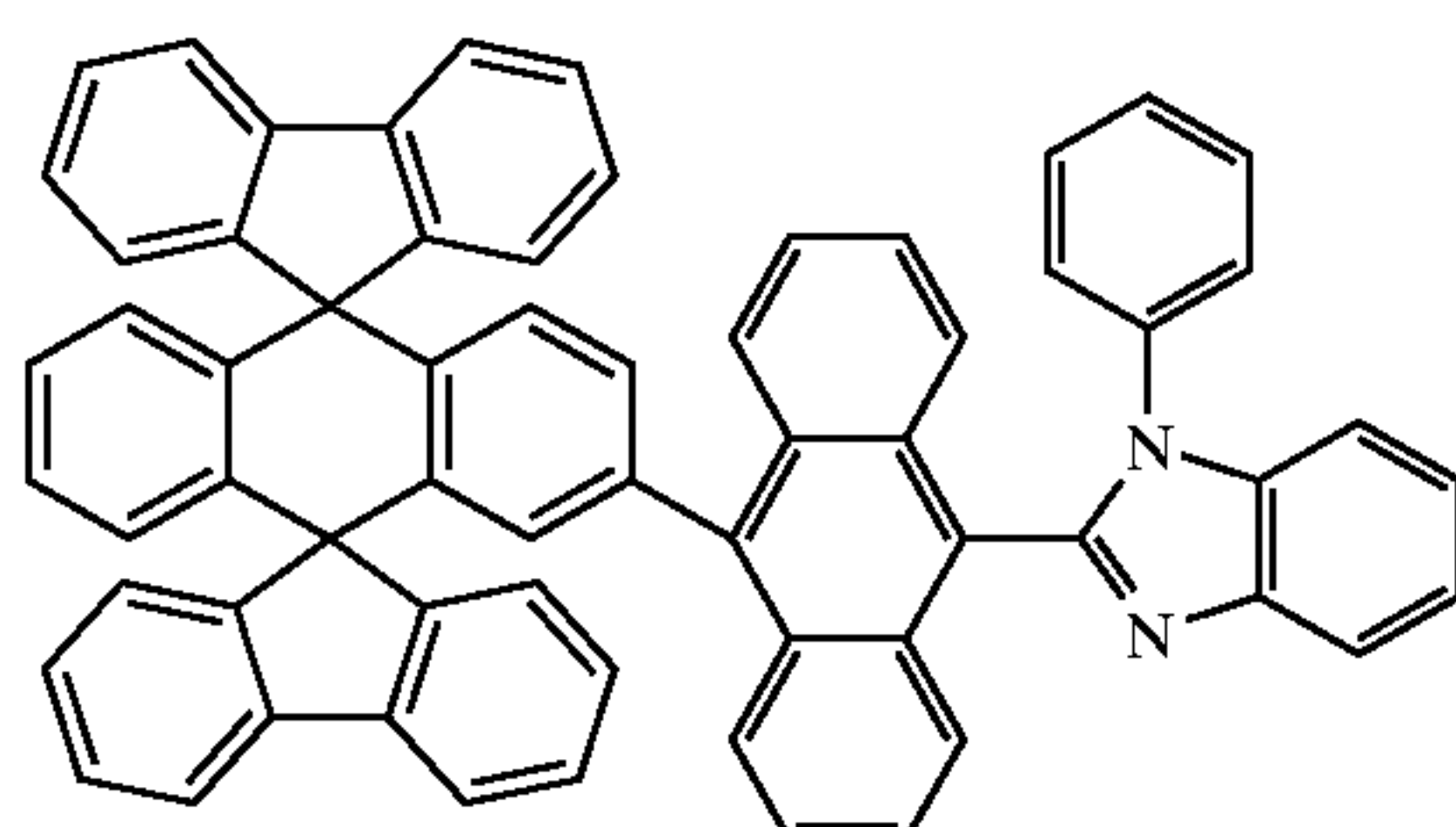
Chemical Compound 200
