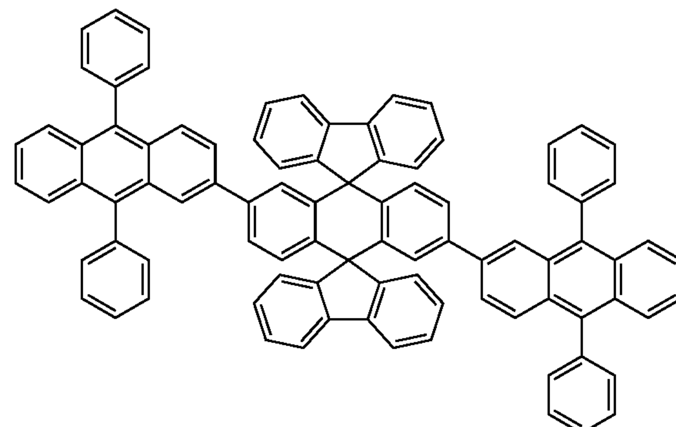
Chemical Compound 122
