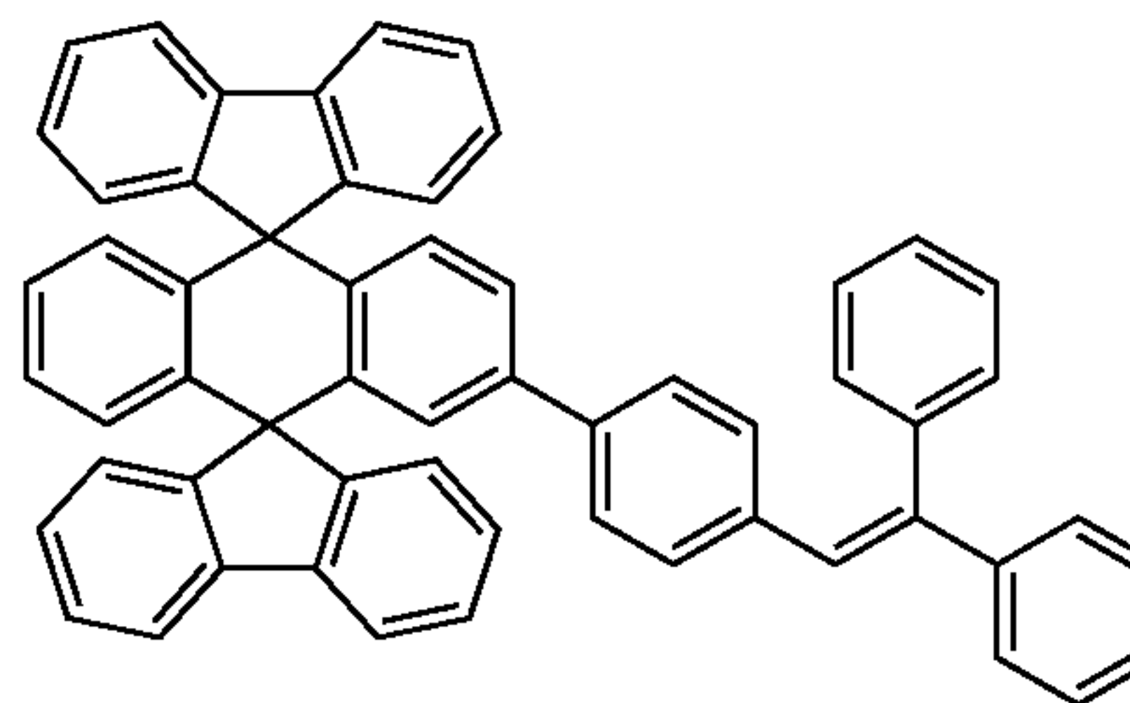
Chemical Compound 107
