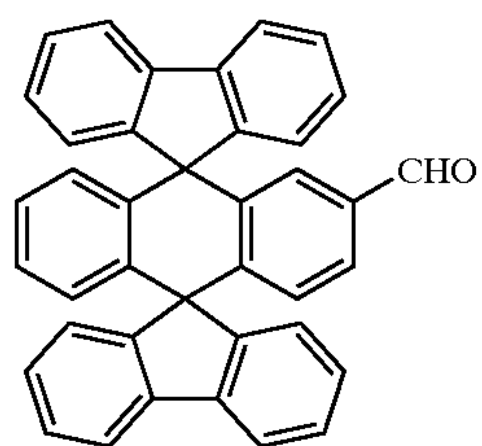
Chemical Compound 3
