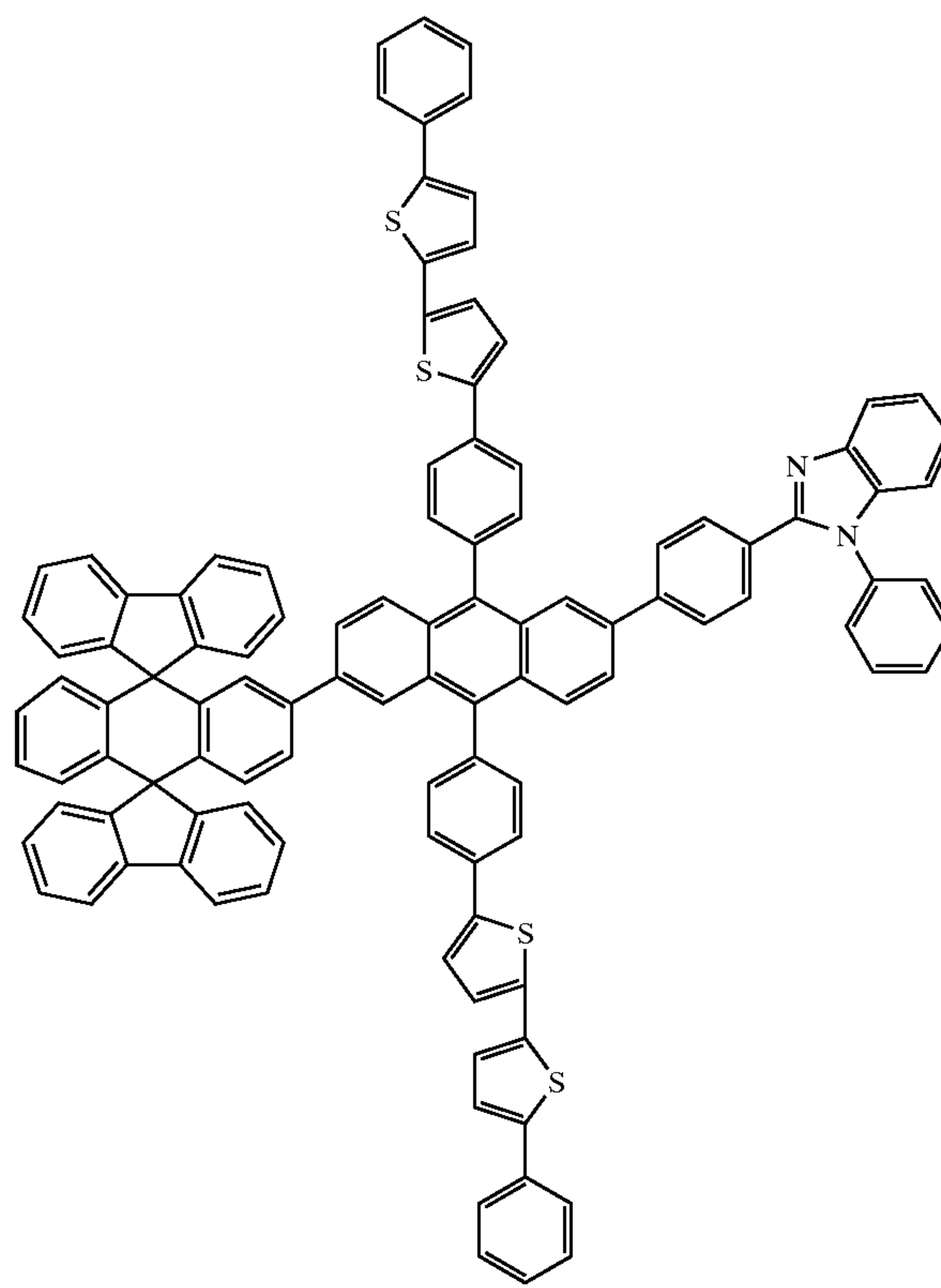
Chemical Compound 130
