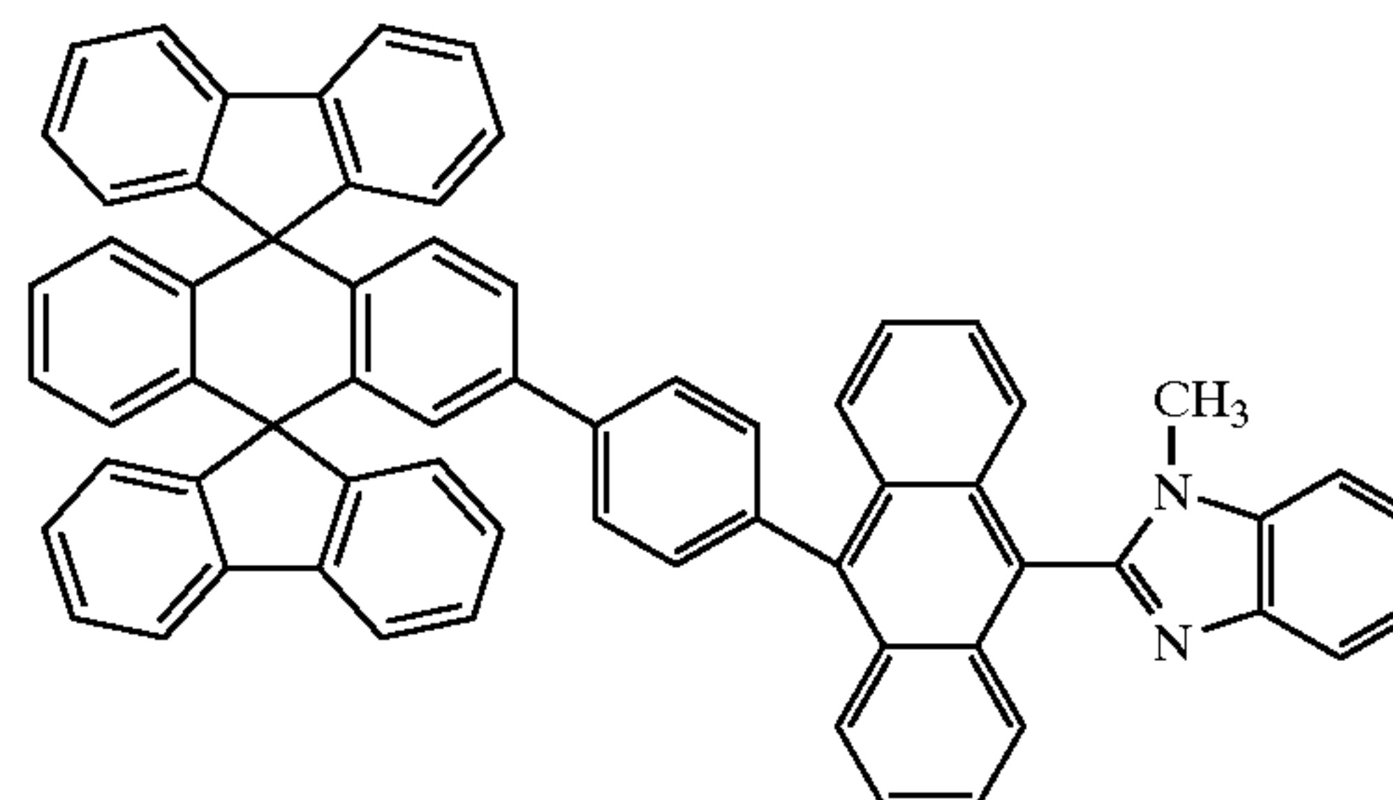
Chemical Compound 201
