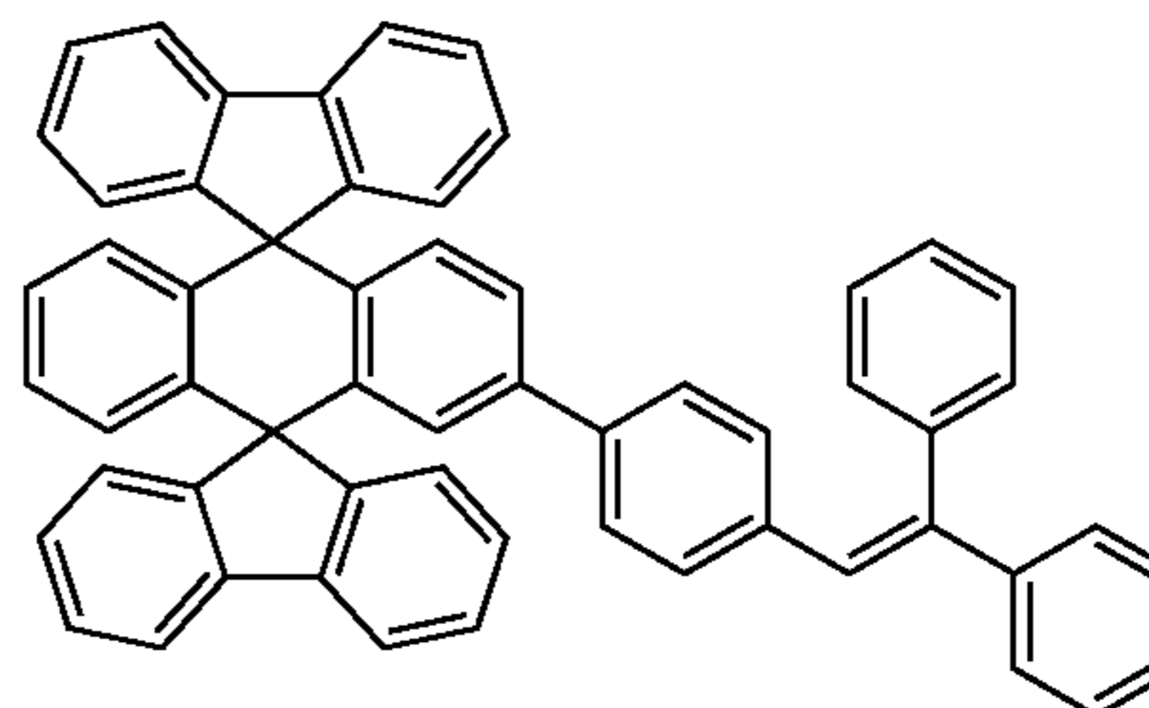
Chemical Compound 107
