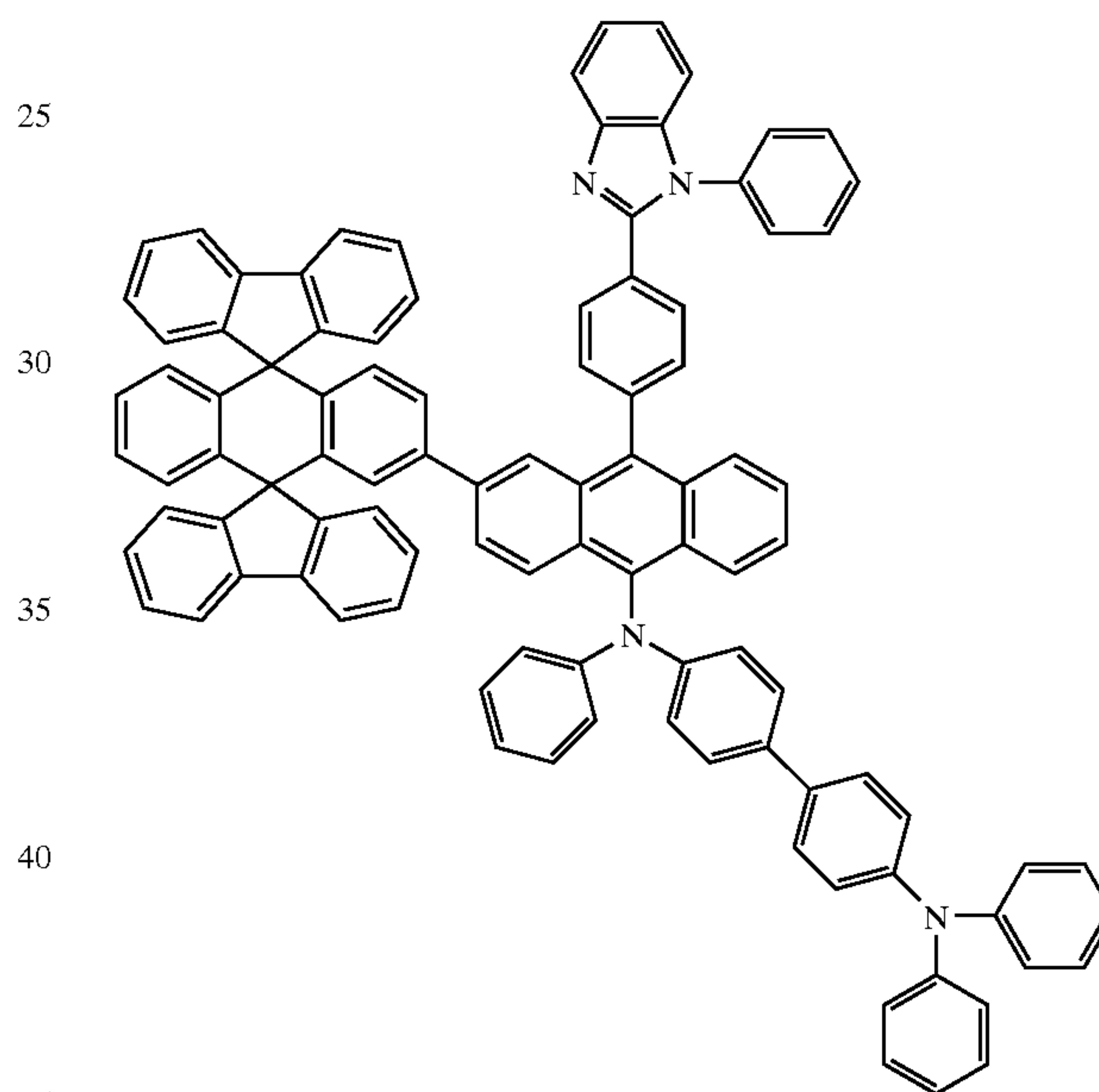
Chemical Compound 124
