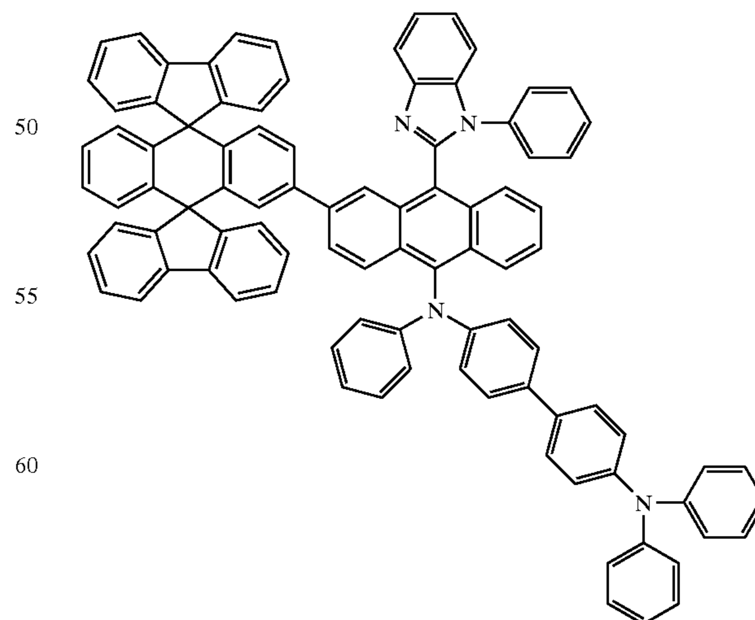
Chemical Compound 125
