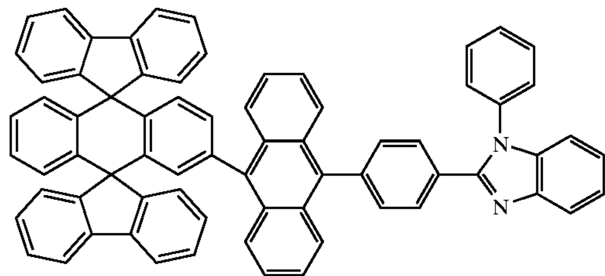
Chemical Compound 204
