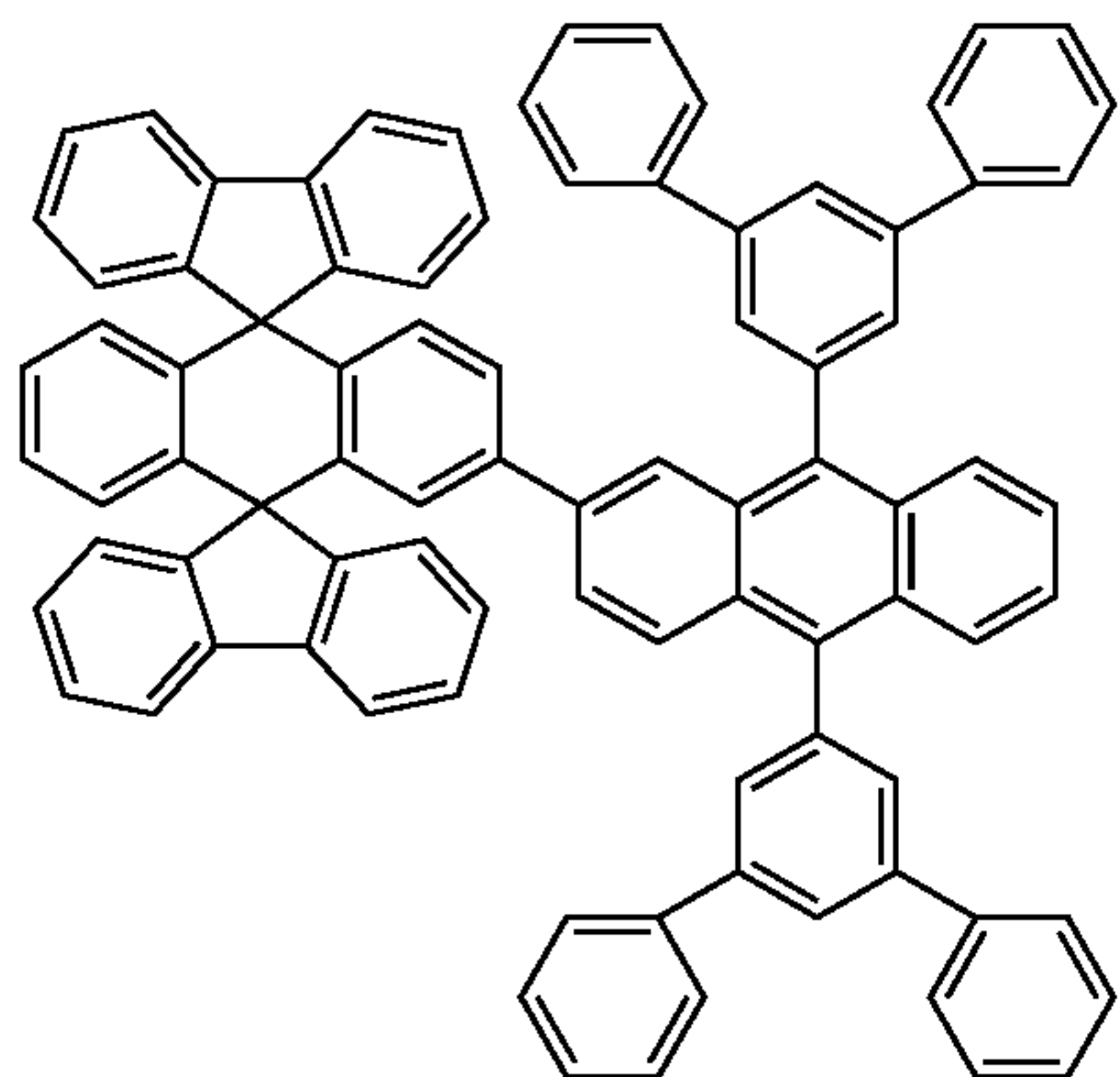
Chemical Compound 119
