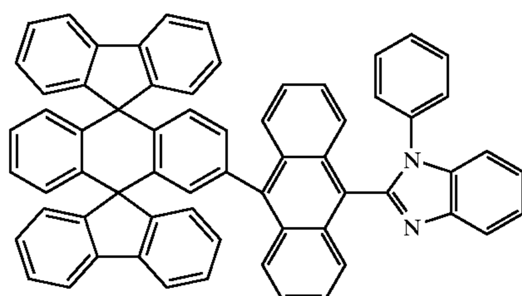
Chemical Compound 200
