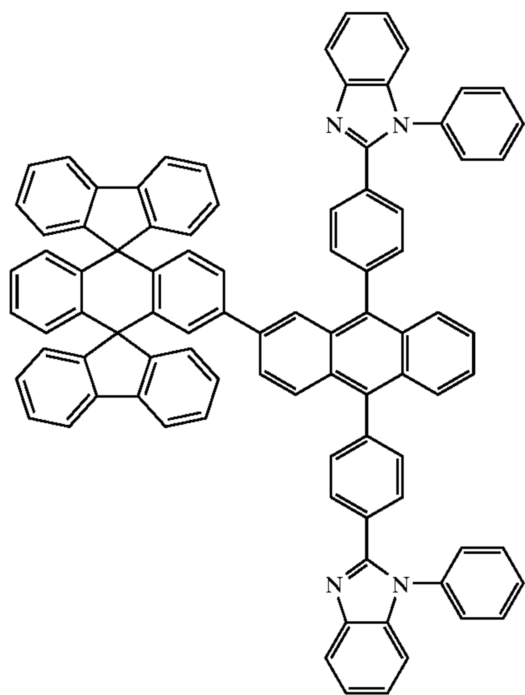
Chemical Compound 206
