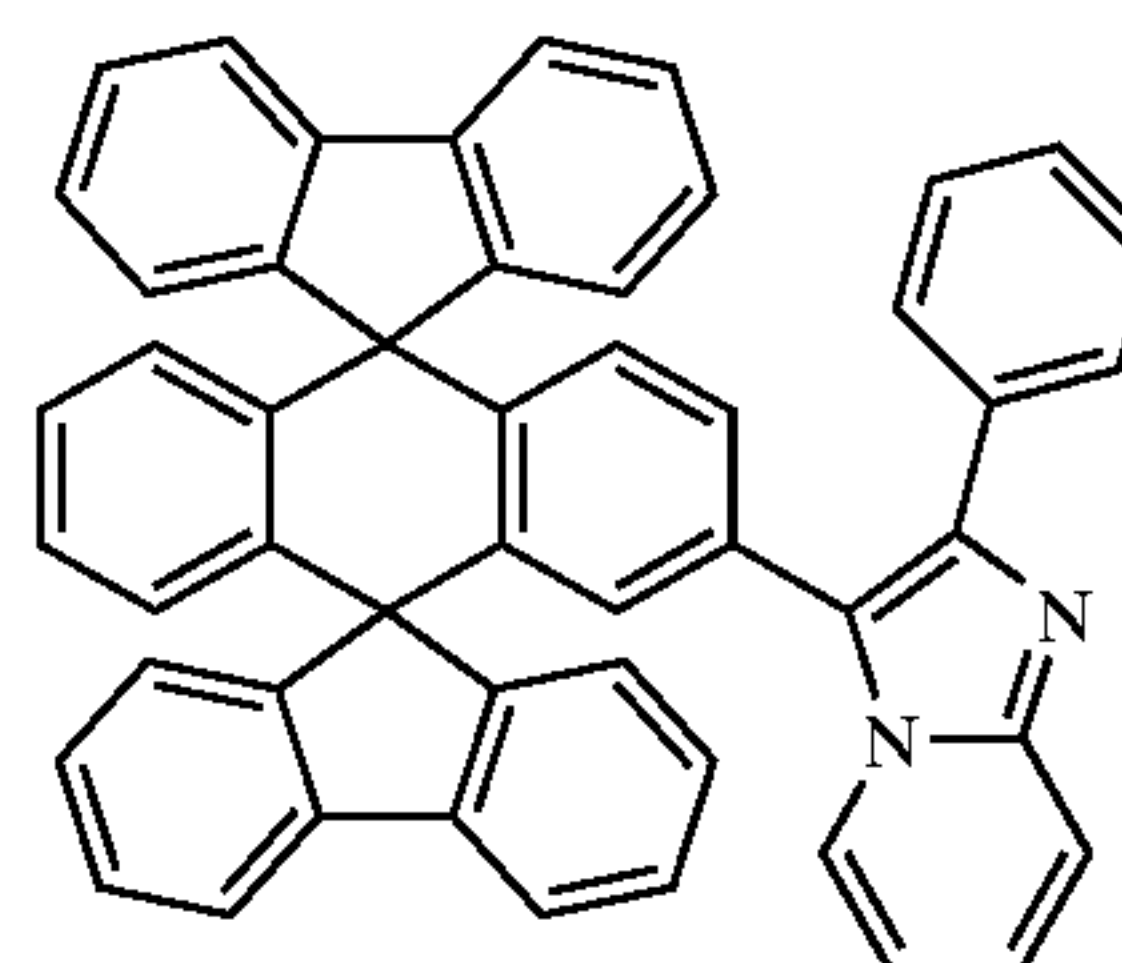
Chemical compound 412
