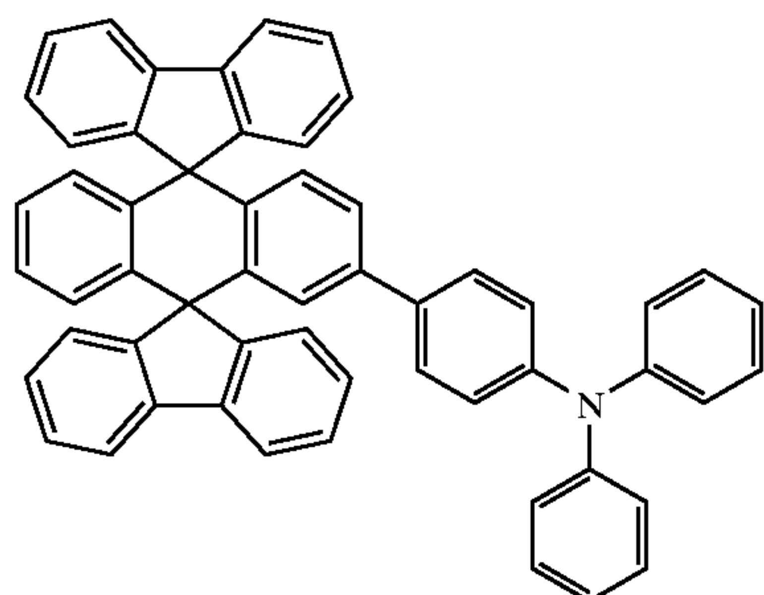
Chemical Compound 303
