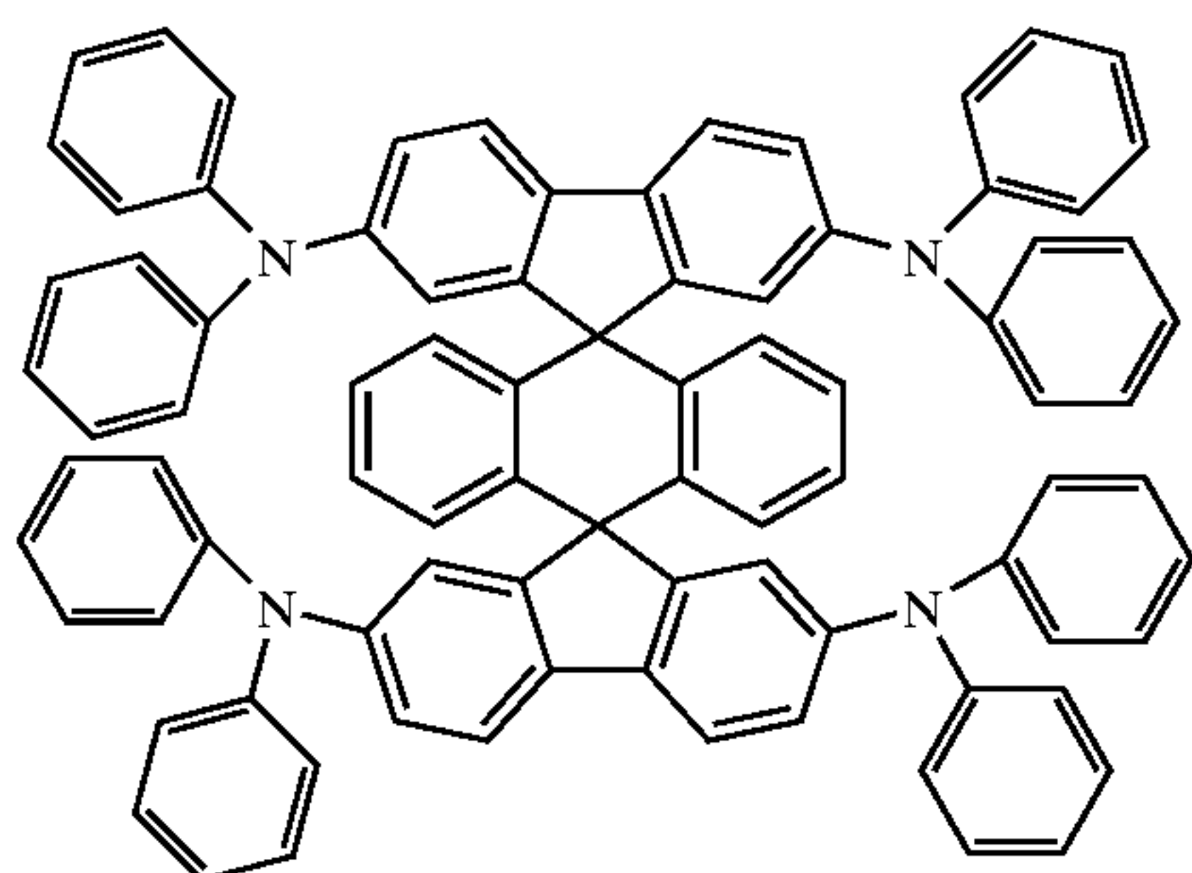
Chemical Compound 304
