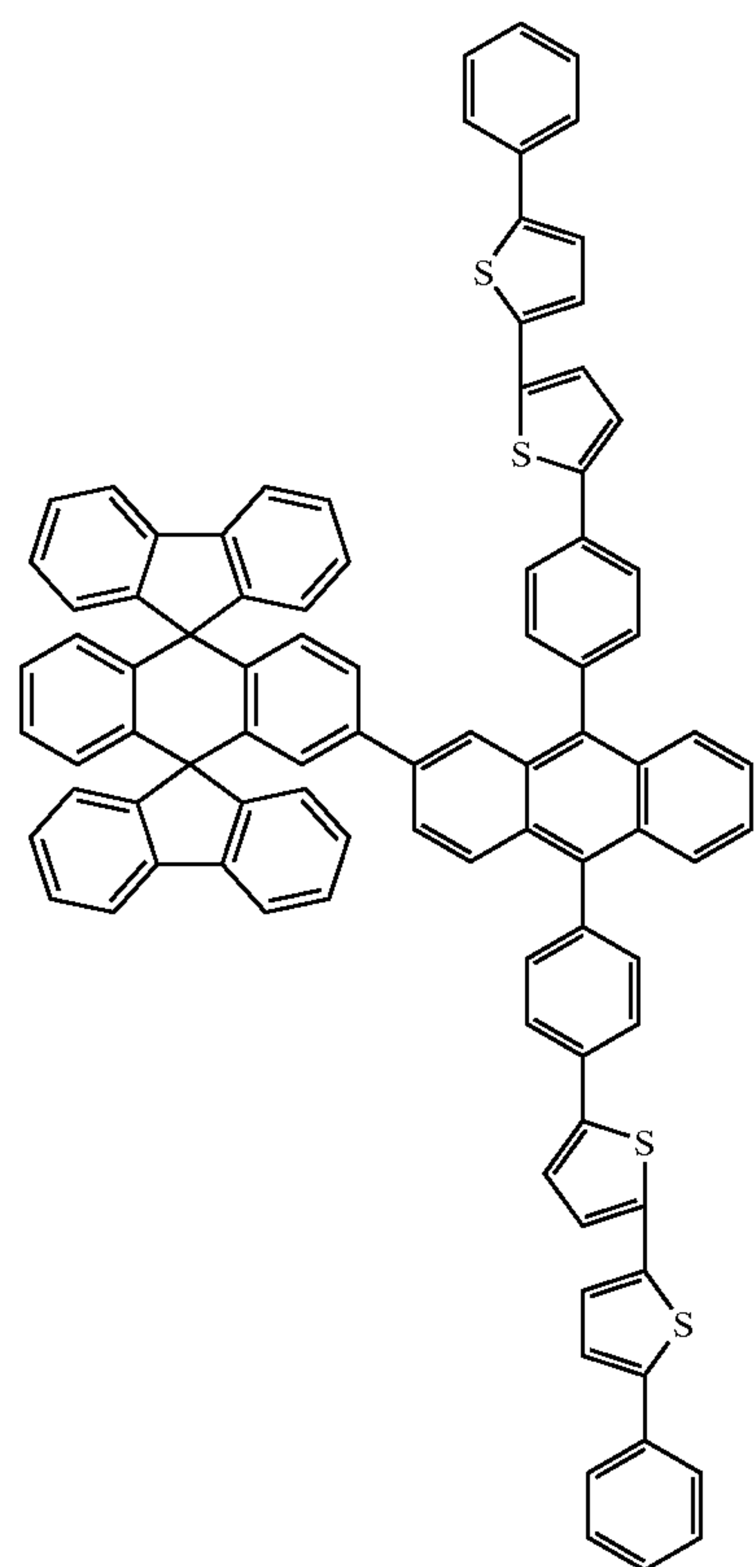
Chemical Compound 129
