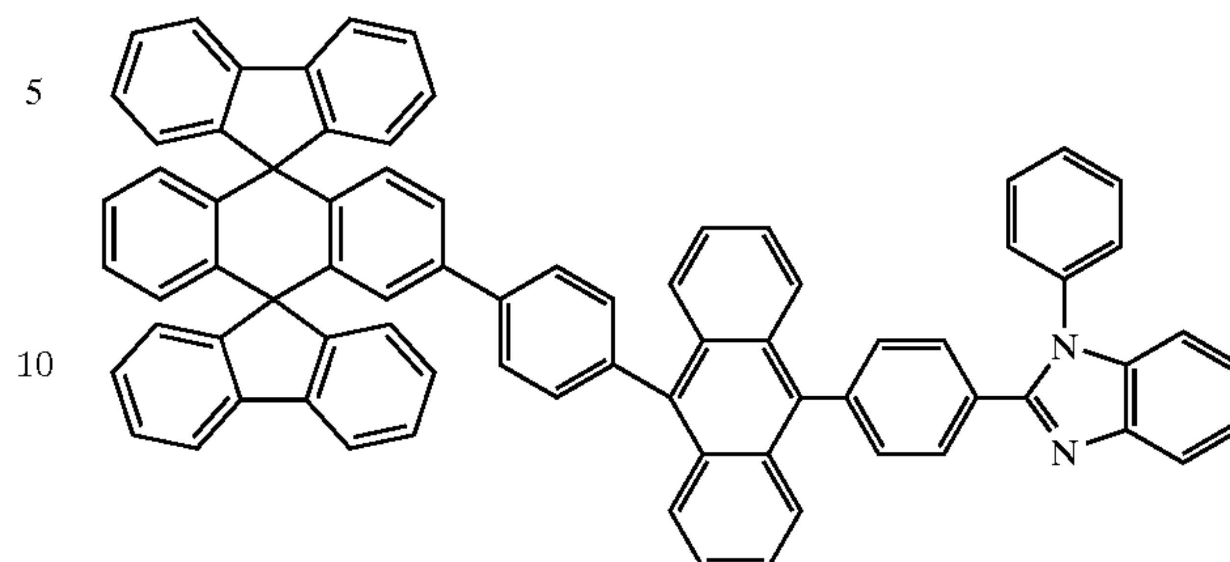
Chemical Compound 210
