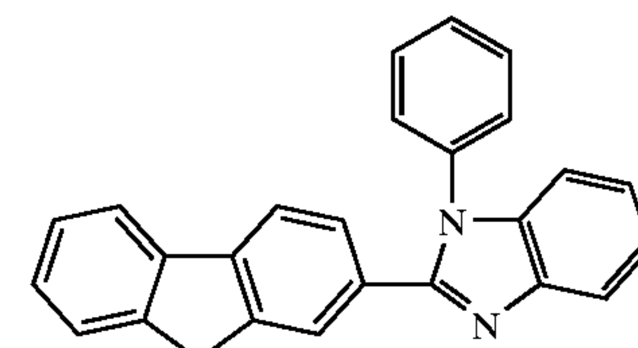
Chemical Compound 220
