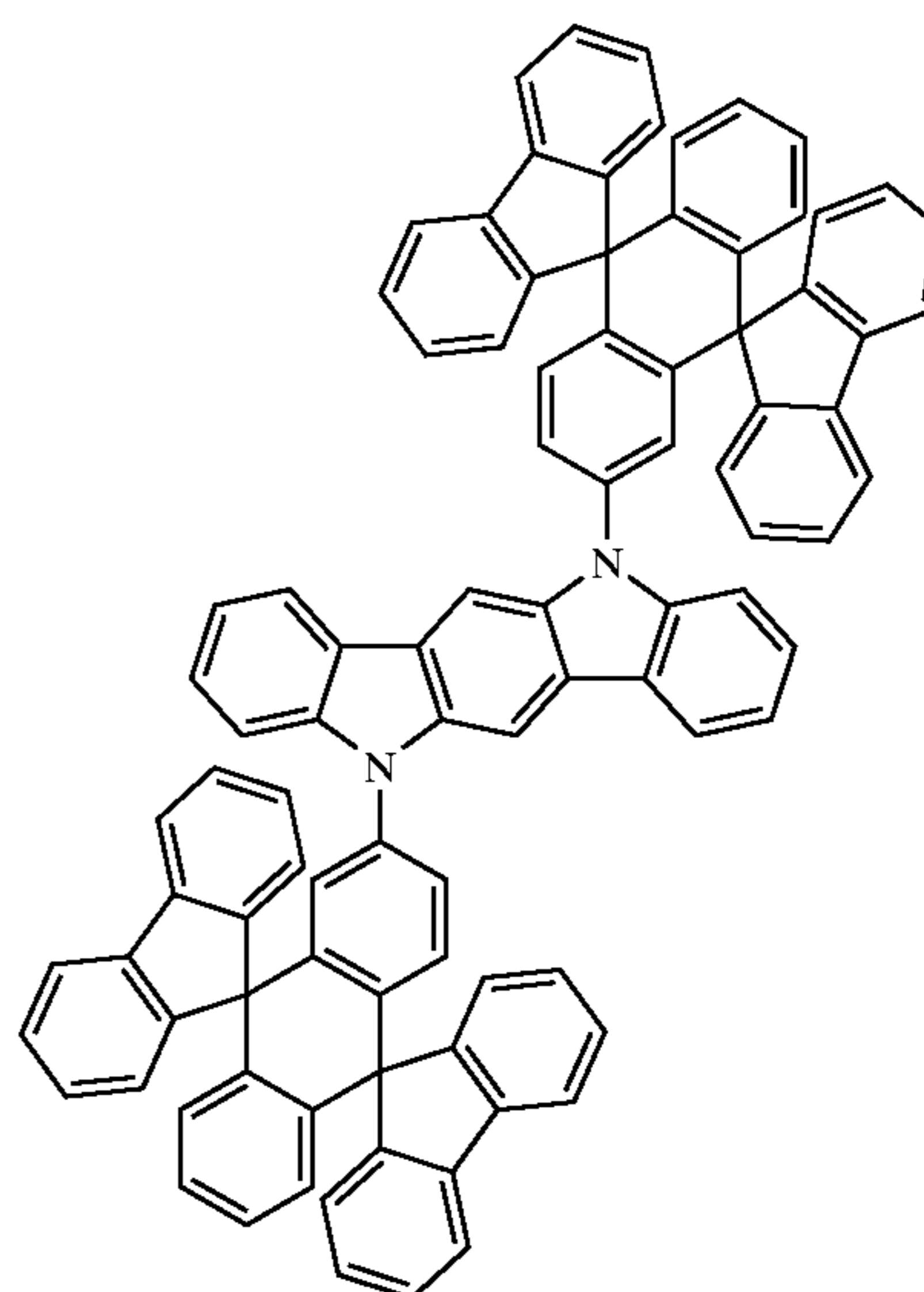
Chemical Compound 405
