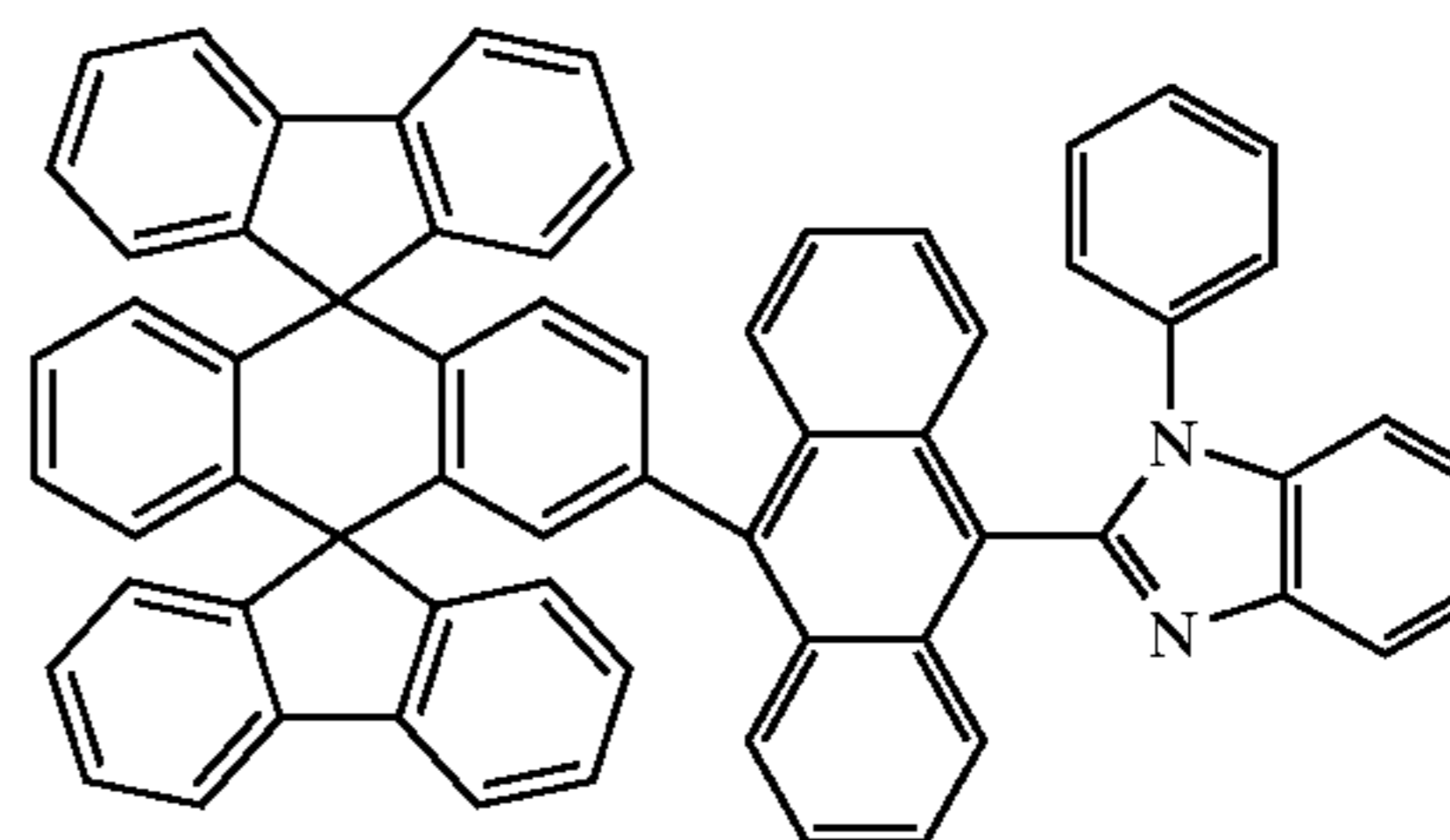
Chemical Compound 200
