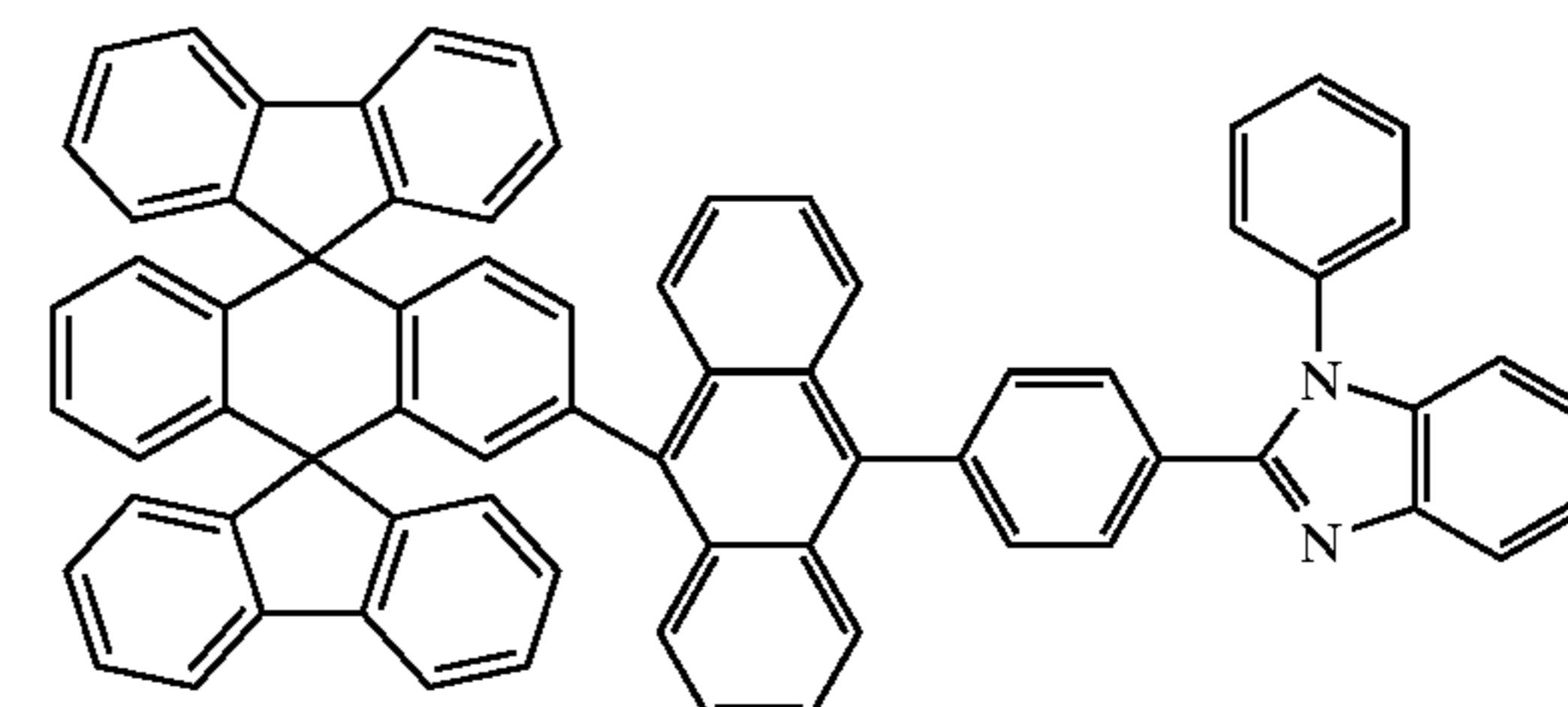
Chemical Compound 204
