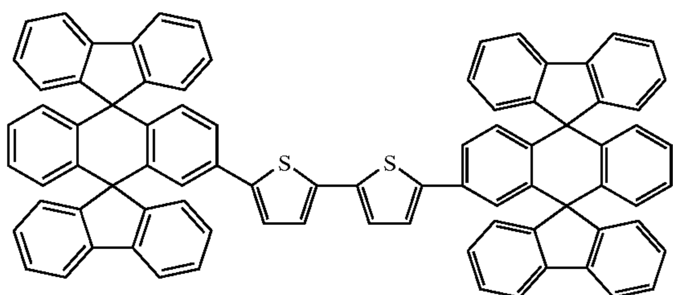
Chemical Compound 135
