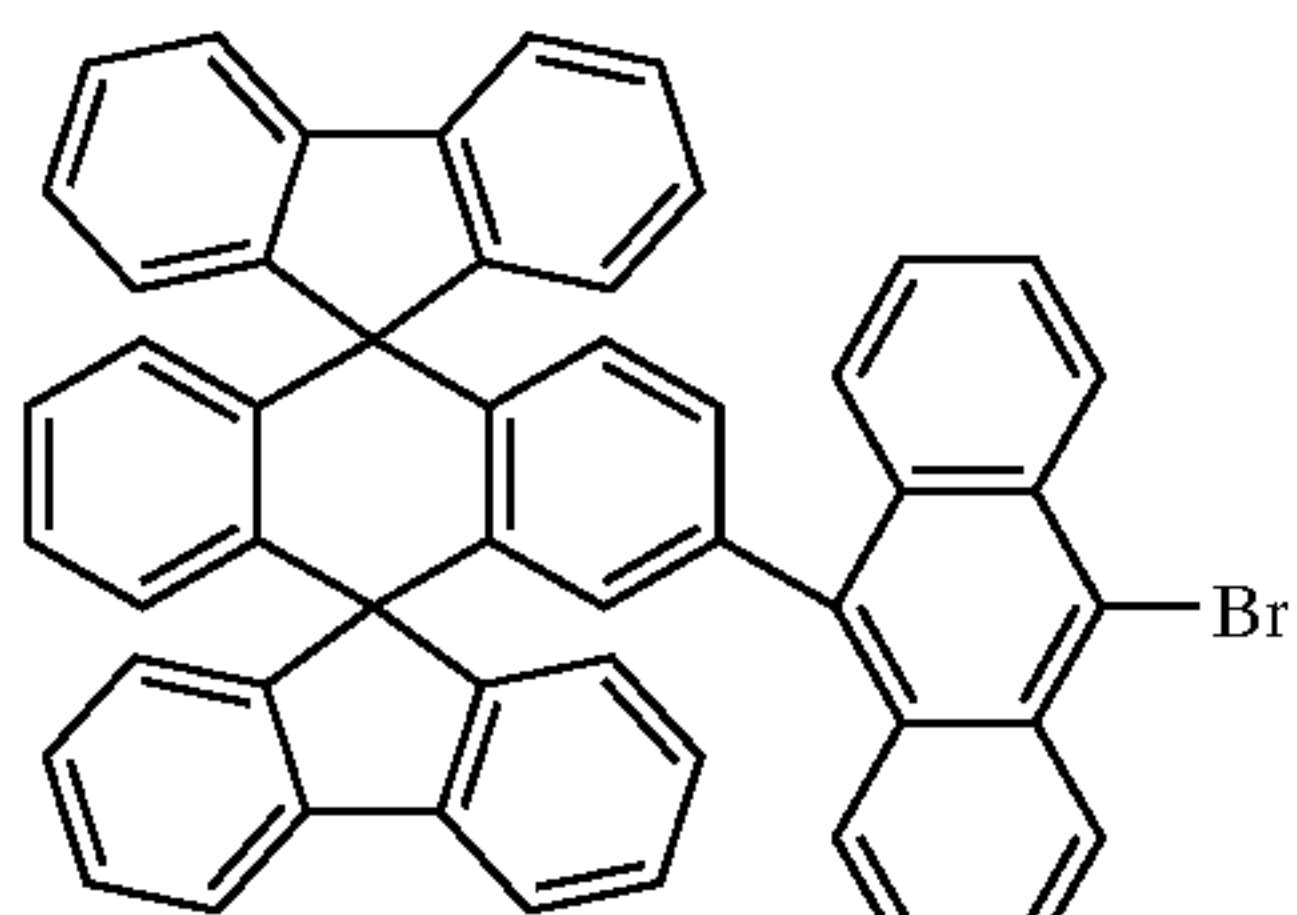
Chemical Compound 5
