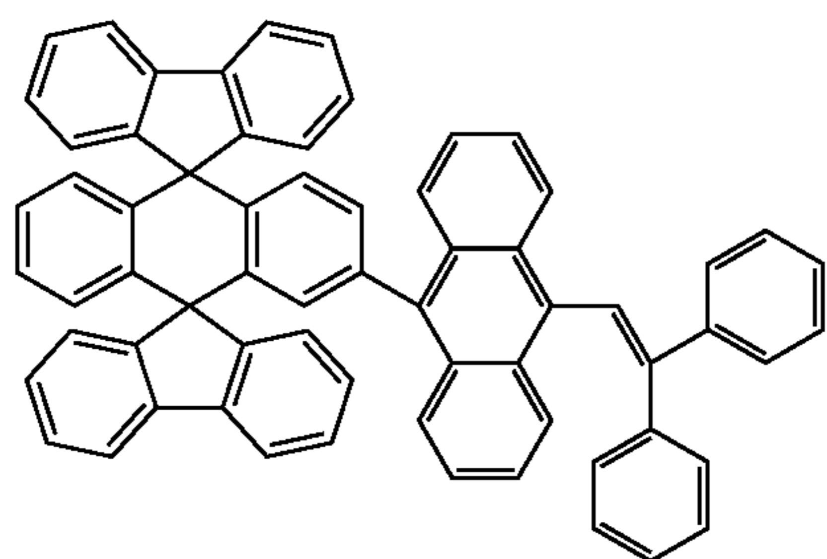
Chemical Compound 137
