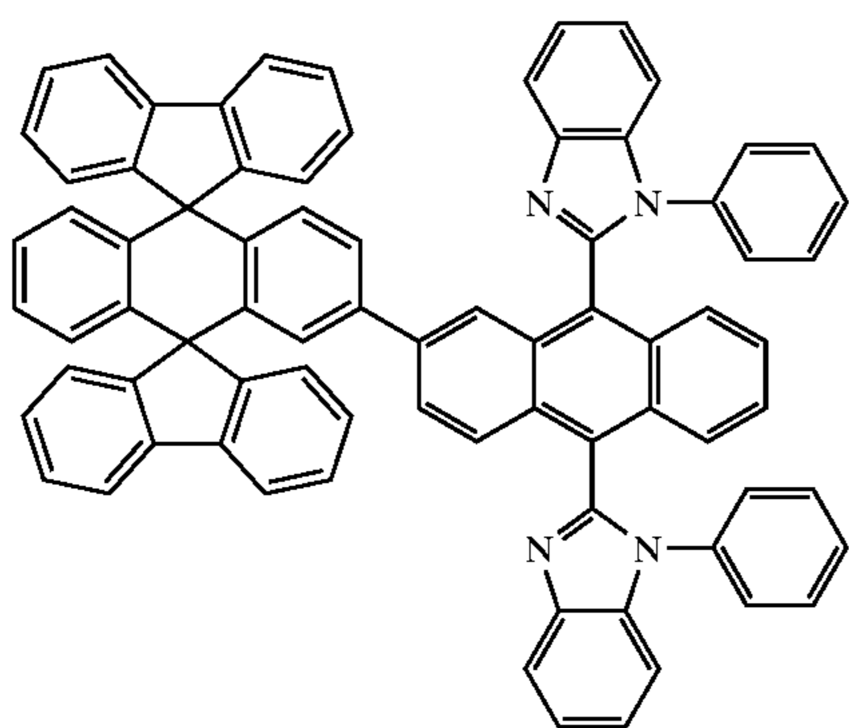
Chemical Compound 202
