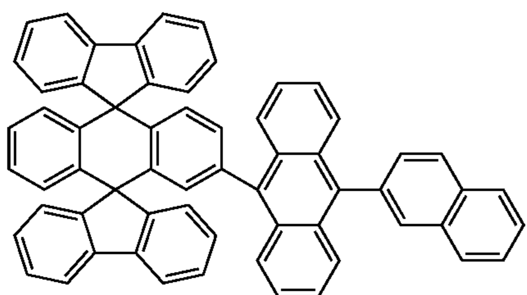
Chemical Compound 110
