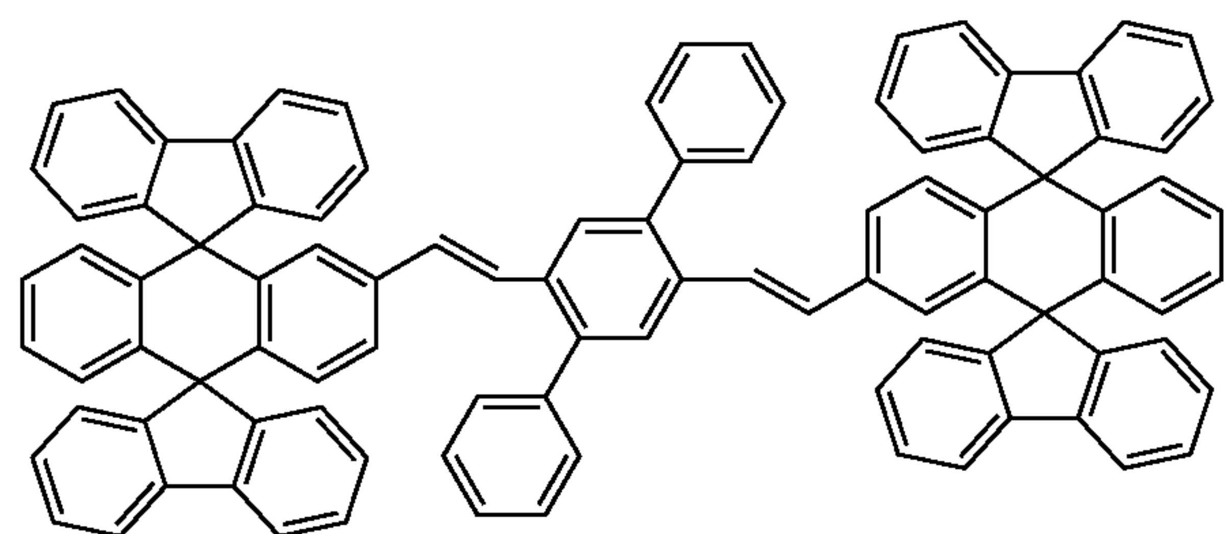
Chemical Compound 101
