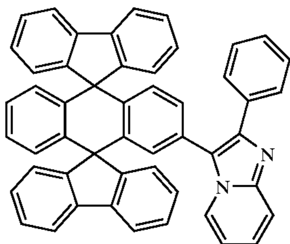
Chemical compound 412
