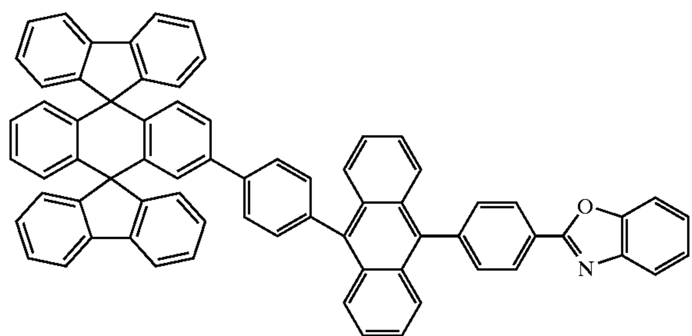
Chemical Compound 126
