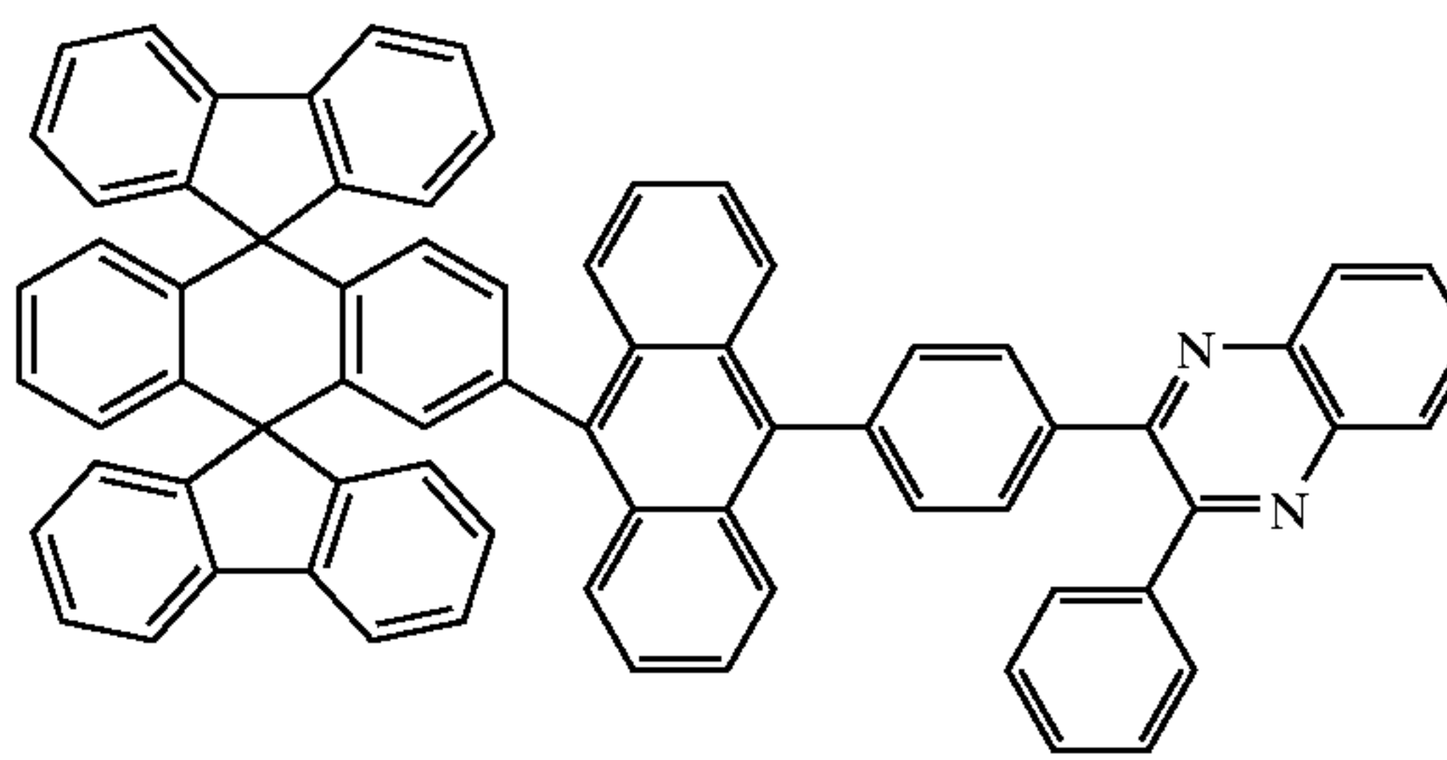
Chemical Compound 209
