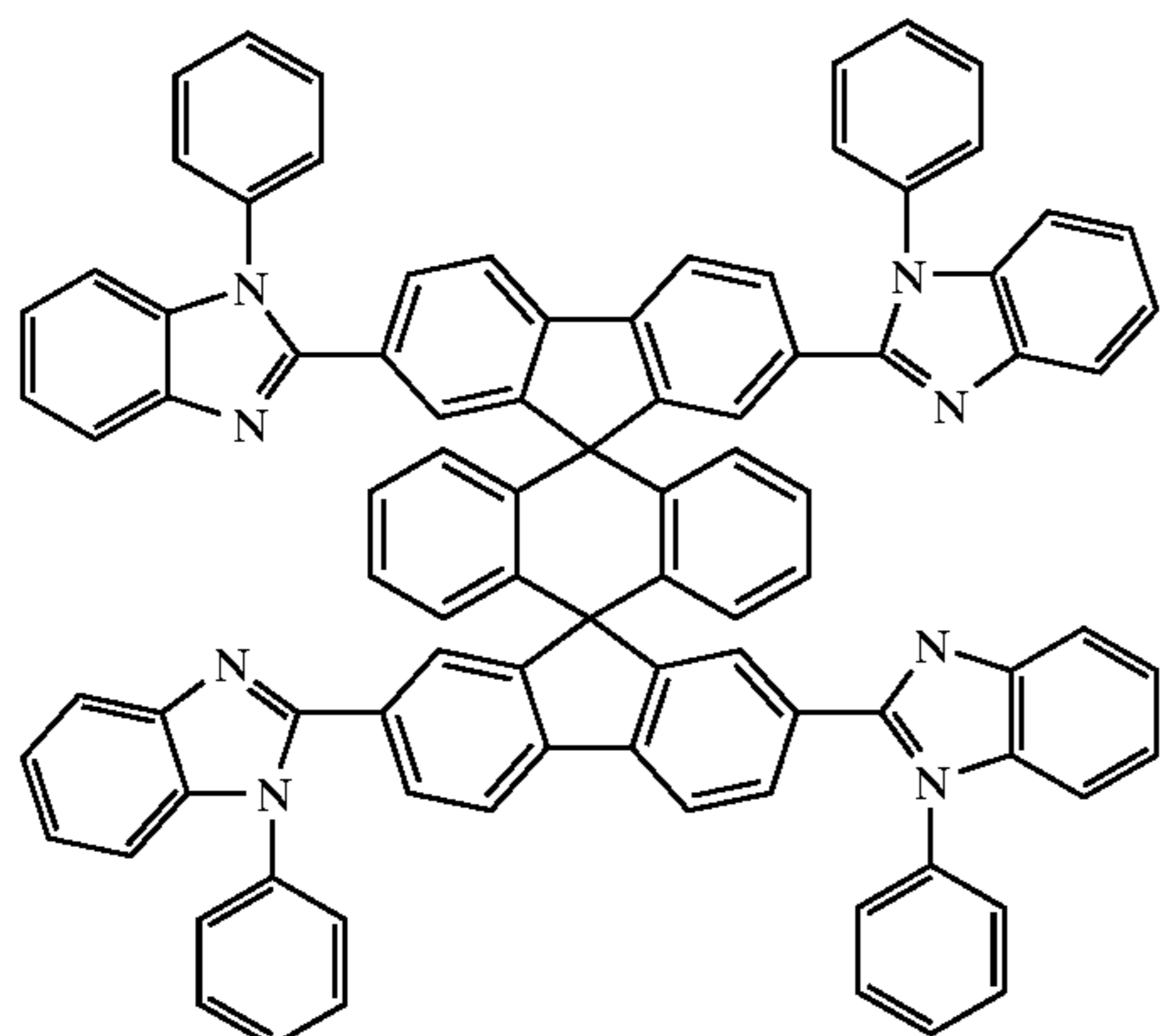
Chemical Compound 219
