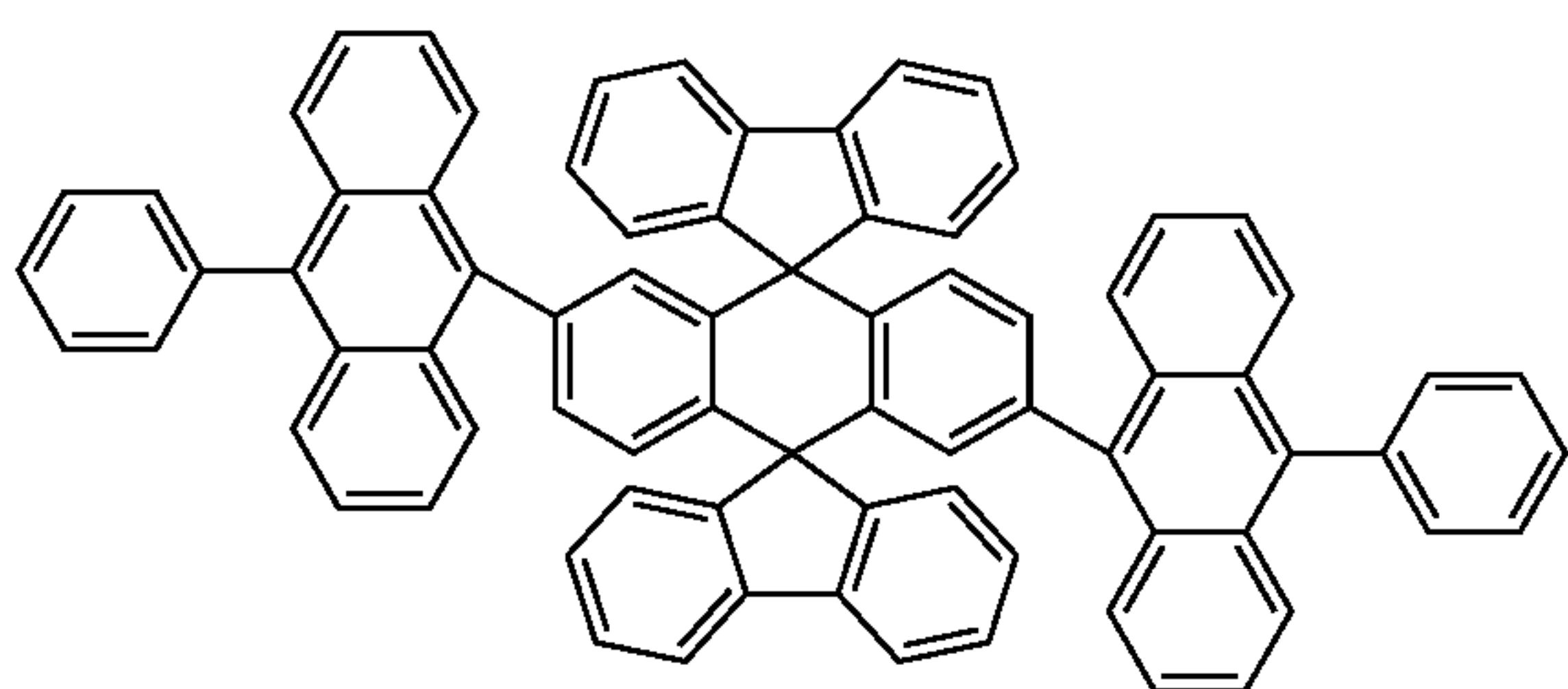
Chemical Compound 114
