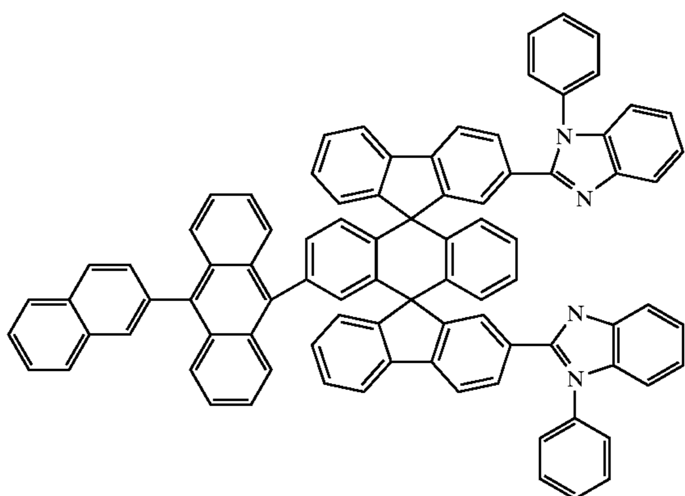
Chemical Compound 222
