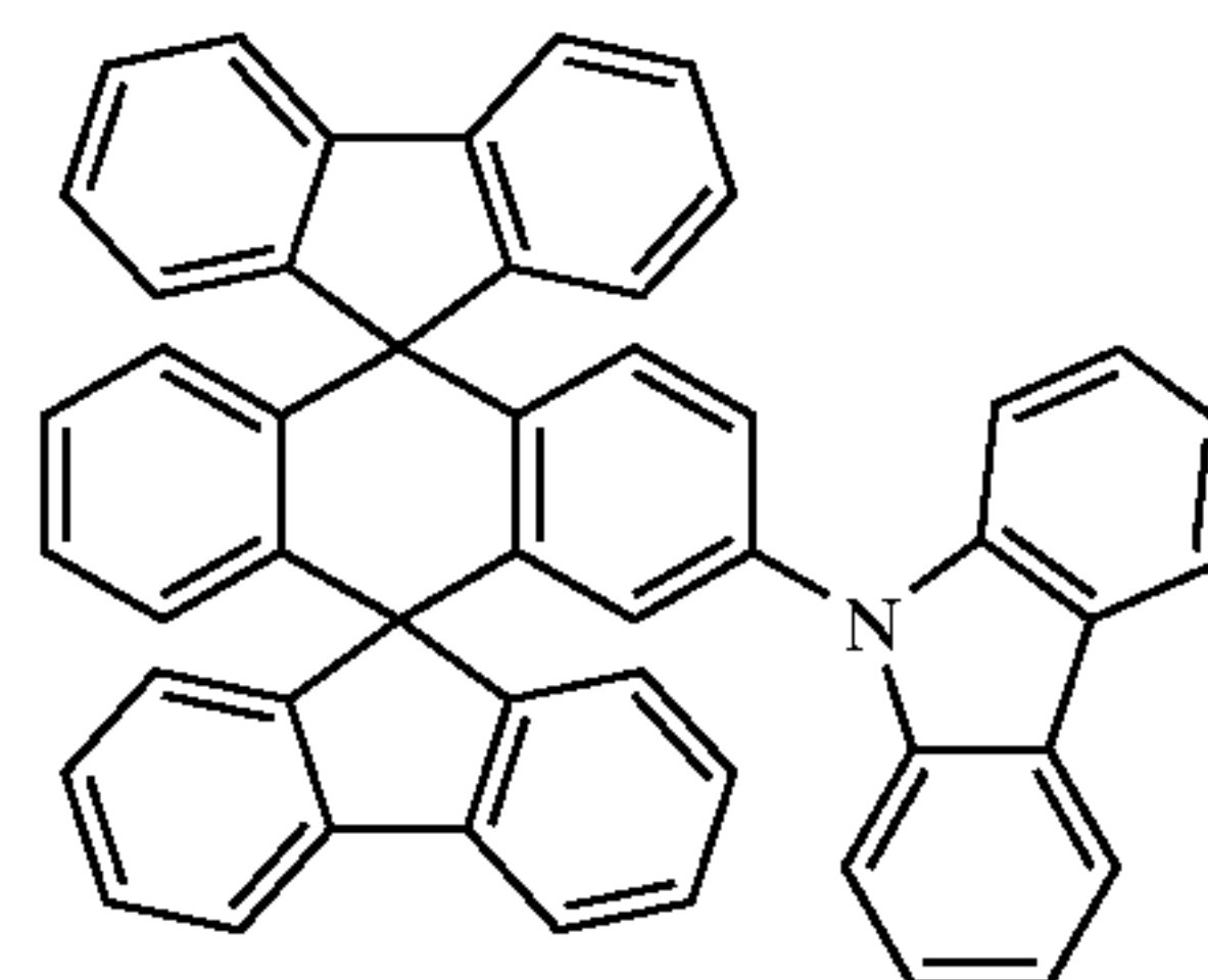
Chemical Compound 10
