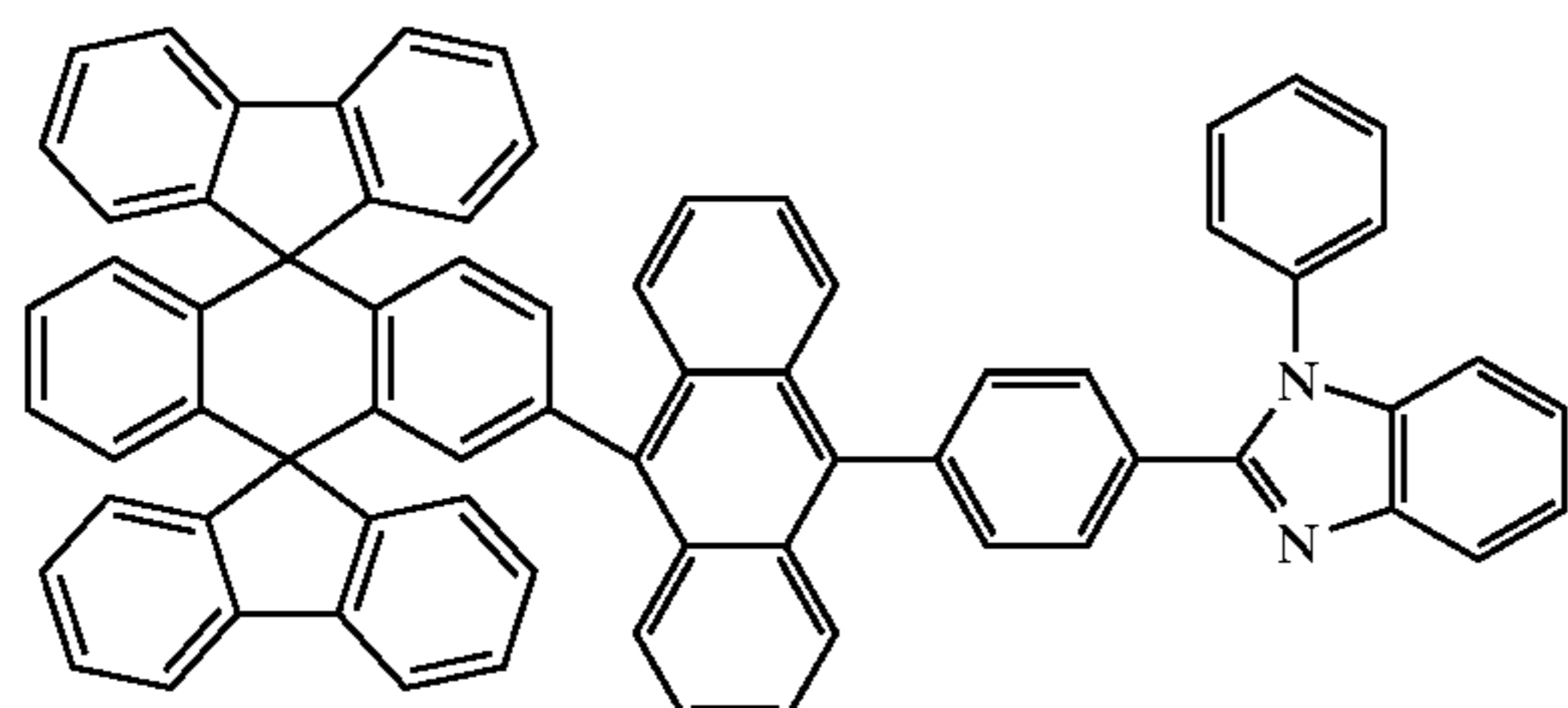
Chemical Compound 204
