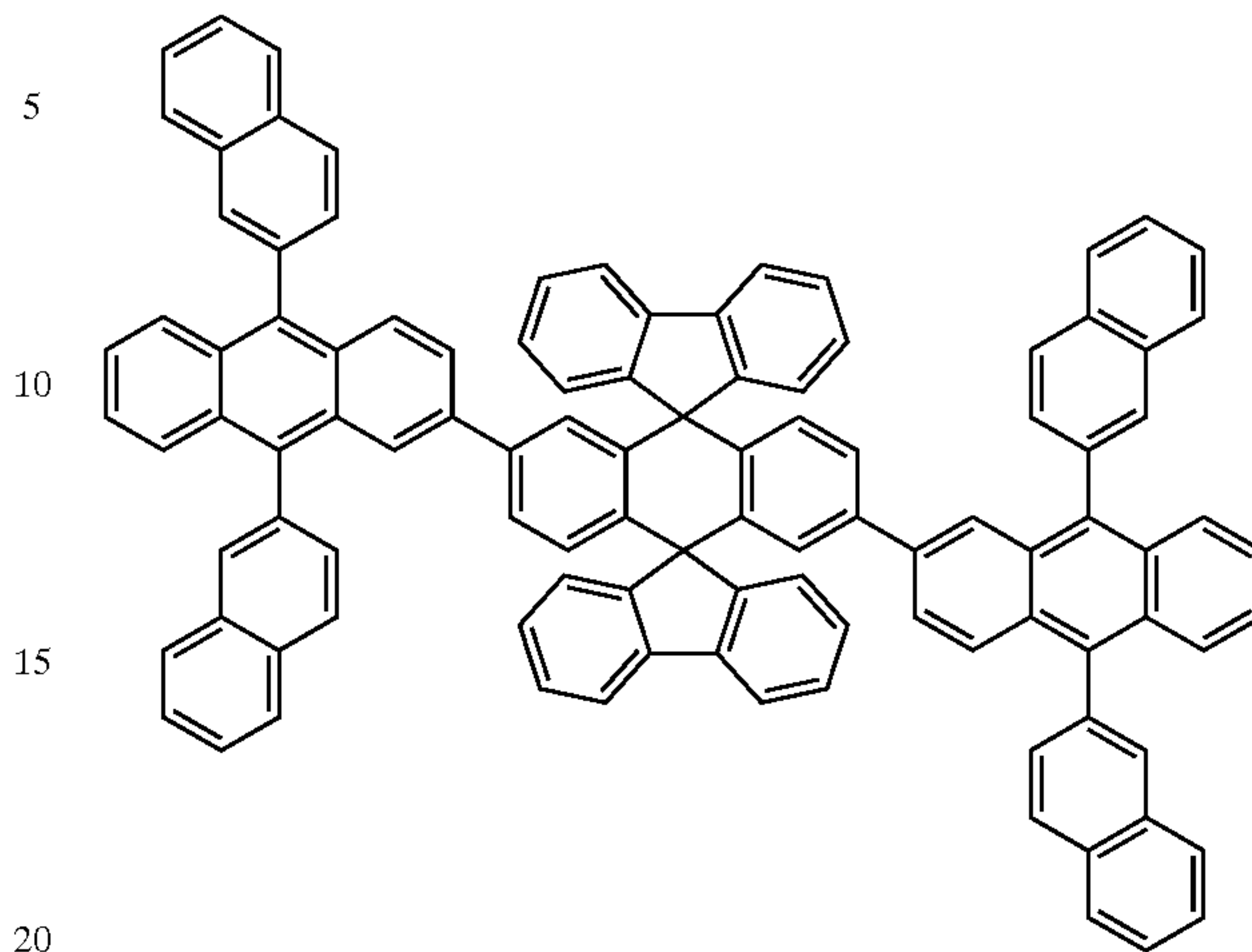
Chemical Compound 123
