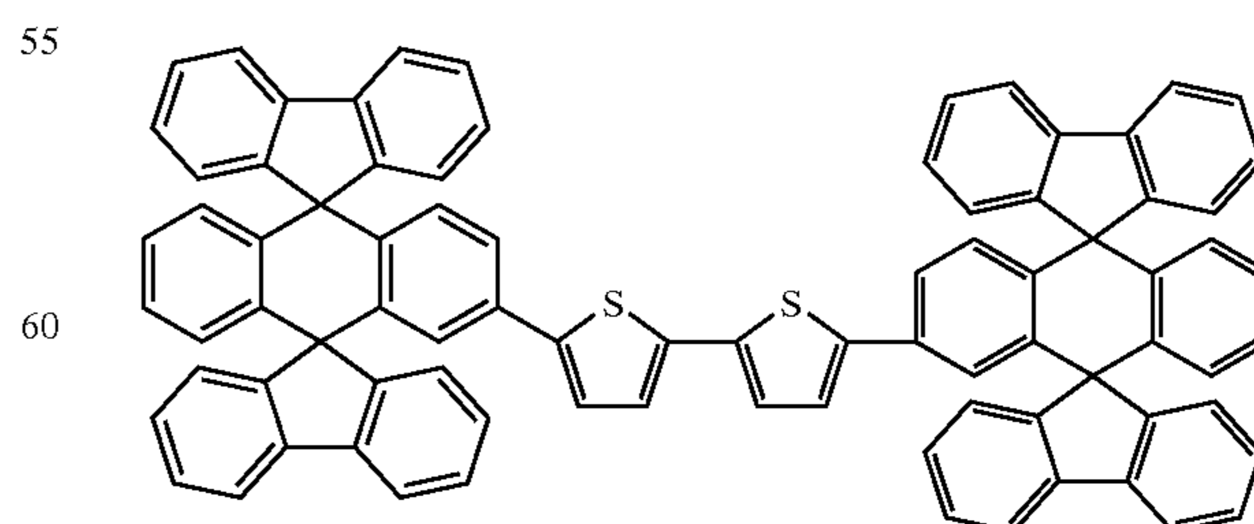
Chemical Compound 135
