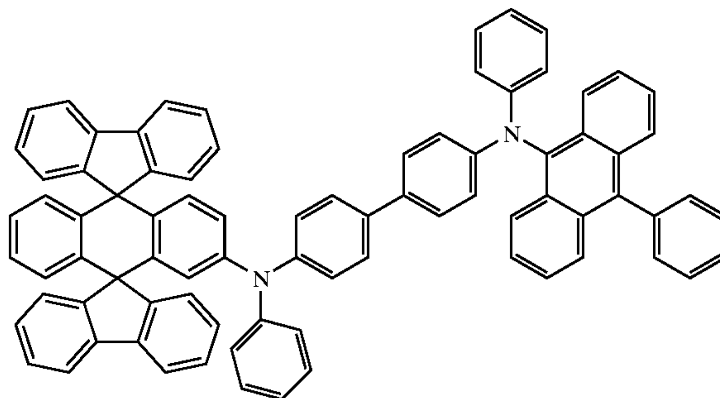
Chemical Compound 408
