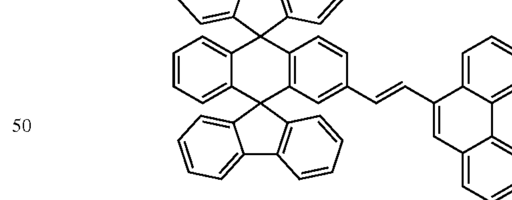
Chemical Compound 104
