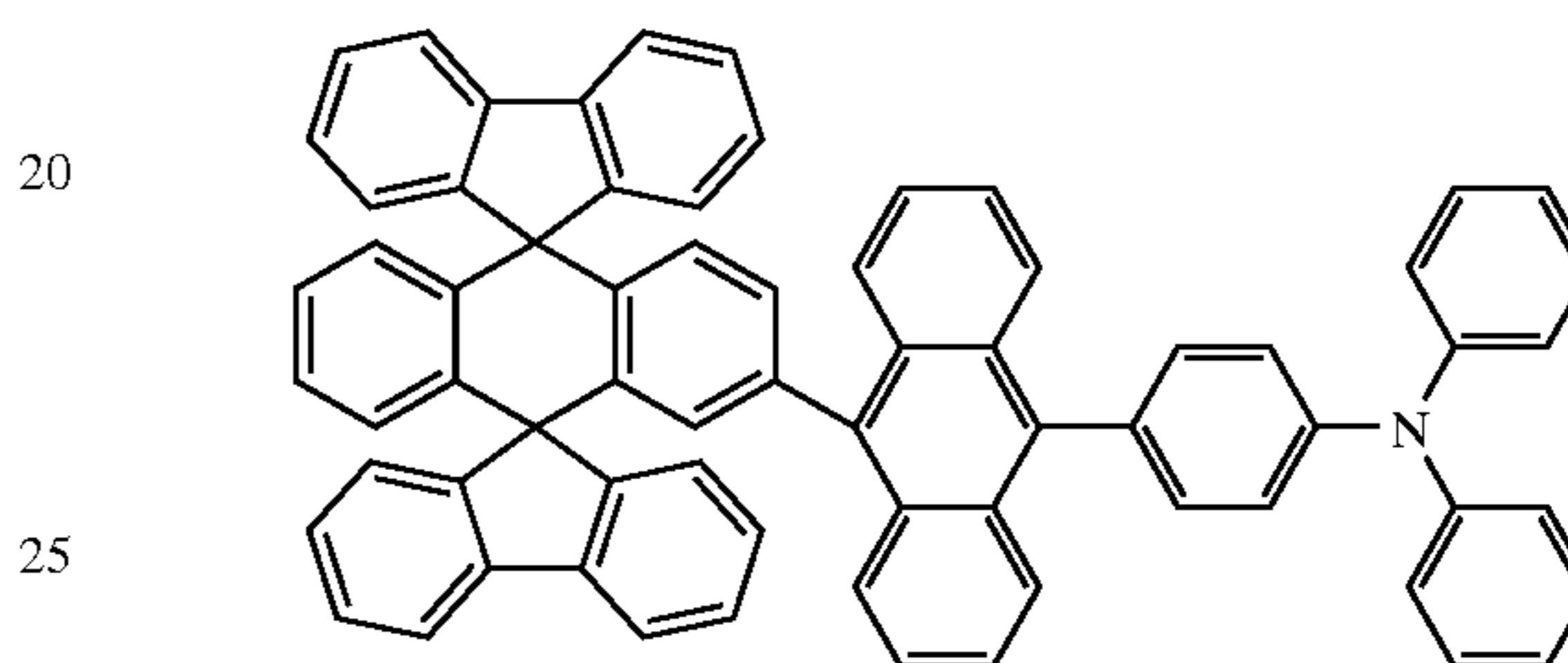
Chemical Compound 401
