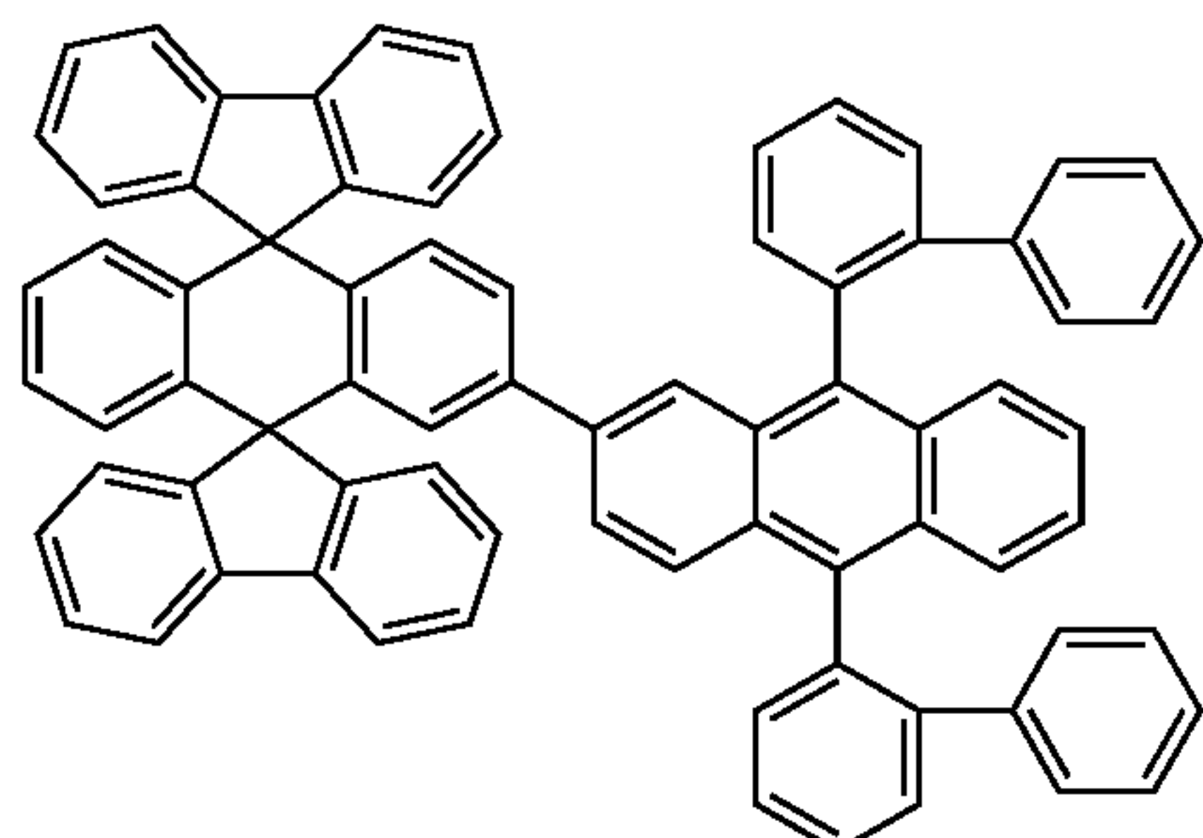
Chemical Compound 118
