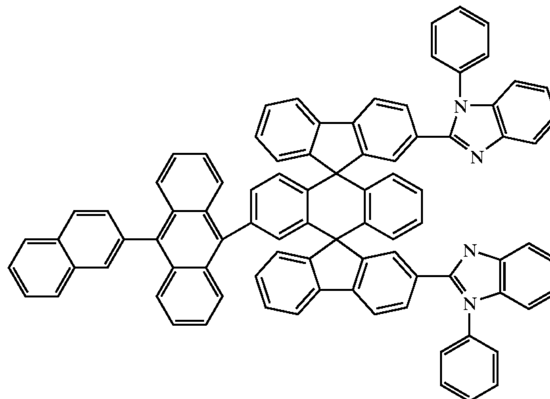
Chemical Compound 222
