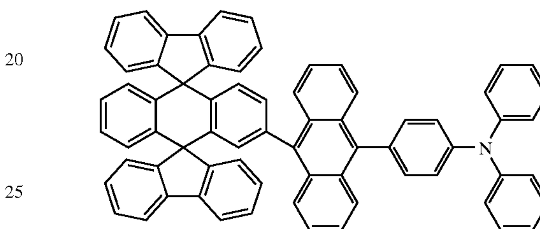
Chemical Compound 401
