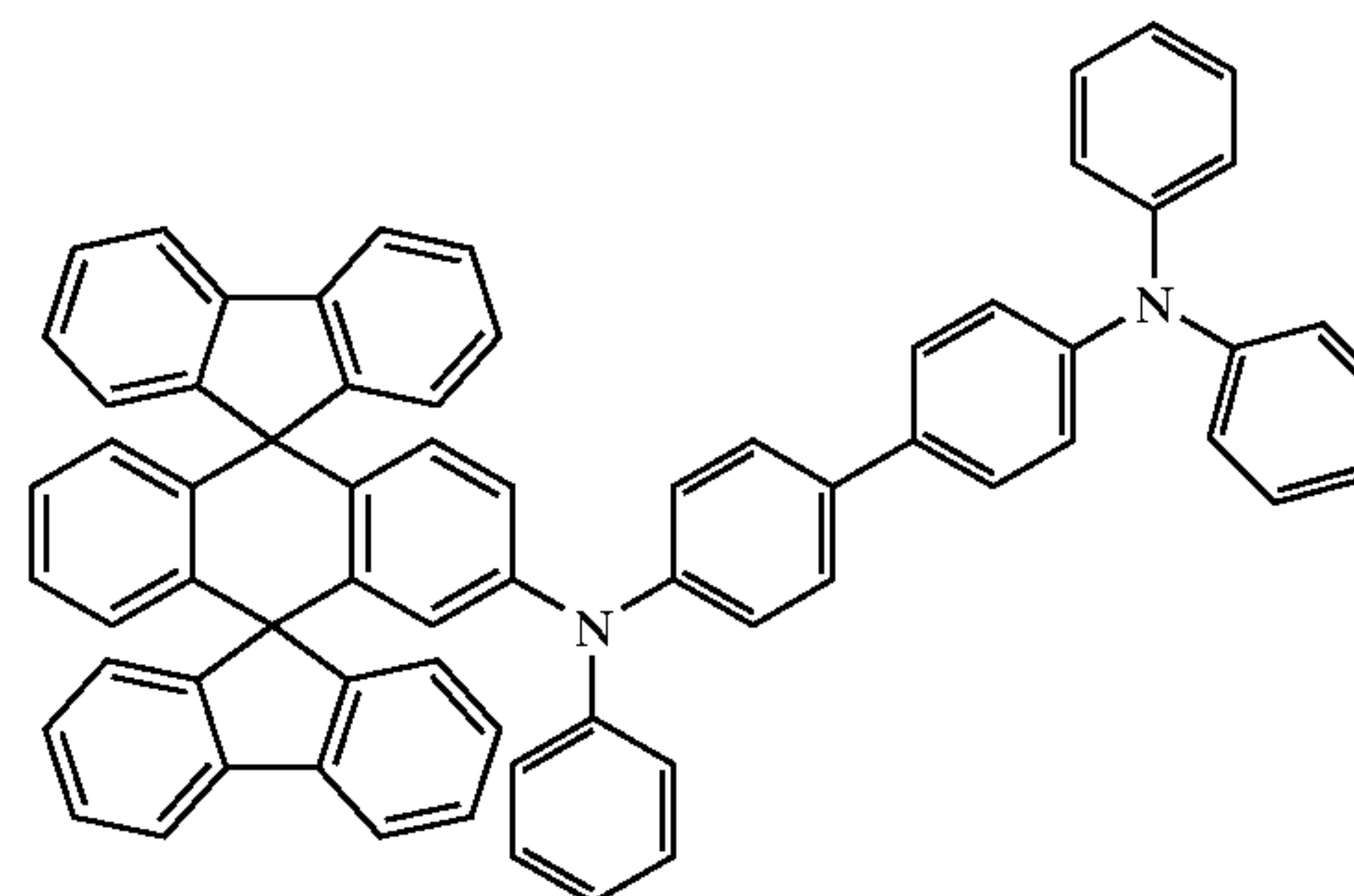
Chemical Compound 307
