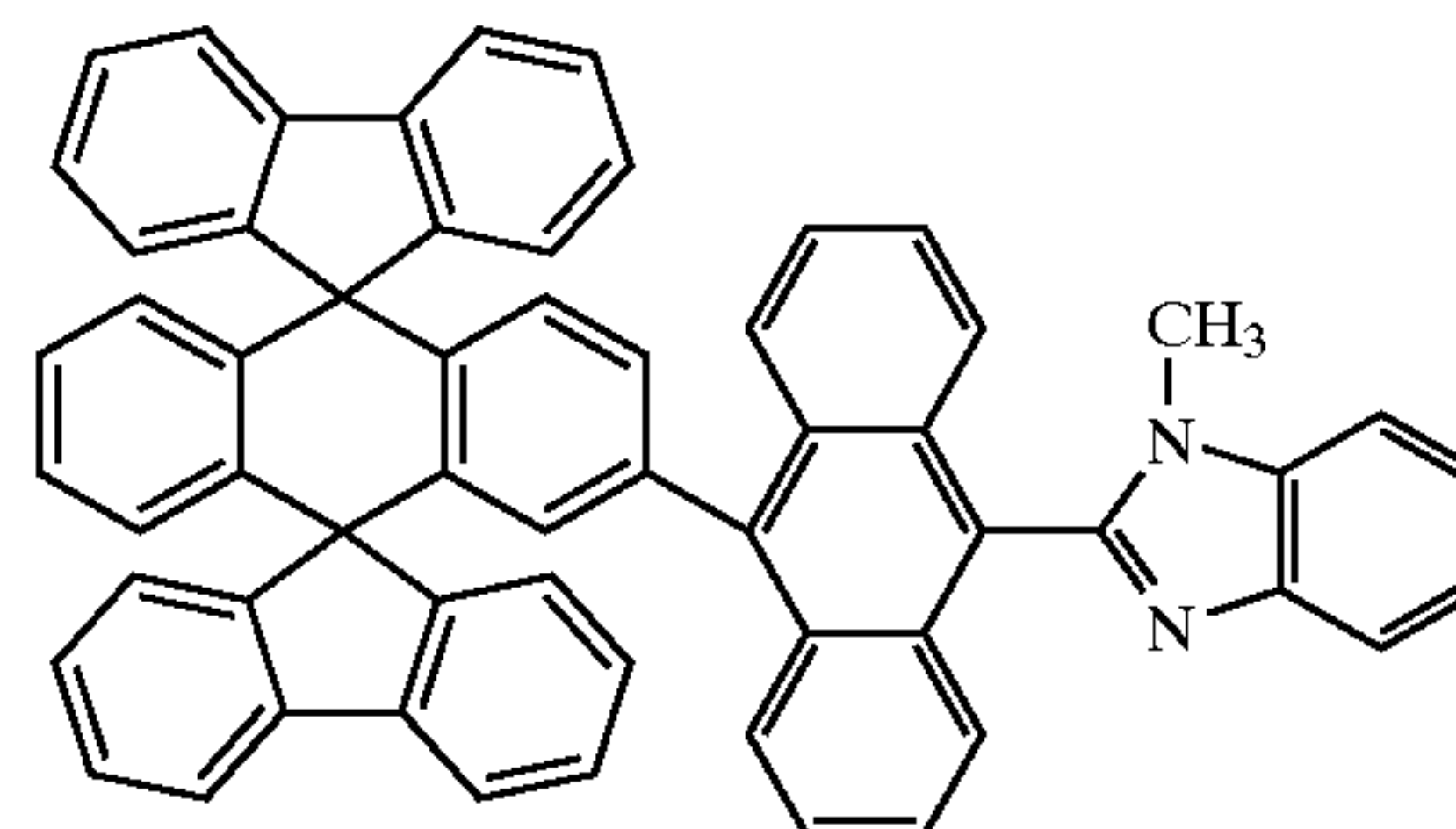
Chemical Compound 205
