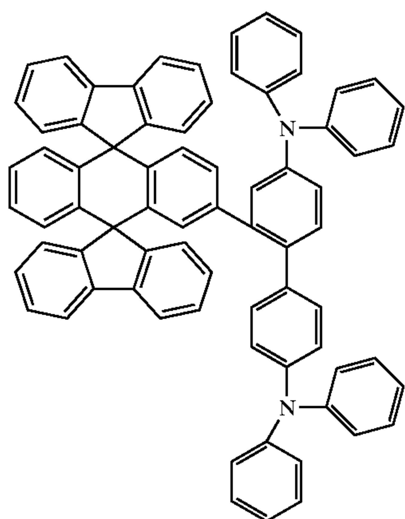
Chemical Compound 305
