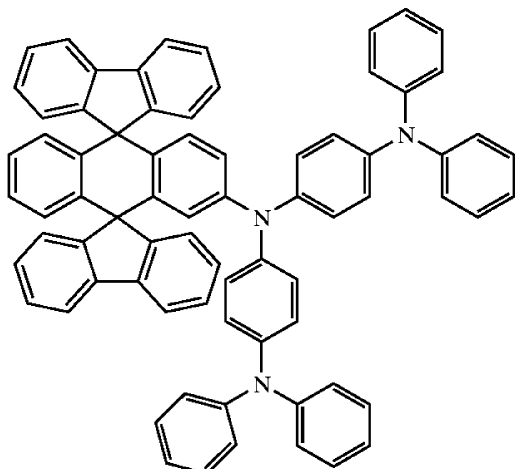
Chemical Compound 308
