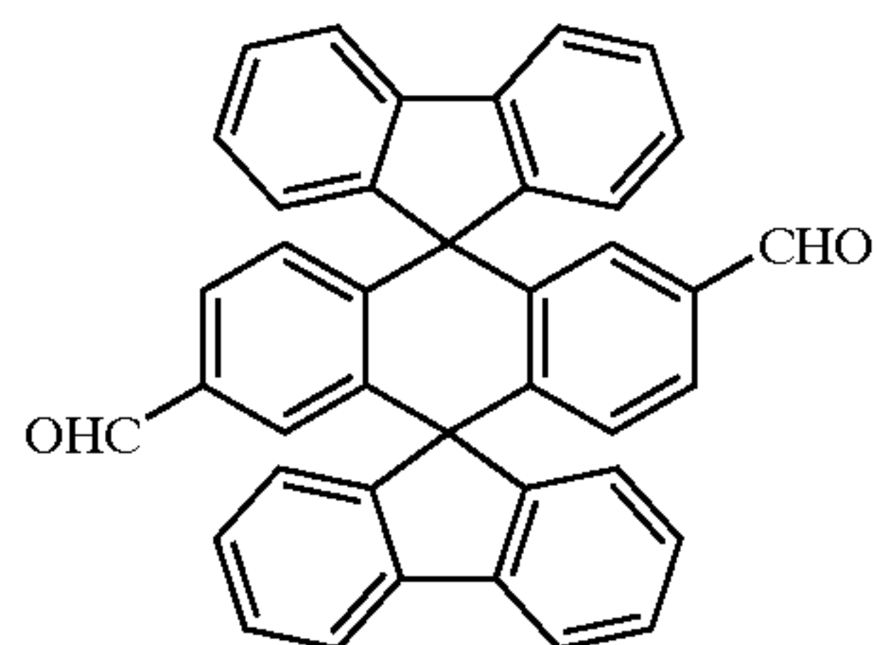
Chemical Compound 4
