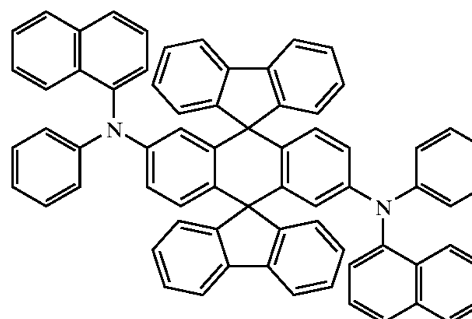
Chemical Compound 302
