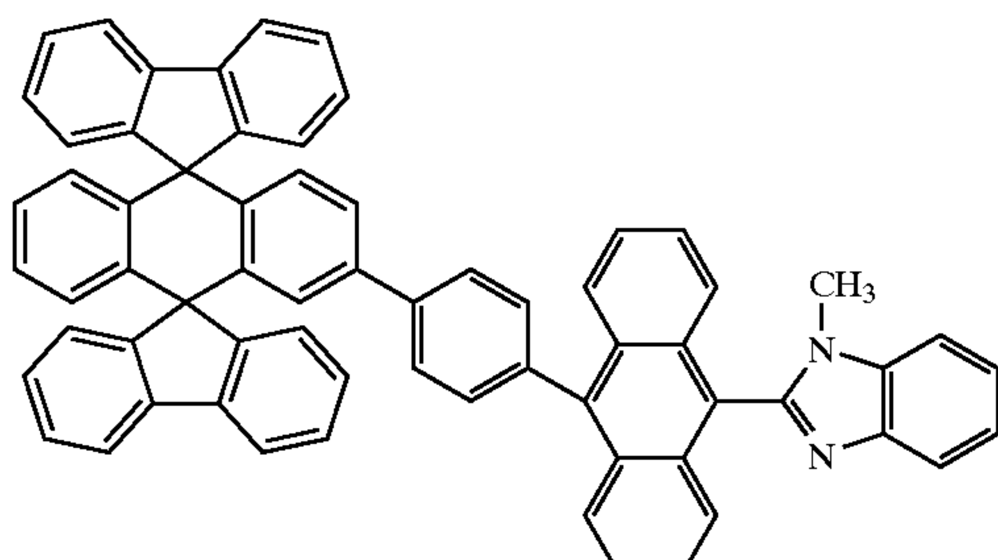
Chemical Compound 201
