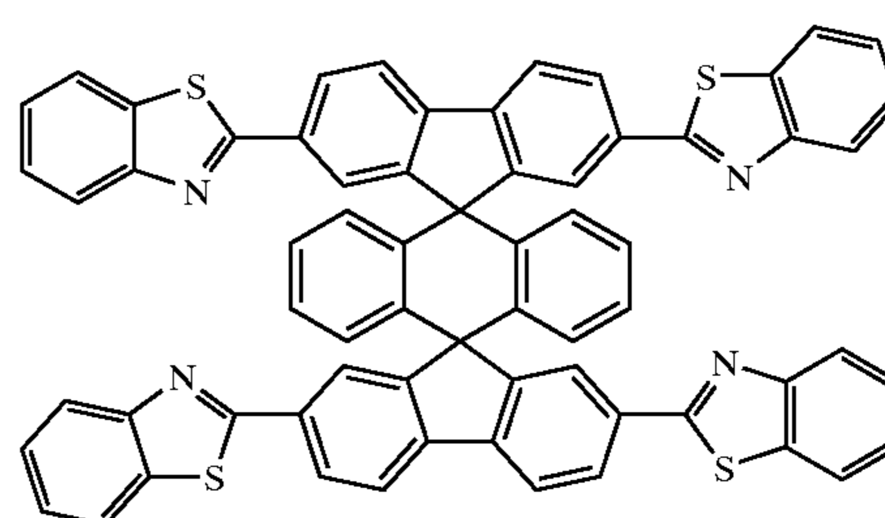
Chemical Compound 218
