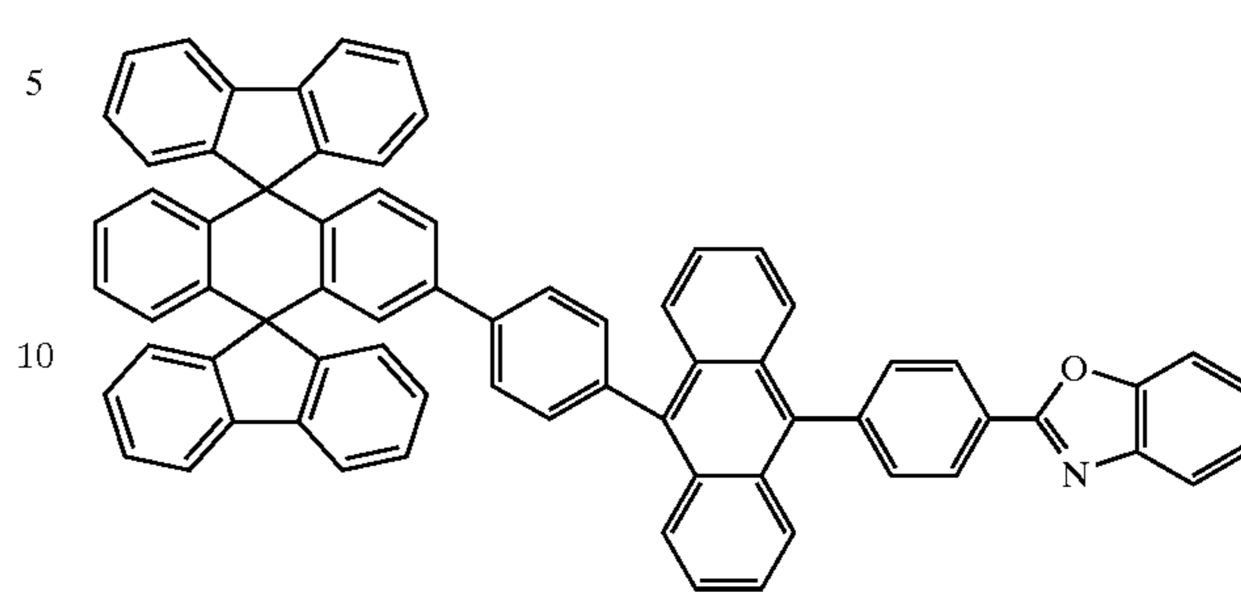
Chemical Compound 126
