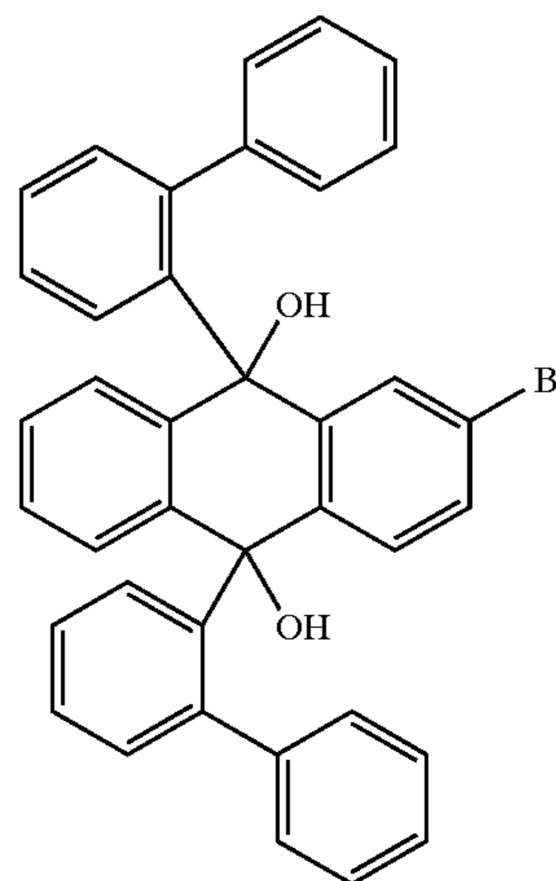
2-bromo-9,10-bis(2-biphenyl-dihydroxy)-anthracene
