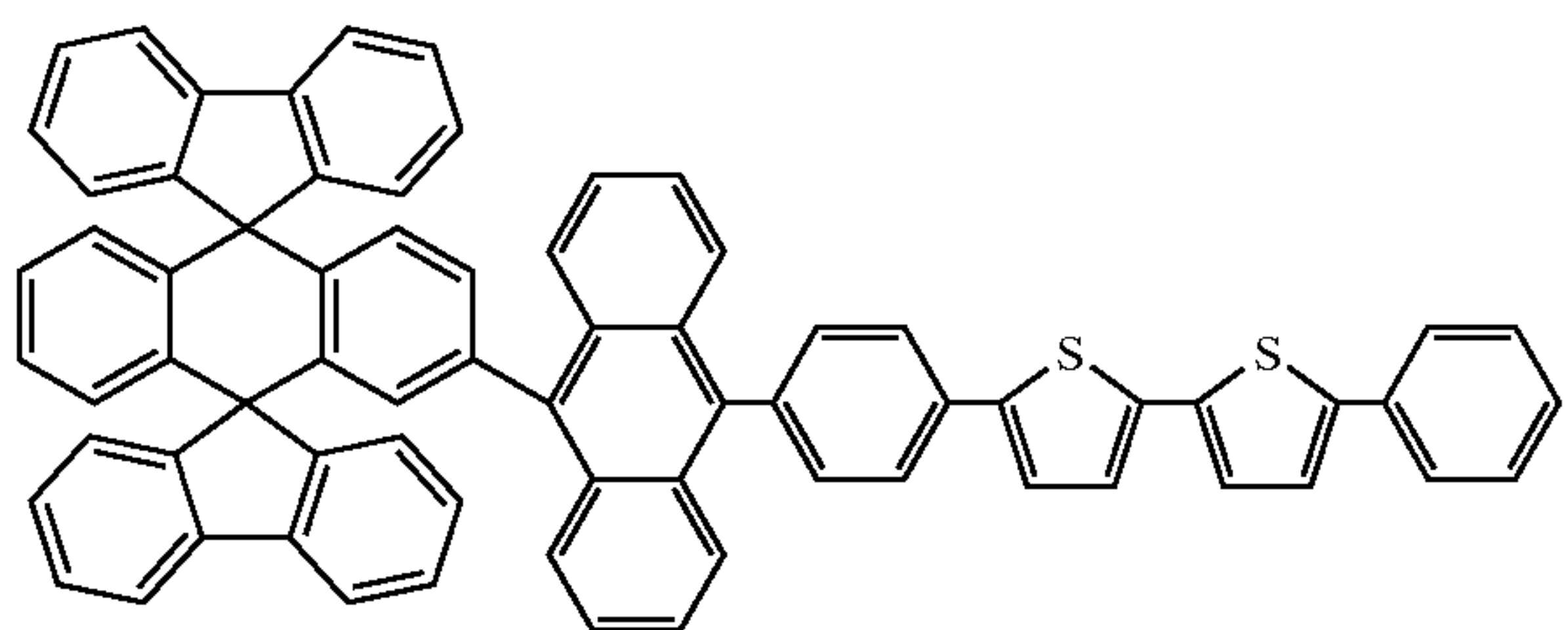
Chemical Compound 131
