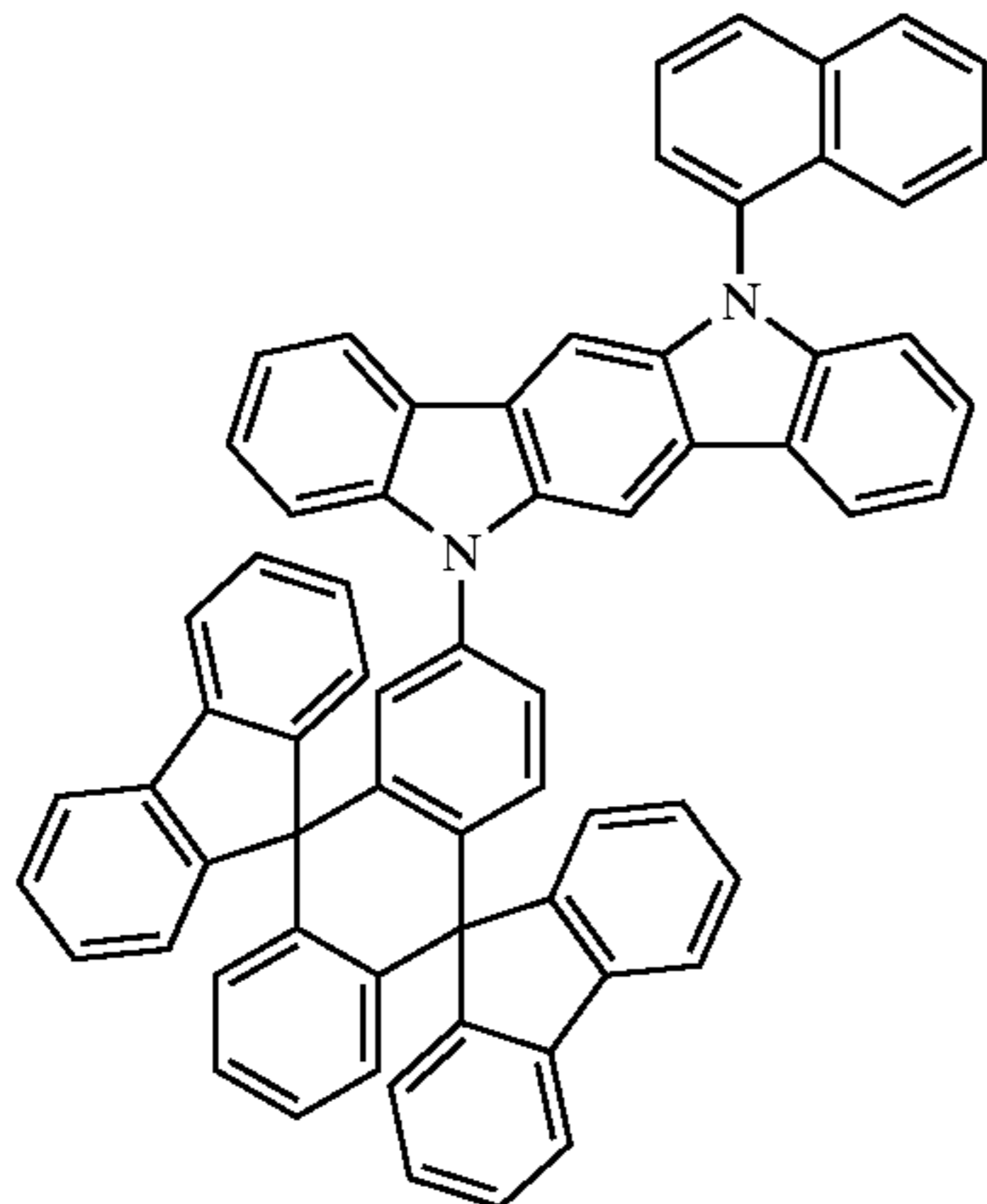
Chemical Compound 411
