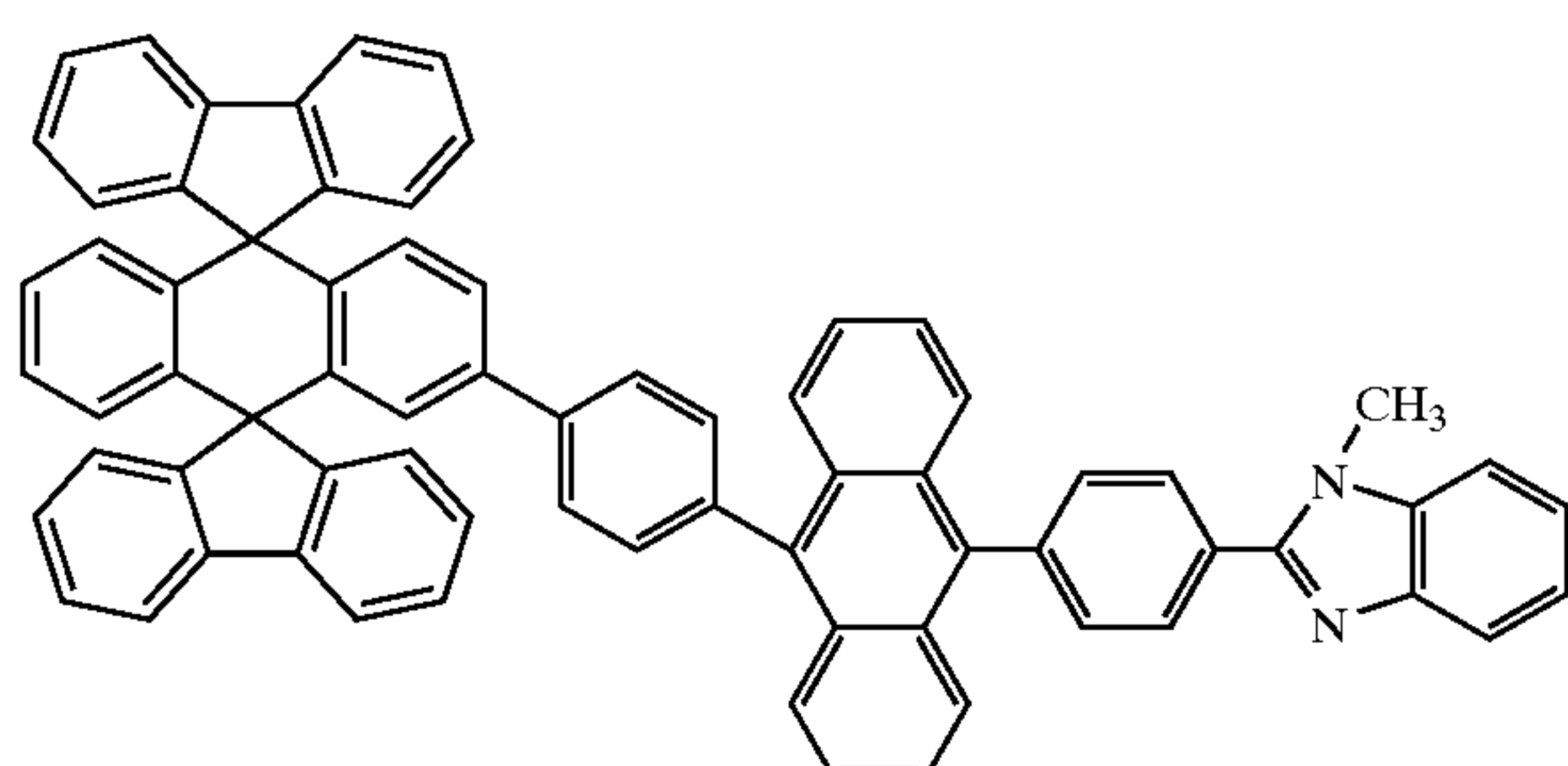
Chemical Compound 211
