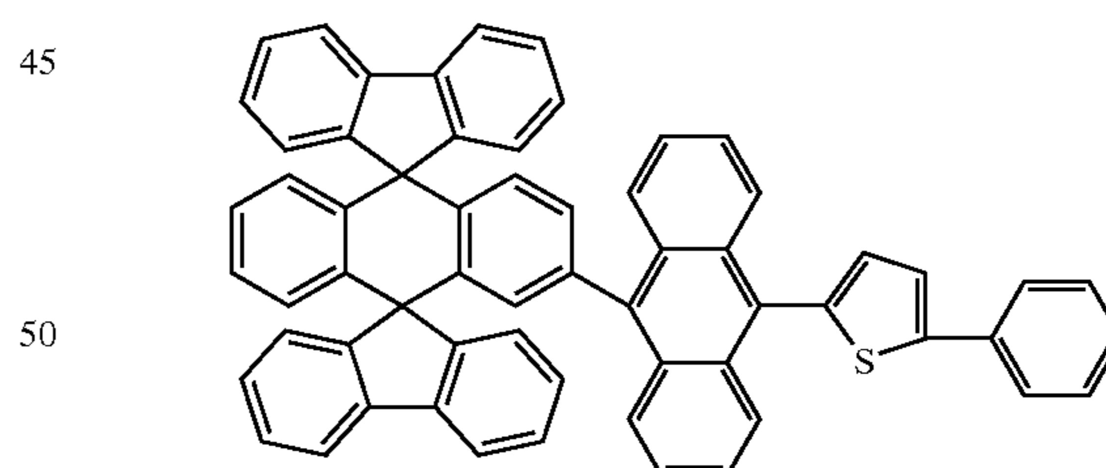
Chemical Compound 134
