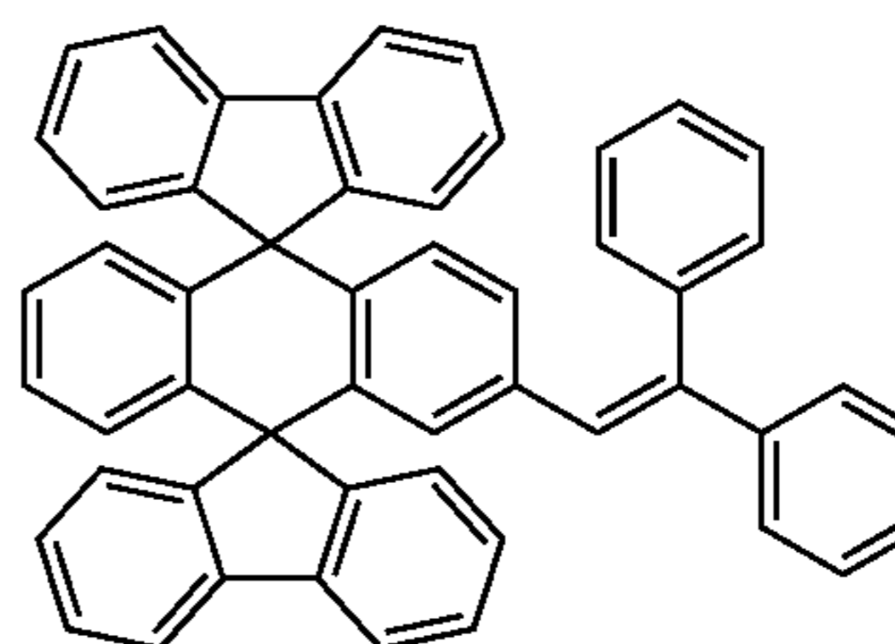
Chemical Compound 106
