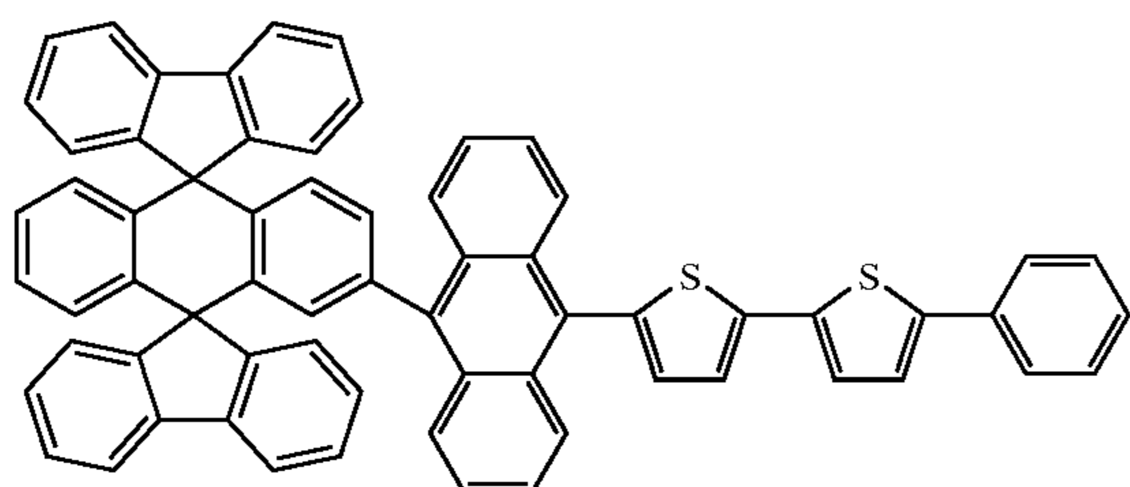
Chemical Compound 133
