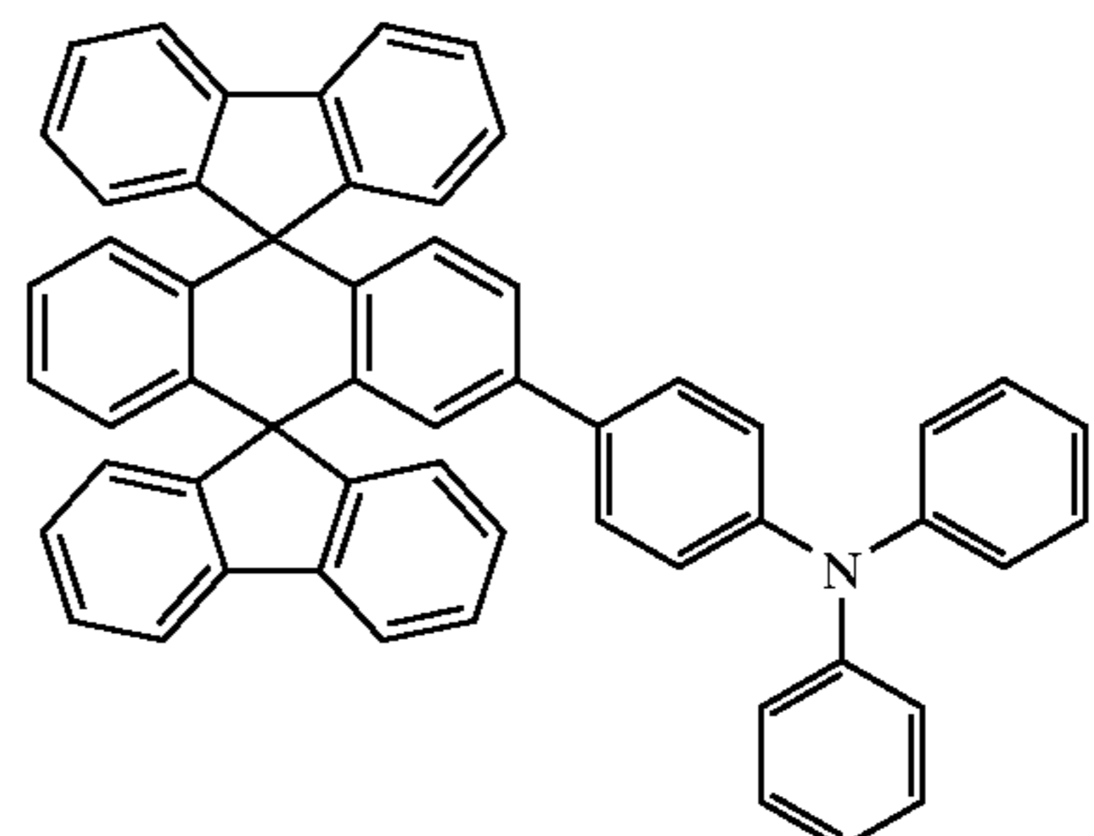
Chemical Compound 303
