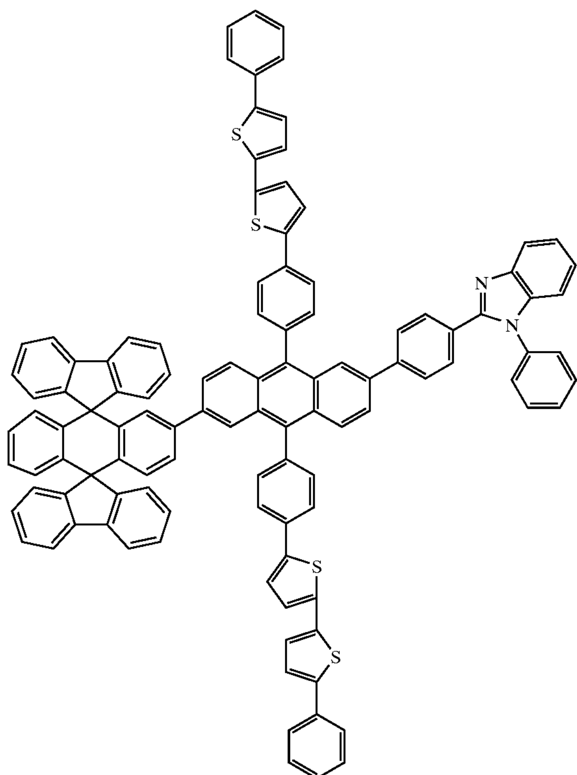
Chemical Compound 130
