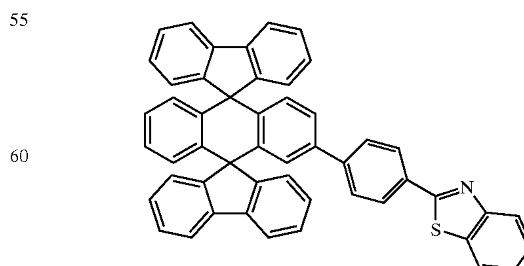
Chemical Compound 213
