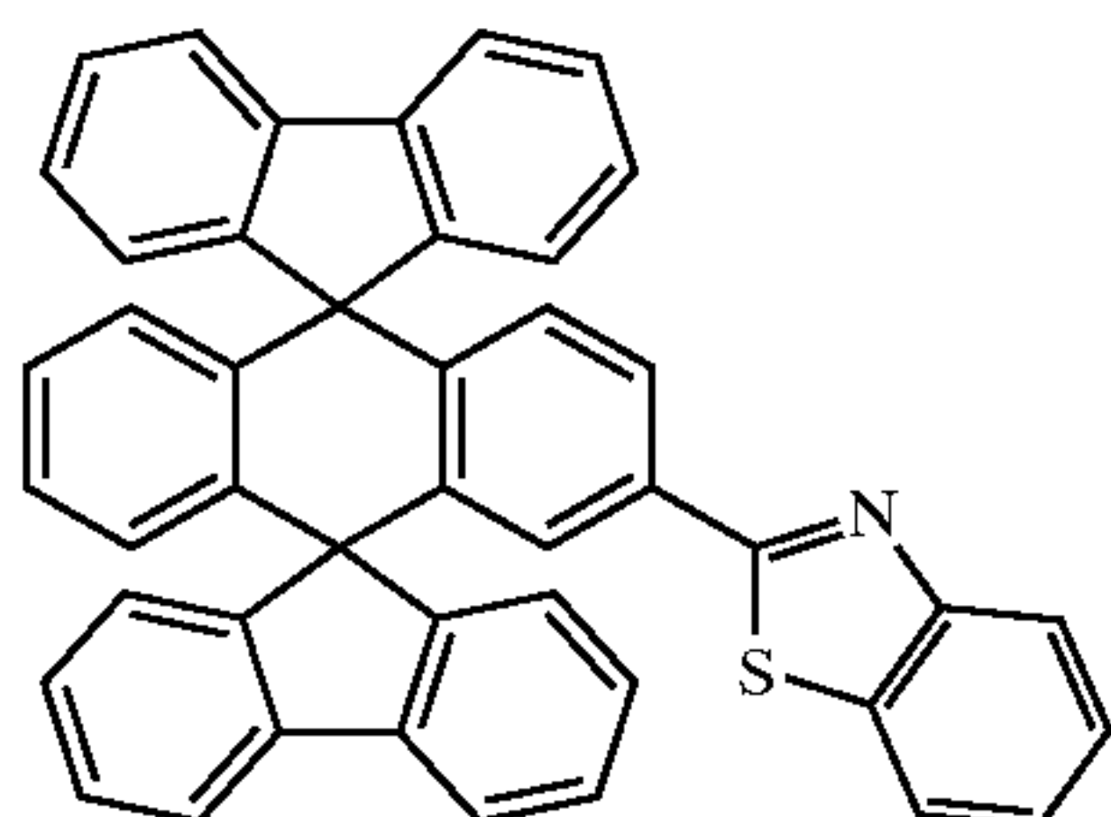
Chemical Compound 215
