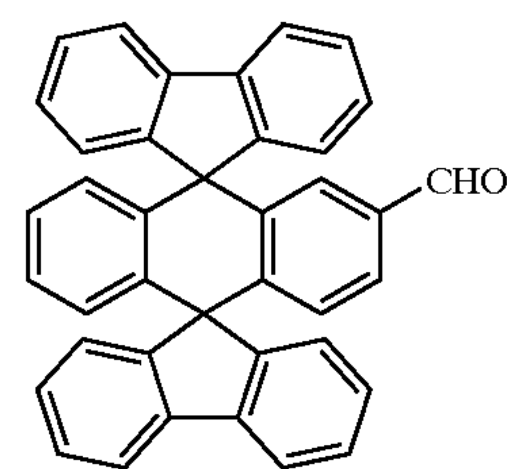
Chemical Compound 3
