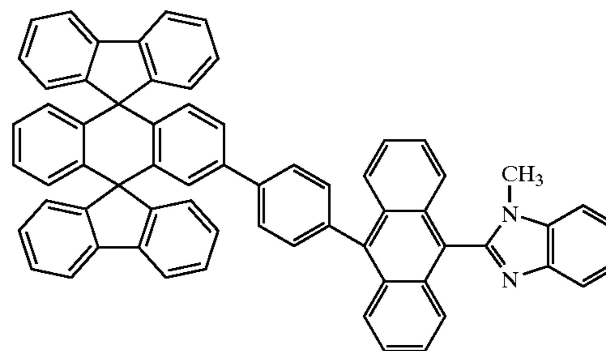
Chemical Compound 201
