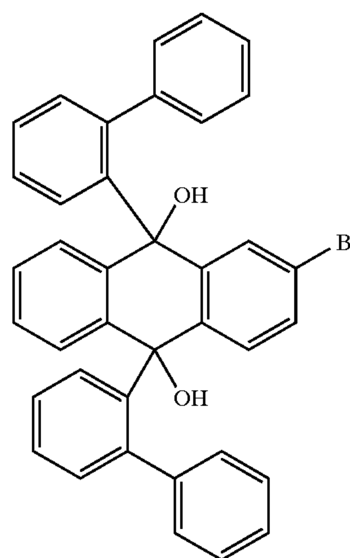
2-bromo-9,10-bis(2-biphenyl-dihydroxy)-anthracene
