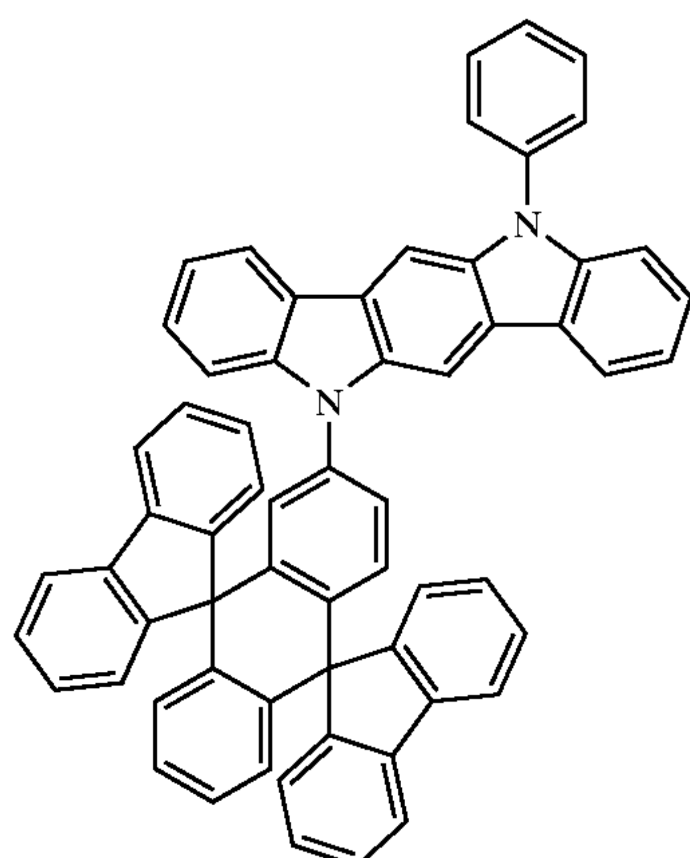
Chemical Compound 410
