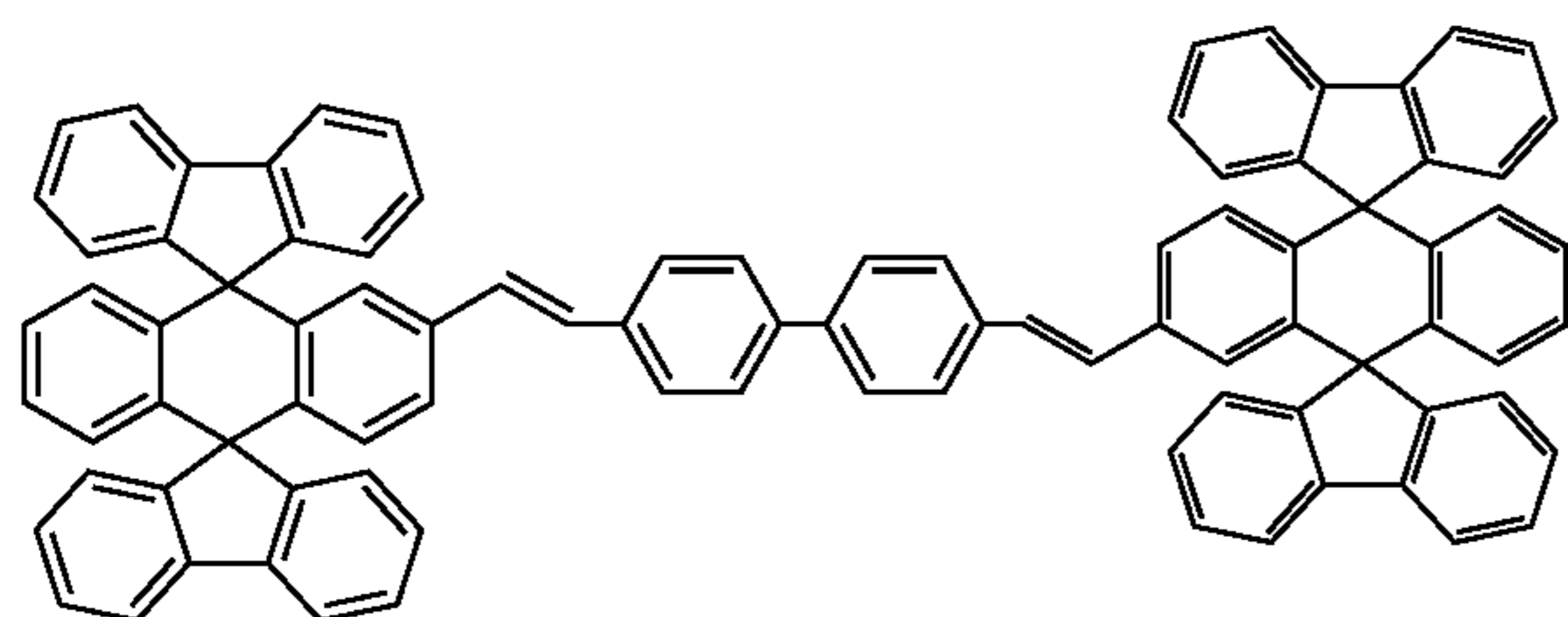
Chemical Compound 100
