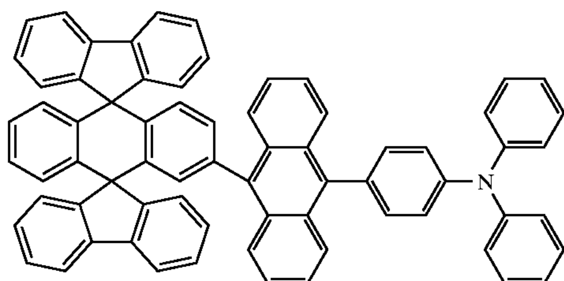
Chemical Compound 401
