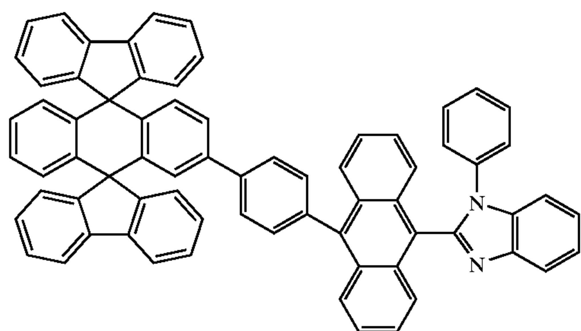
Chemical Compound 207
