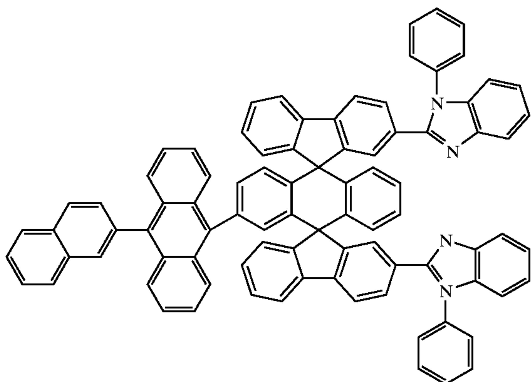
Chemical Compound 222
