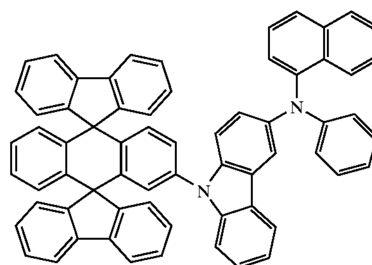
Chemical Compound 306
