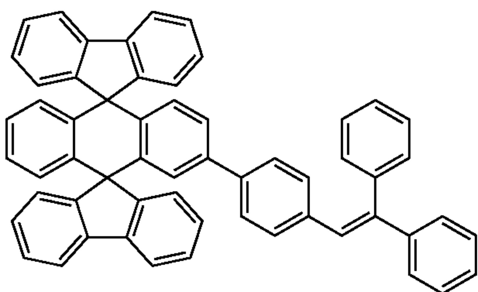
Chemical Compound 107
