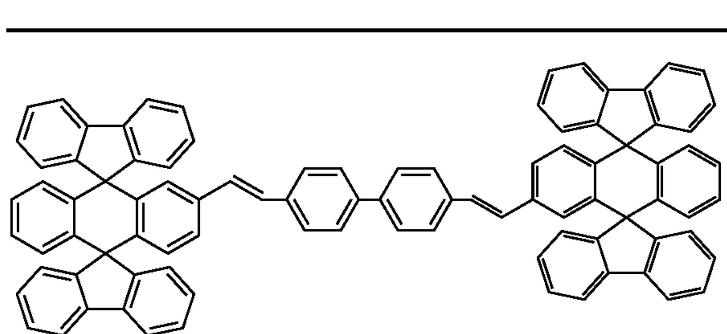
Chemical Compound 100
