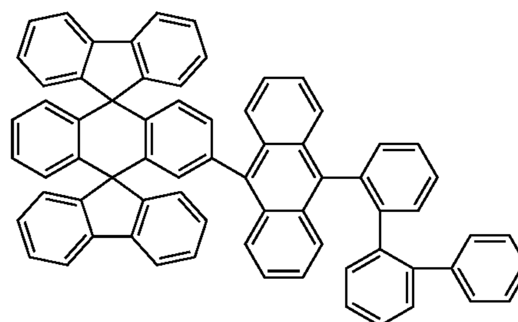
Chemical Compound 112
