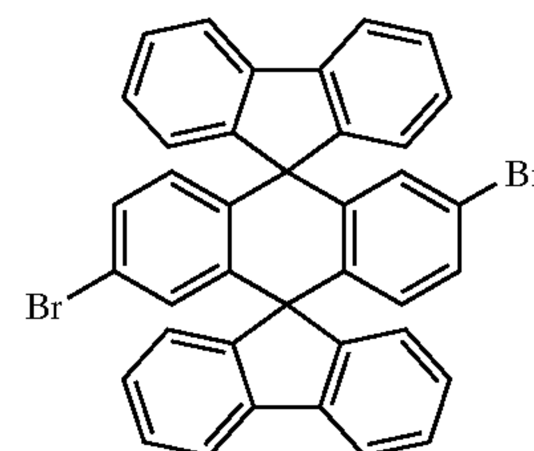
Chemical Compound 2
