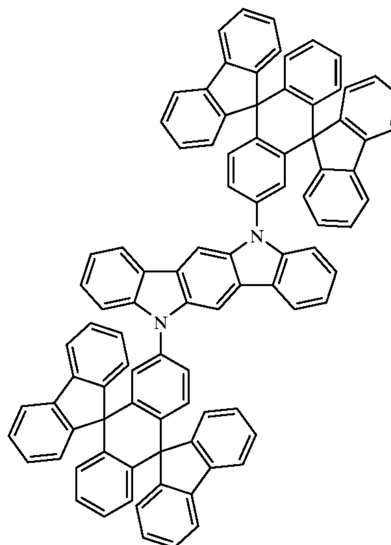
Chemical Compound 405
