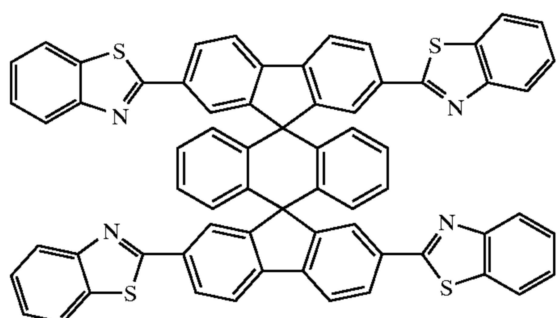
Chemical Compound 218
