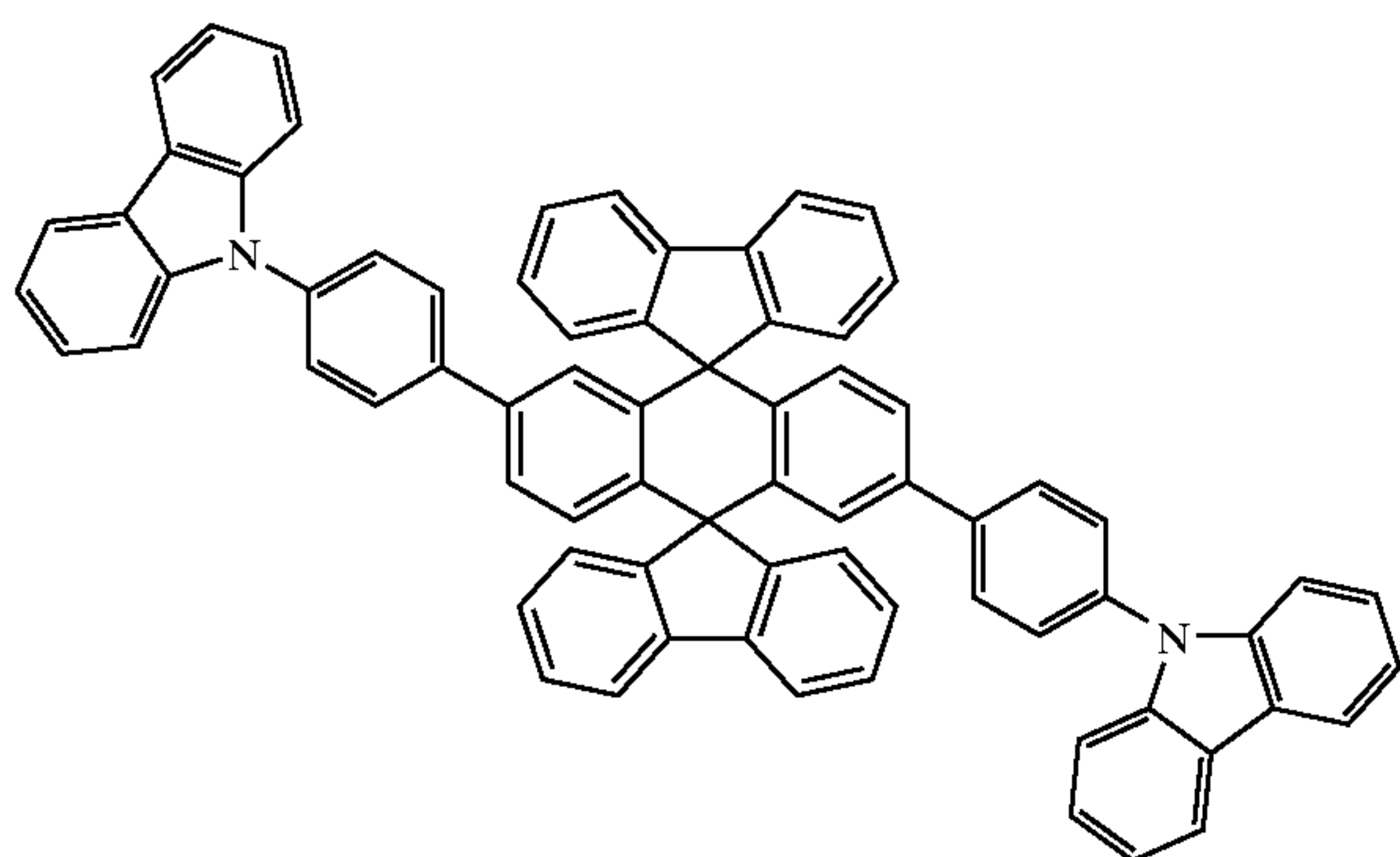
Chemical Compound 402
