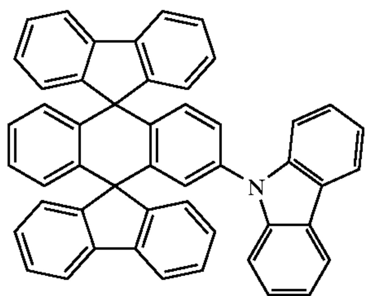
Chemical Compound 404
