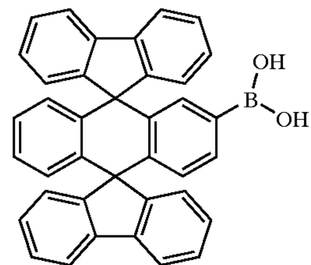
Chemical Compound 8
