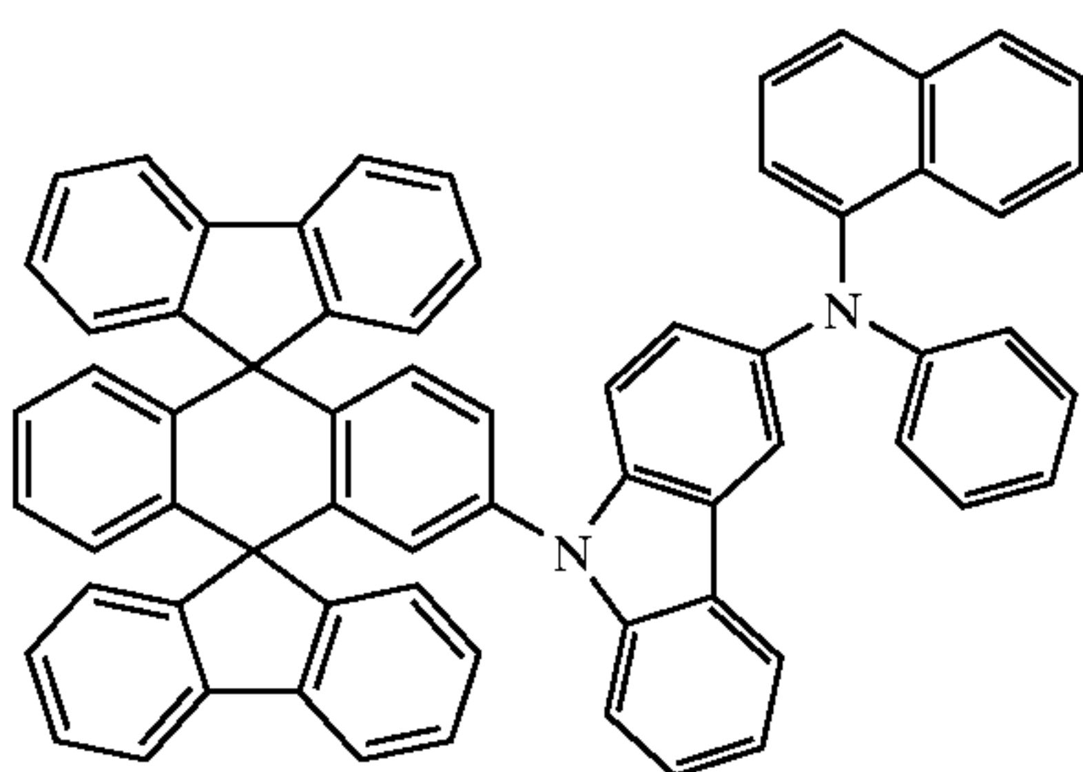
Chemical Compound 306
