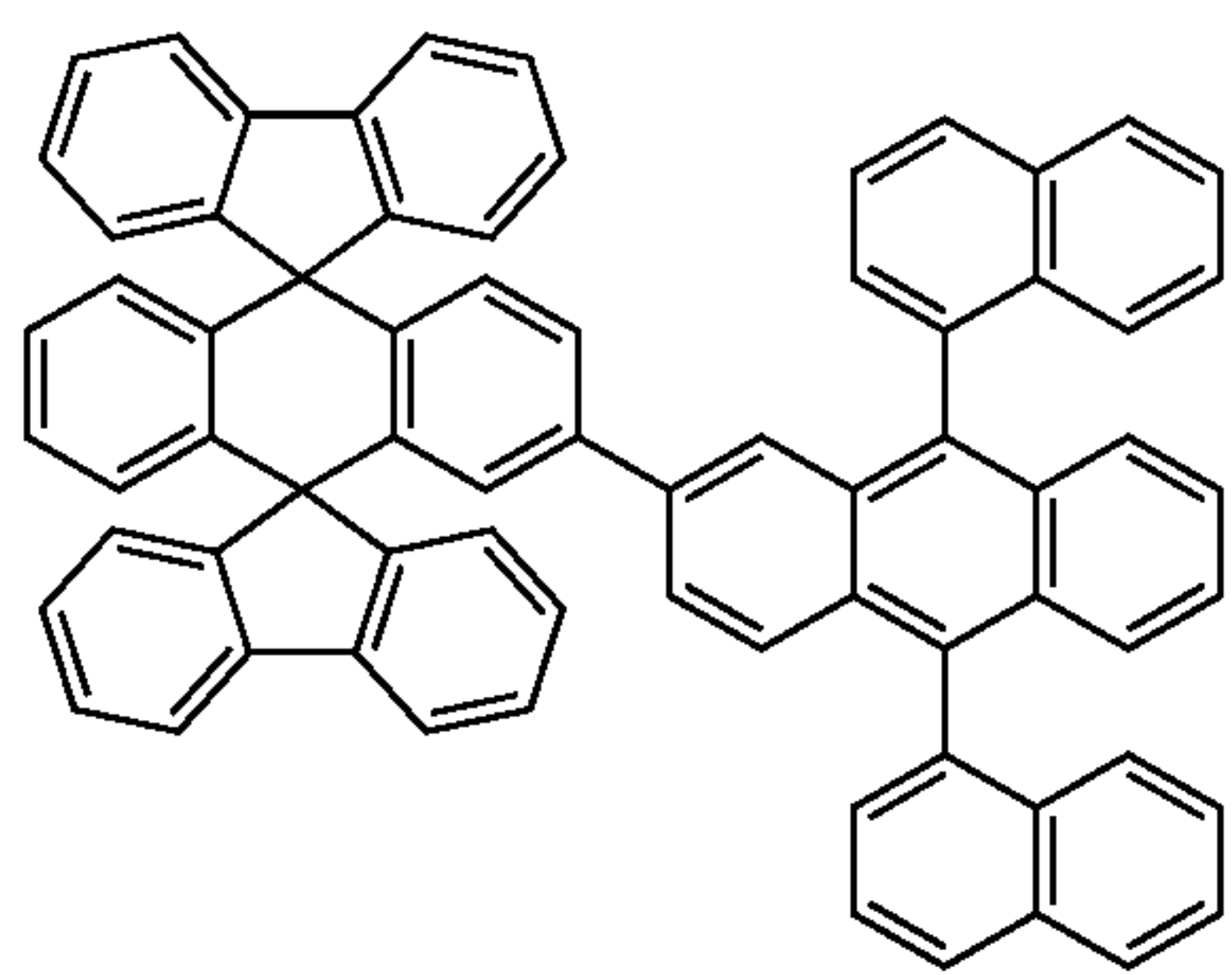
Chemical Compound 120
