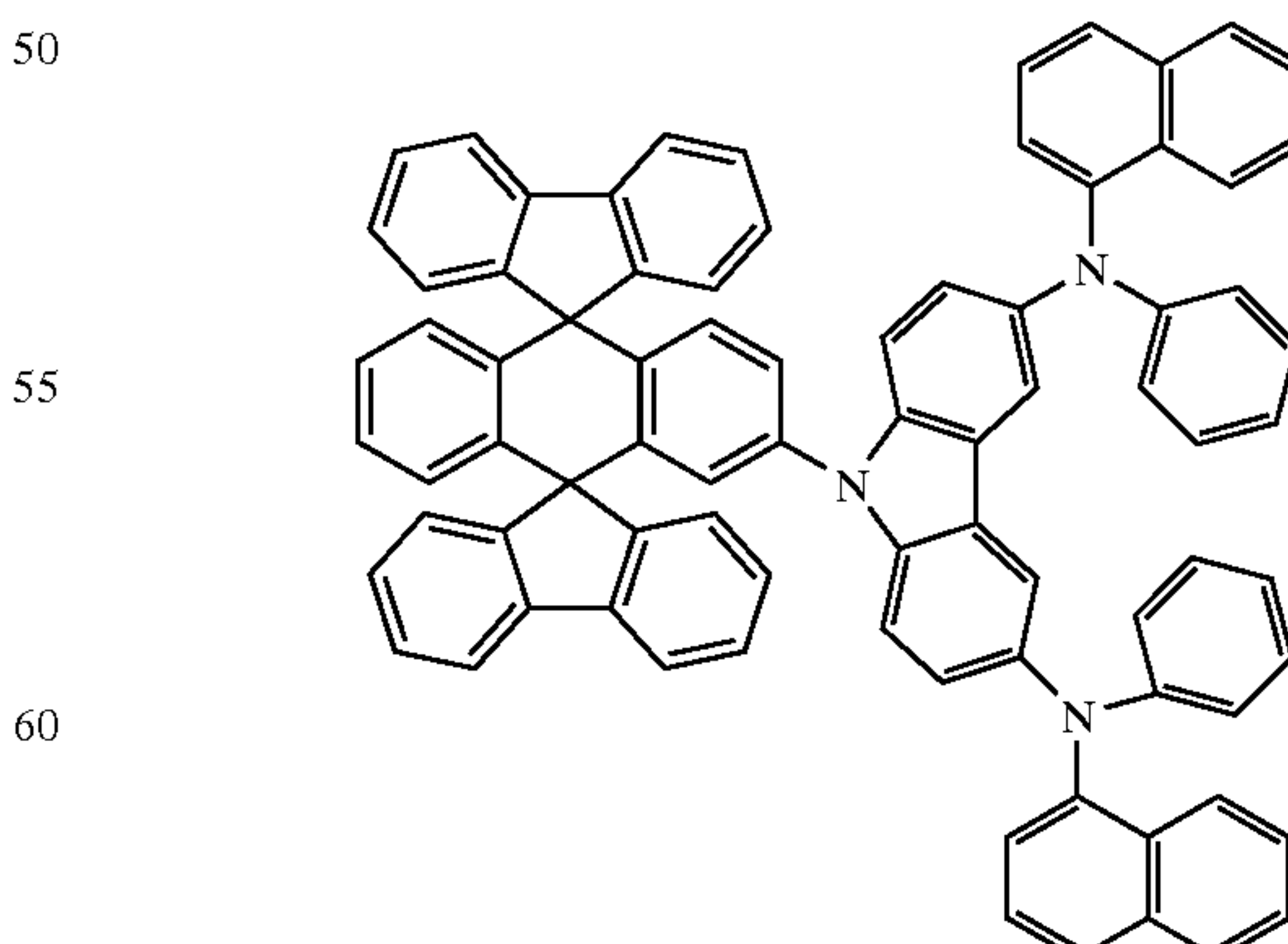
Chemical Compound 403
