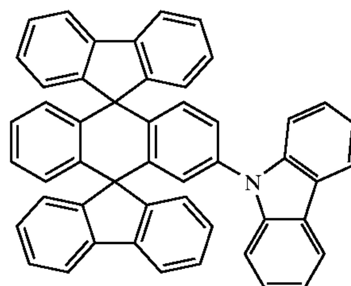
Chemical Compound 404
