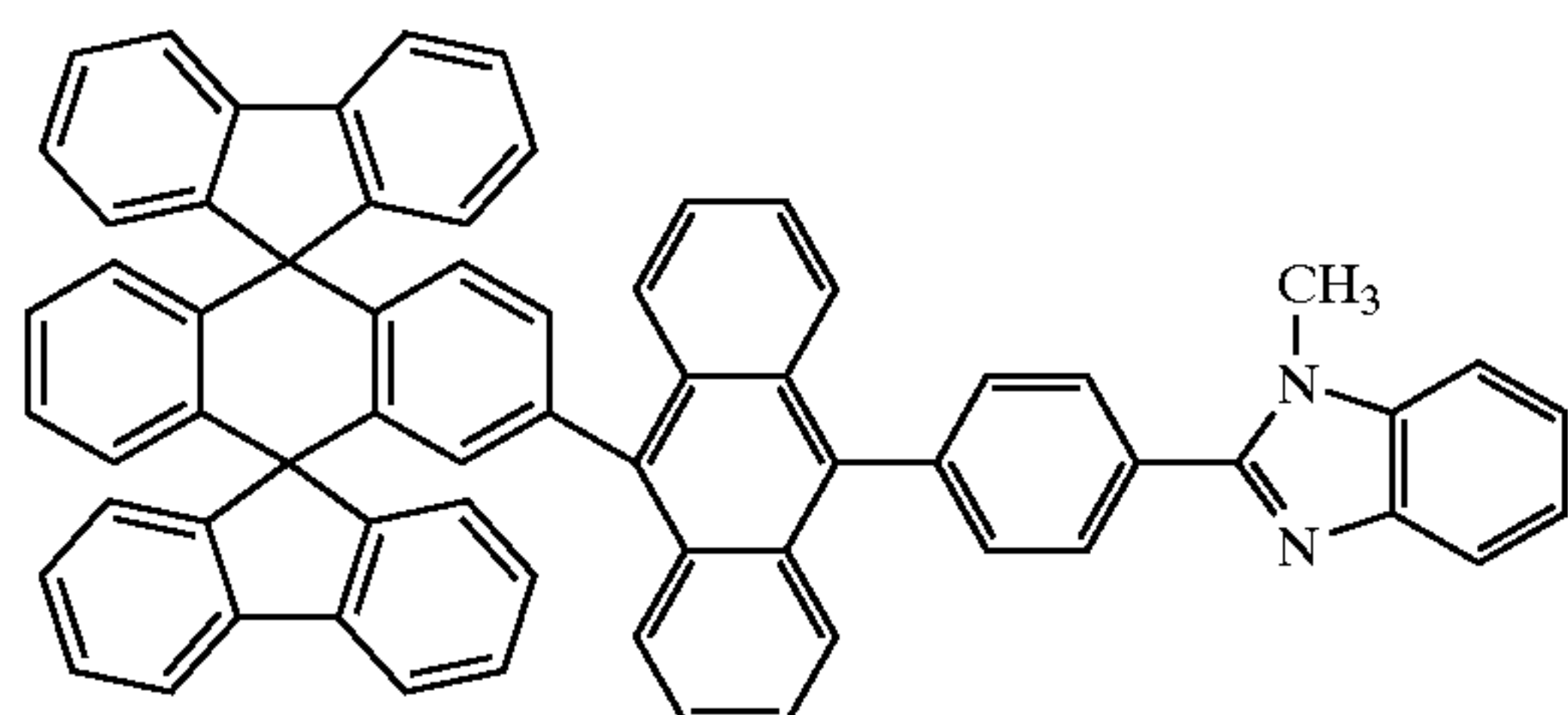
Chemical Compound 208
