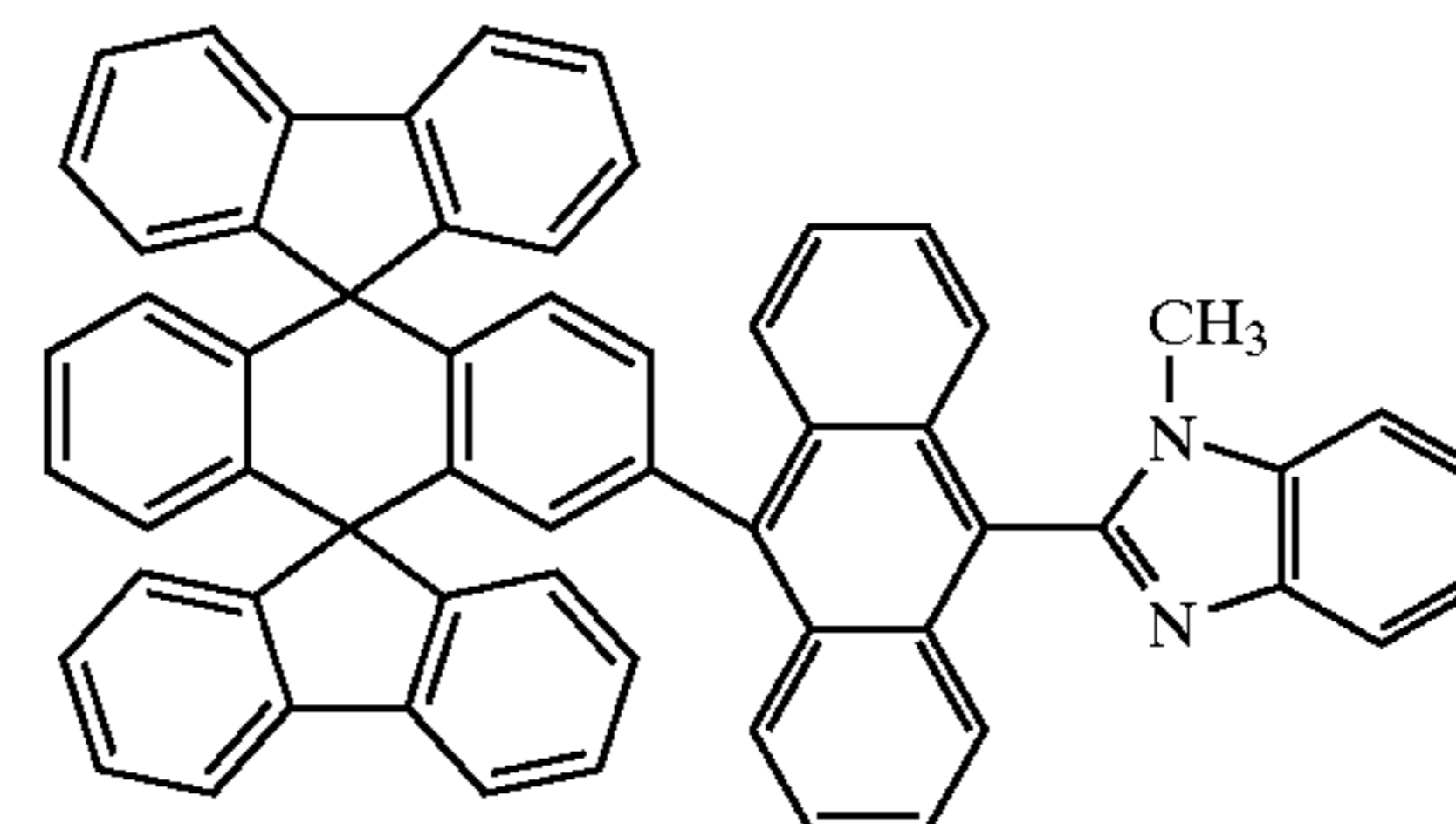
Chemical Compound 205
