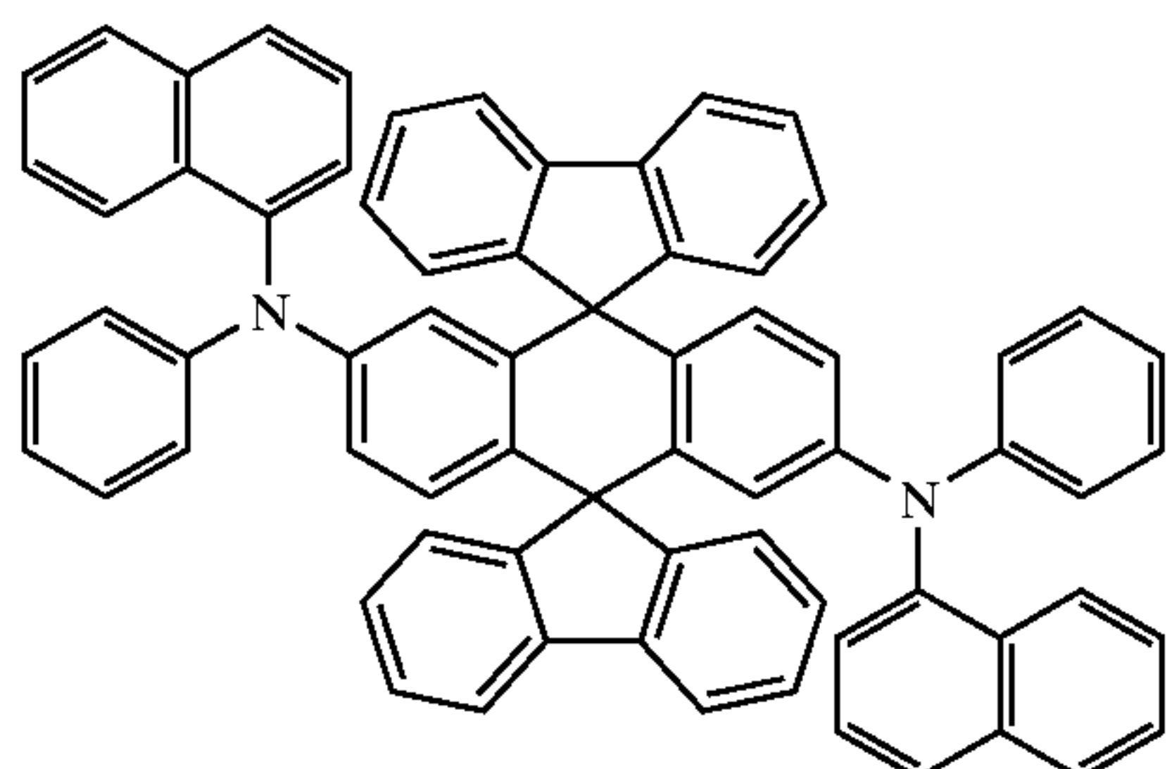
Chemical Compound 302
