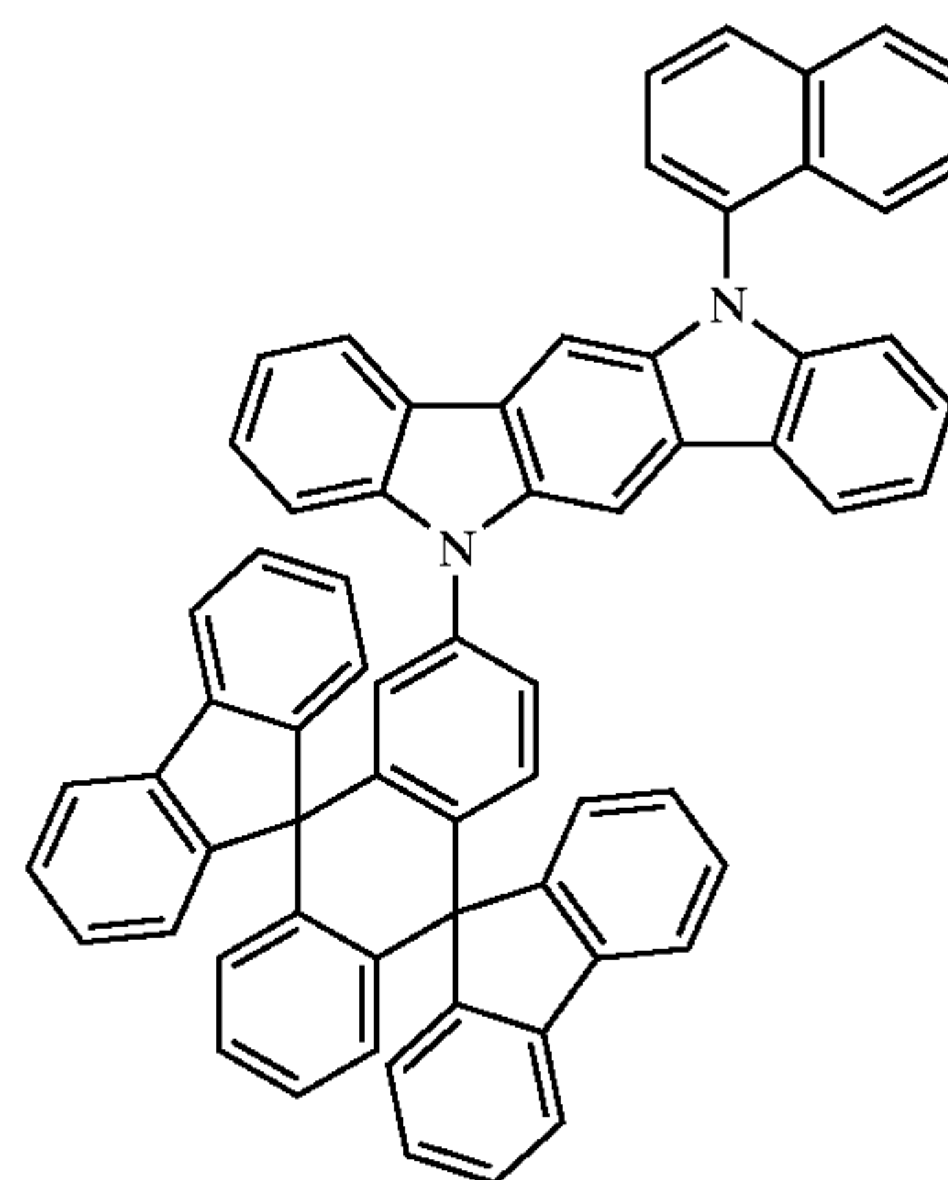
Chemical Compound 411
