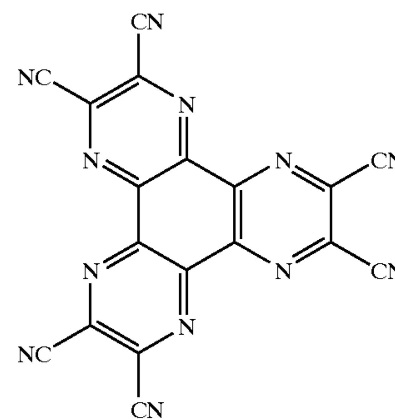
Hexanitrite hexaazatriphenylene
