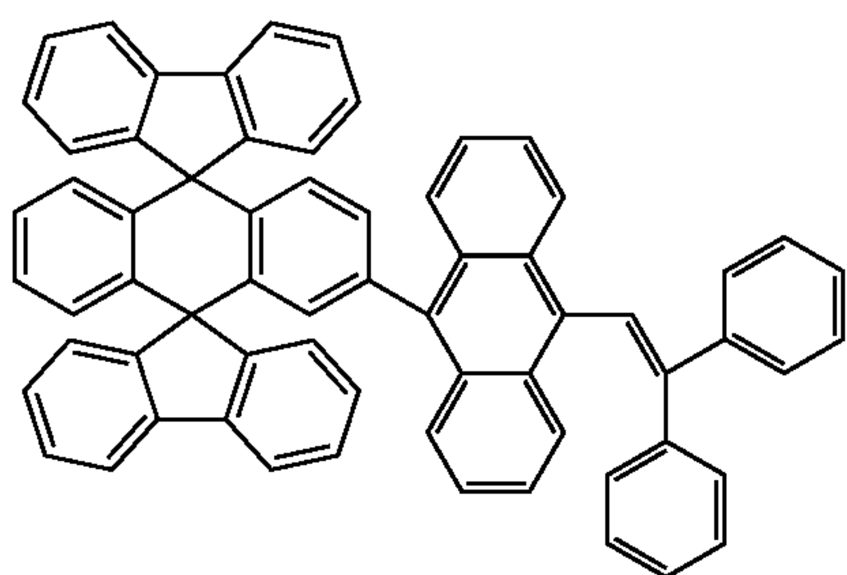
Chemical Compound 137
