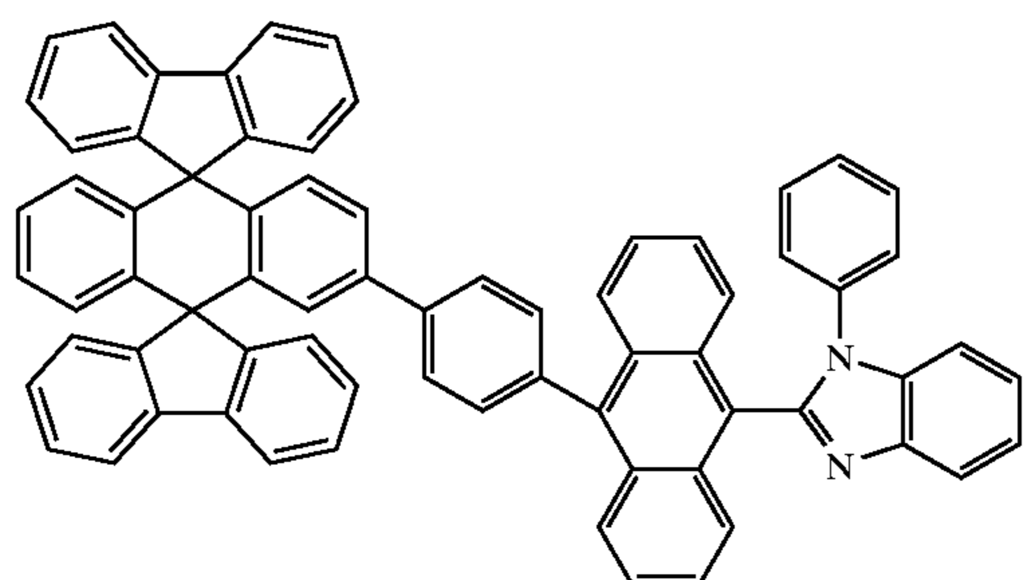
Chemical Compound 207
