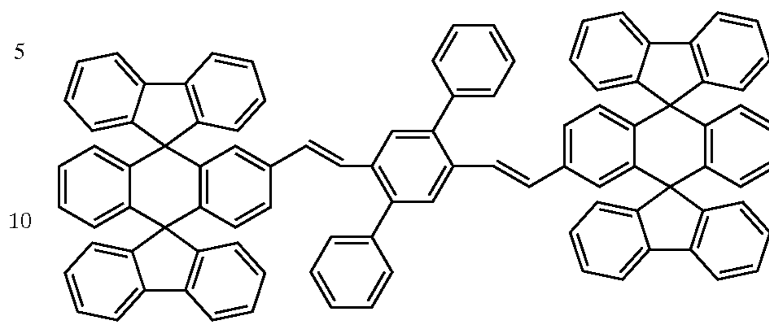
Chemical Compound 101
