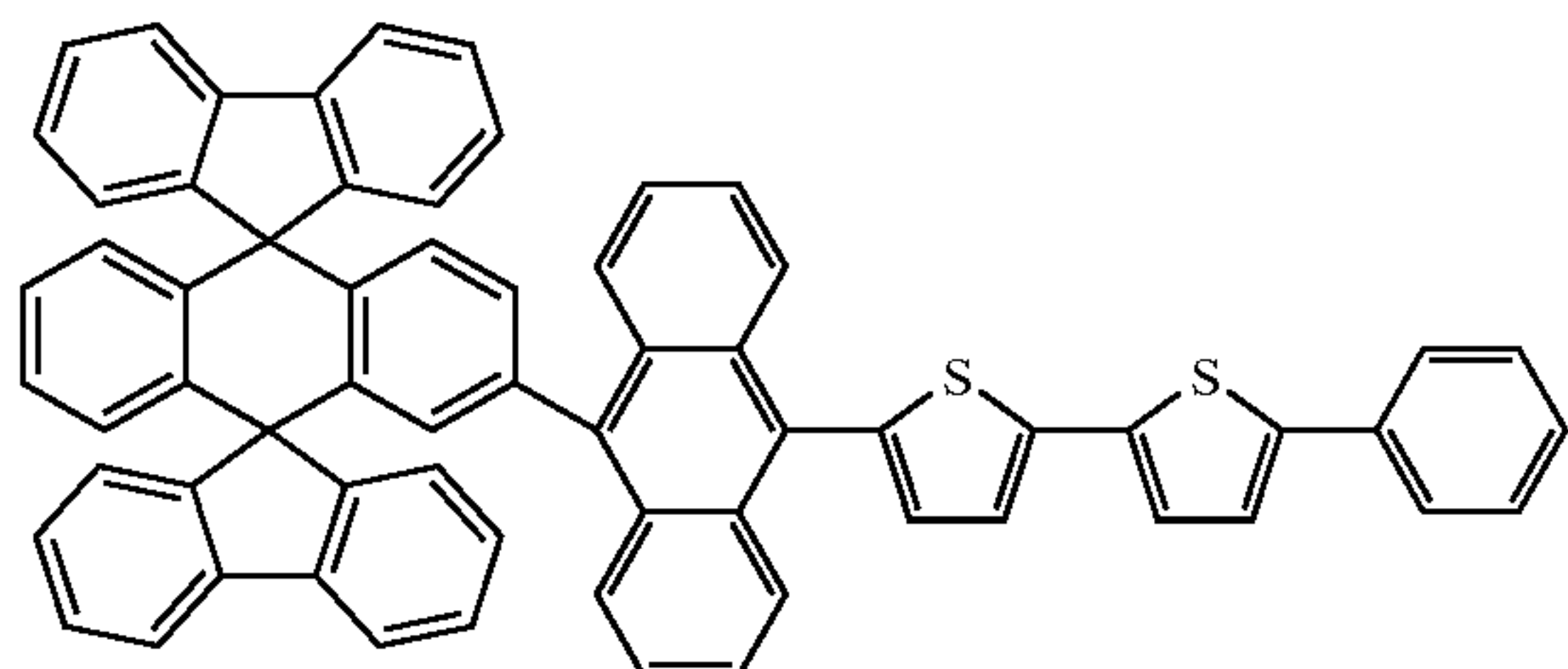
Chemical Compound 133
