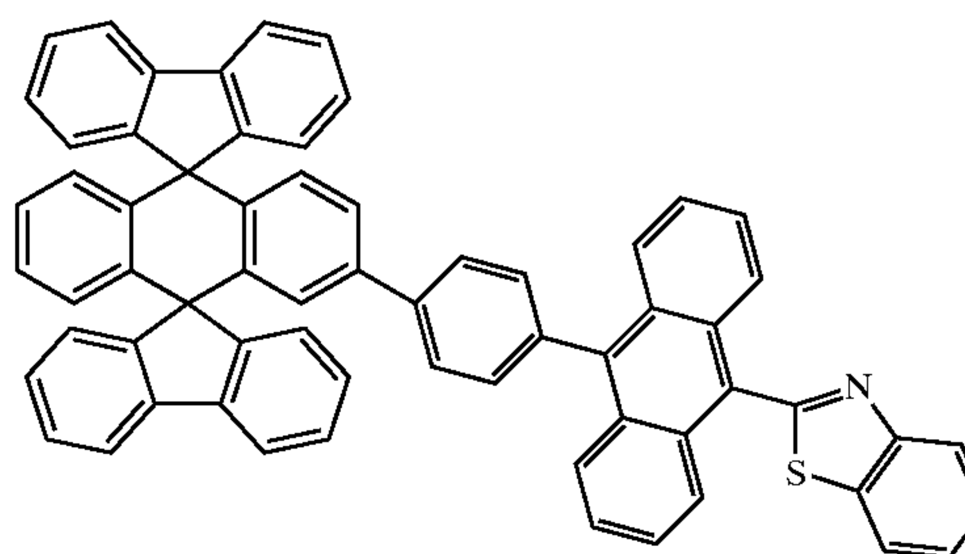
Chemical Compound 216
