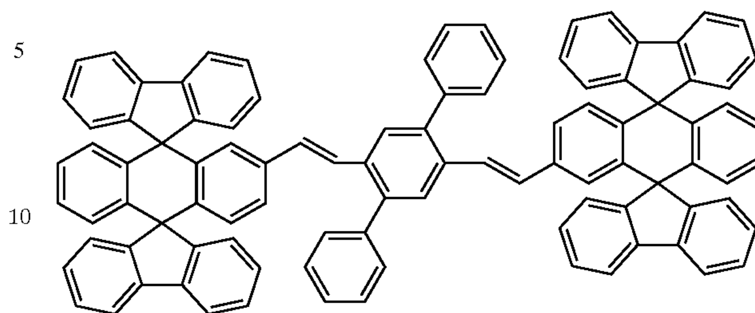
Chemical Compound 101
