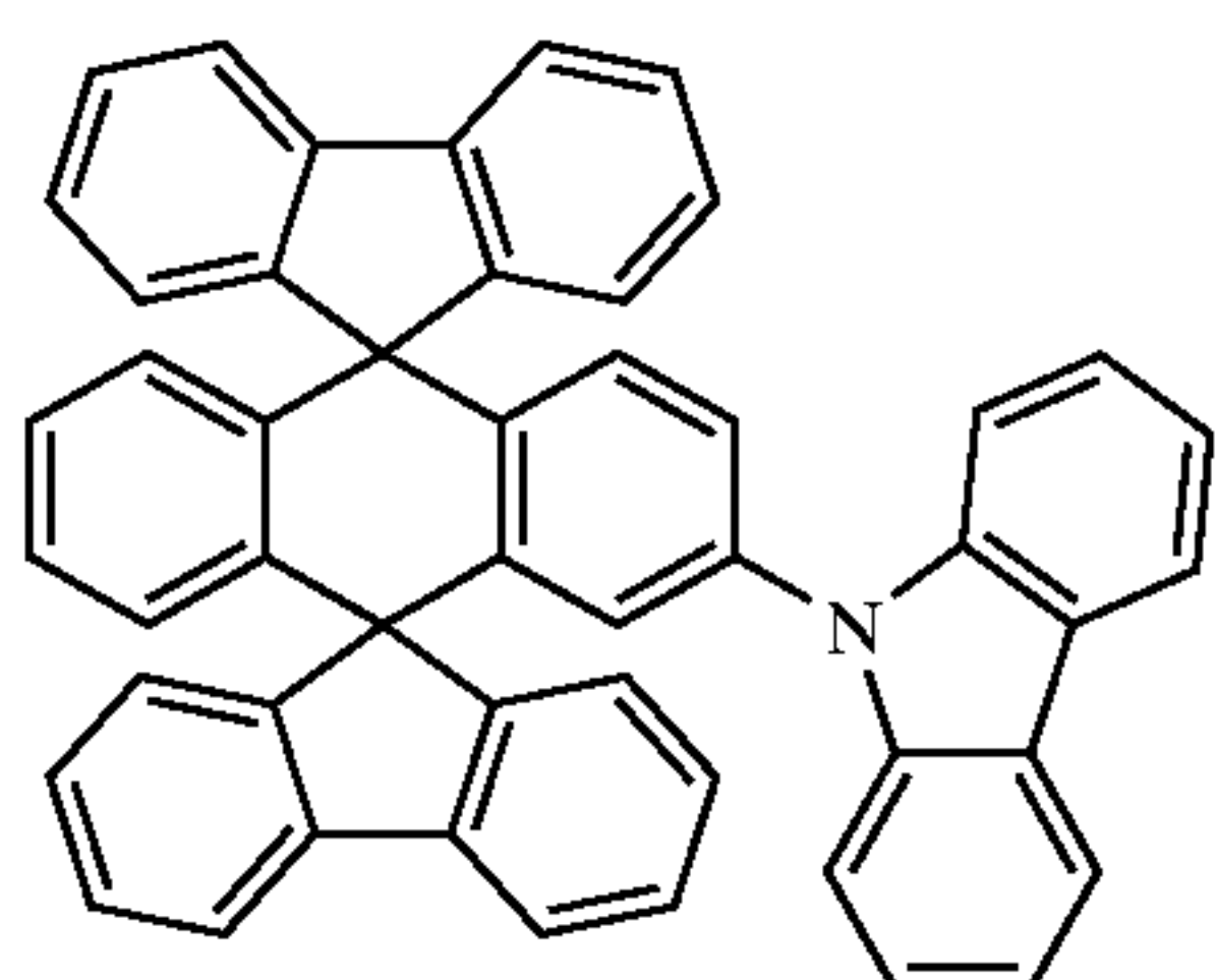
Chemical Compound 10
