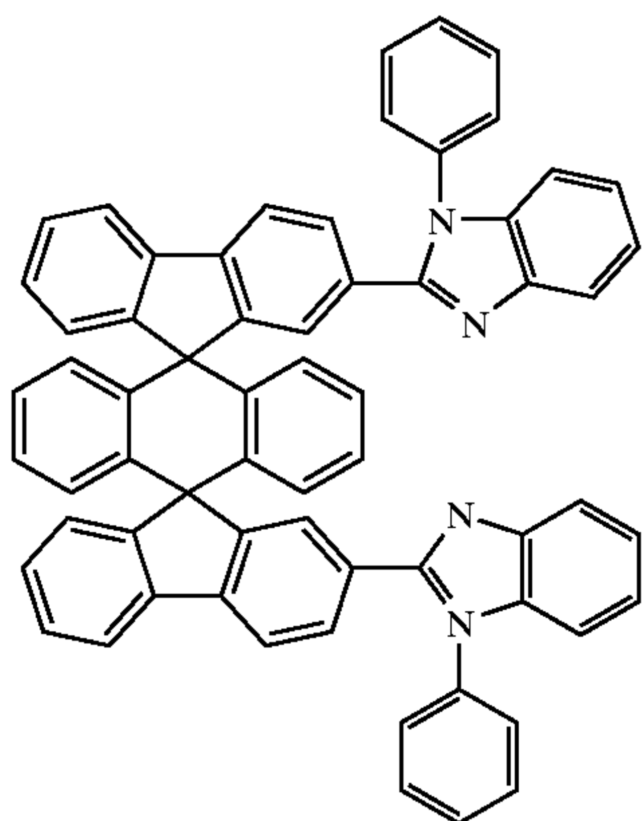
Chemical Compound 221
