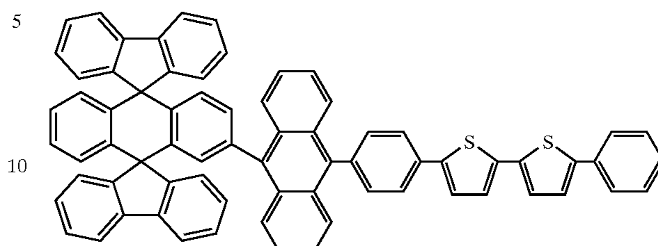
Chemical Compound 131
