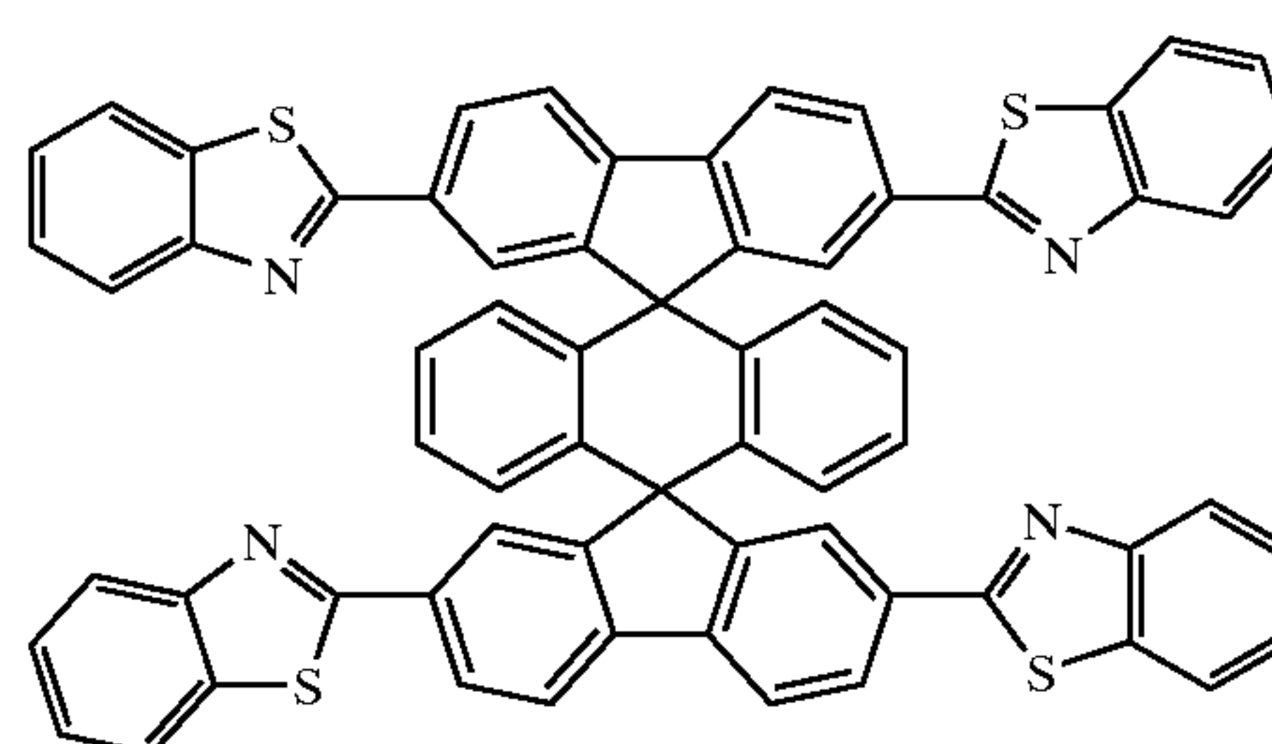
Chemical Compound 218
