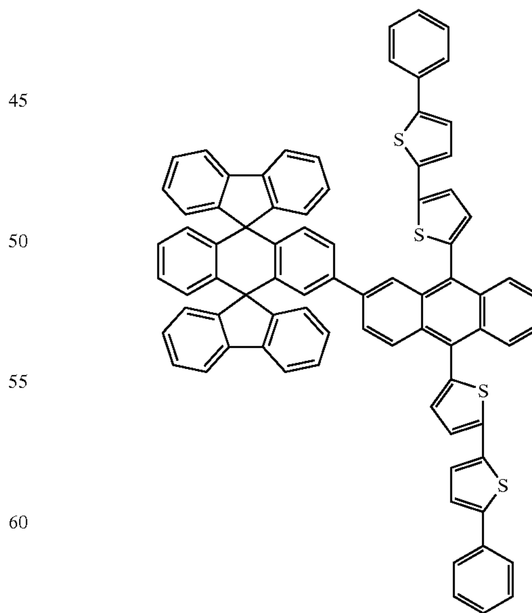
Chemical Compound 128
