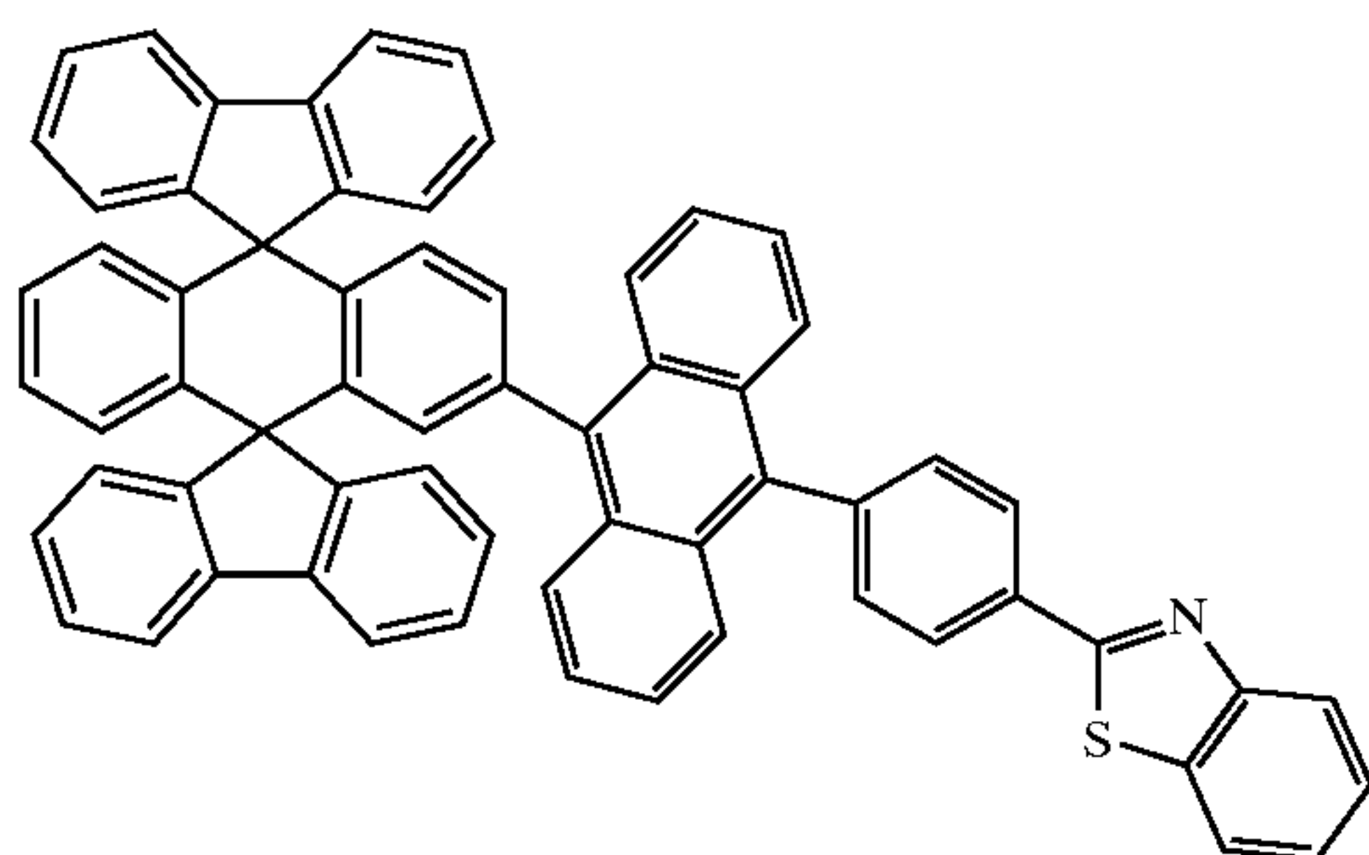
Chemical Compound 217
