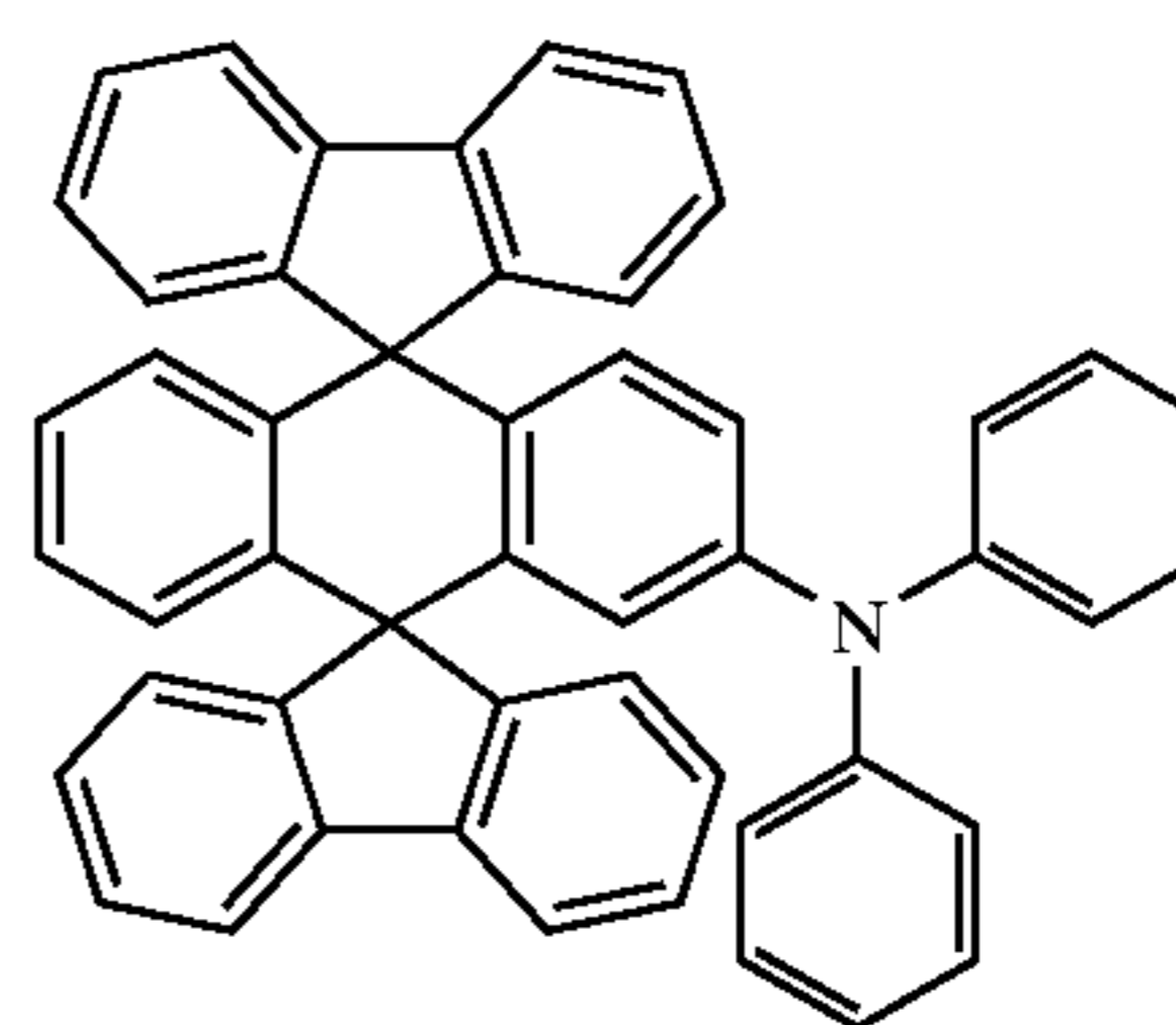
Chemical Compound 300
