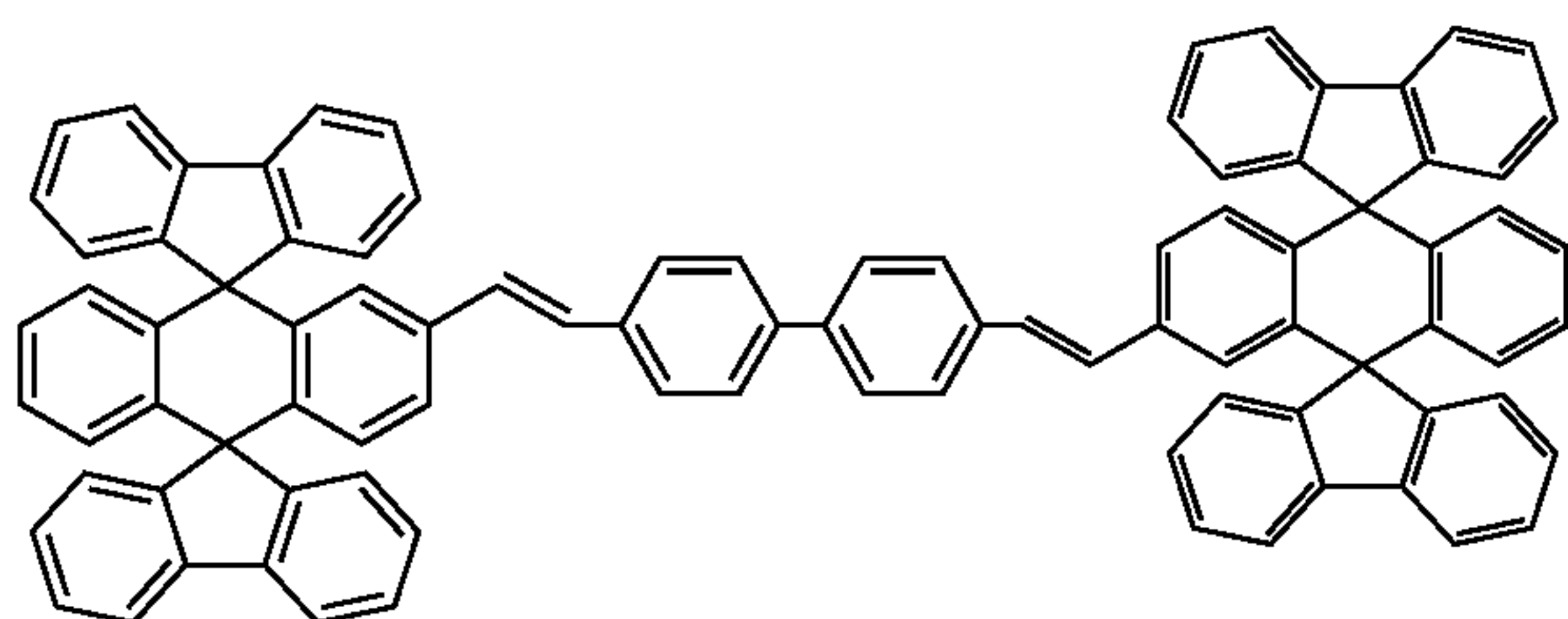
Chemical Compound 100
