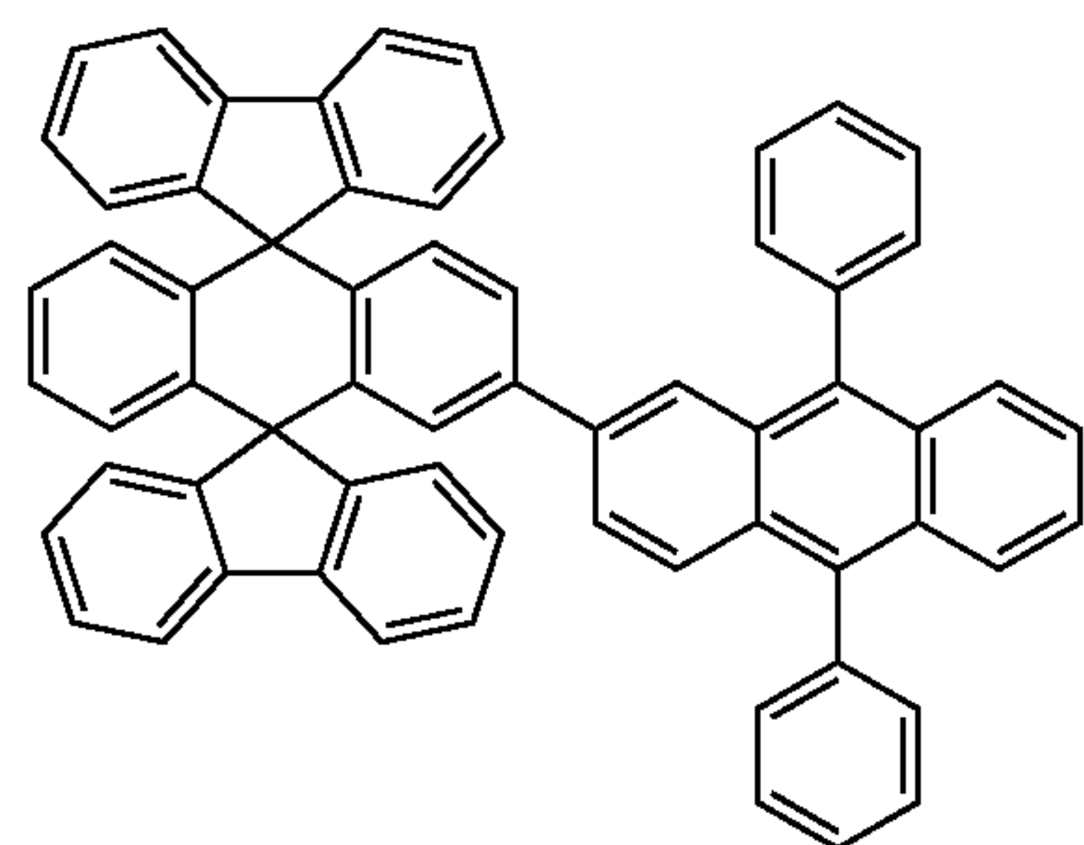
Chemical Compound 116
