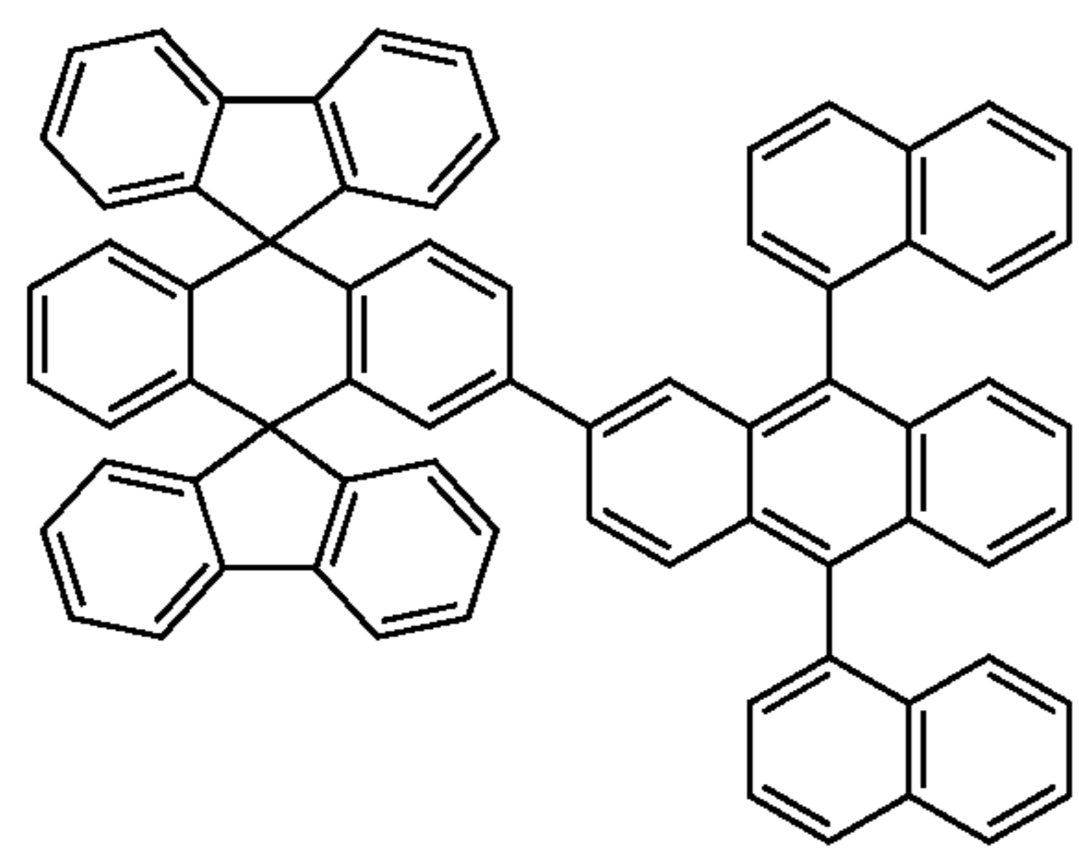
Chemical Compound 120
