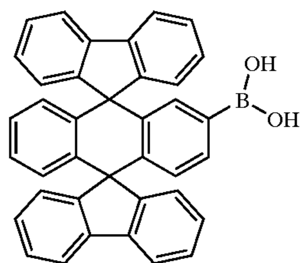
Chemical Compound 8
