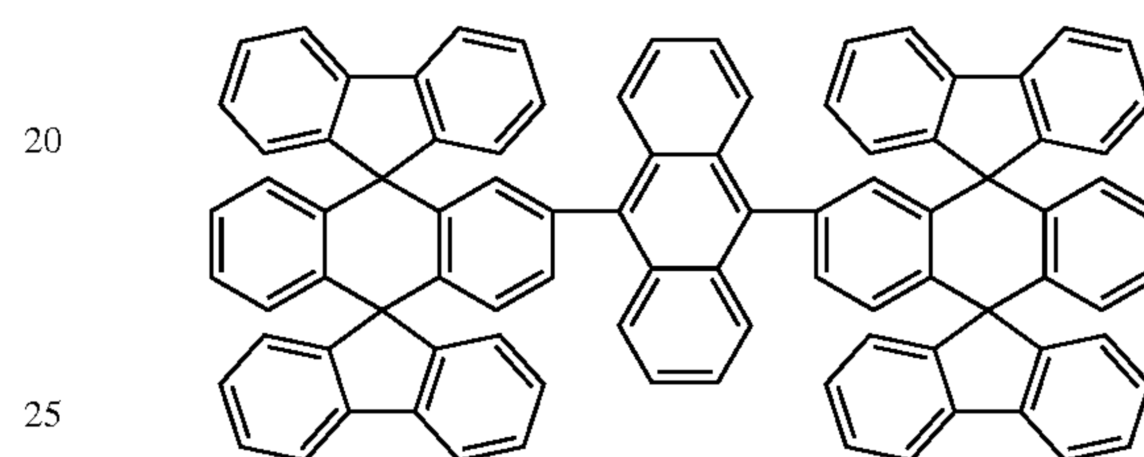
Chemical Compound 102
