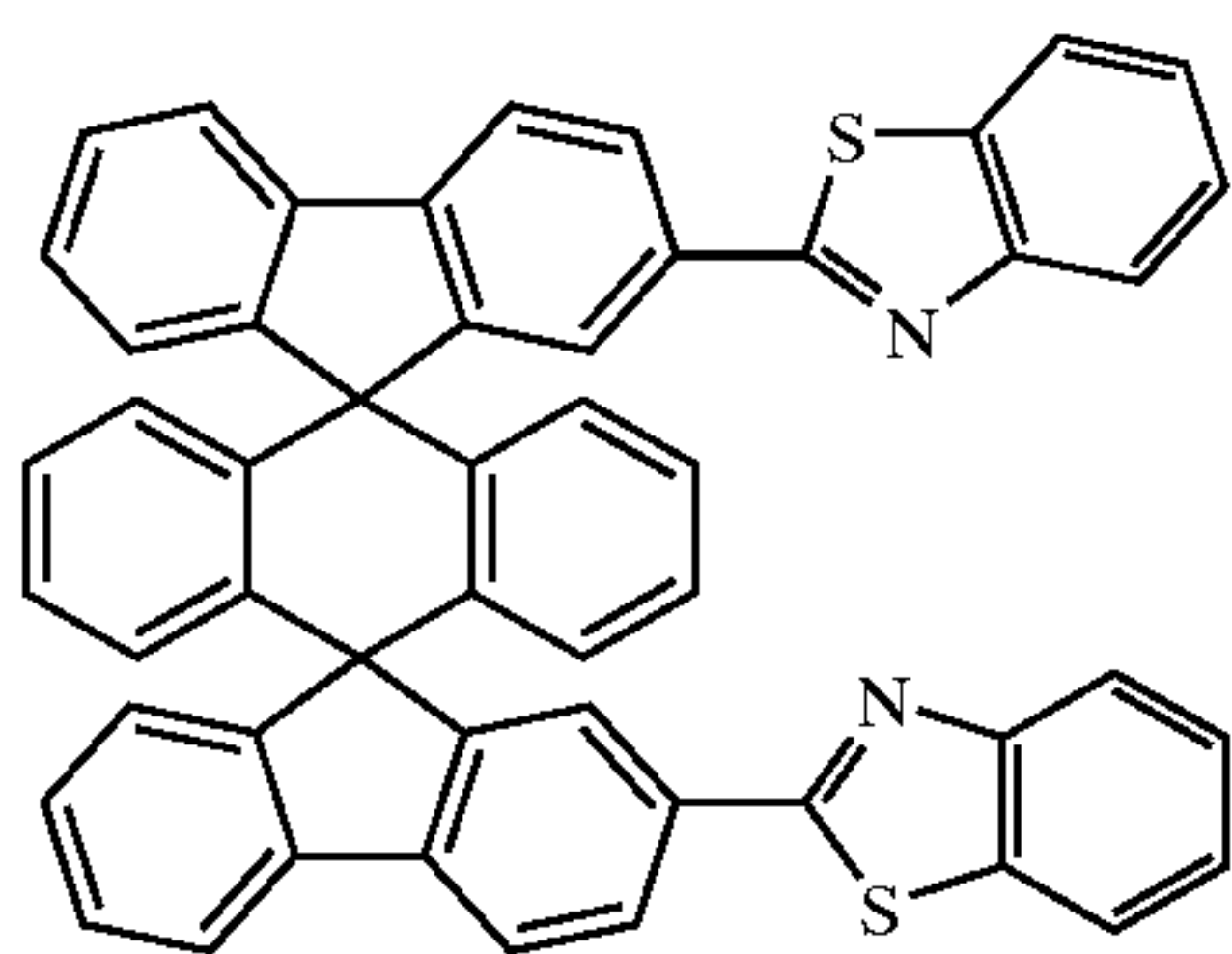
Chemical Compound 220
