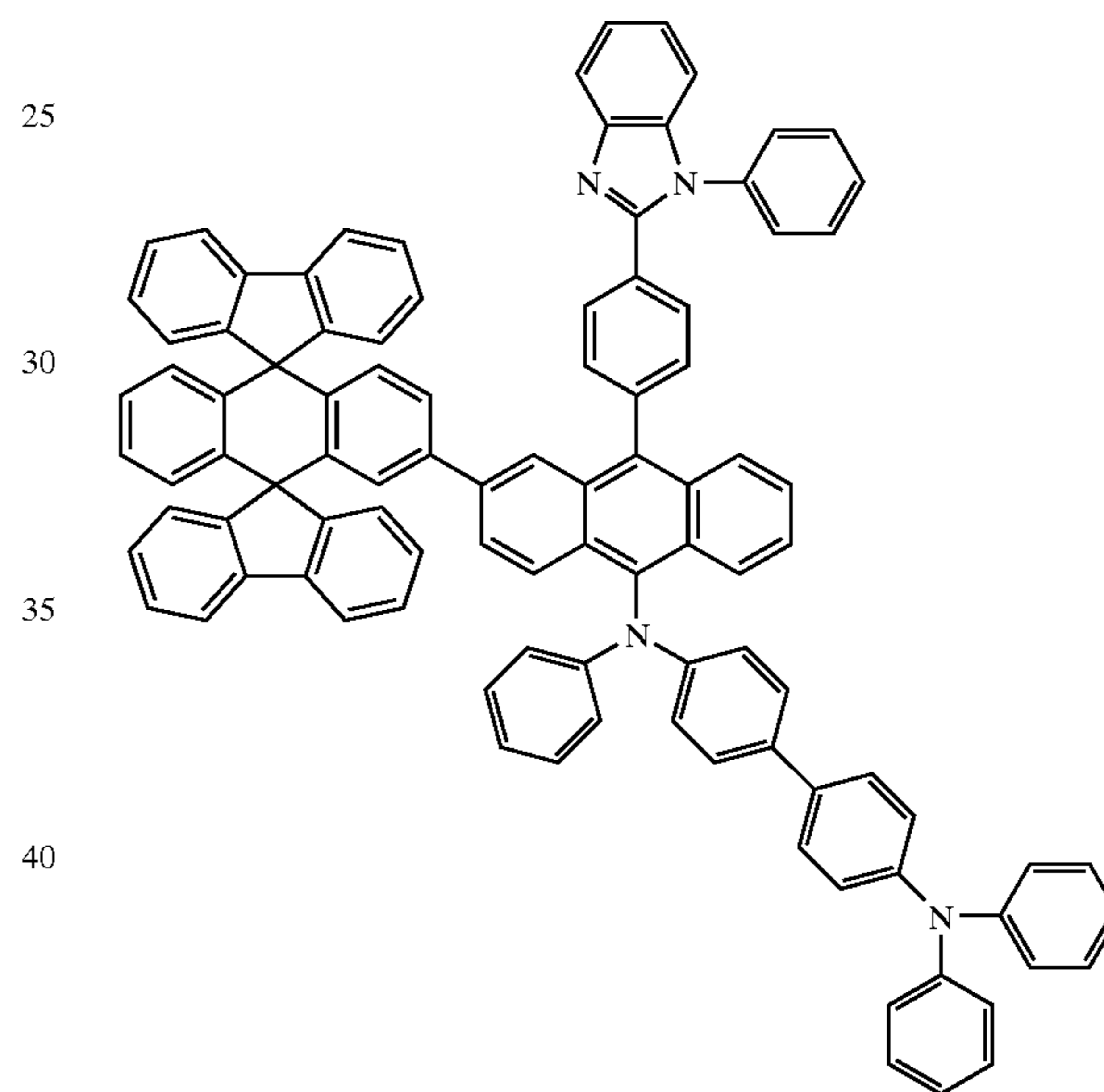
Chemical Compound 124
