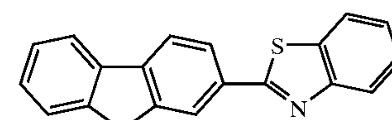
Chemical Compound 219
