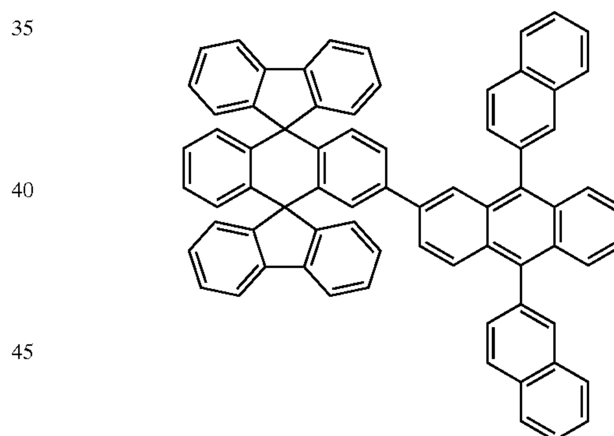
Chemical Compound 117
