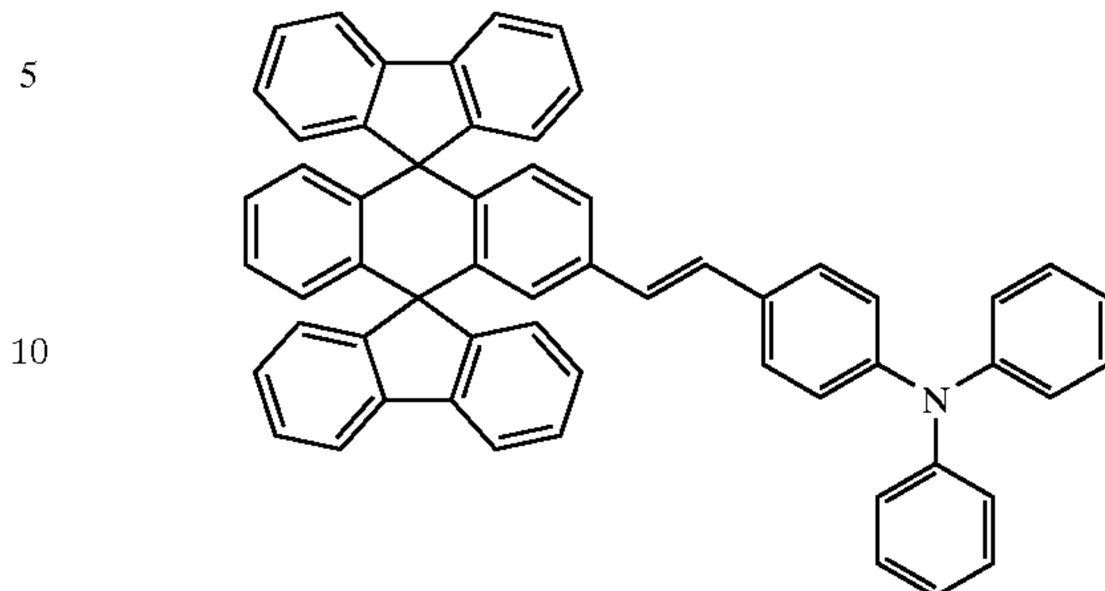
Chemical Compound 400
