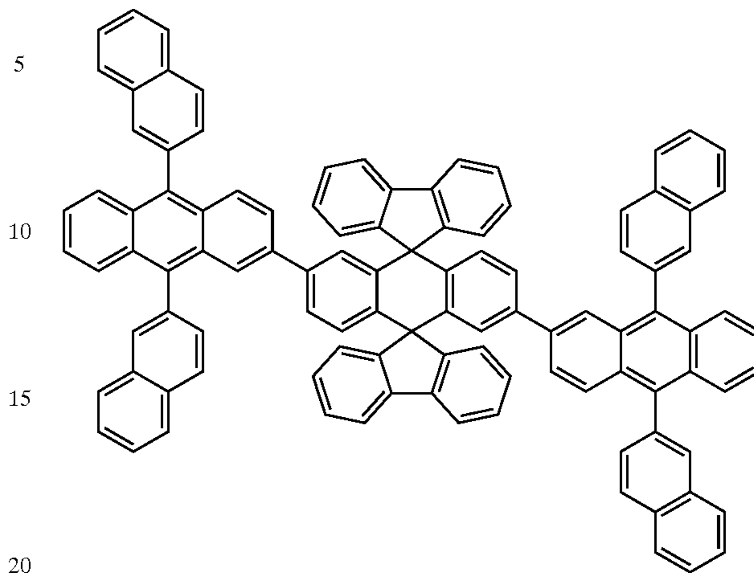
Chemical Compound 123
