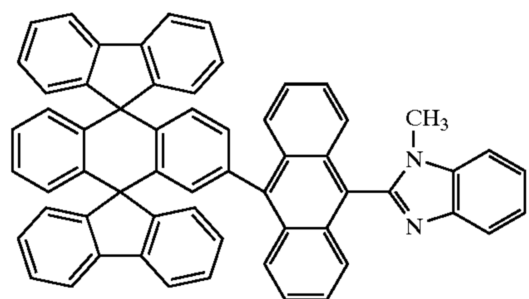
Chemical Compound 205
