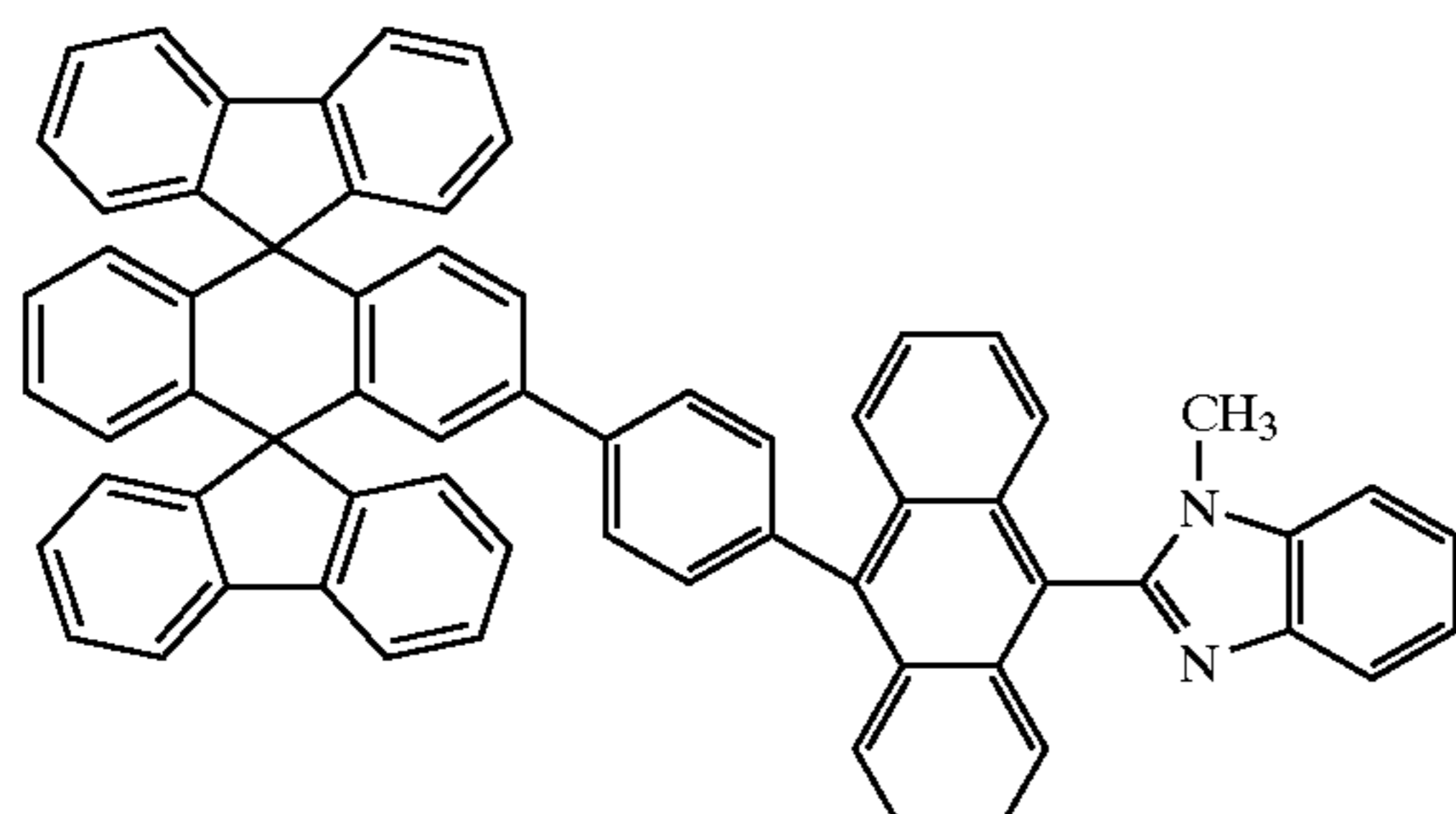
Chemical Compound 201
