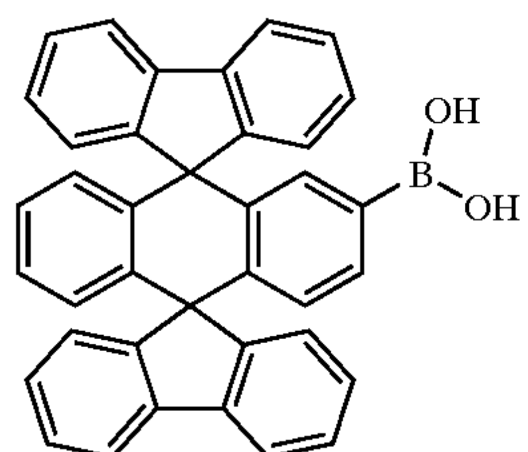
Chemical Compound 8
