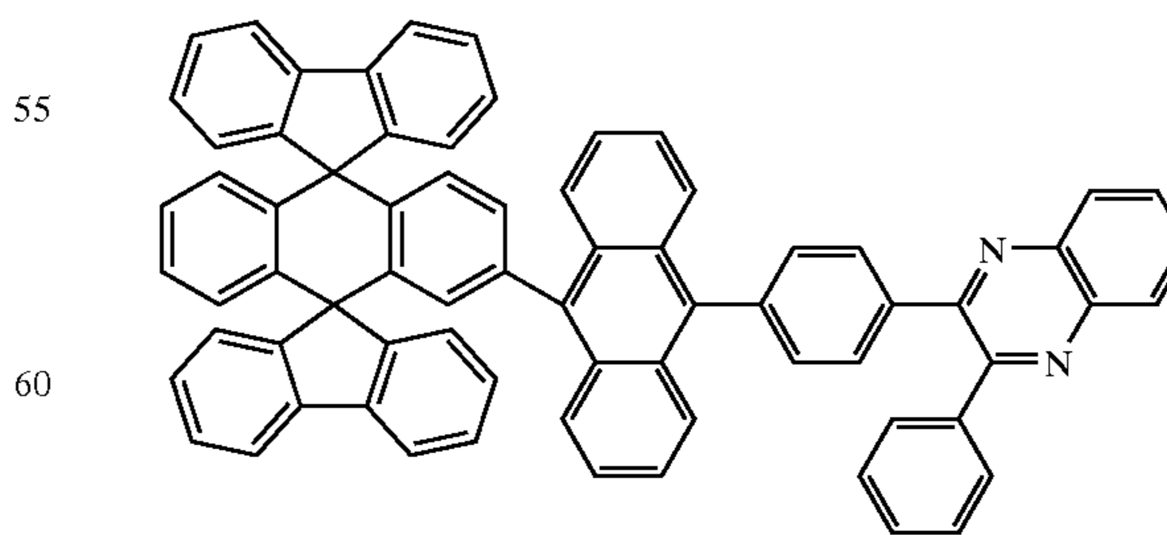
Chemical Compound 209
