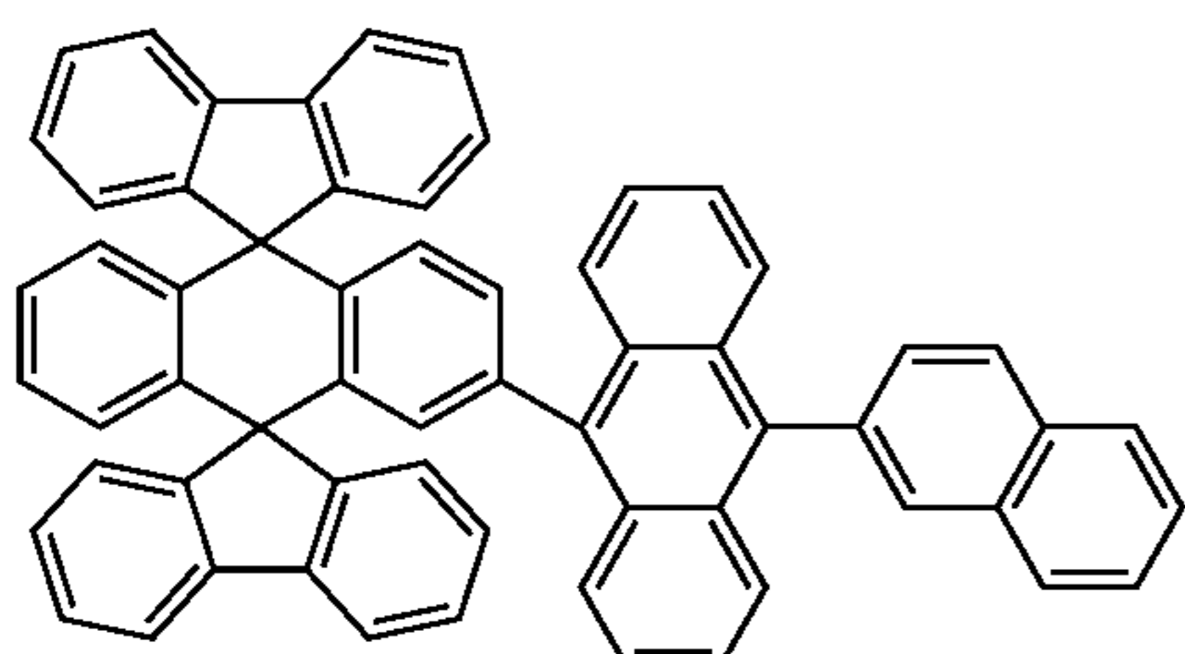
Chemical Compound 110
