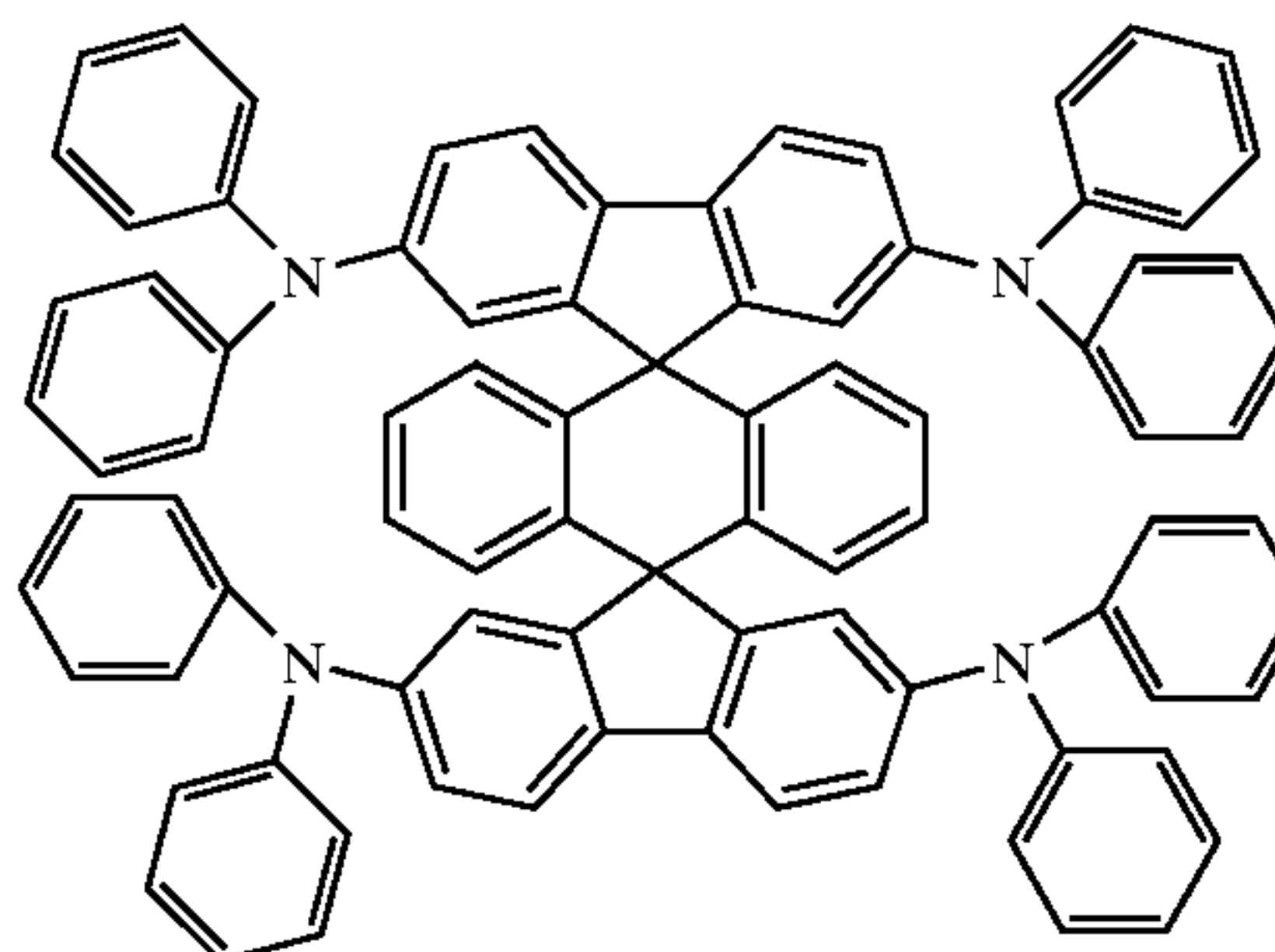
Chemical Compound 304
