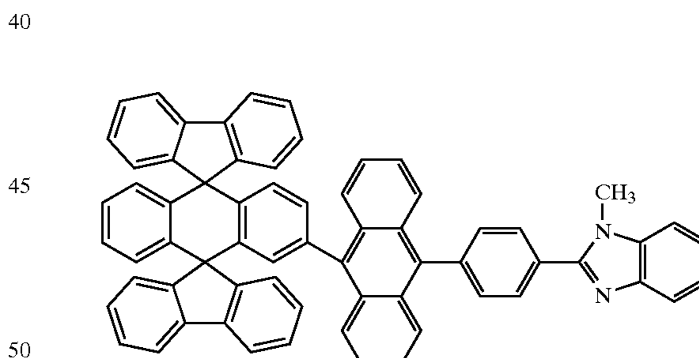
Chemical Compound 208
