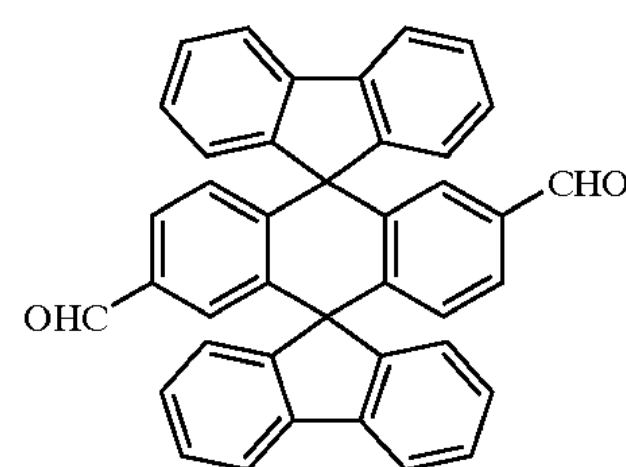
Chemical Compound 4
