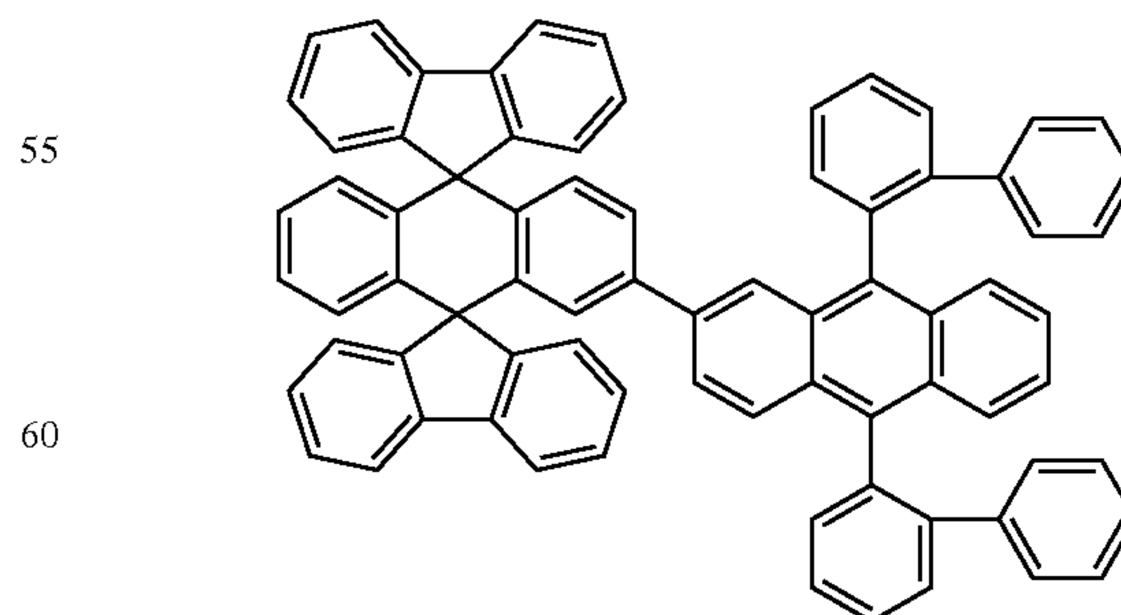
Chemical Compound 118
