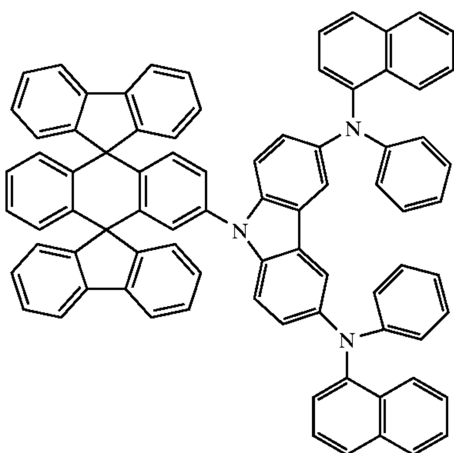
Chemical Compound 403
