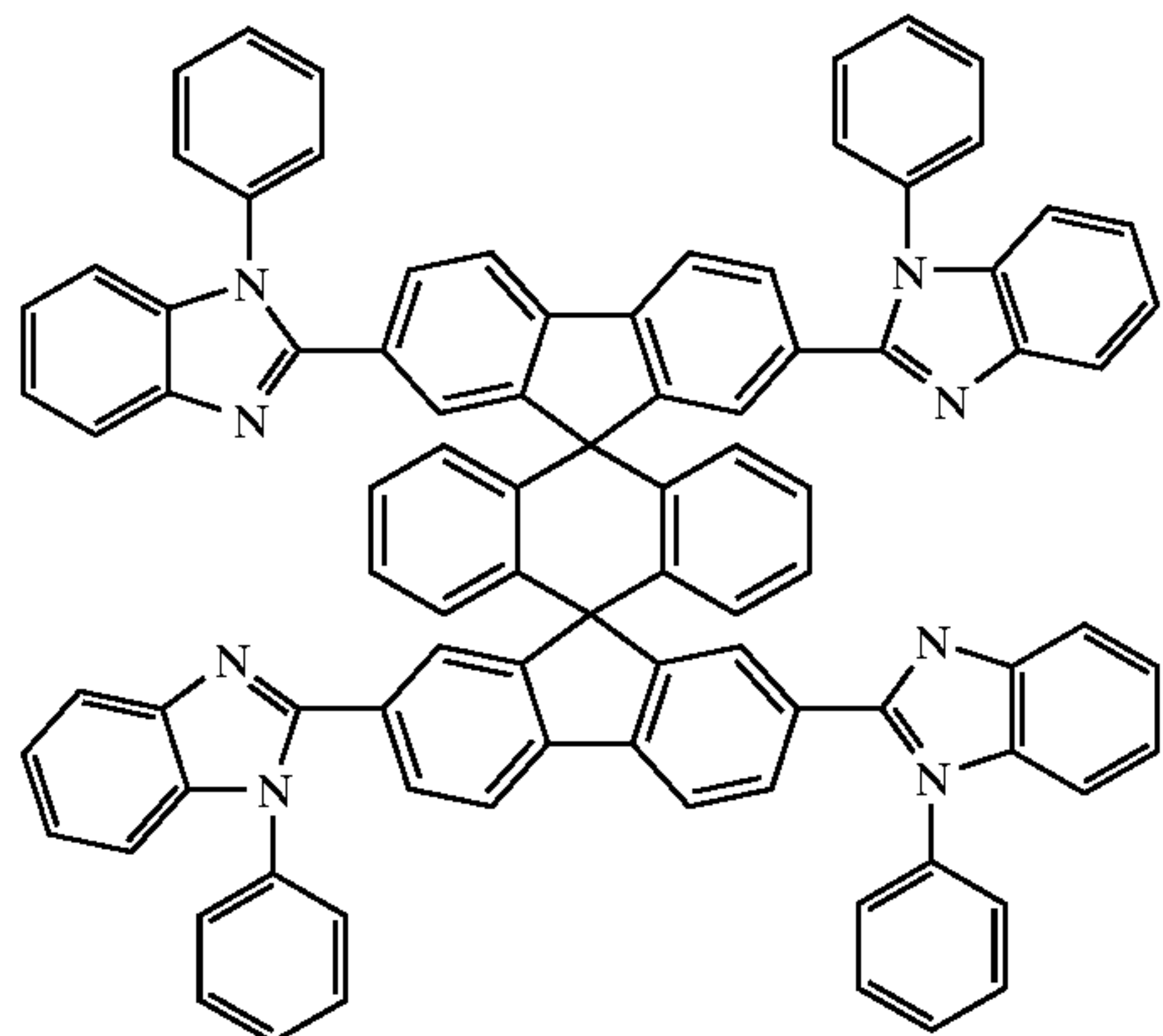
Chemical Compound 219
