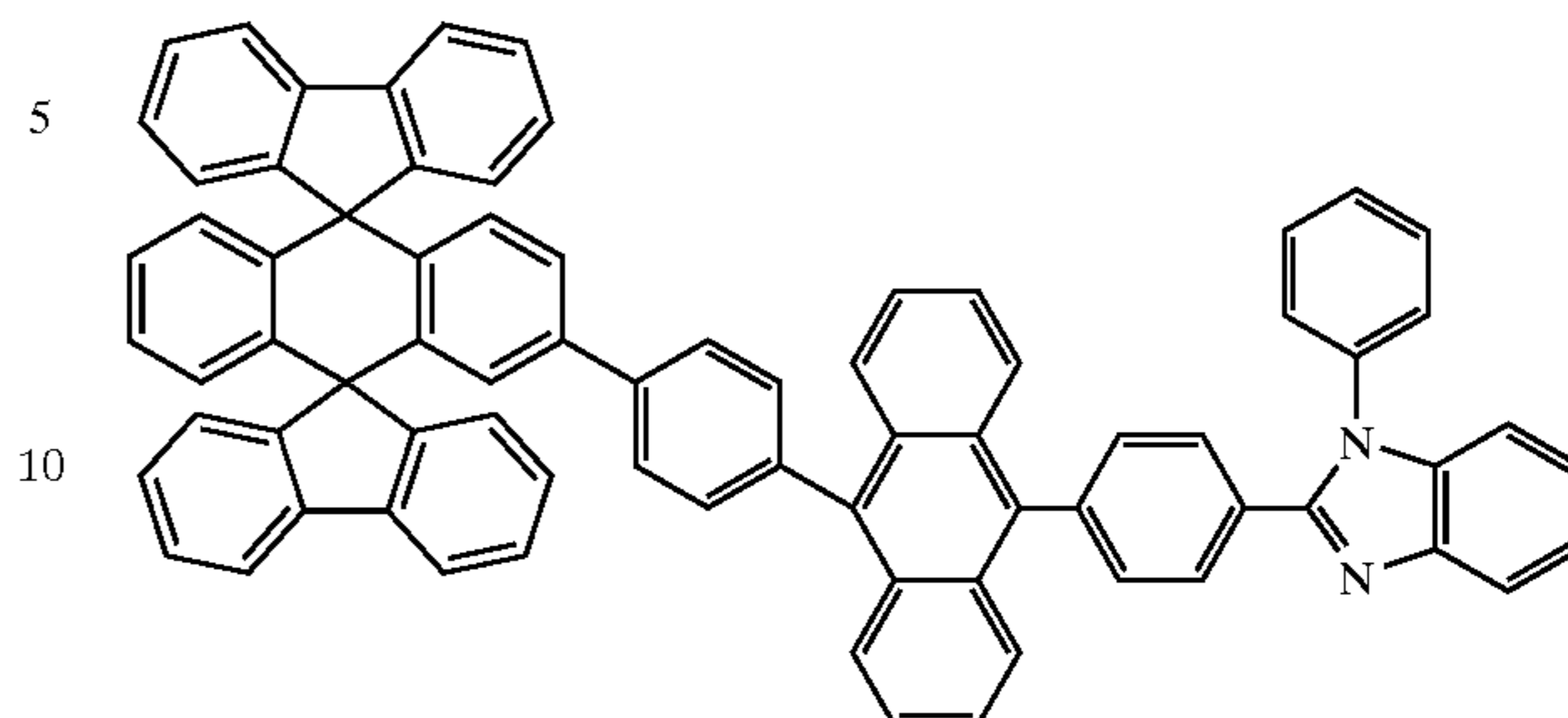
Chemical Compound 210
