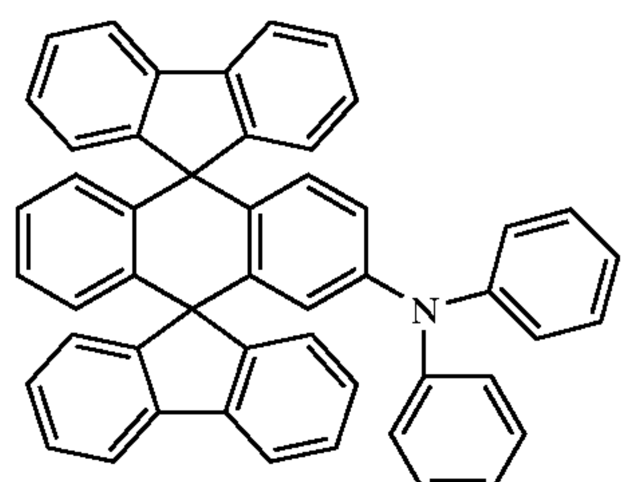
Chemical Compound 11
