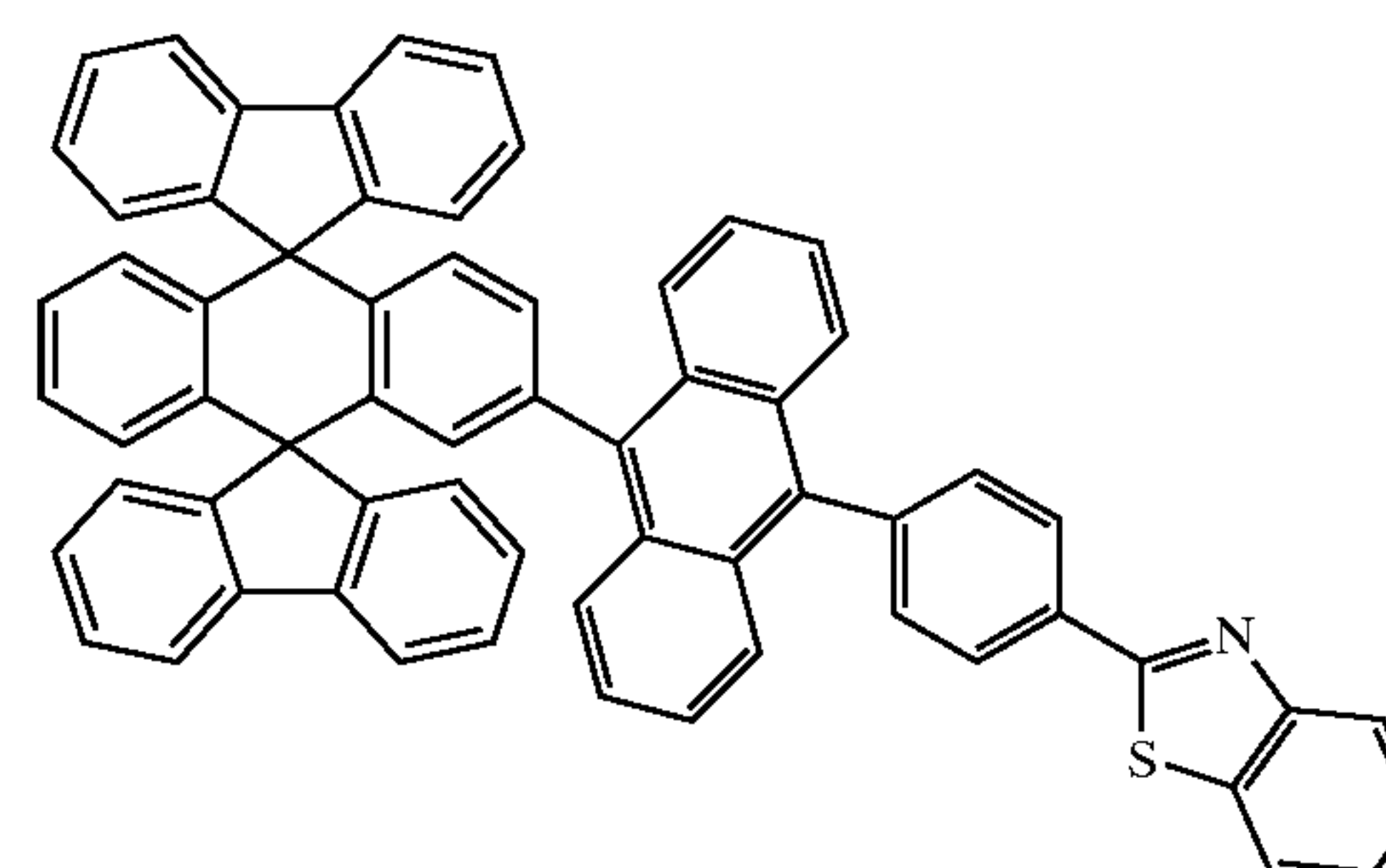
Chemical Compound 217
