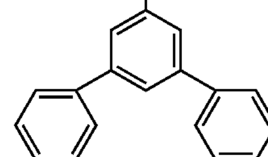
Chemical Compound 119
