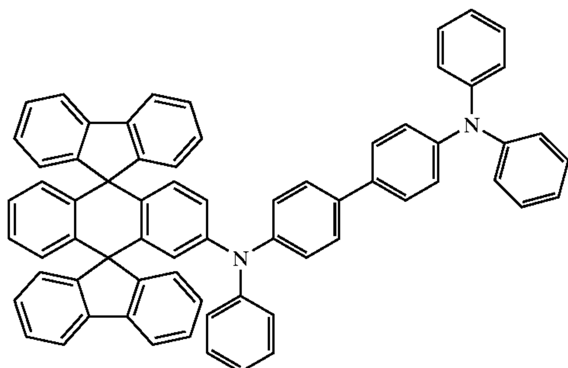
Chemical Compound 307
