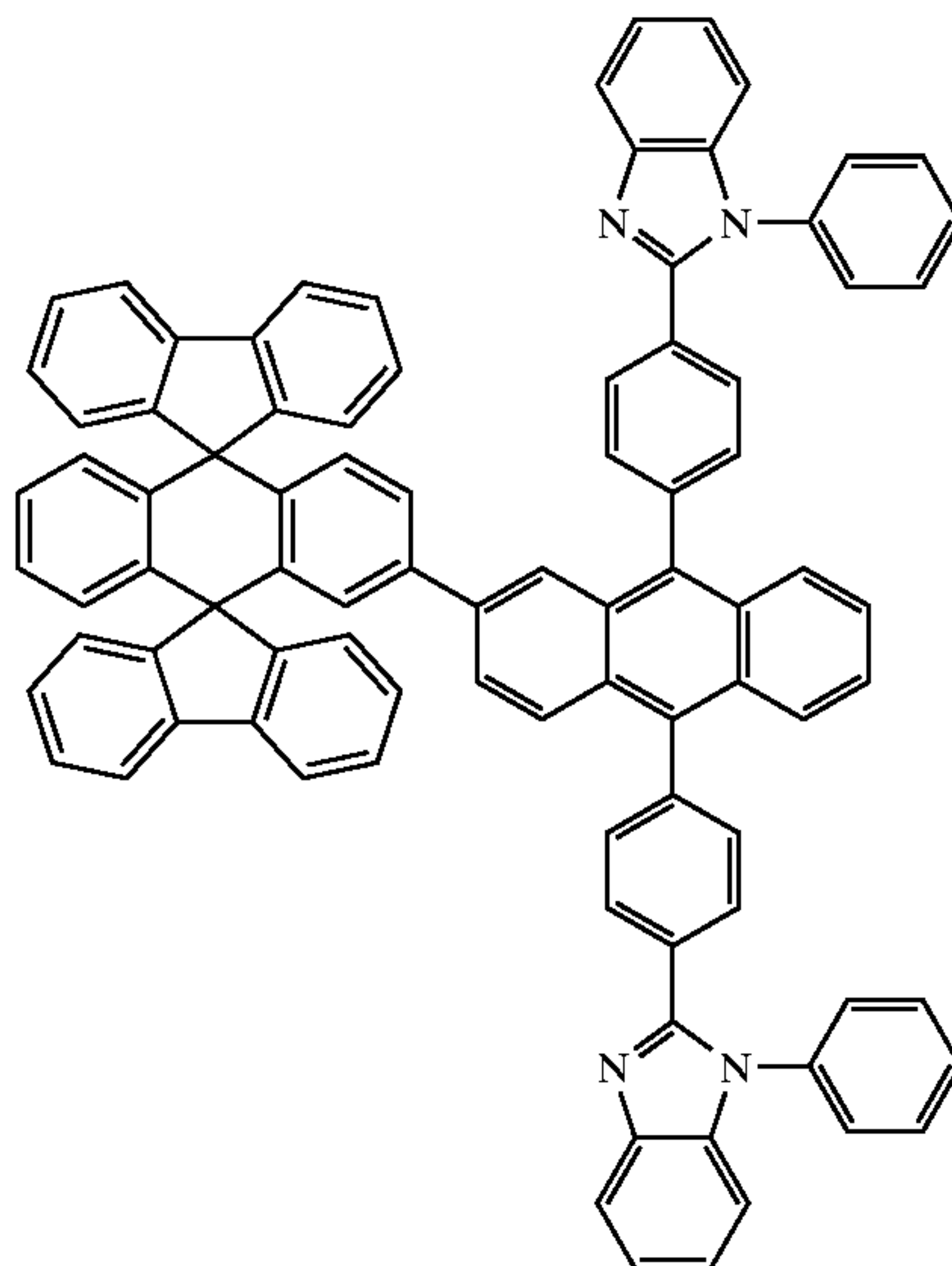
Chemical Compound 206
