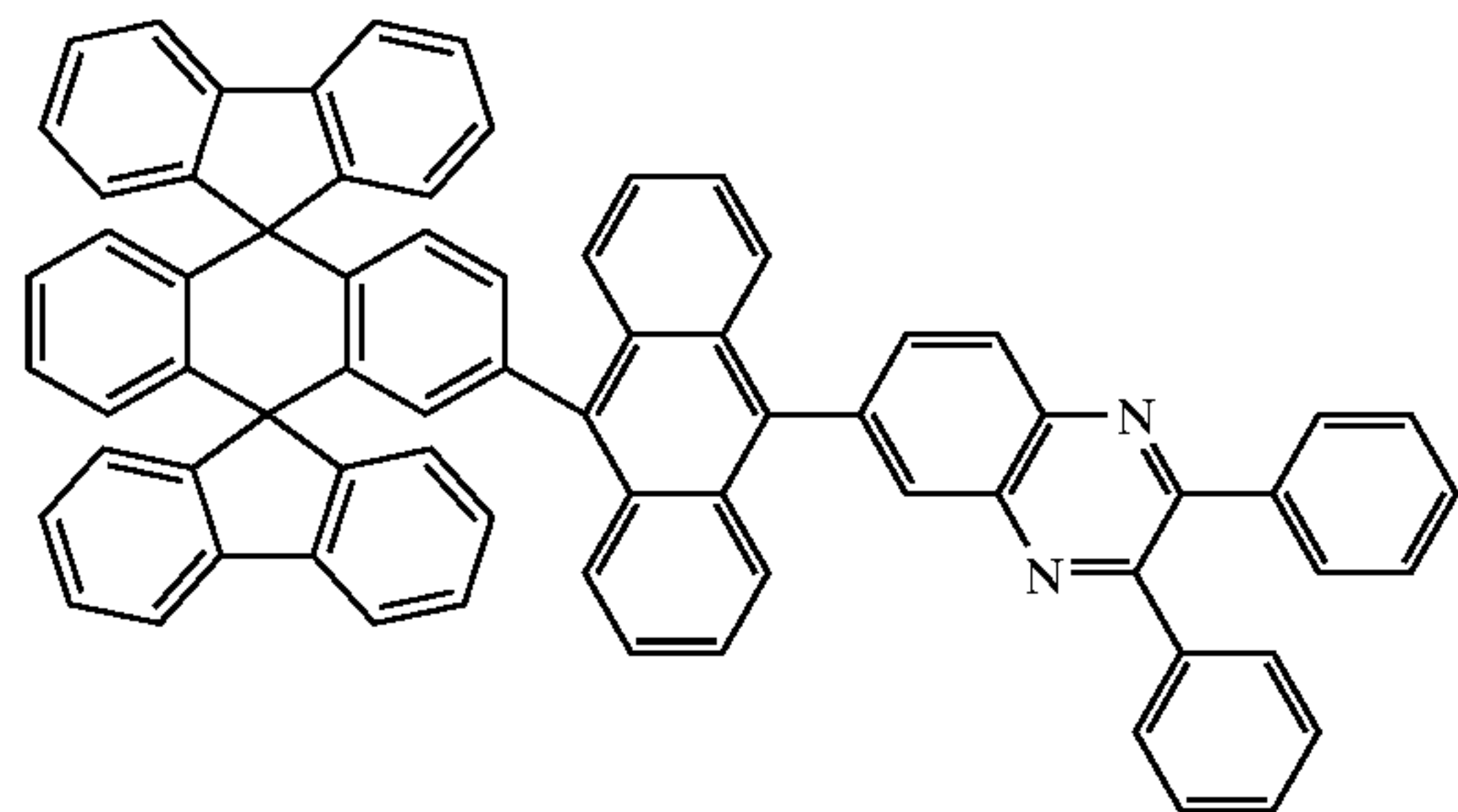
Chemical Compound 203
