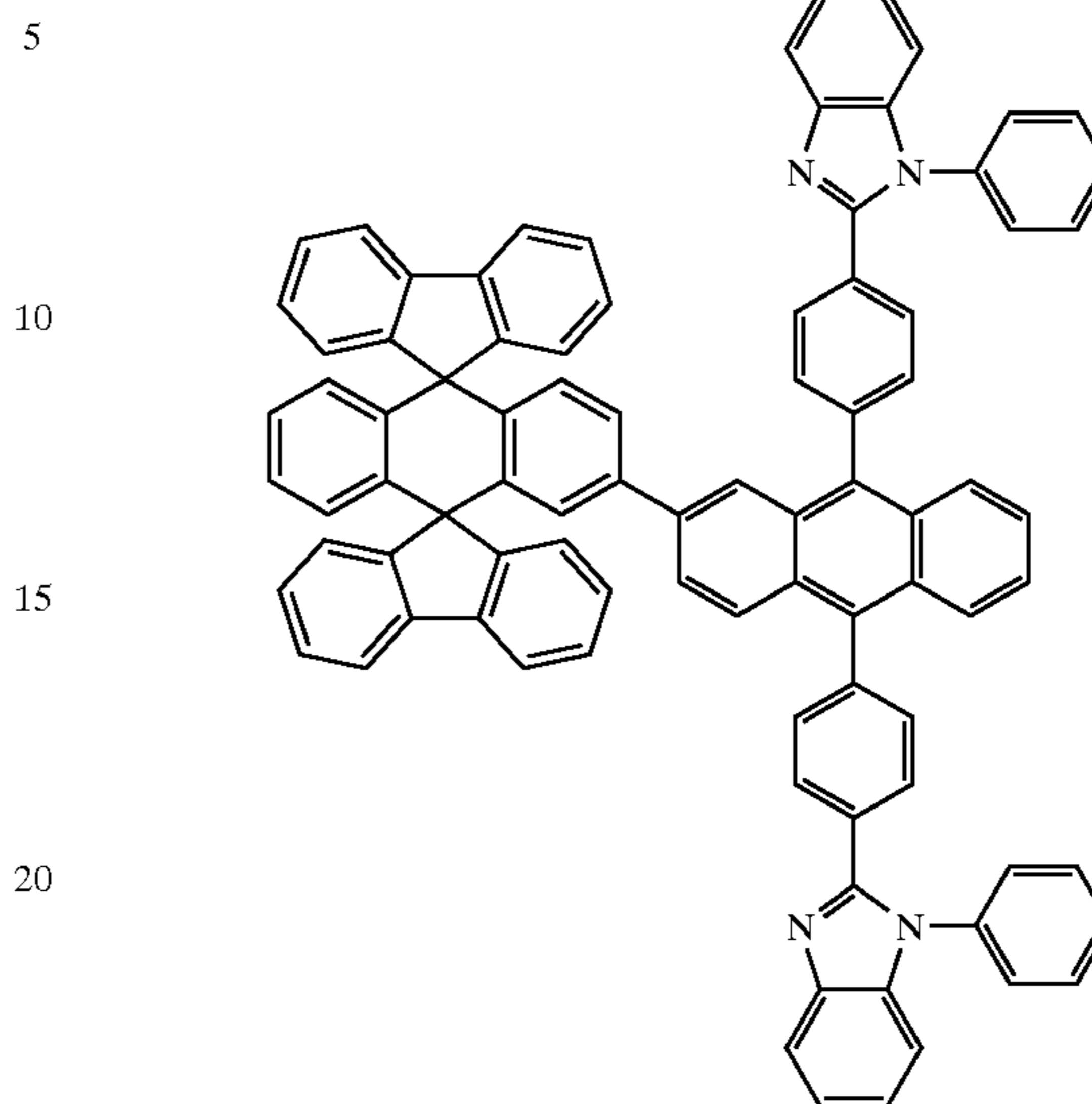
Chemical Compound 206
