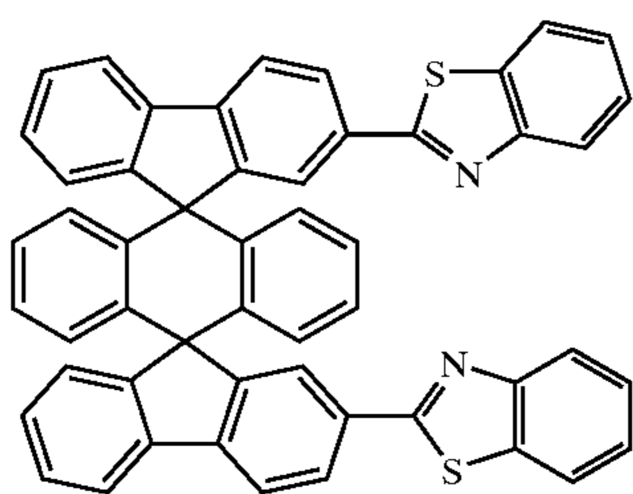
Chemical Compound 220
