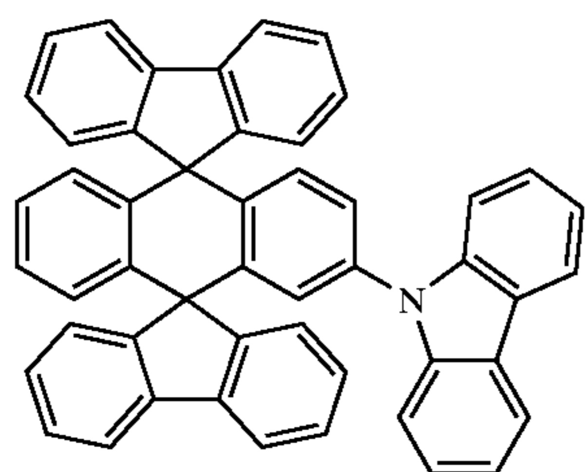
Chemical Compound 10
