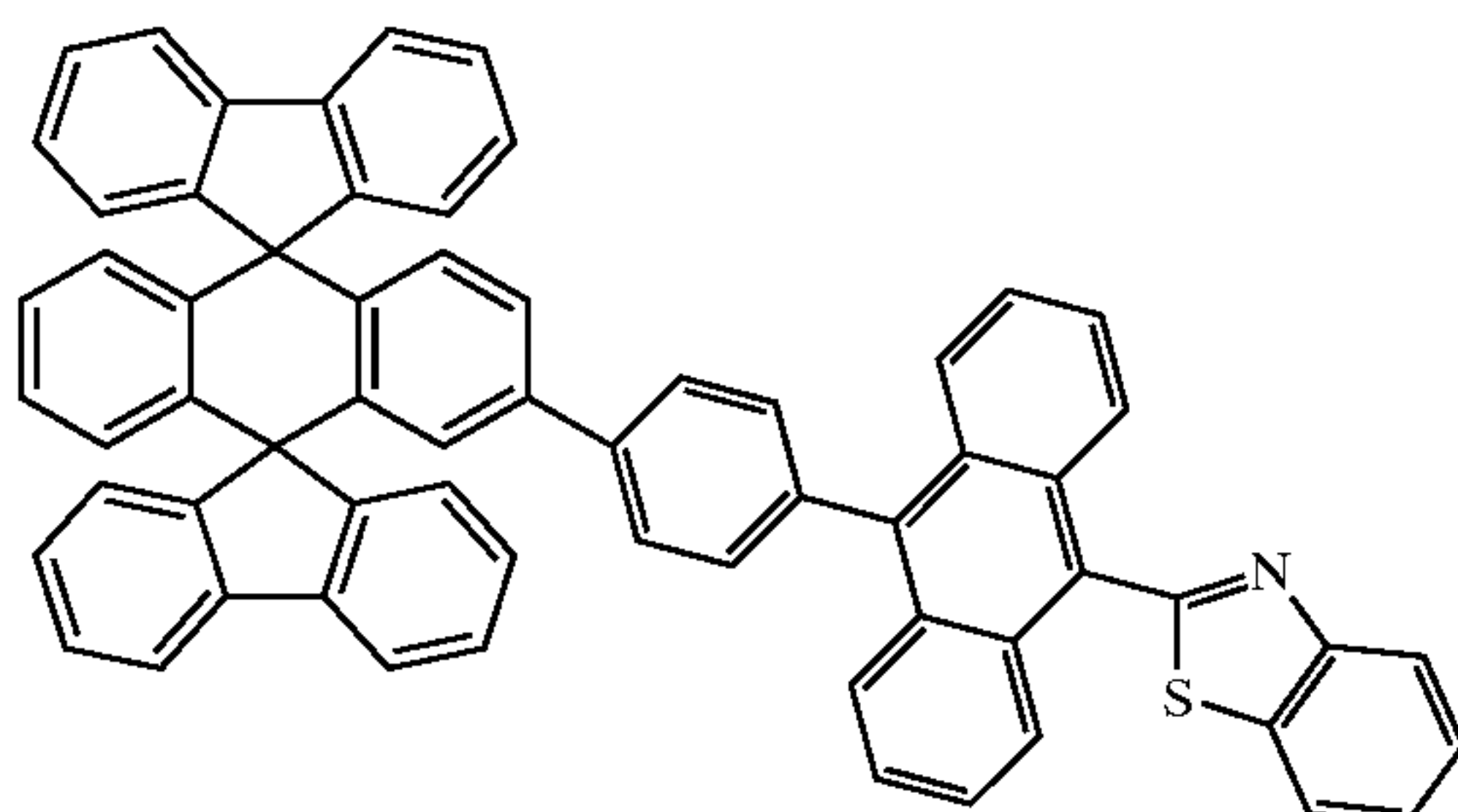
Chemical Compound 216
