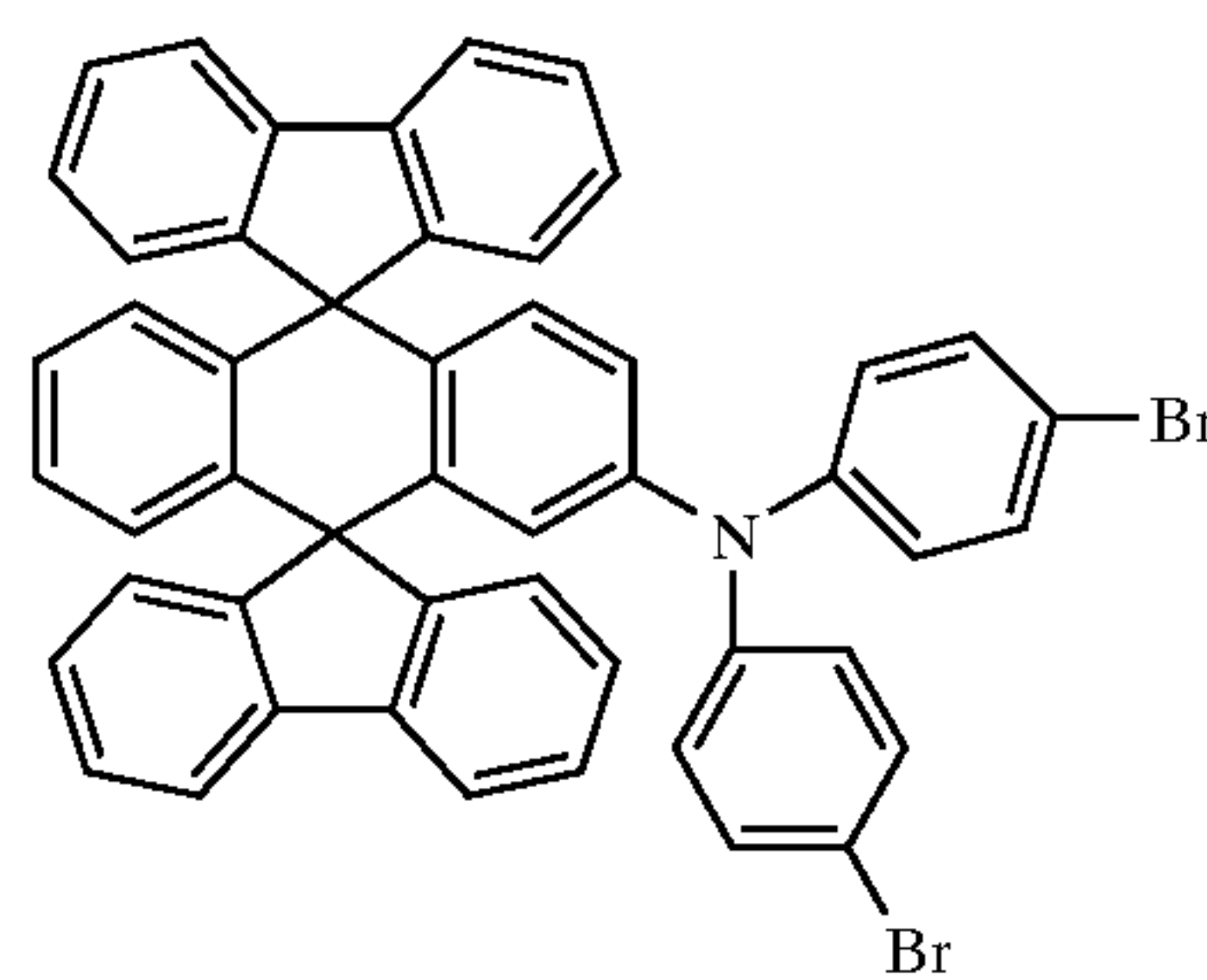
Chemical Compound 7
