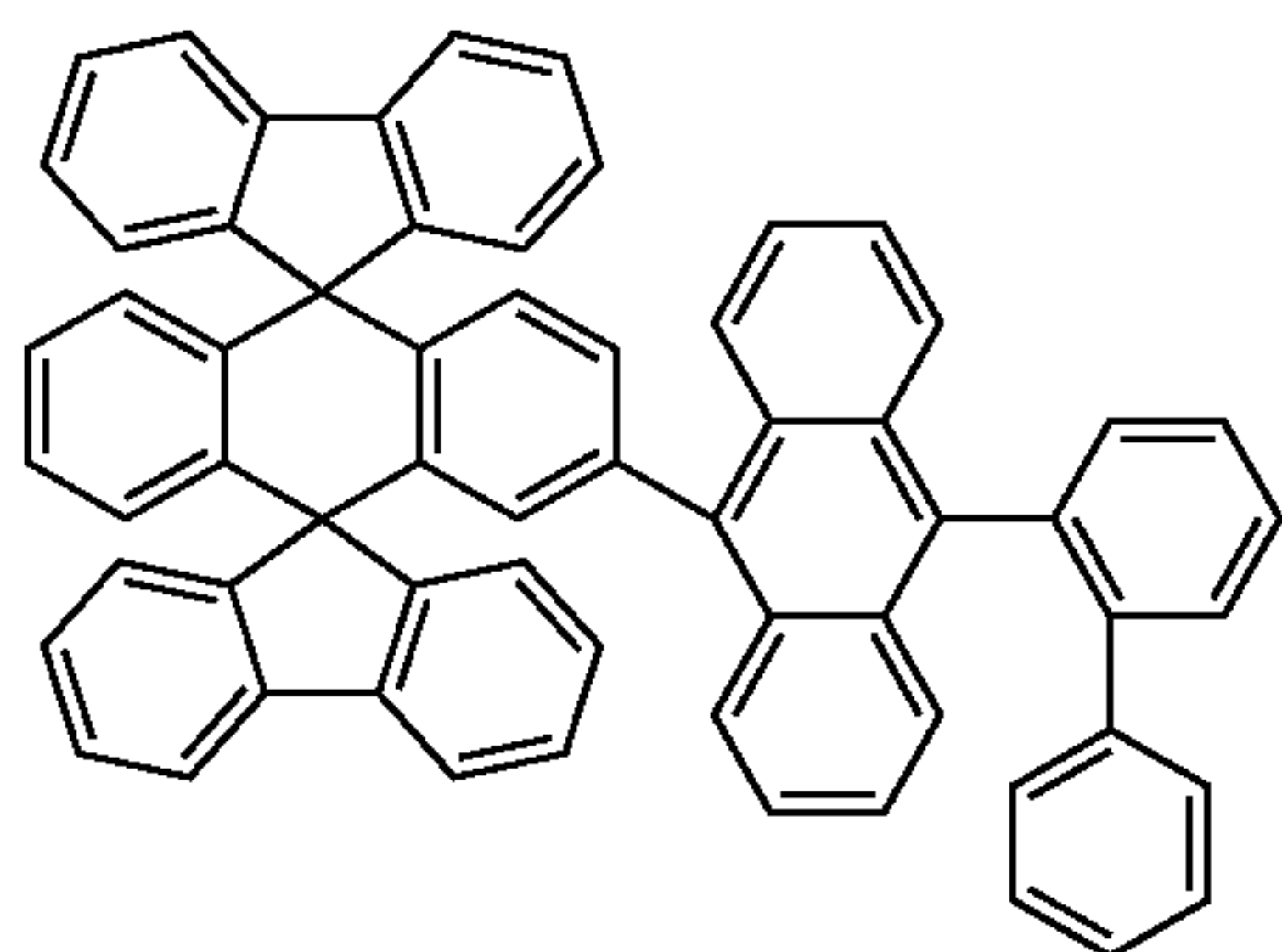
Chemical Compound 111
