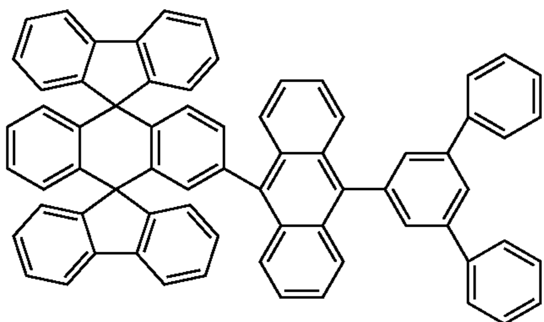
Chemical Compound 113
