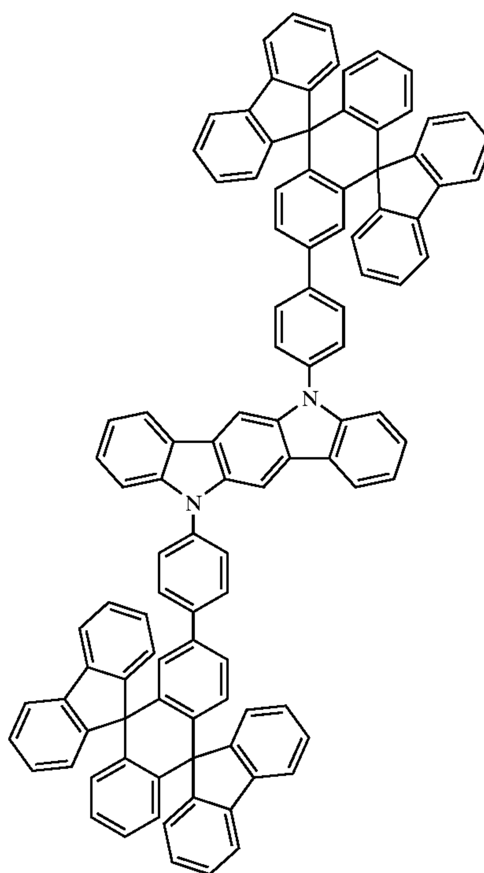
Chemical Compound 409
