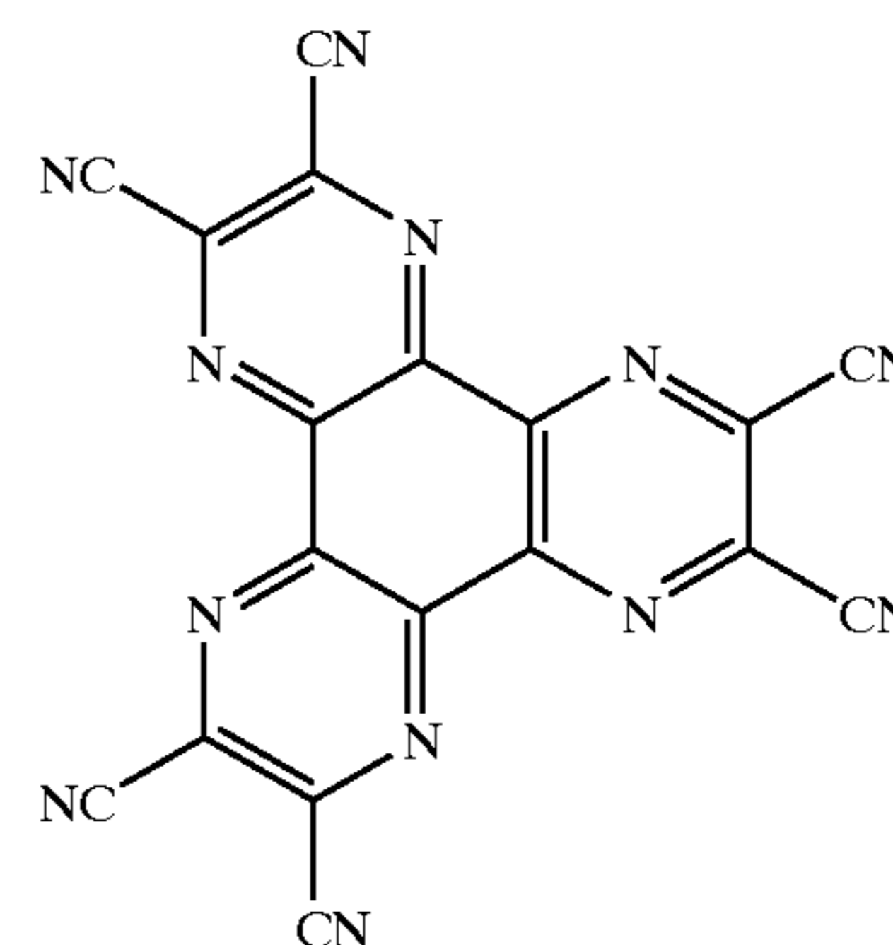
Hexanitrite hexaazatriphenylene
