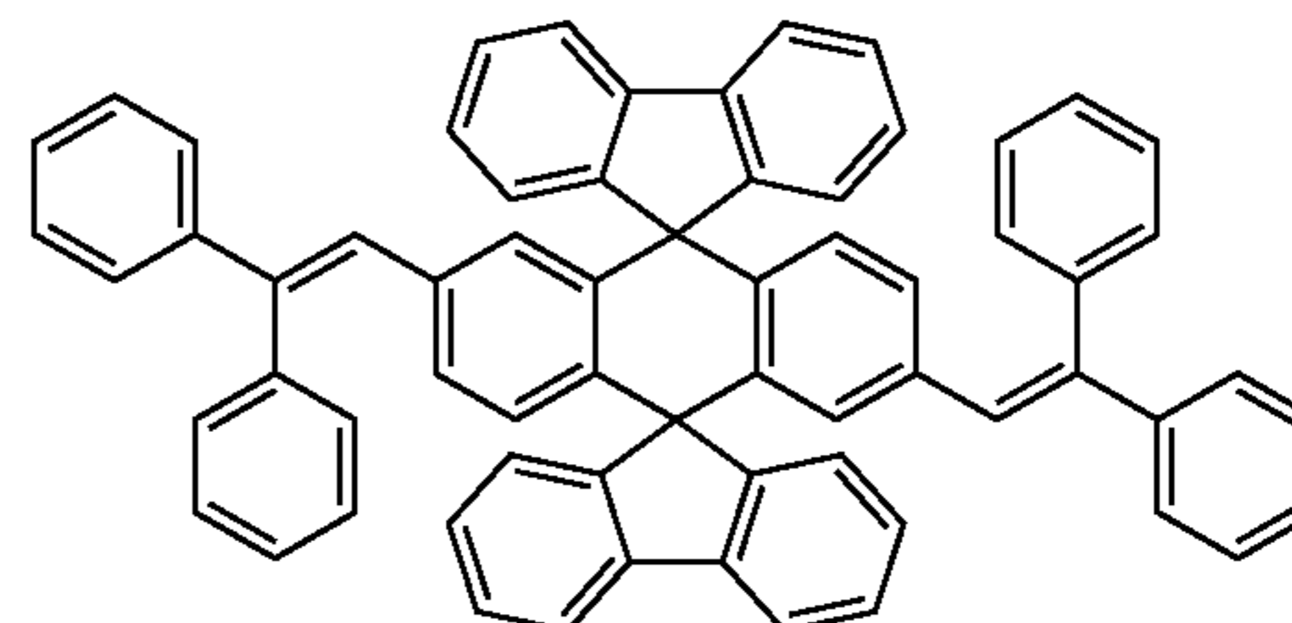
Chemical Compound 105
