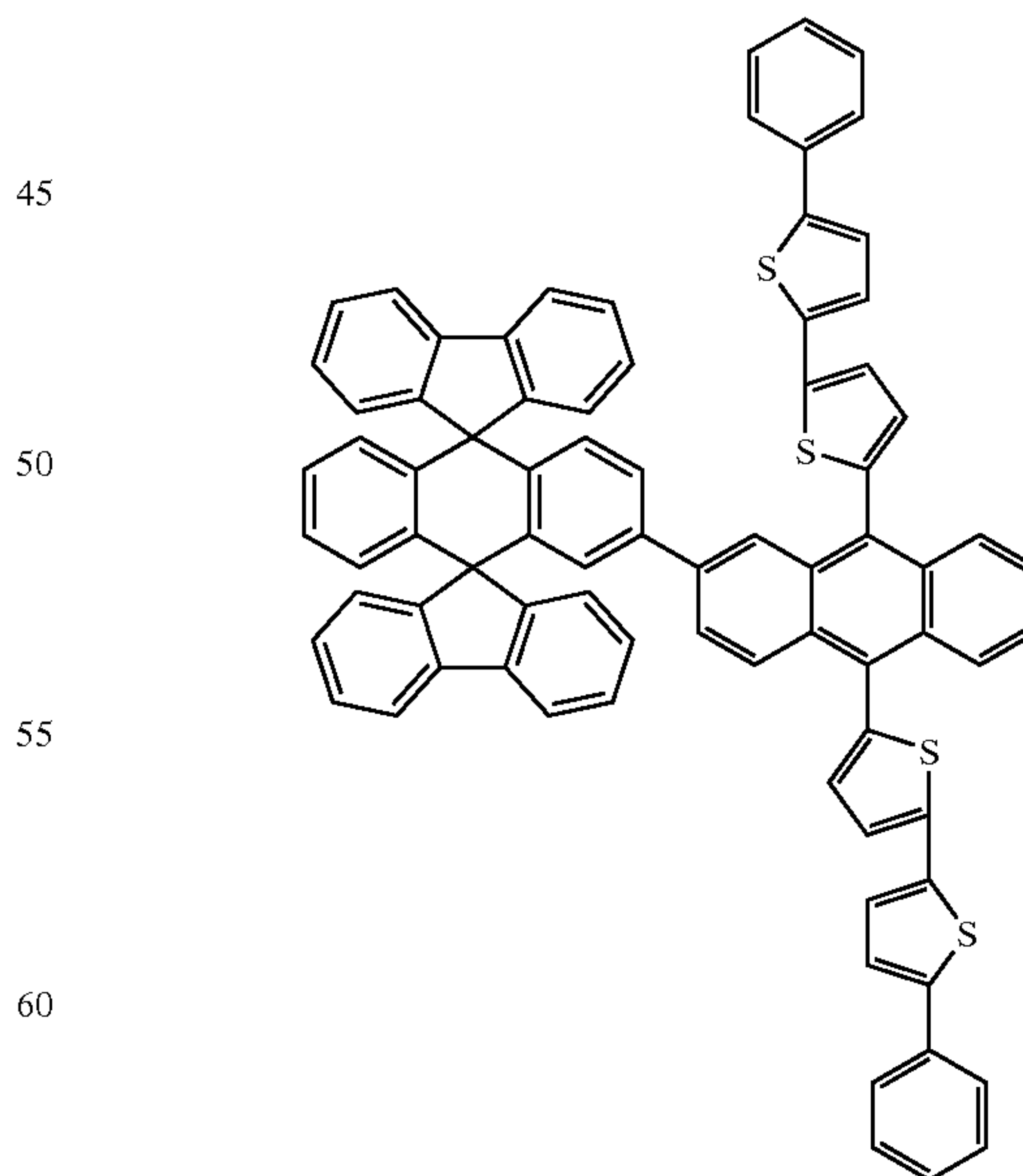
Chemical Compound 128
