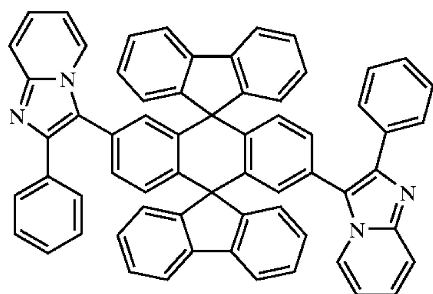
Chemical Compound 413
