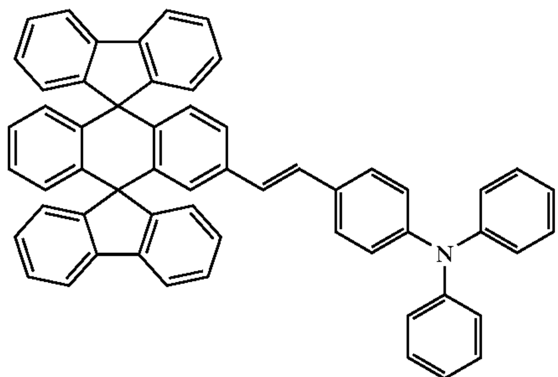
Chemical Compound 400
