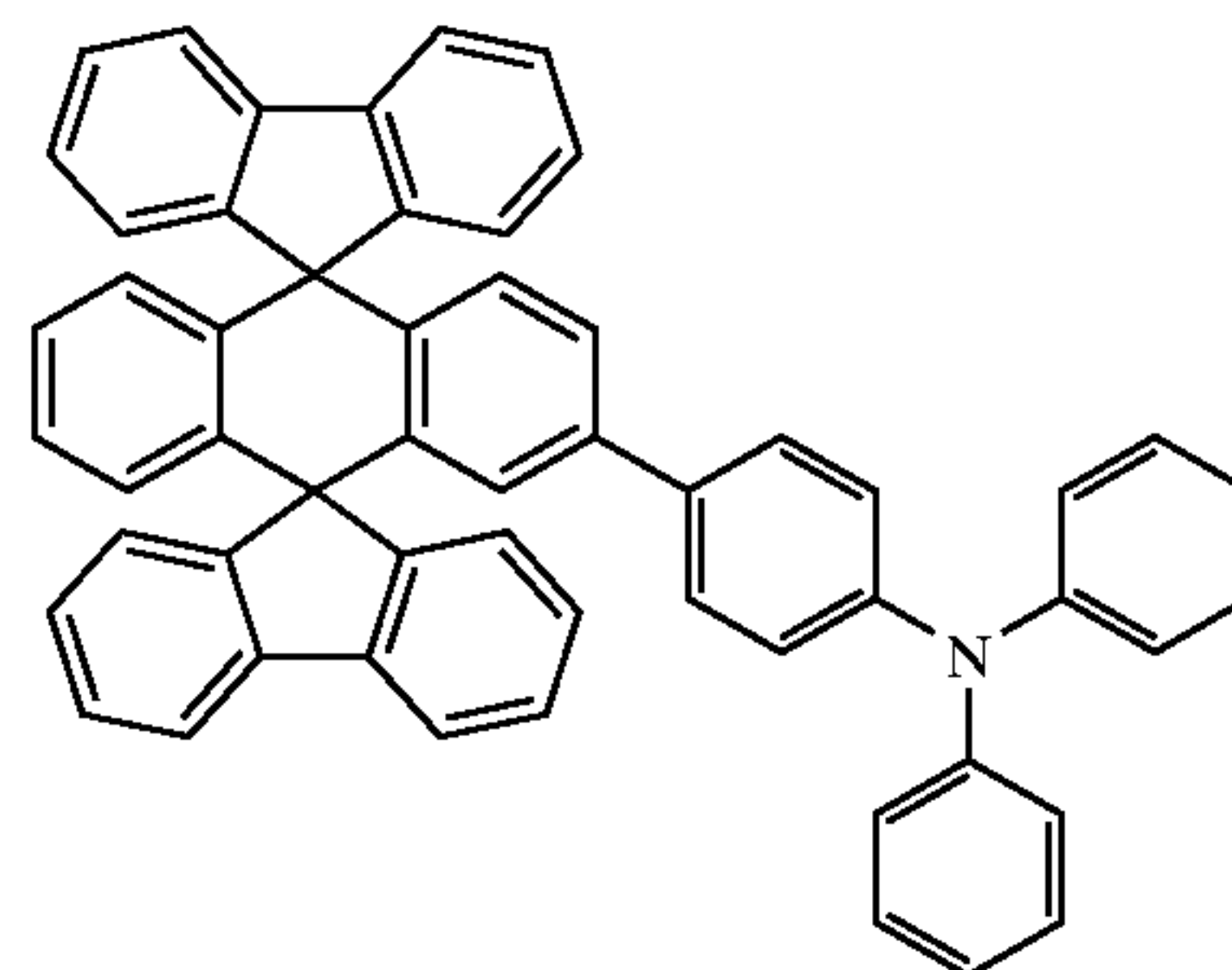
Chemical Compound 303
