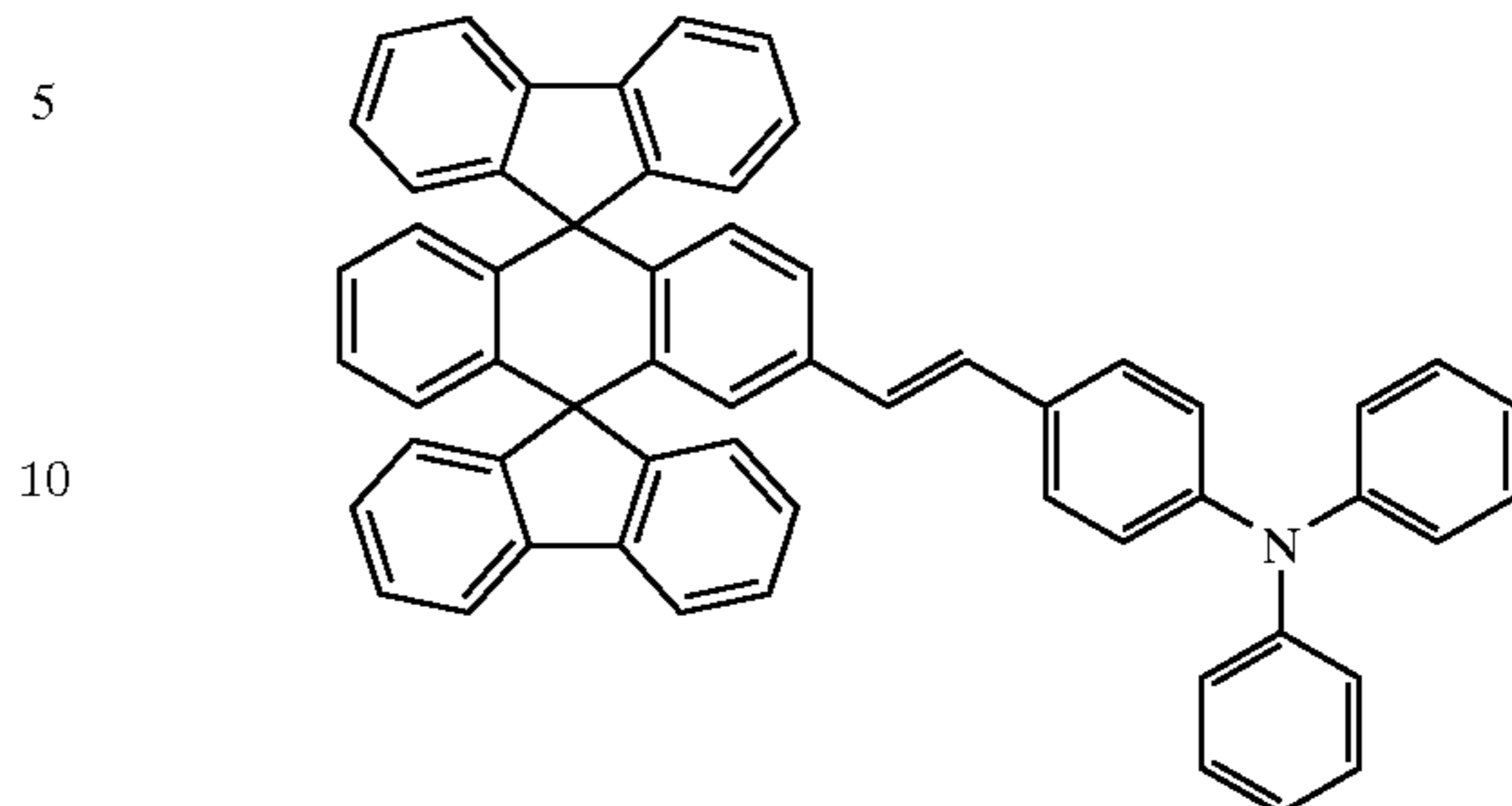
Chemical Compound 400
