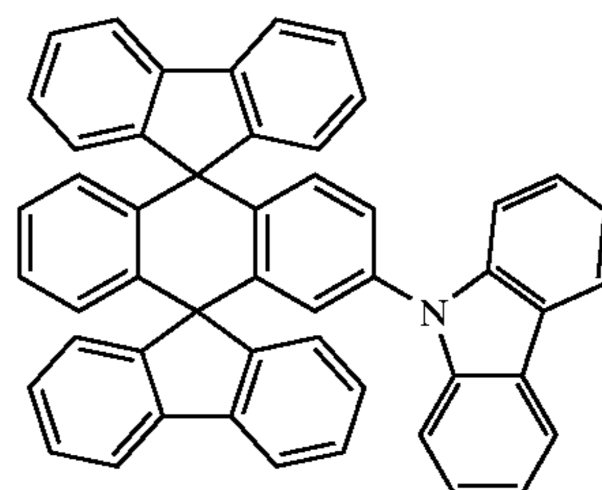
Chemical Compound 404
