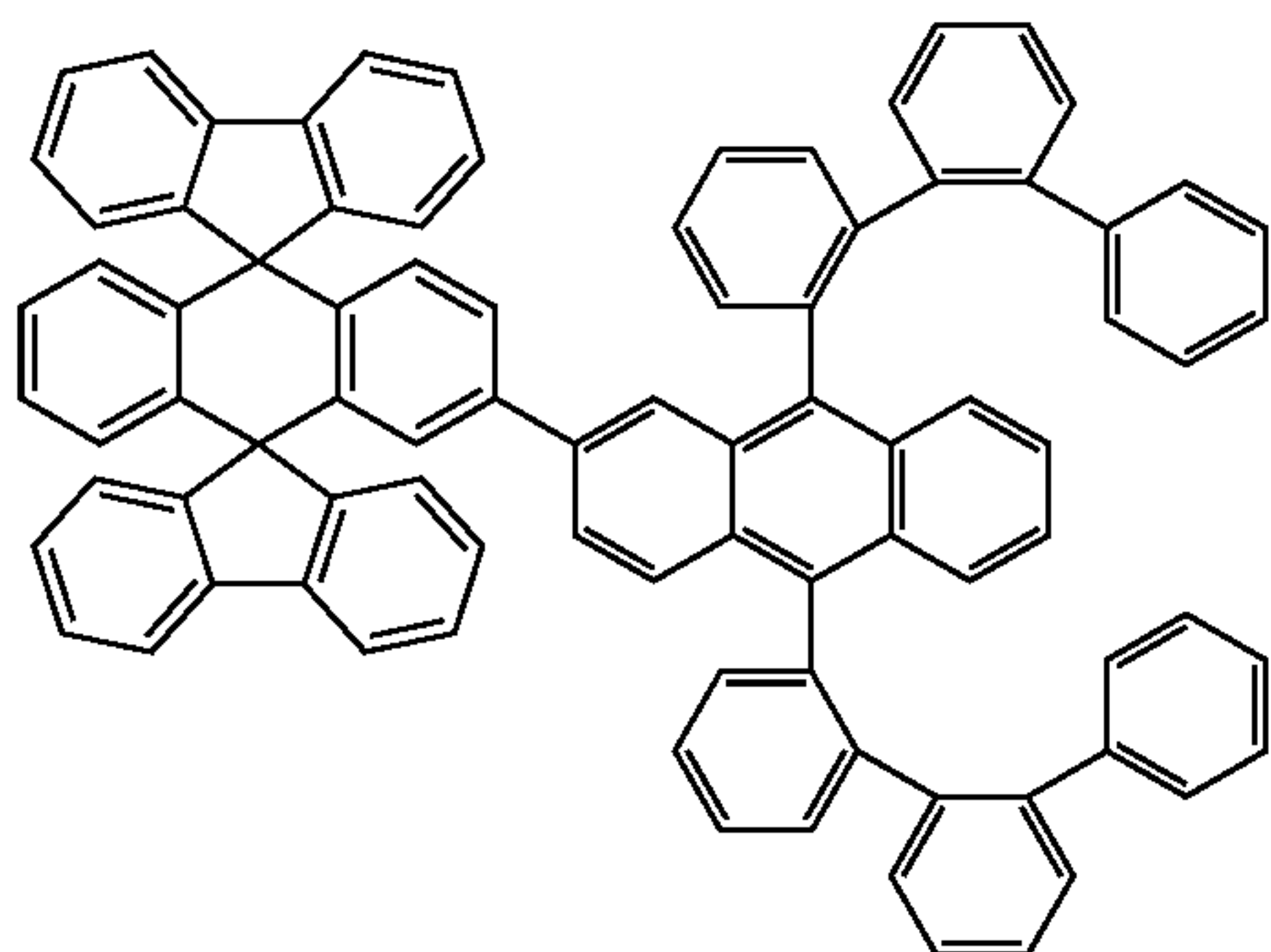
Chemical Compound 136
