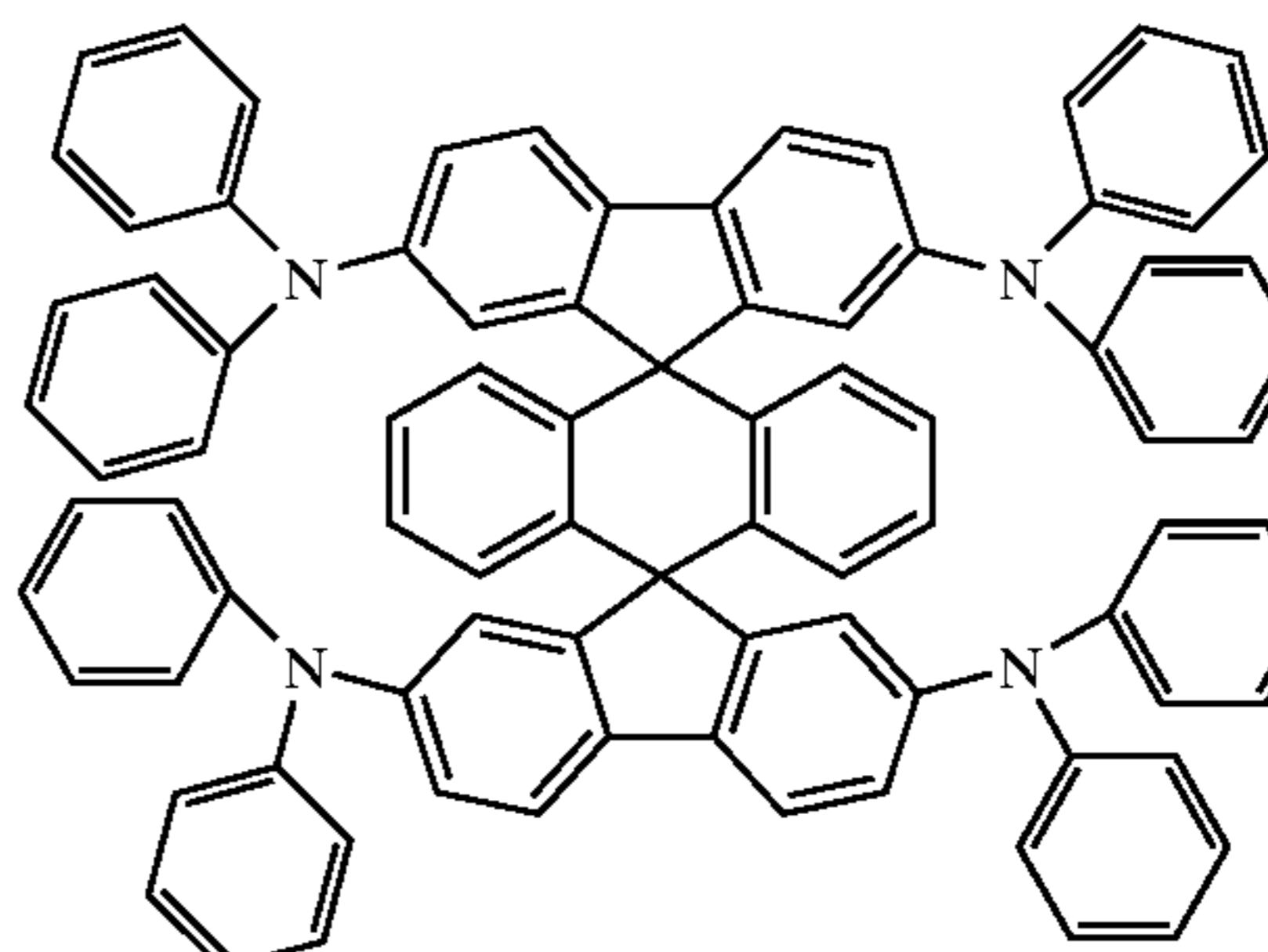
Chemical Compound 304
