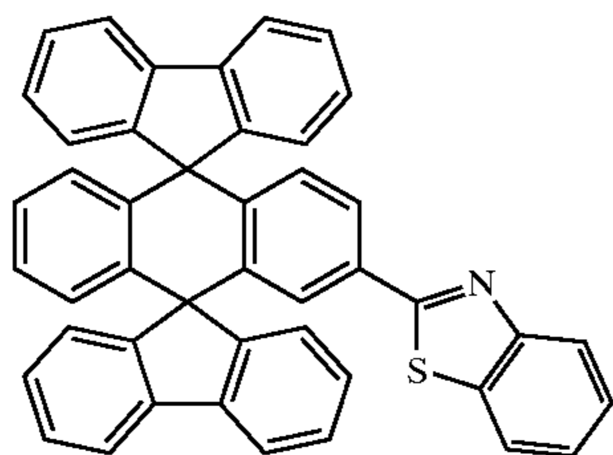
Chemical Compound 215
