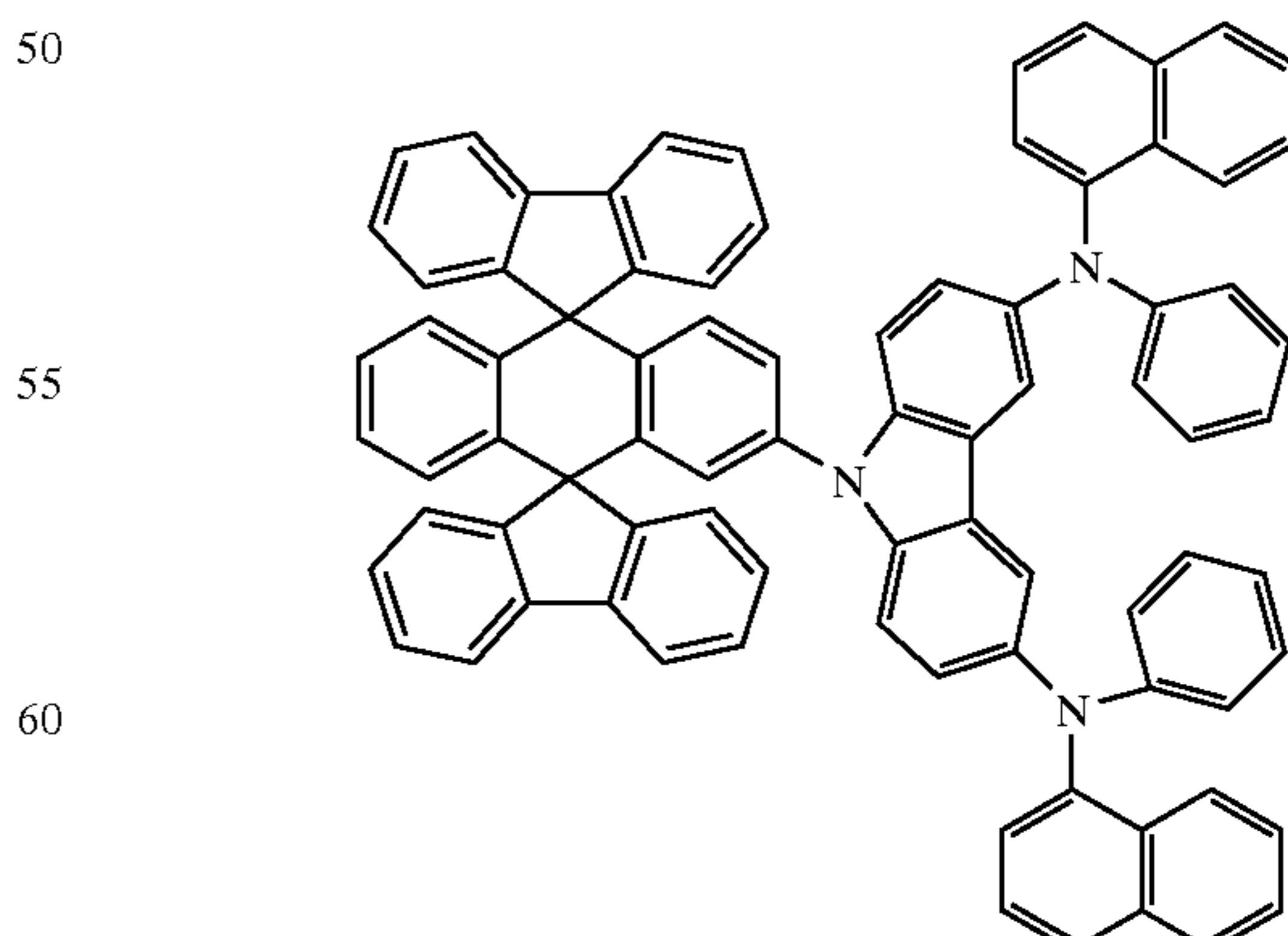
Chemical Compound 403
