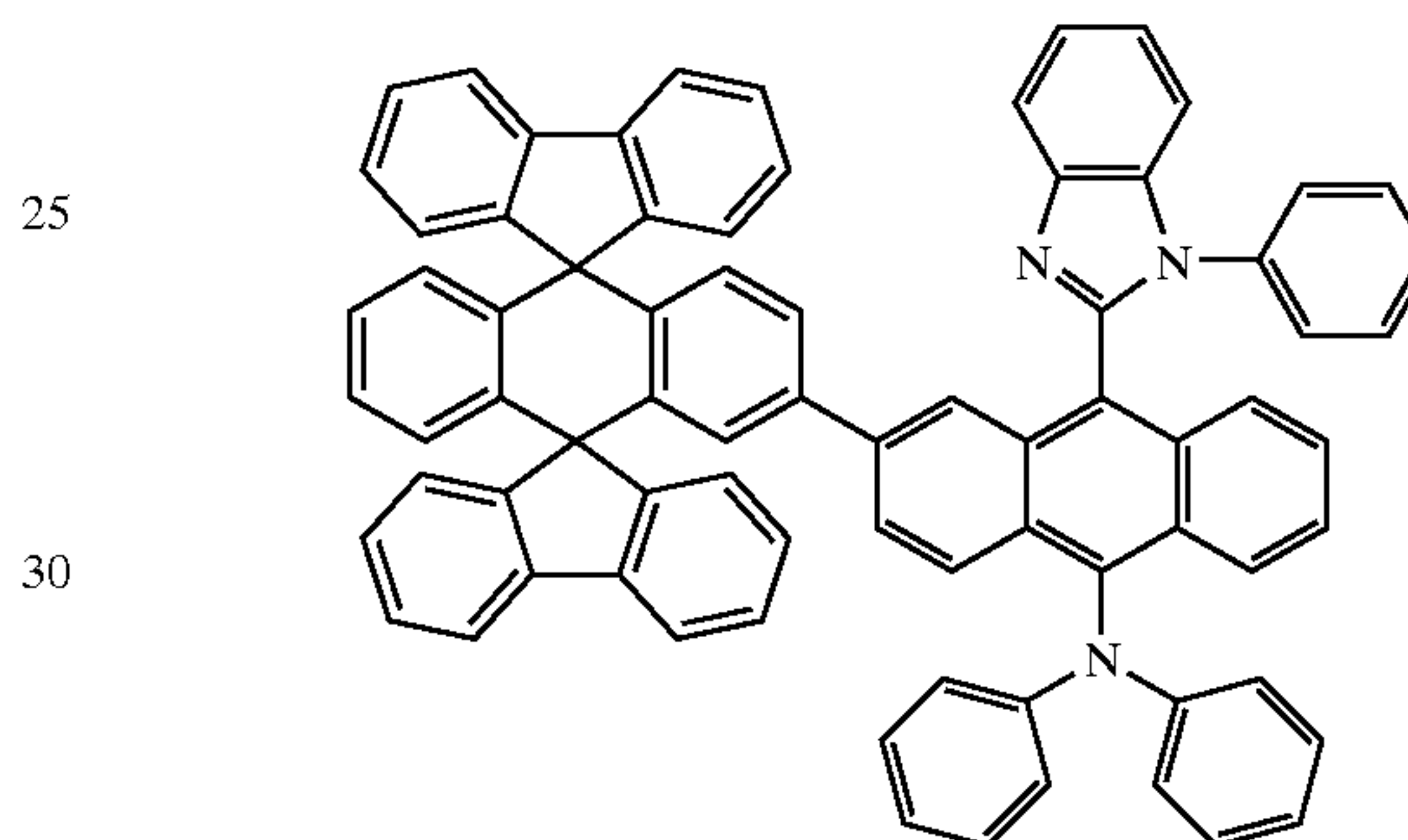
Chemical Compound 127
