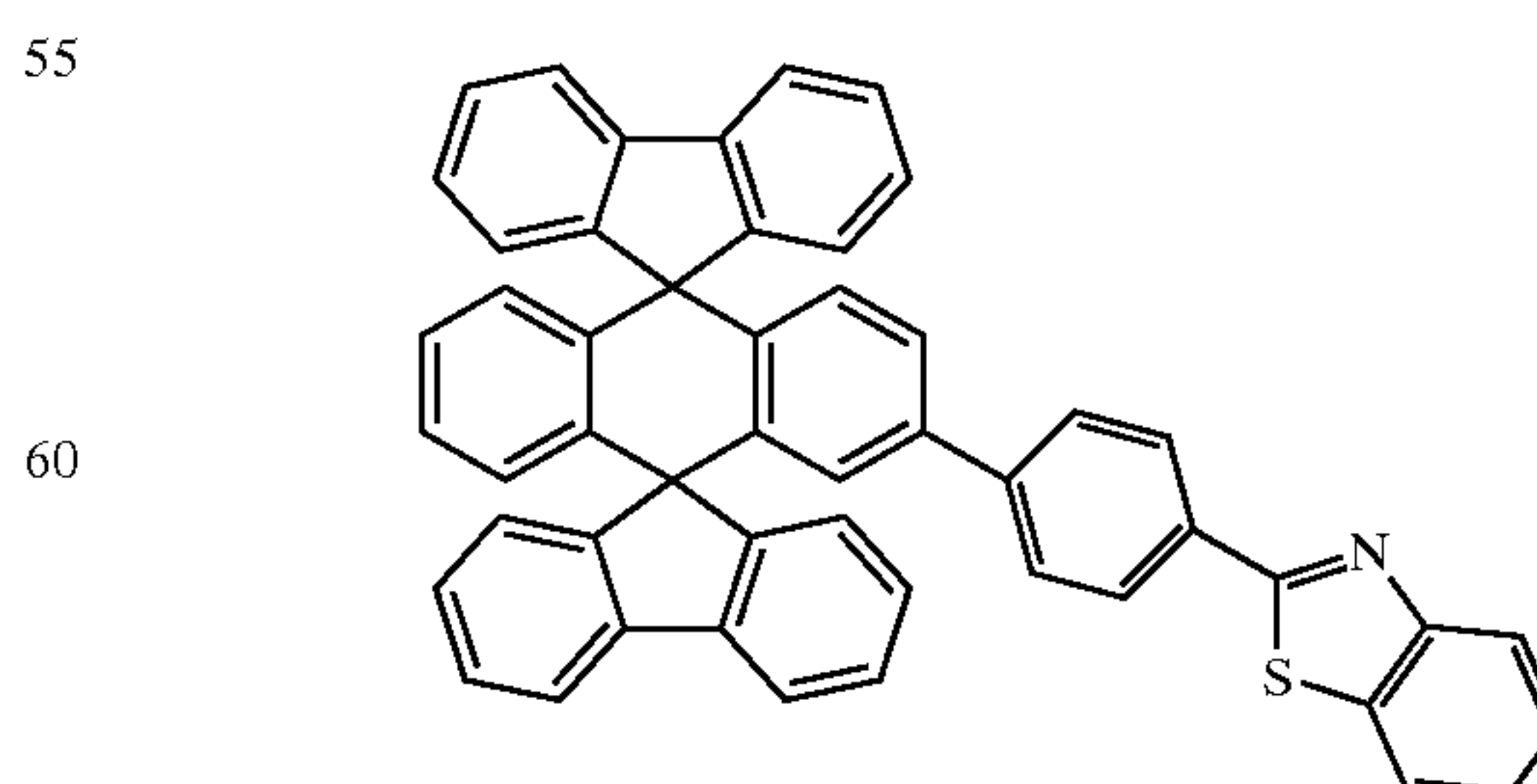
Chemical Compound 213
