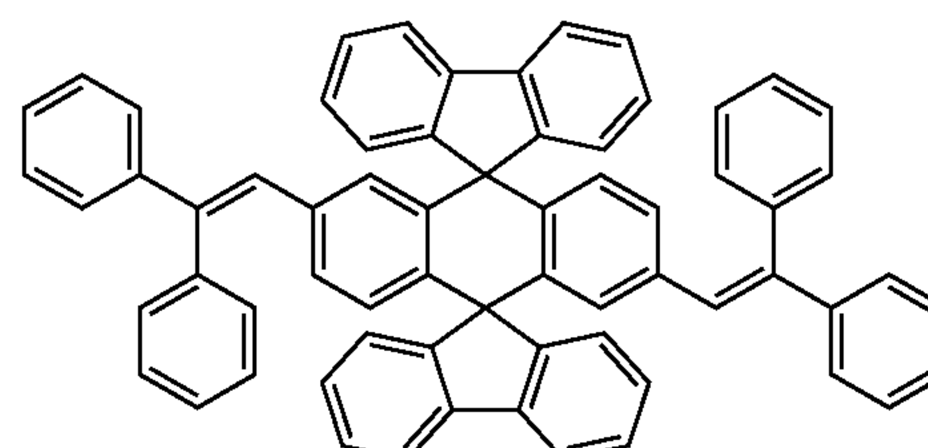
Chemical Compound 105
