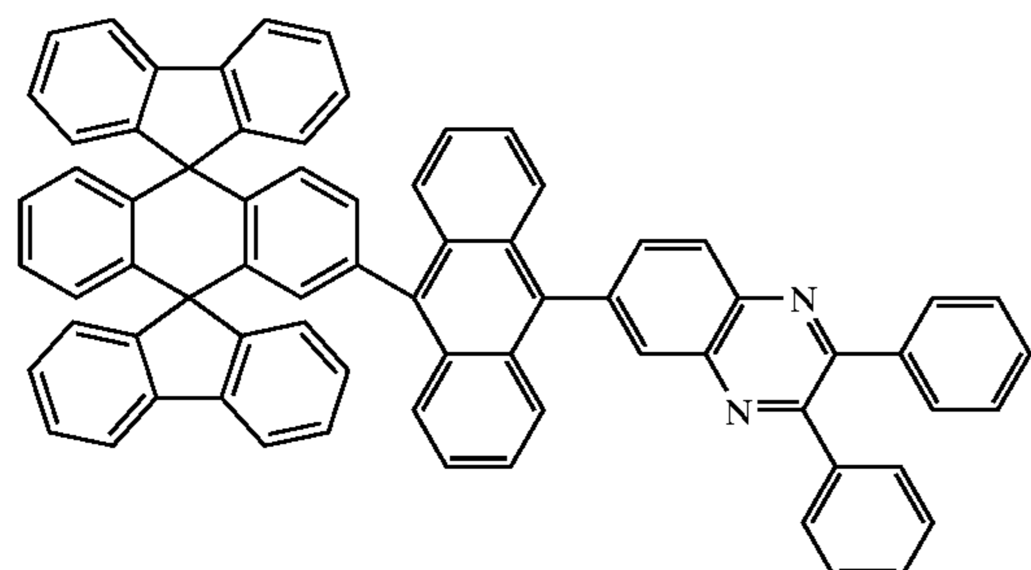
Chemical Compound 203
