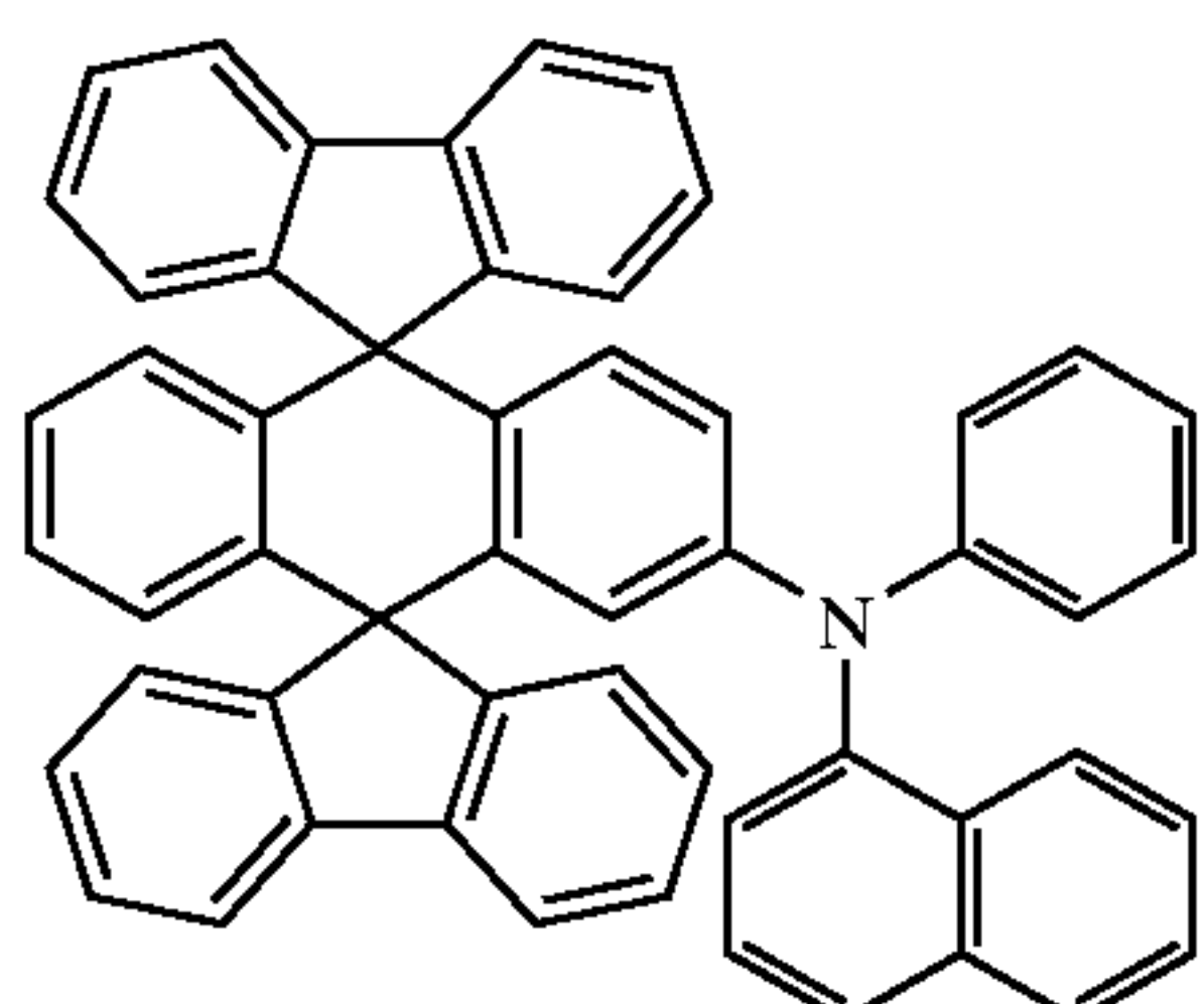
Chemical Compound 301
