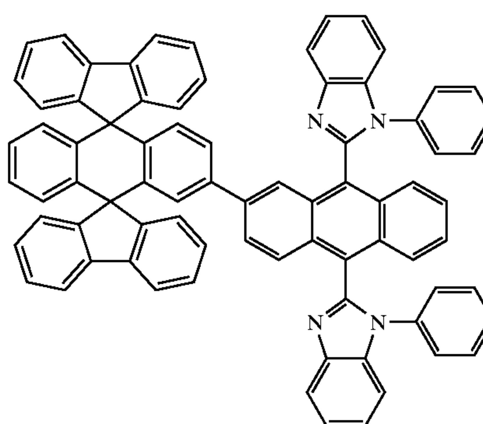
Chemical Compound 202
