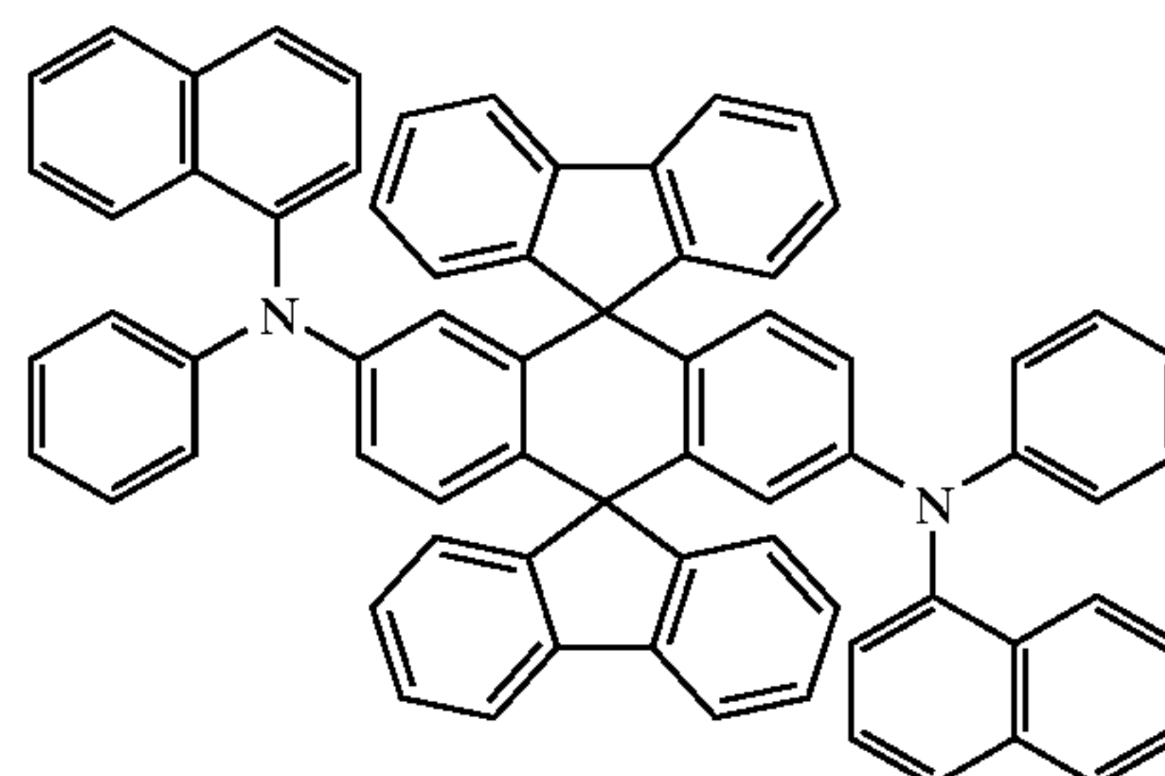
Chemical Compound 302
