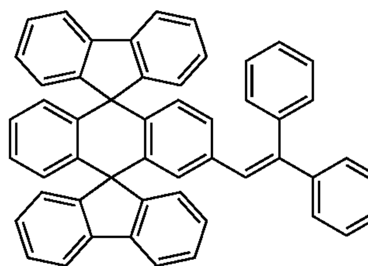
Chemical Compound 106
