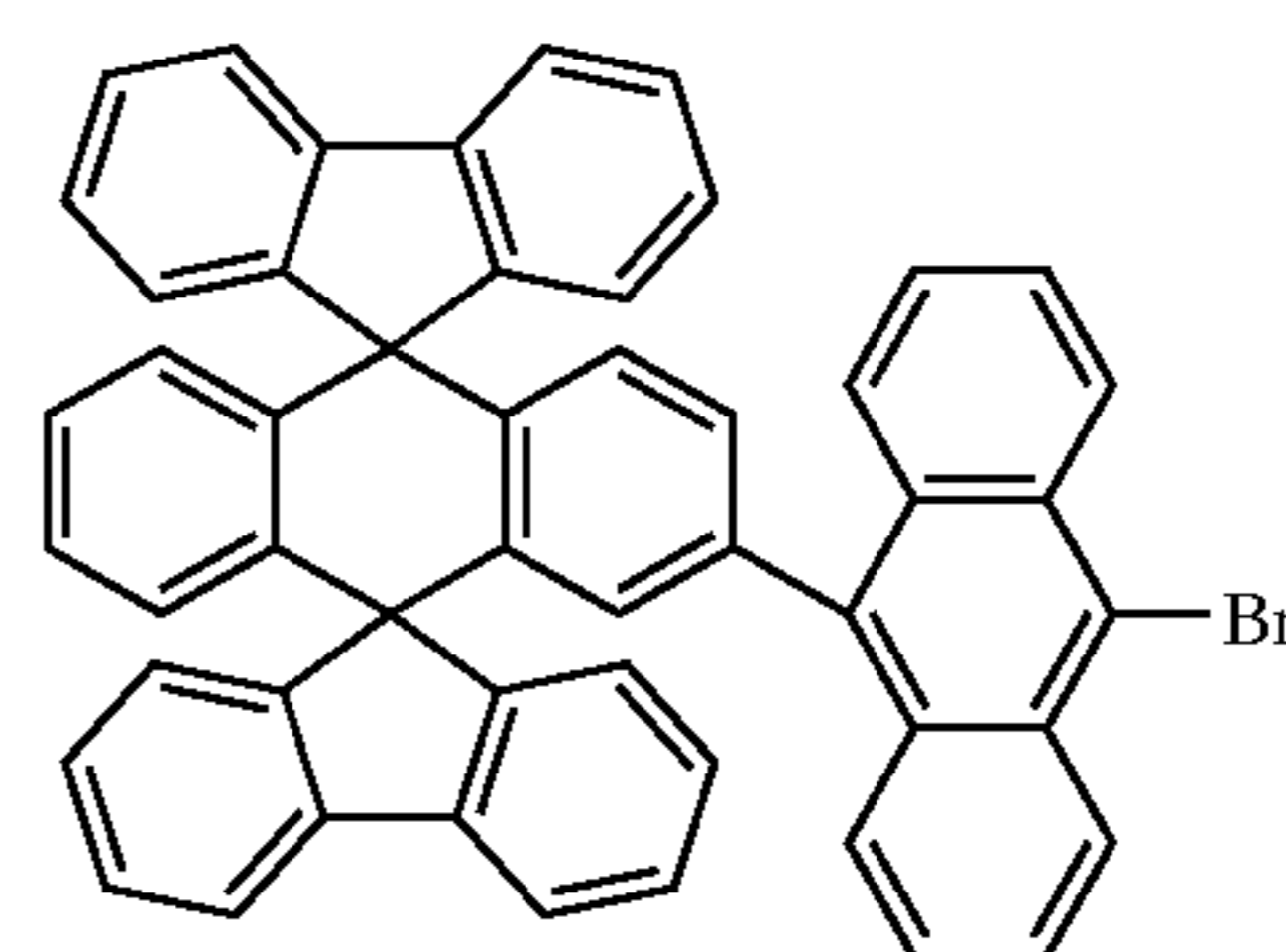
Chemical Compound 5
