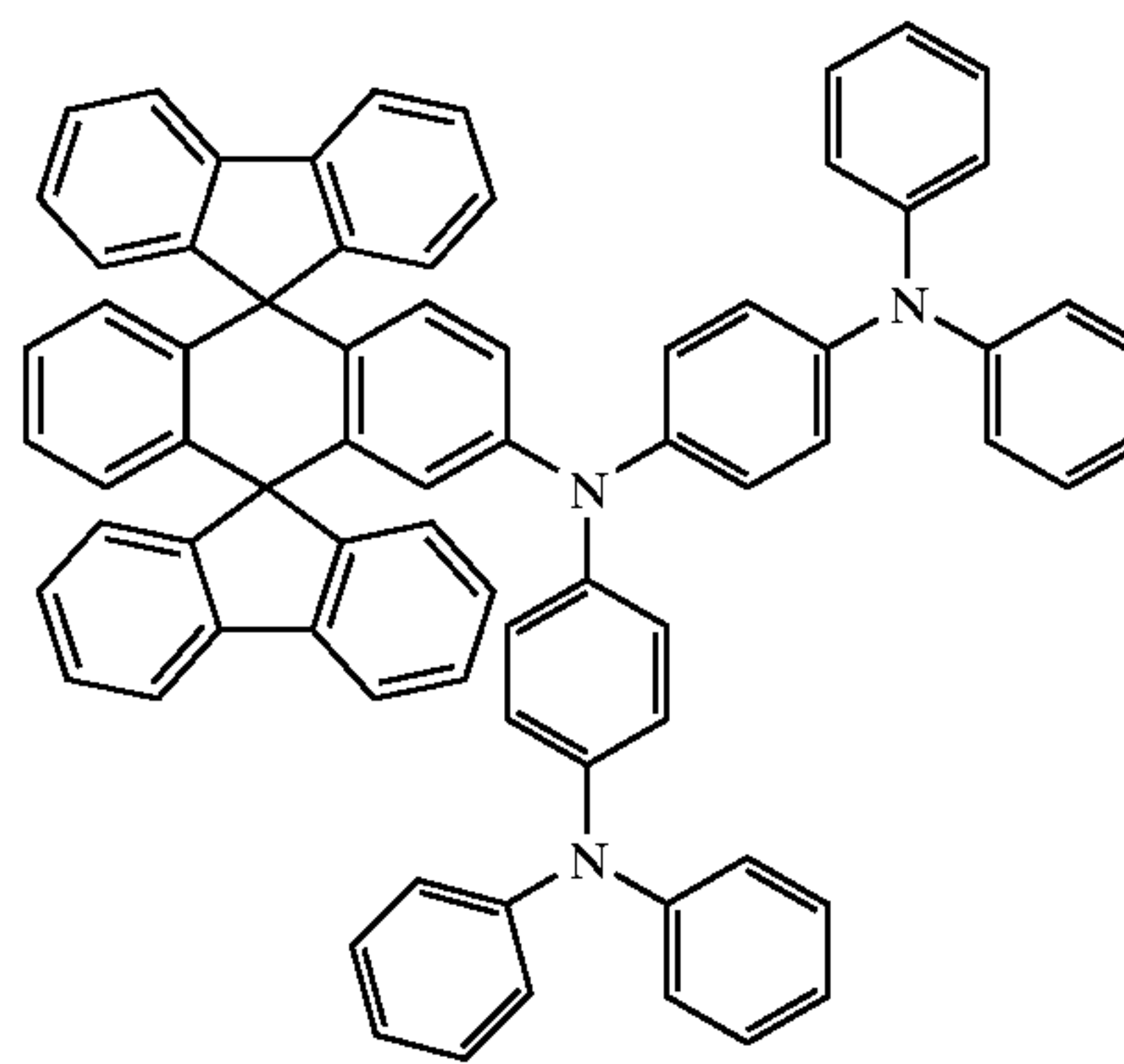
Chemical Compound 308
