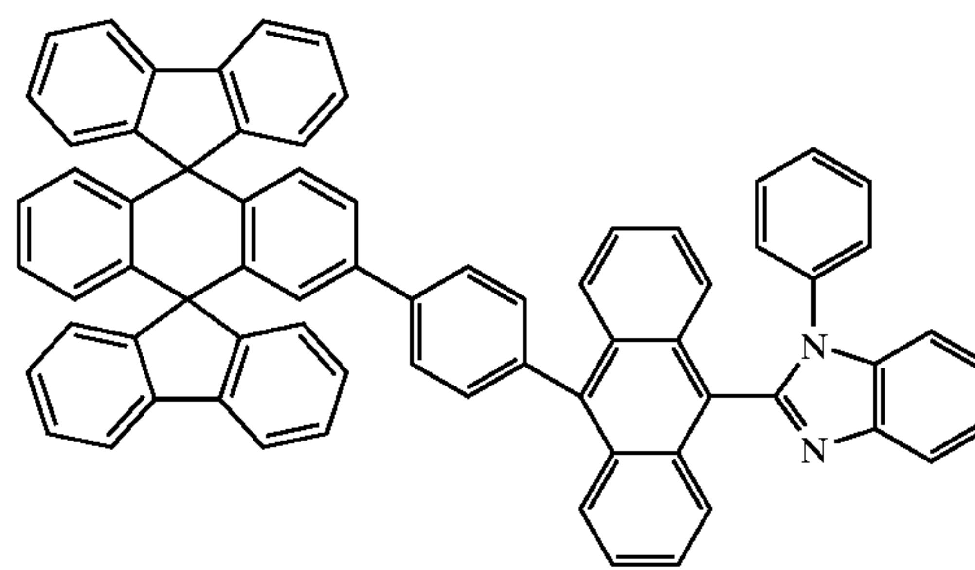
Chemical Compound 207
