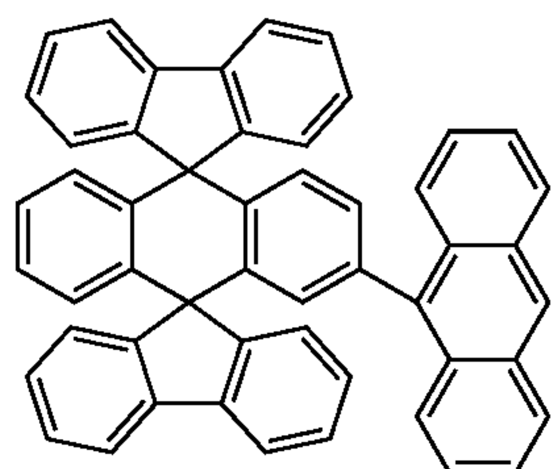
Chemical Compound 9
