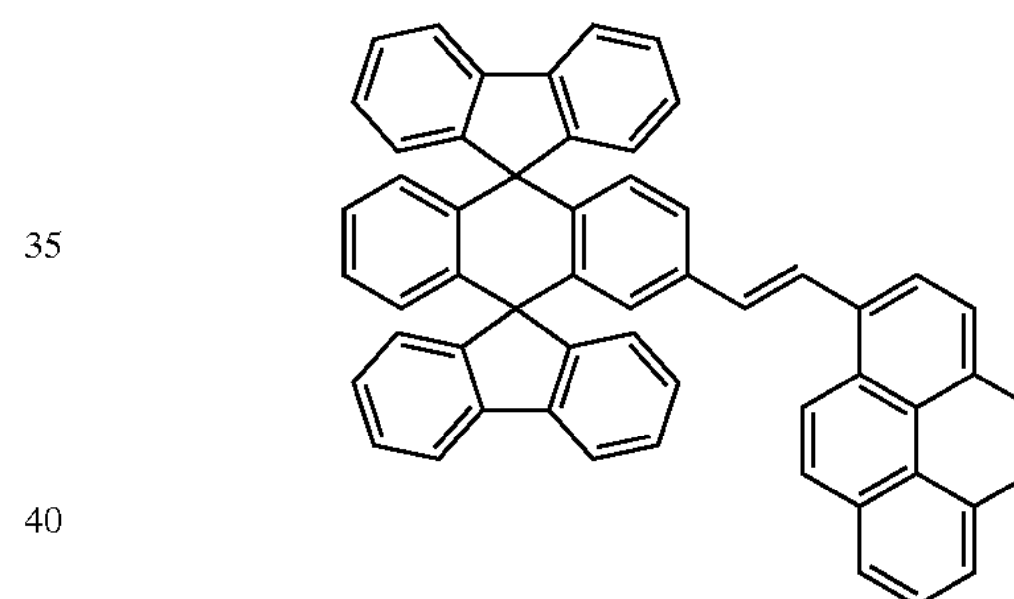
Chemical Compound 103
