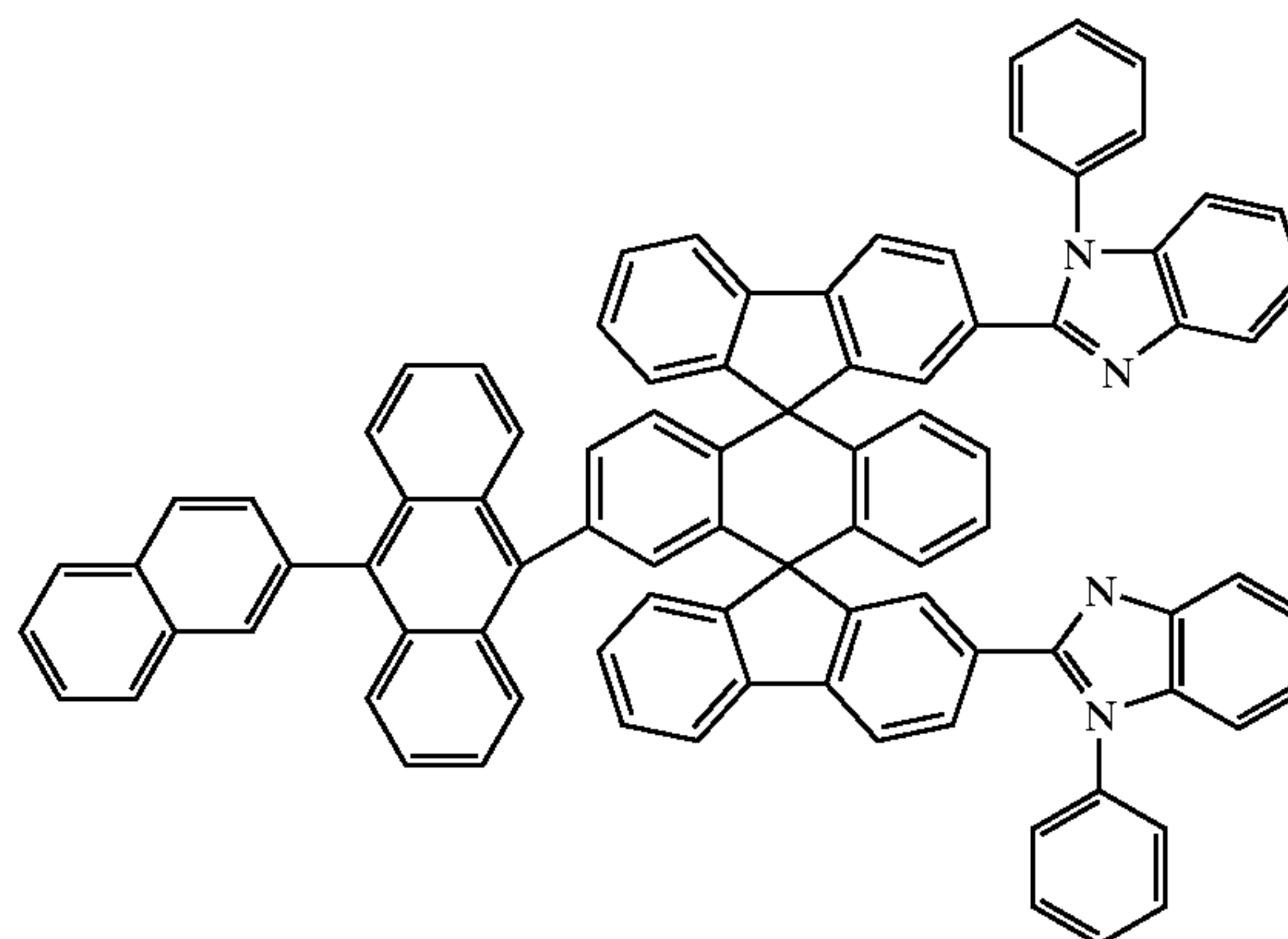
Chemical Compound 222
