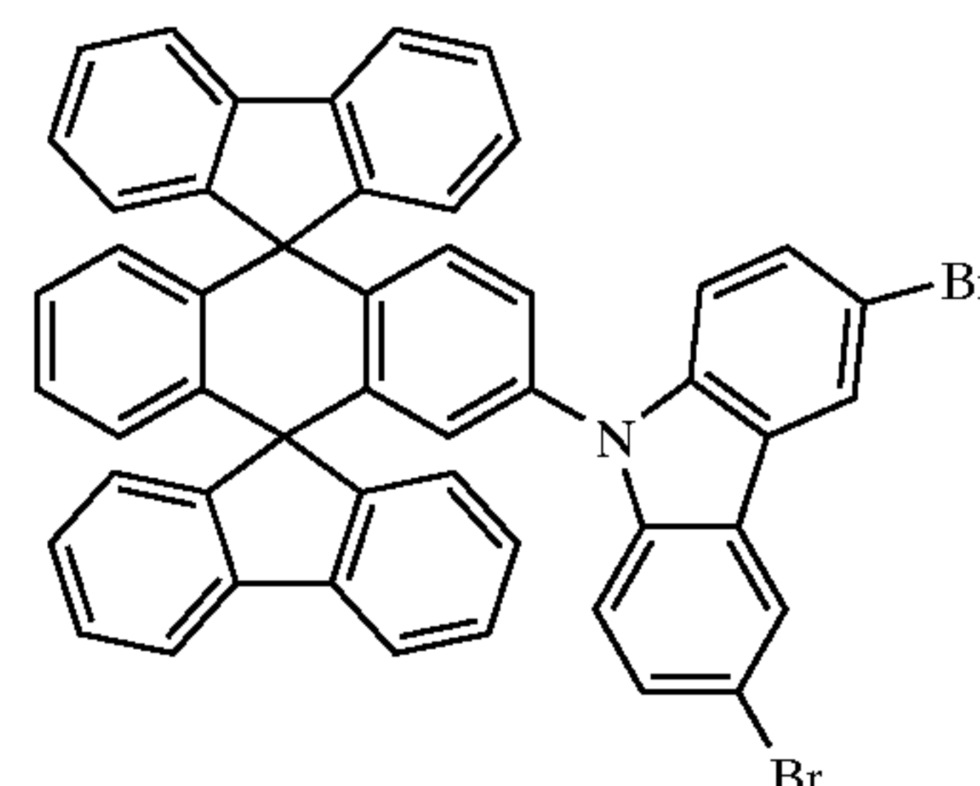
Chemical Compound 6
