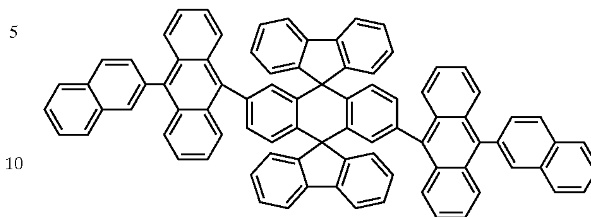
Chemical Compound 115
