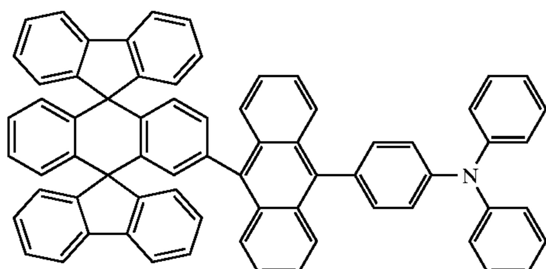
Chemical Compound 401
