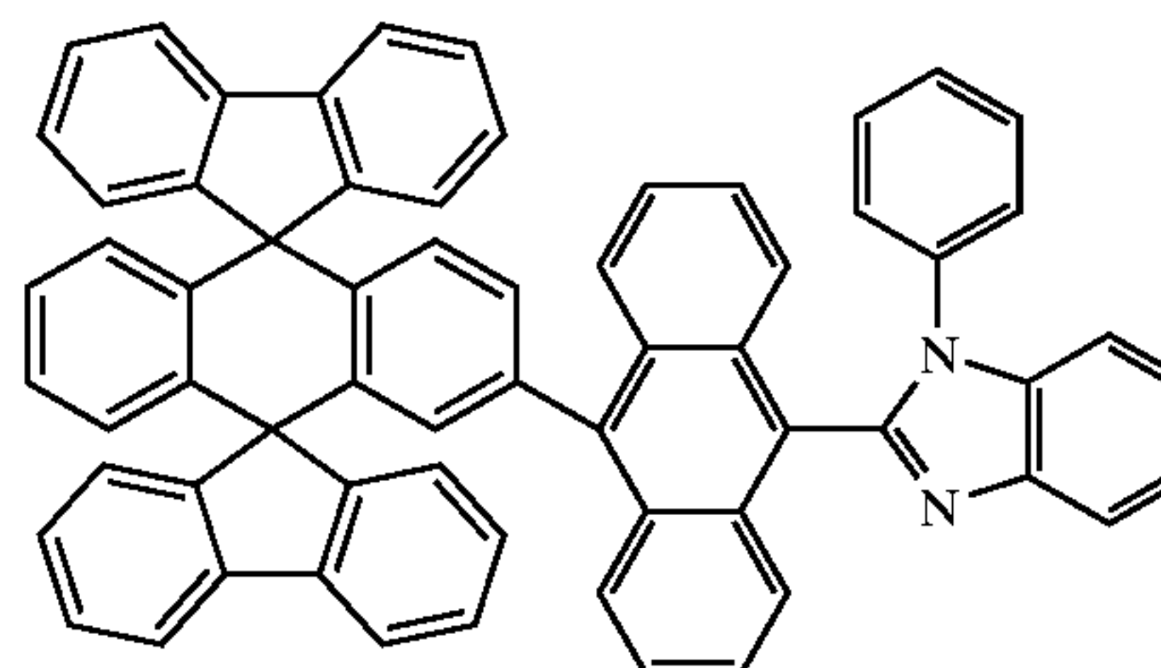
Chemical Compound 200
