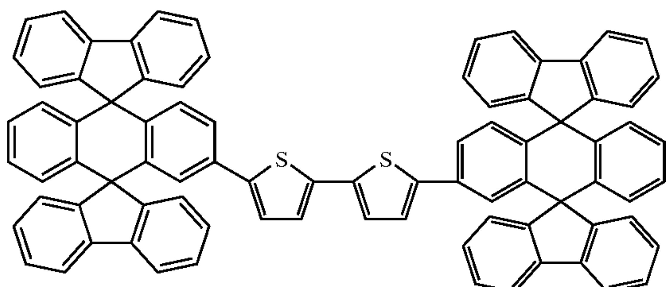
Chemical Compound 135
