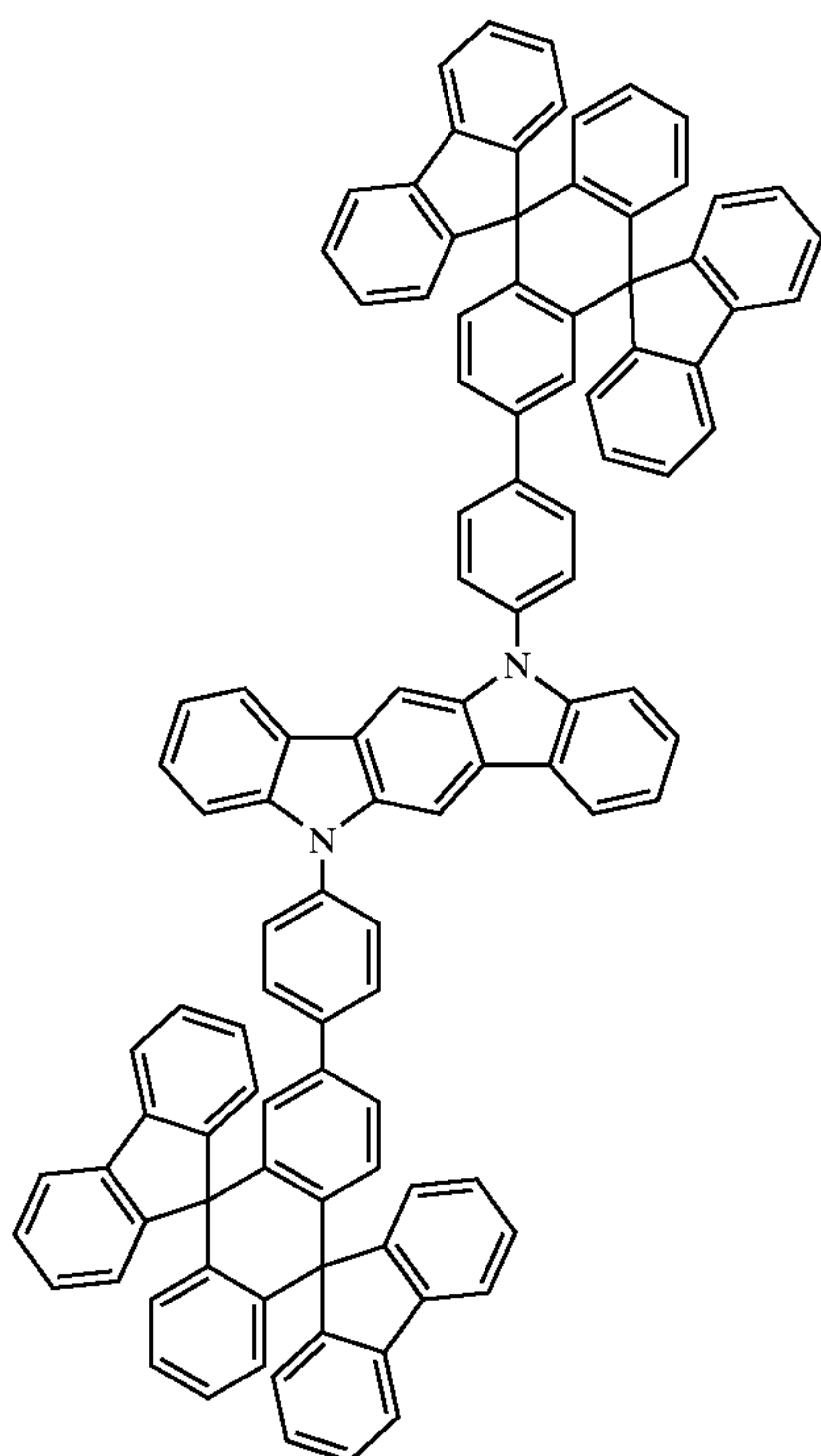
Chemical Compound 409
