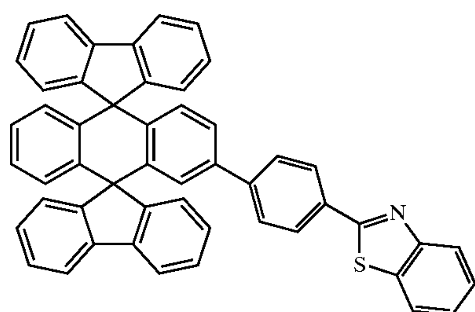
Chemical Compound 213
