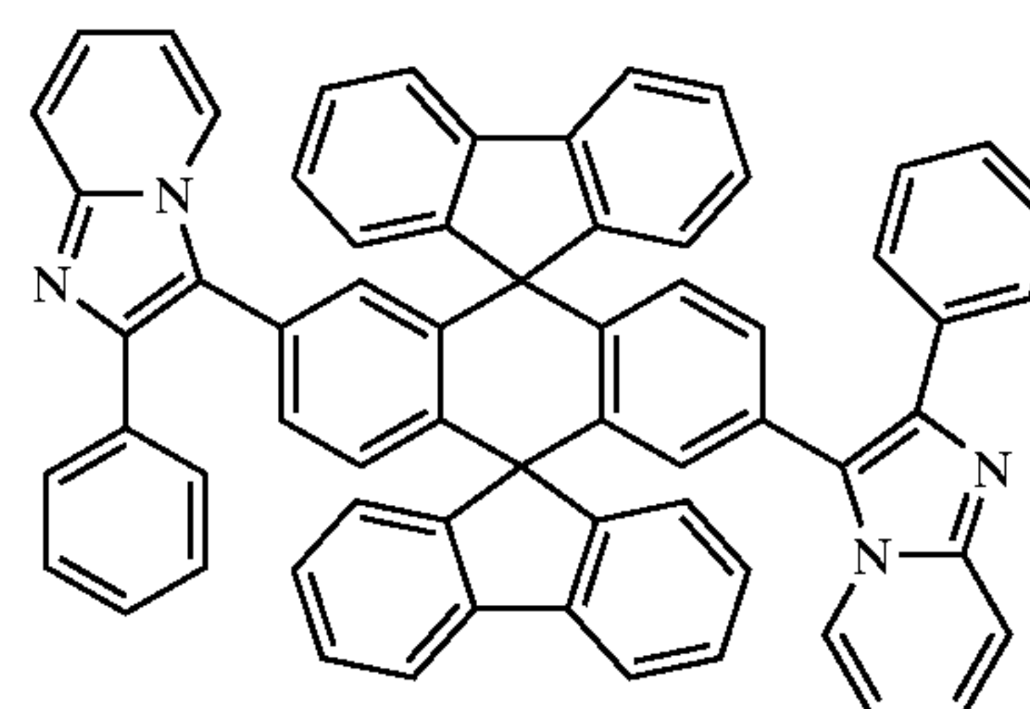
Chemical Compound 413.
