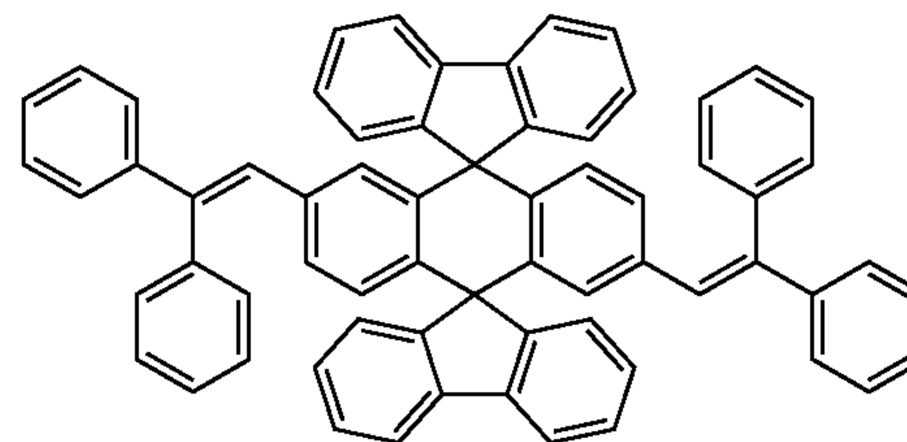
Chemical Compound 105
