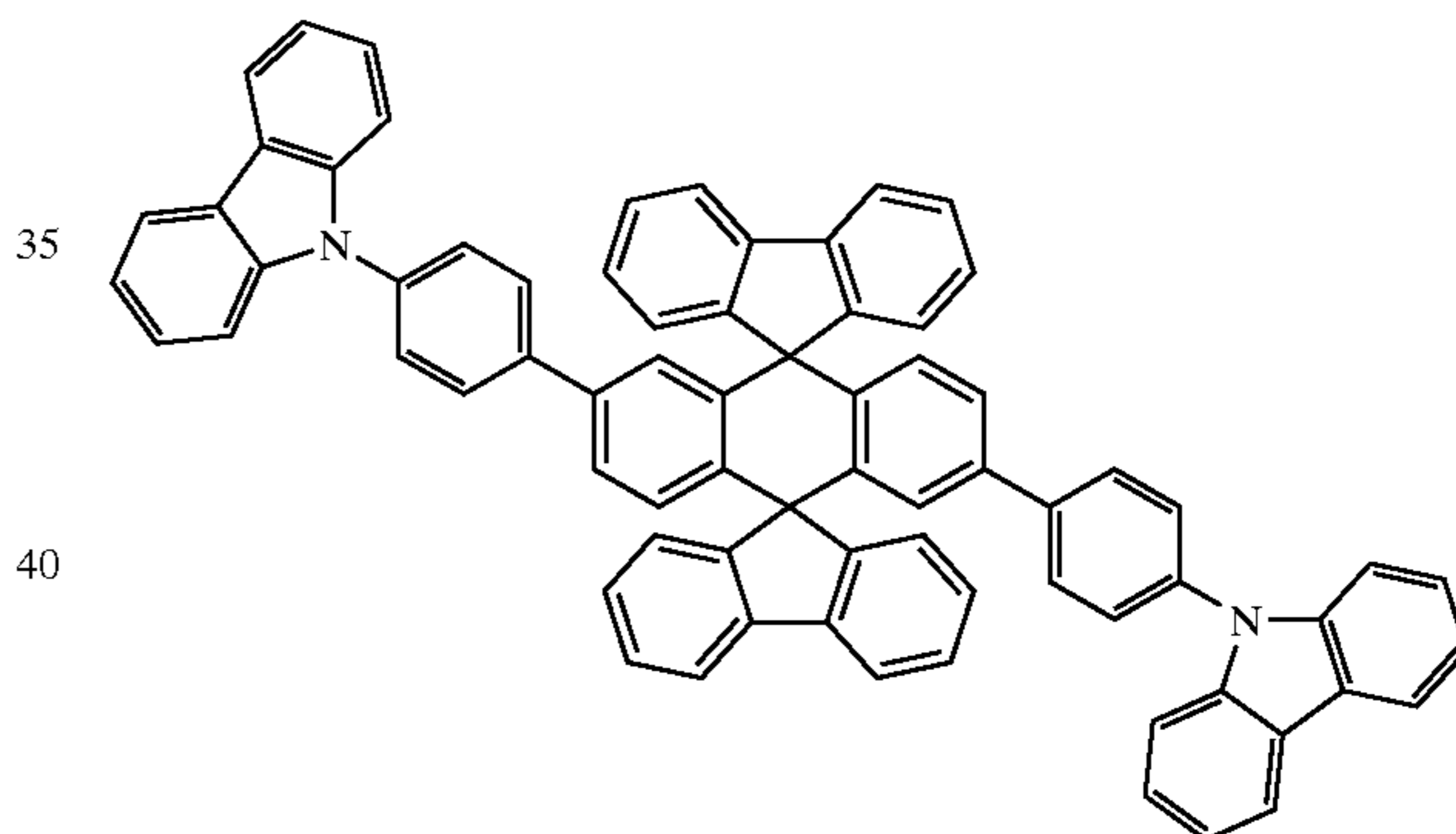
Chemical Compound 402
