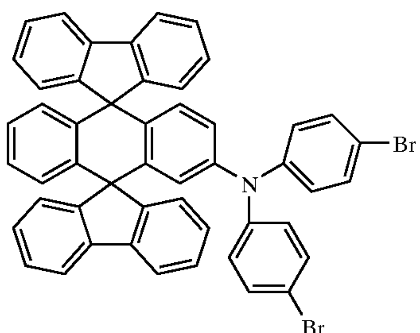
Chemical Compound 7
