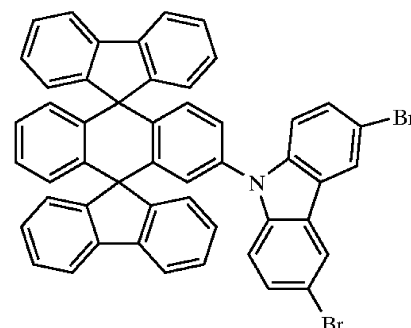
Chemical Compound 6
