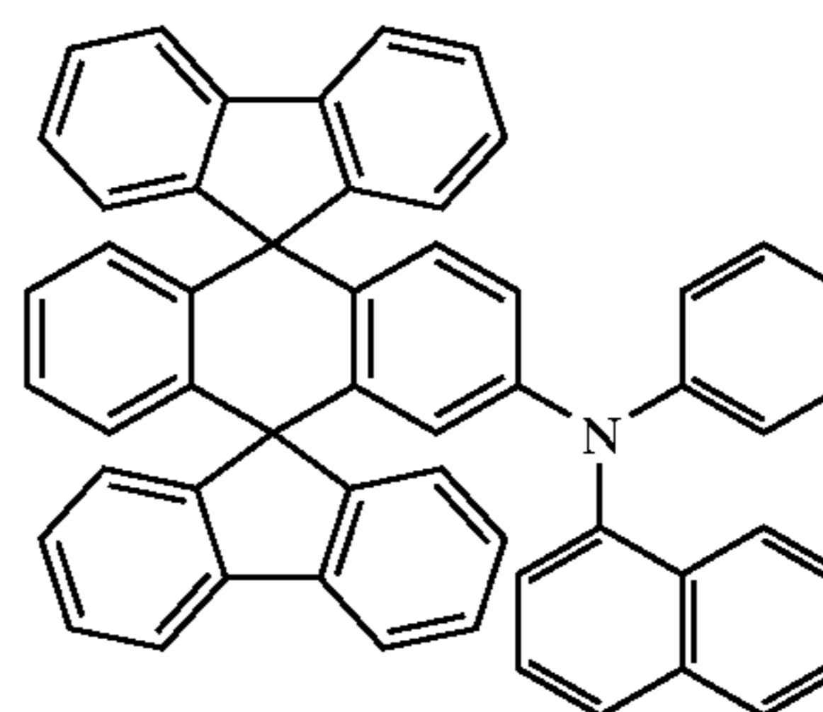
Chemical Compound 301
