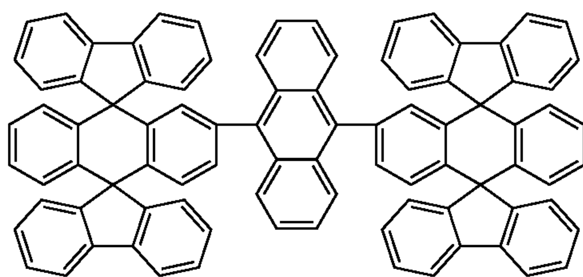
Chemical Compound 102
