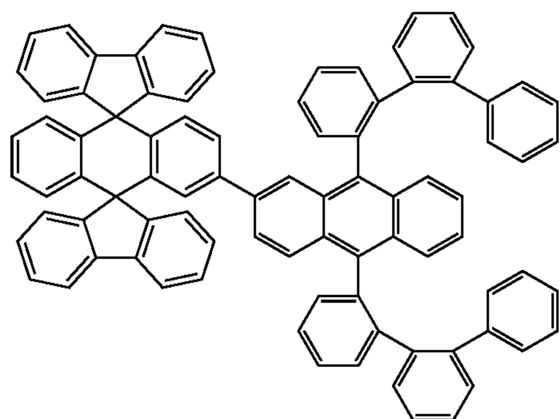
Chemical Compound 136
