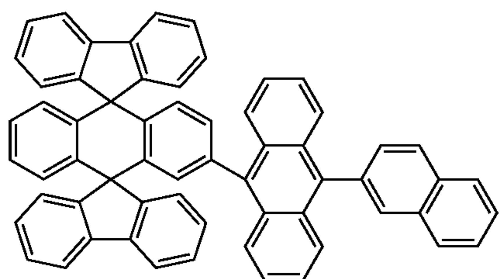
Chemical Compound 110
