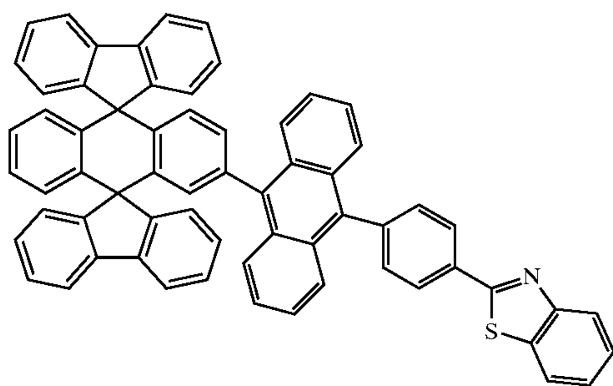
Chemical Compound 217
