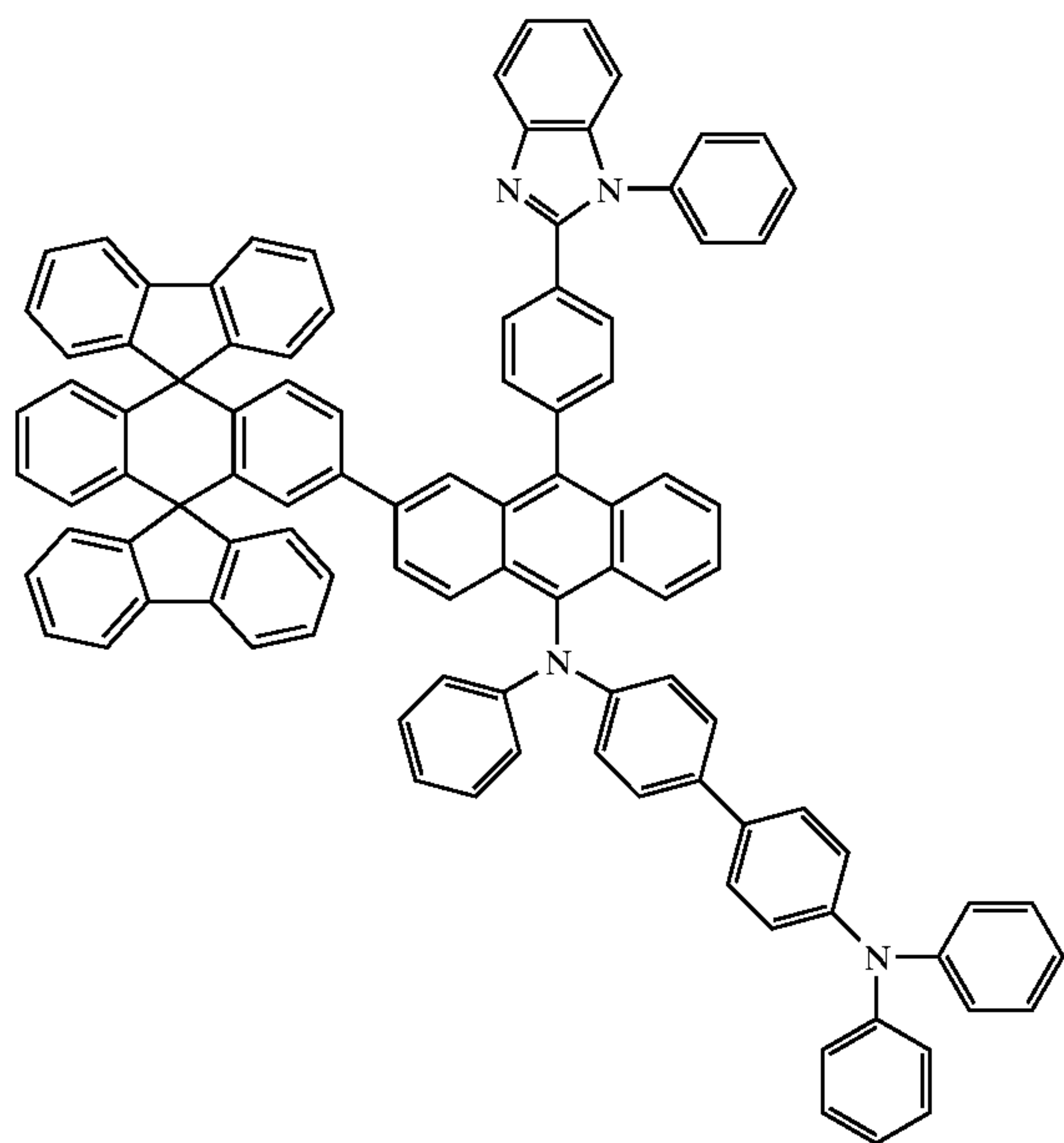
Chemical Compound 124
