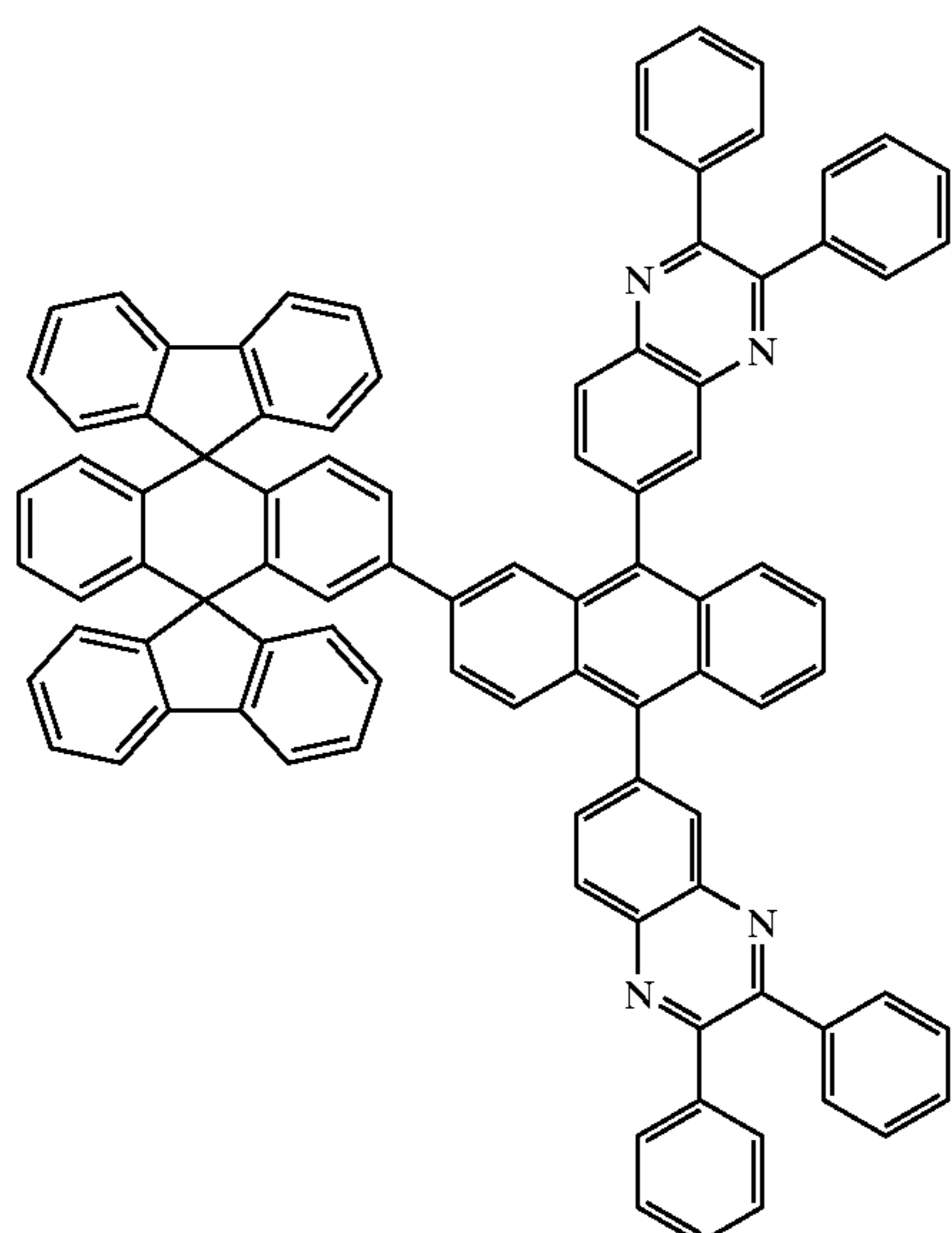
Chemical Compound 212
