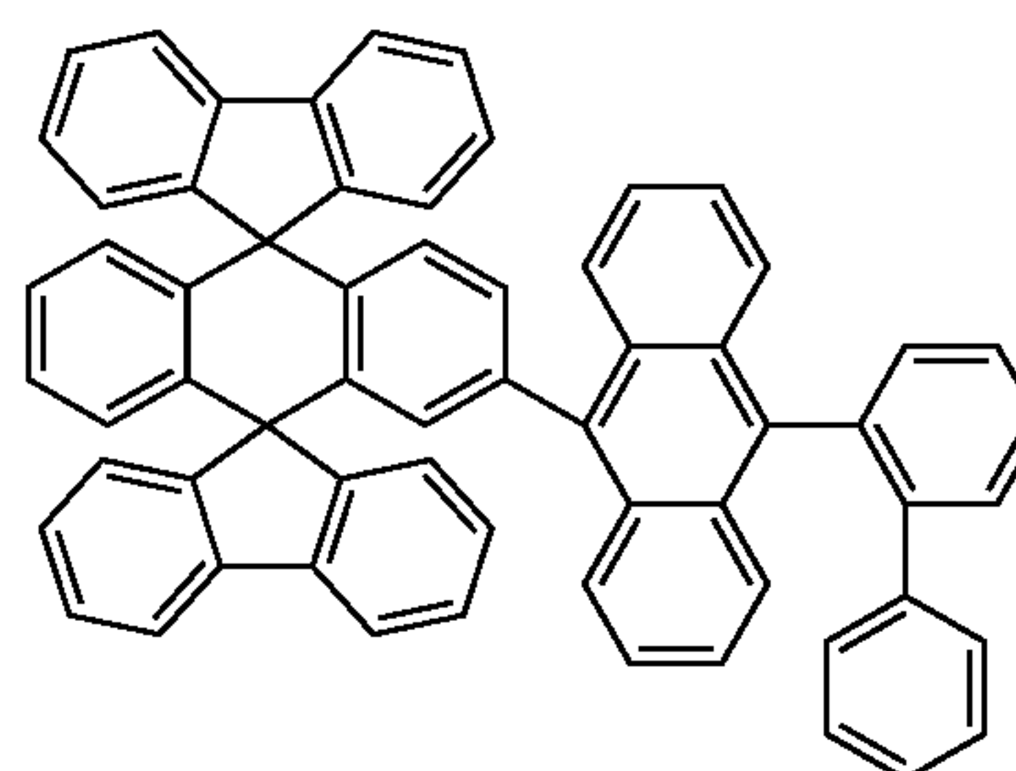
Chemical Compound 111
