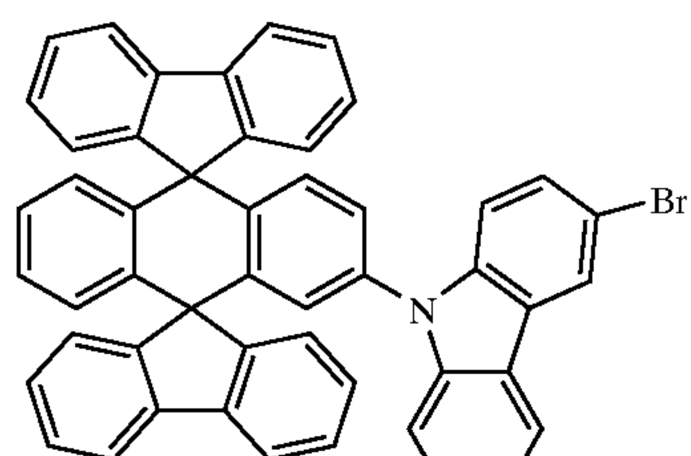
Chemical Compound 6
