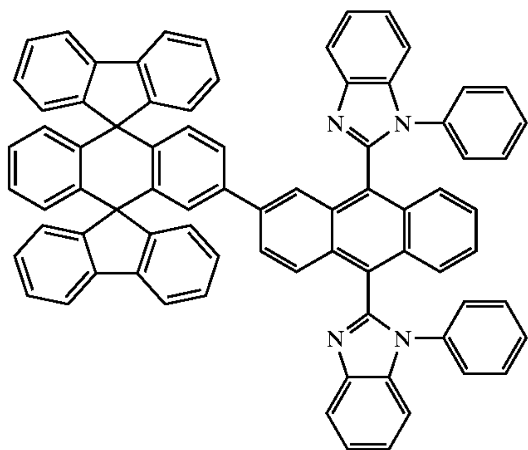
Chemical Compound 202
