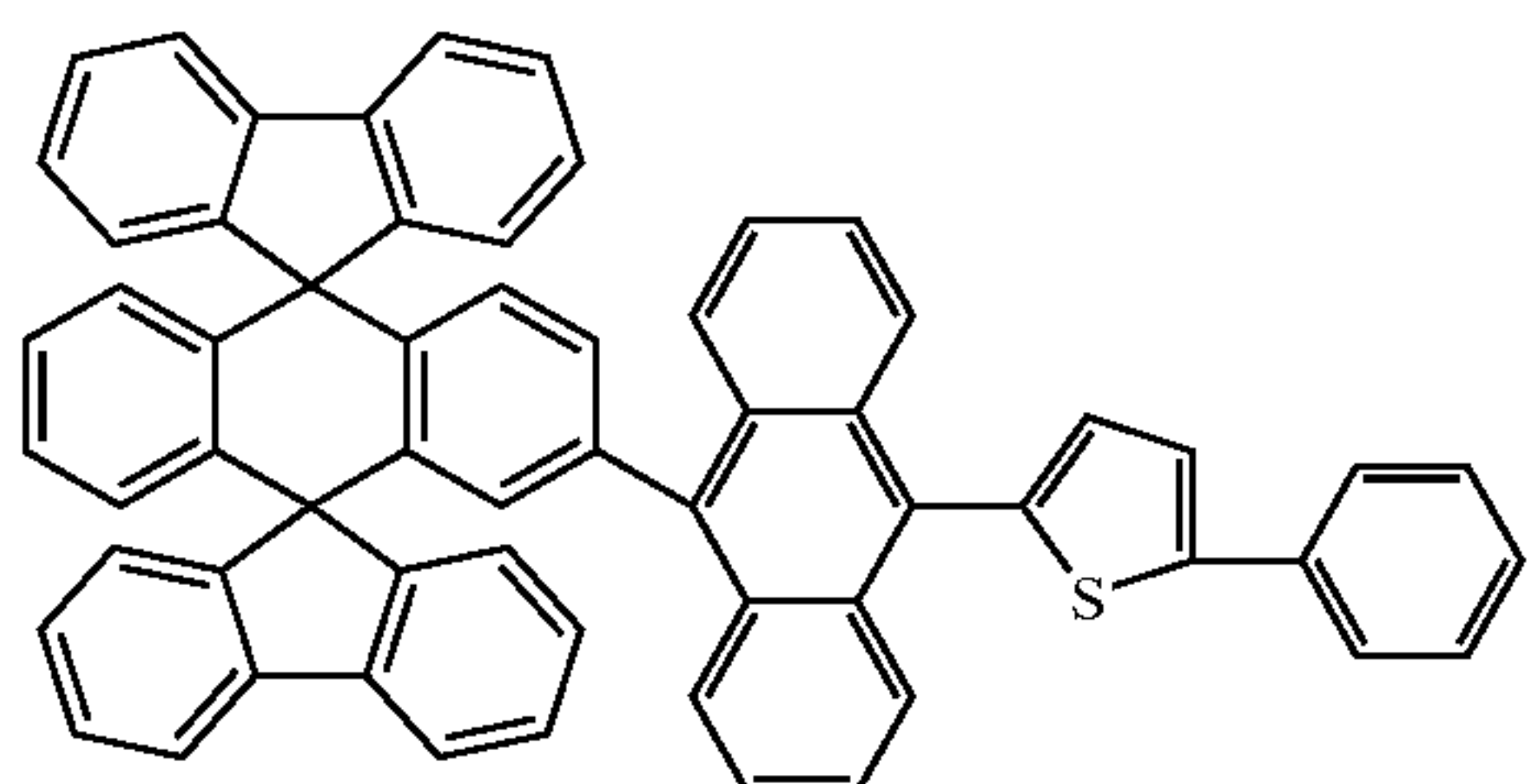
Chemical Compound 134
