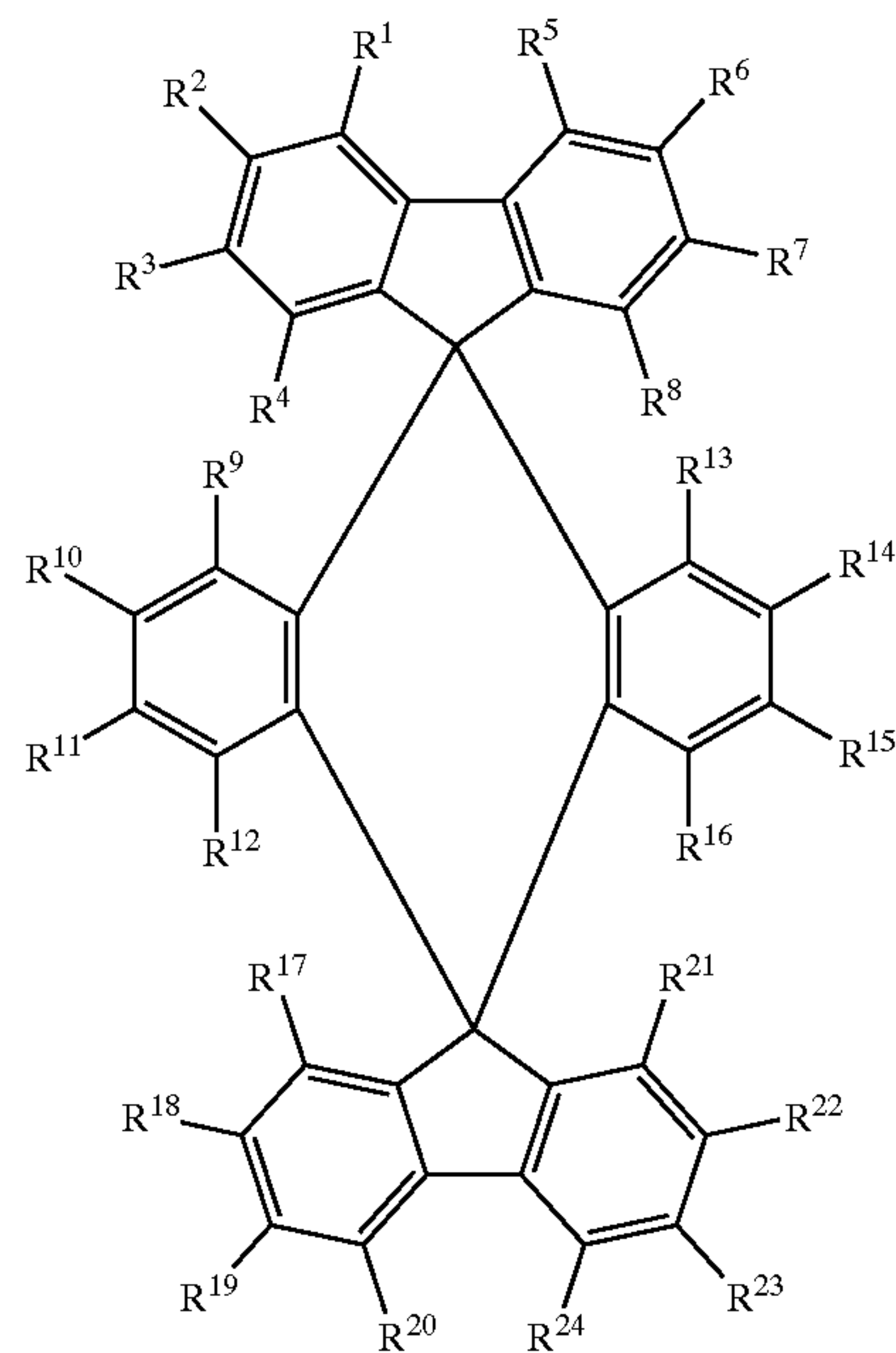
Chemical Formula 1
