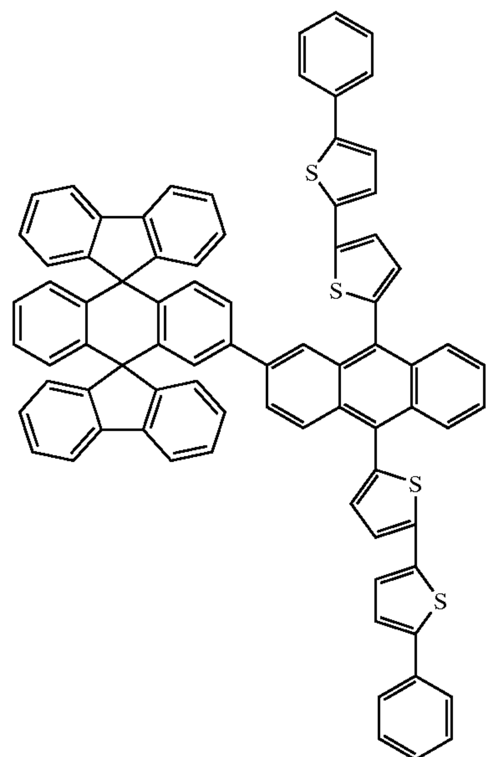
Chemical Compound 128
