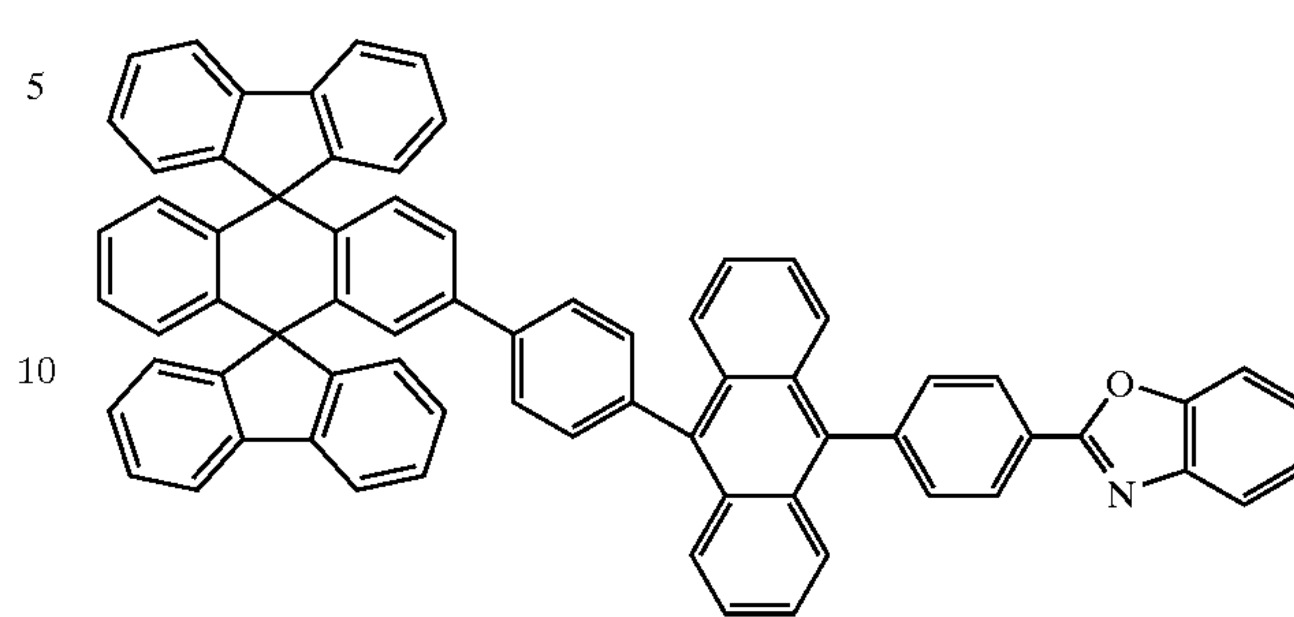
Chemical Compound 126
