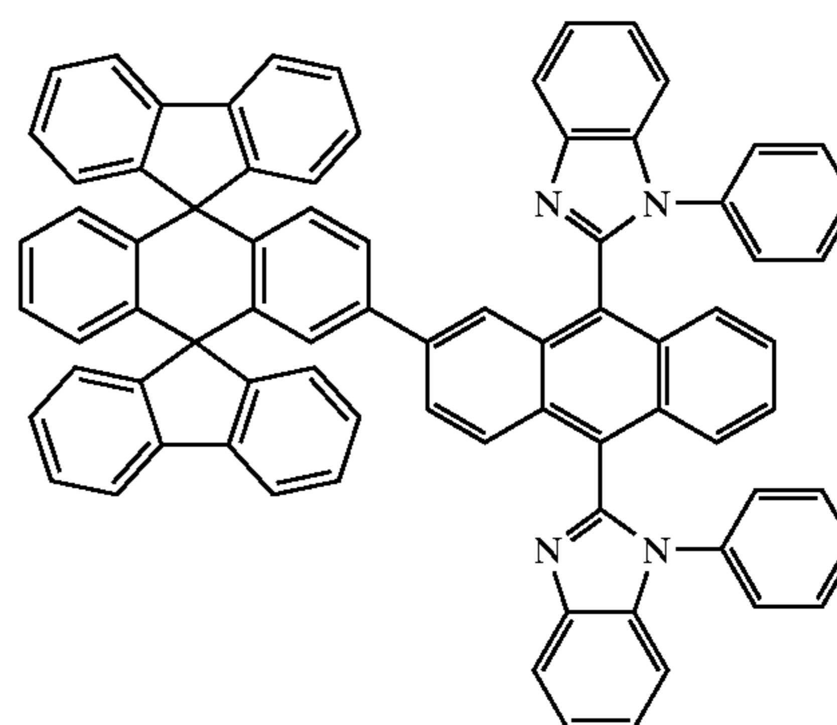
Chemical Compound 202
