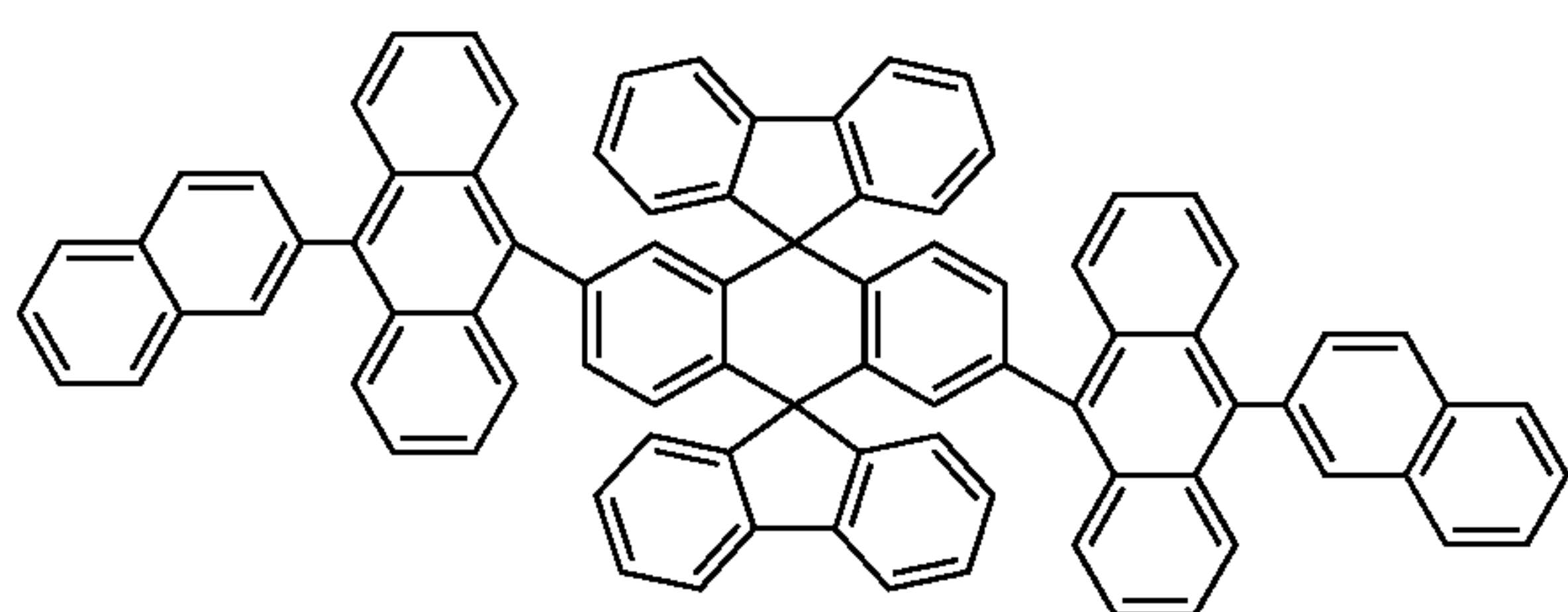
Chemical Compound 115
