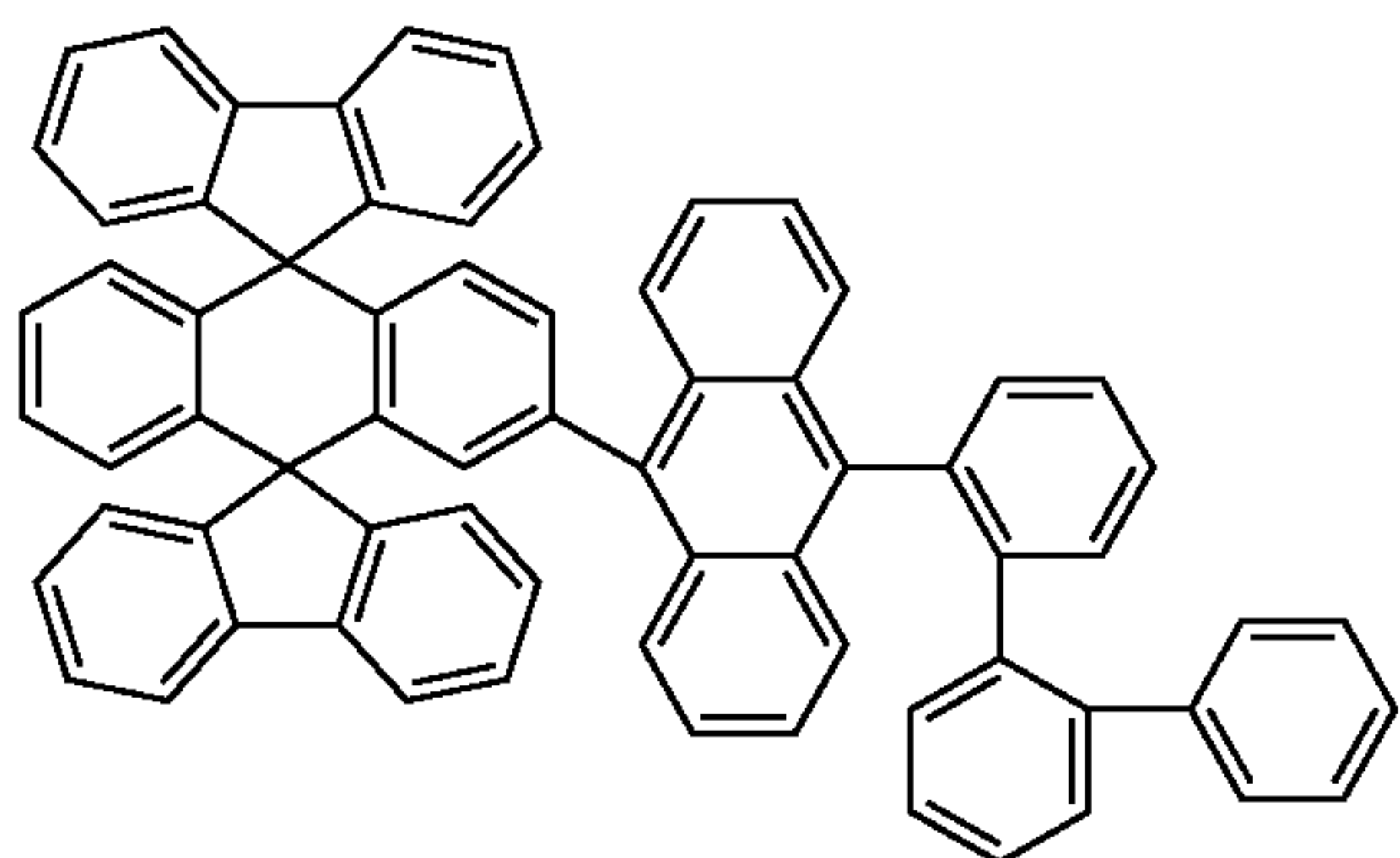
Chemical Compound 112
