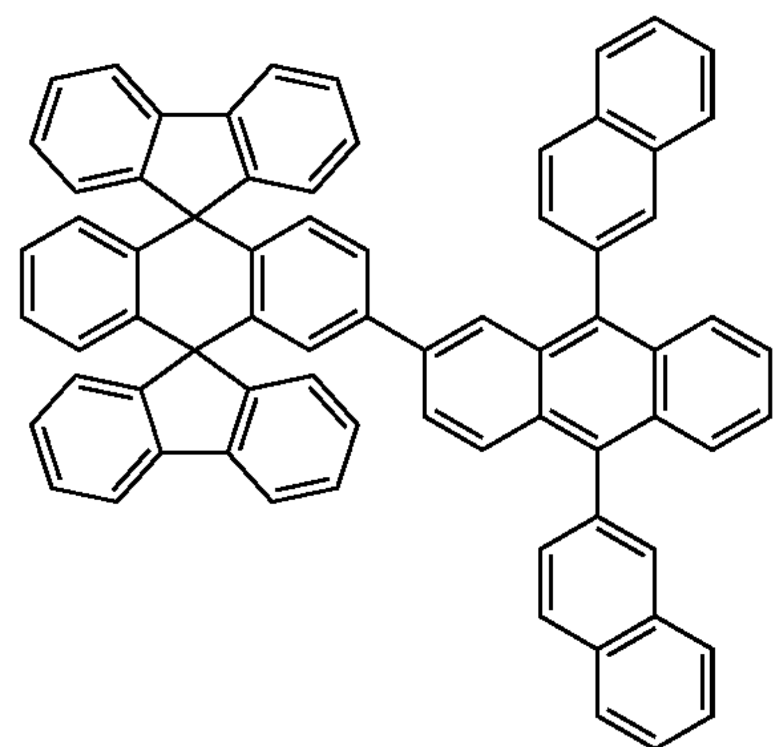
Chemical Compound 117
