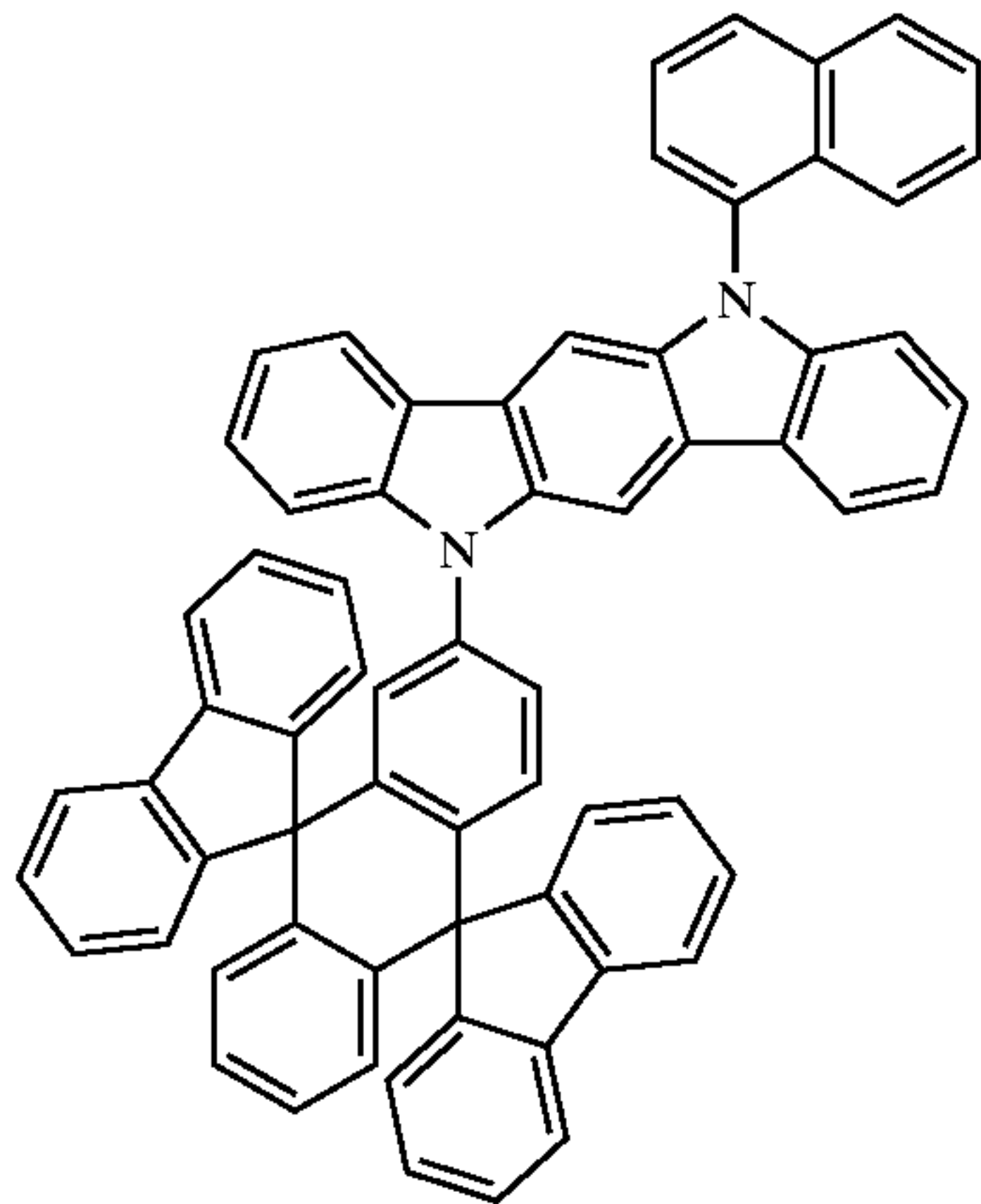
Chemical Compound 411
