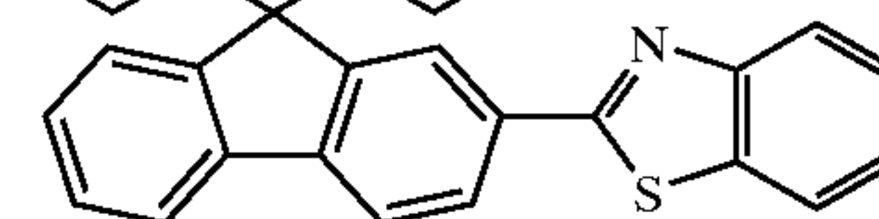
Chemical Compound 220
