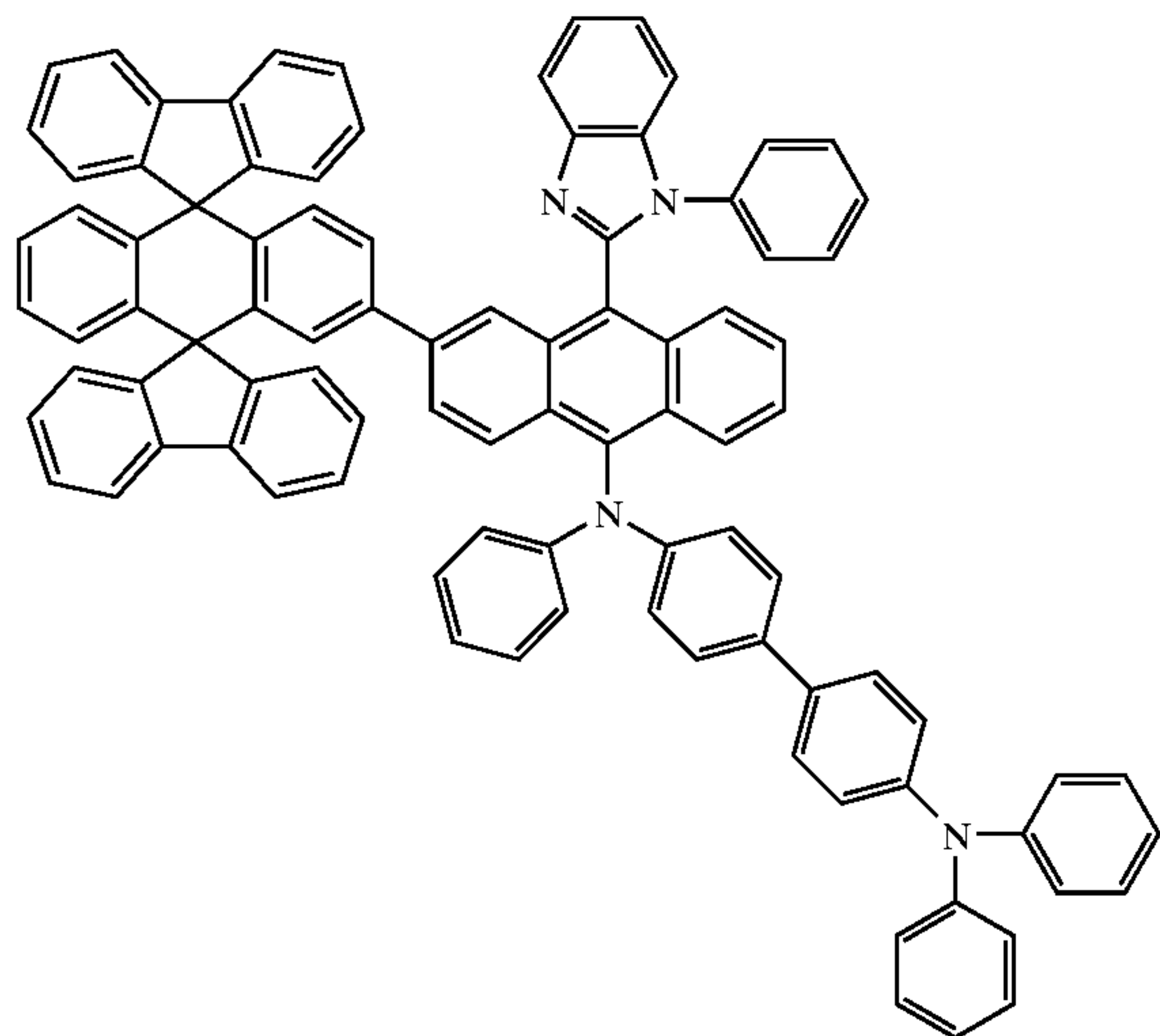
Chemical Compound 125
