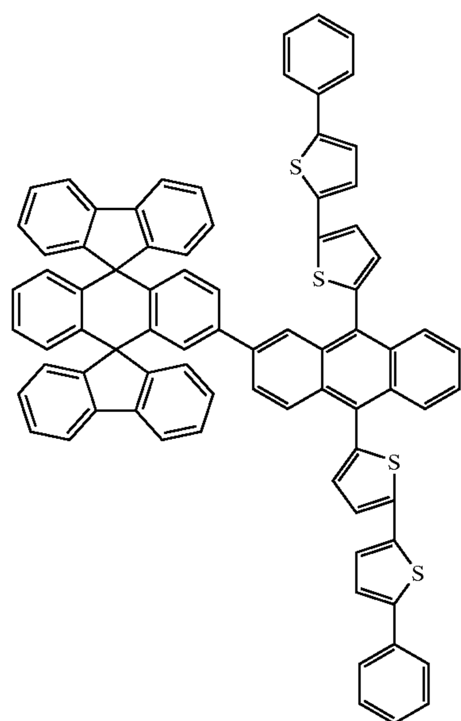
Chemical Compound 128
