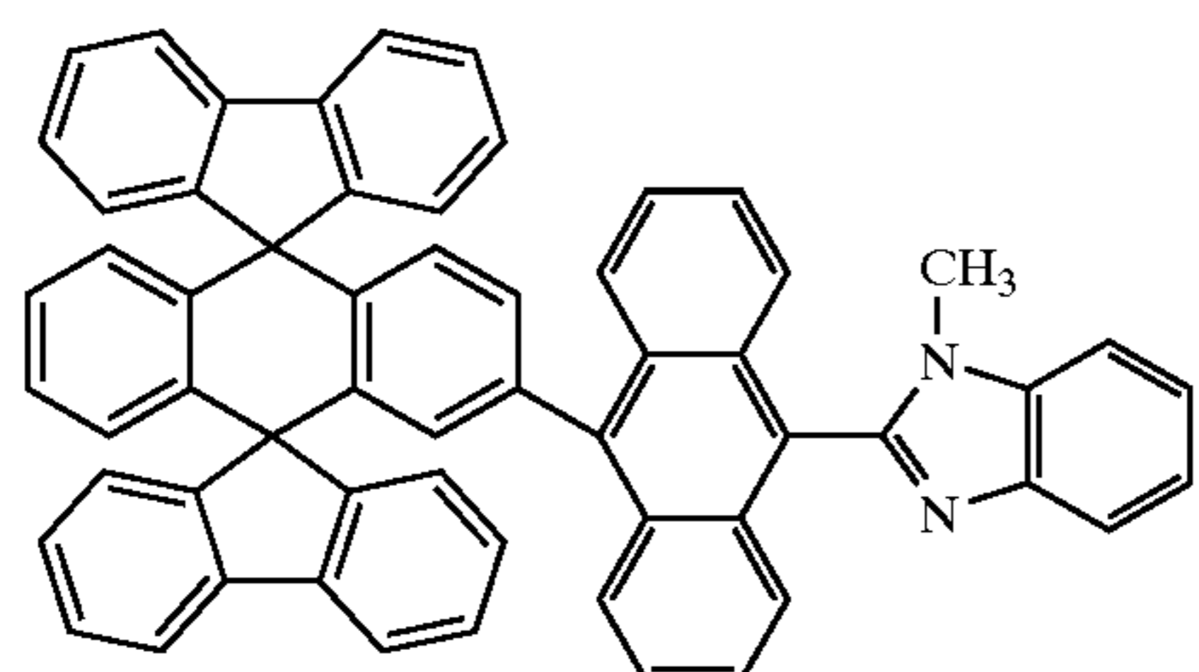
Chemical Compound 205
