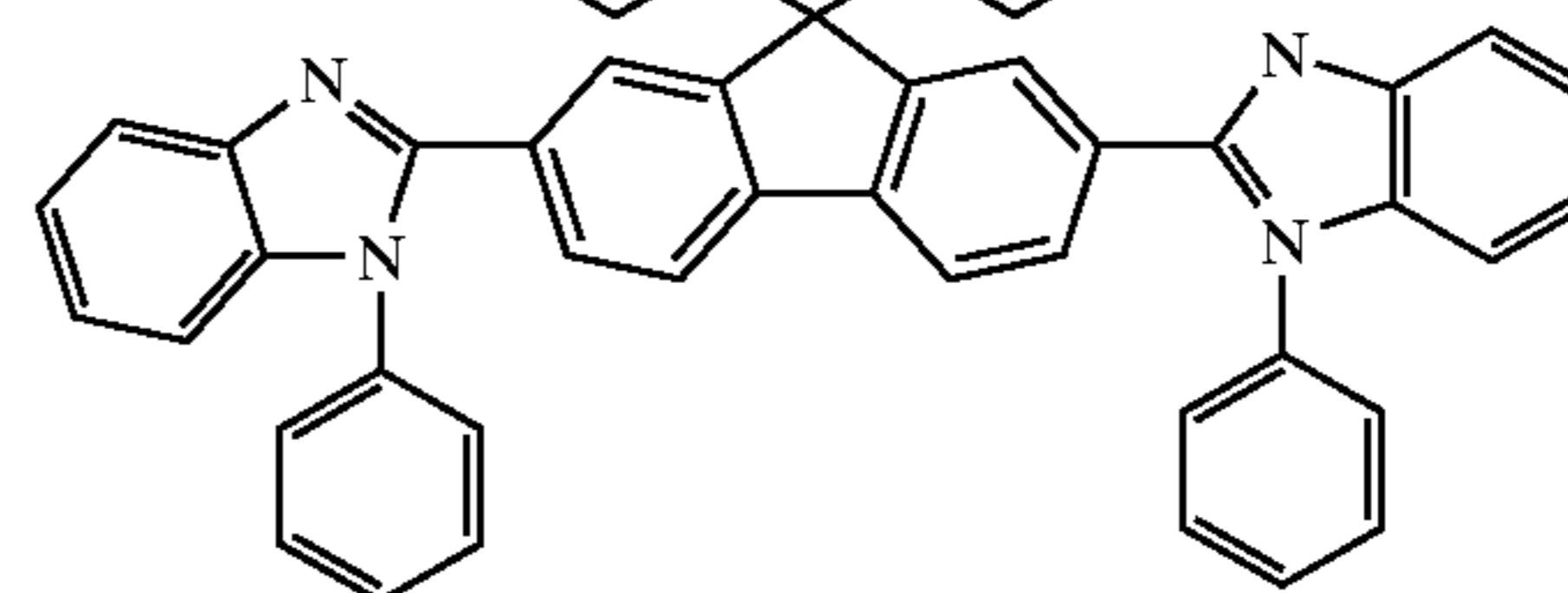
Chemical Compound 219
