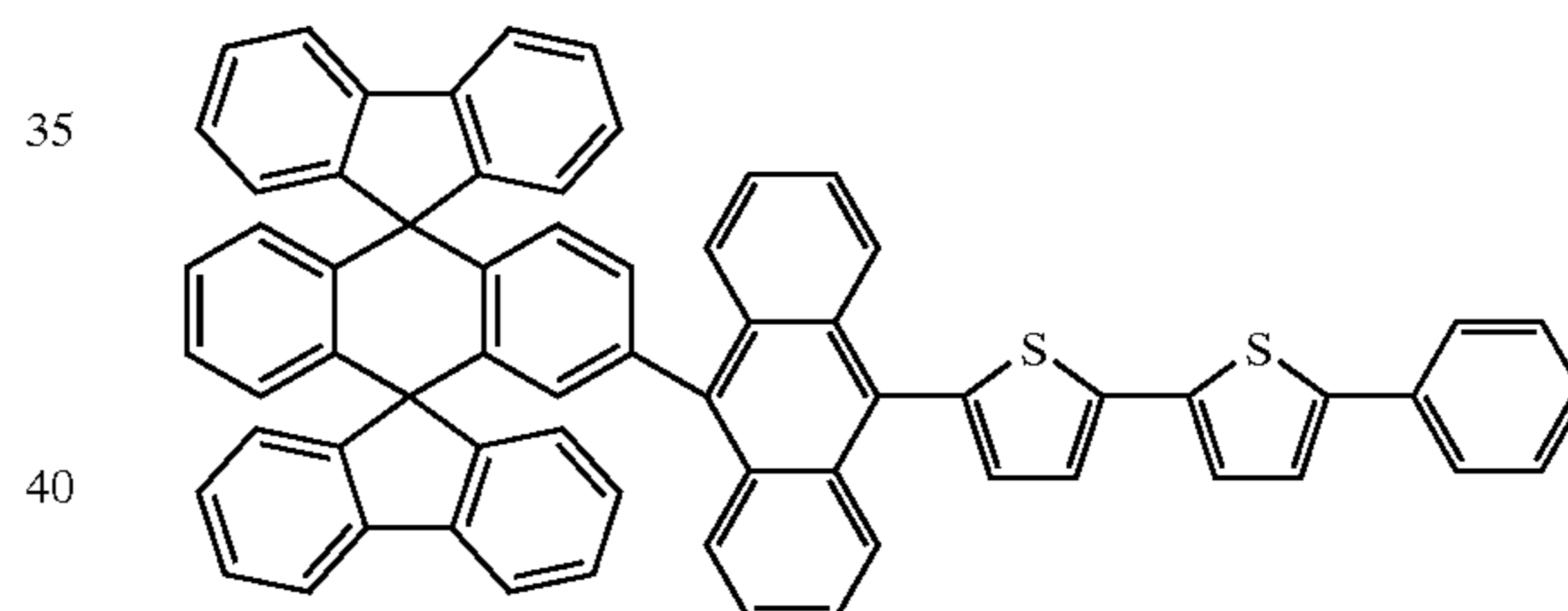
Chemical Compound 133
