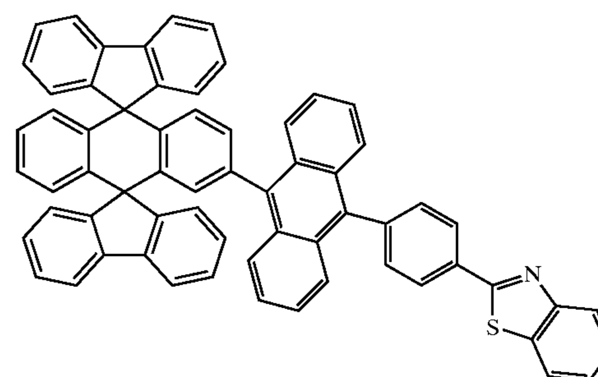
Chemical Compound 217
