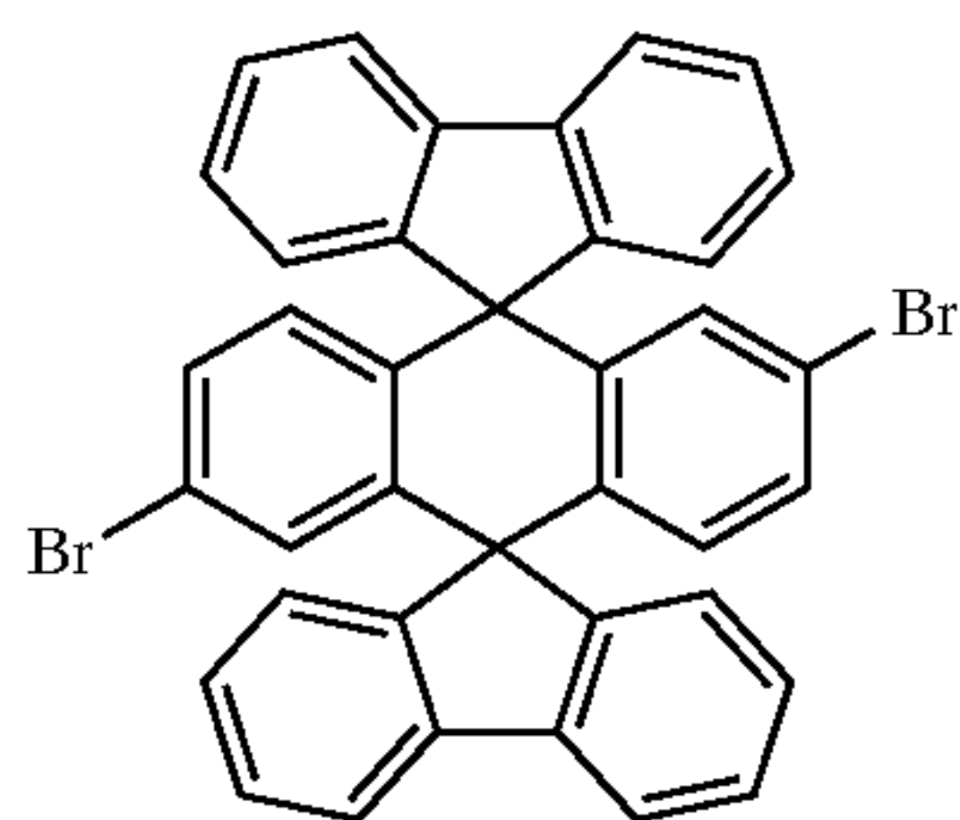
Chemical Compound 2
