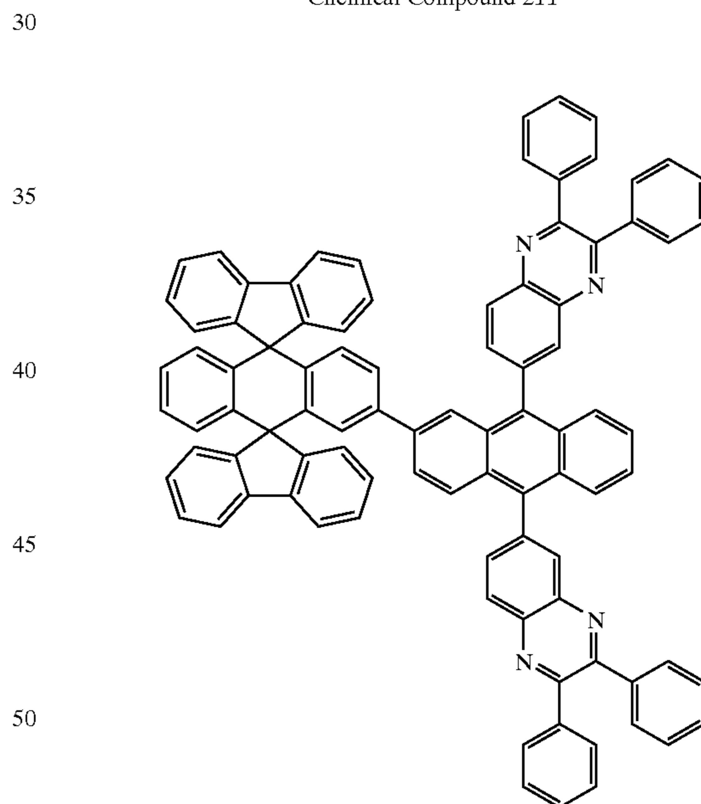
Chemical Compound 212
