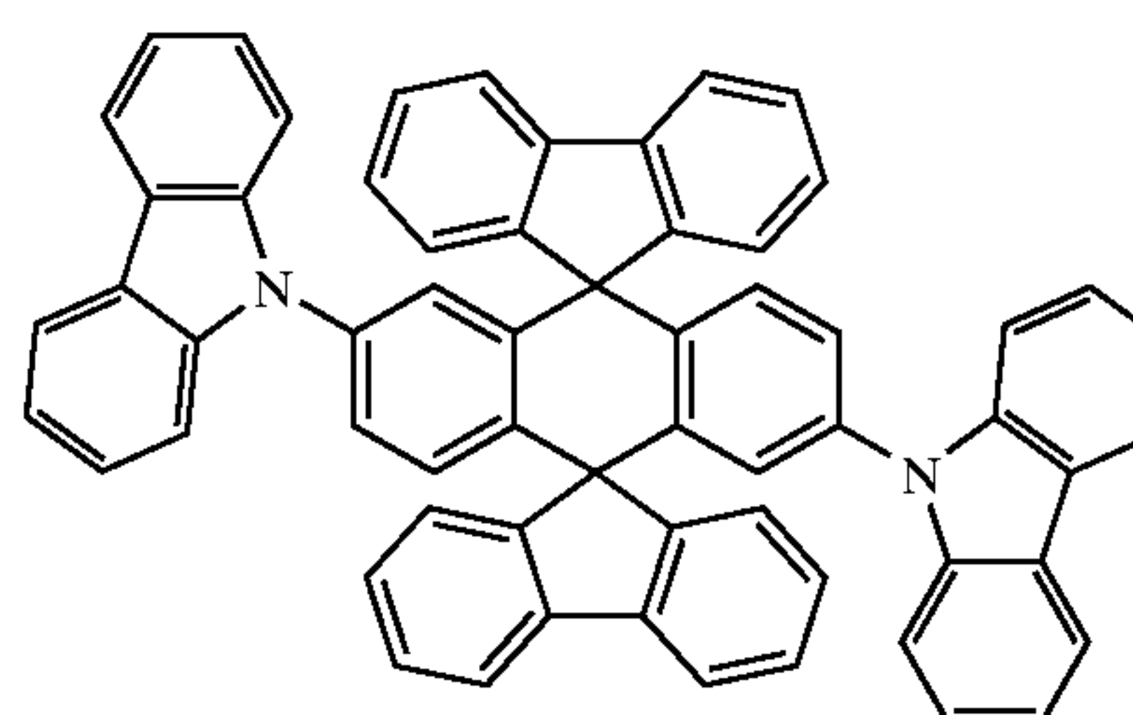
Chemical Compound 407
