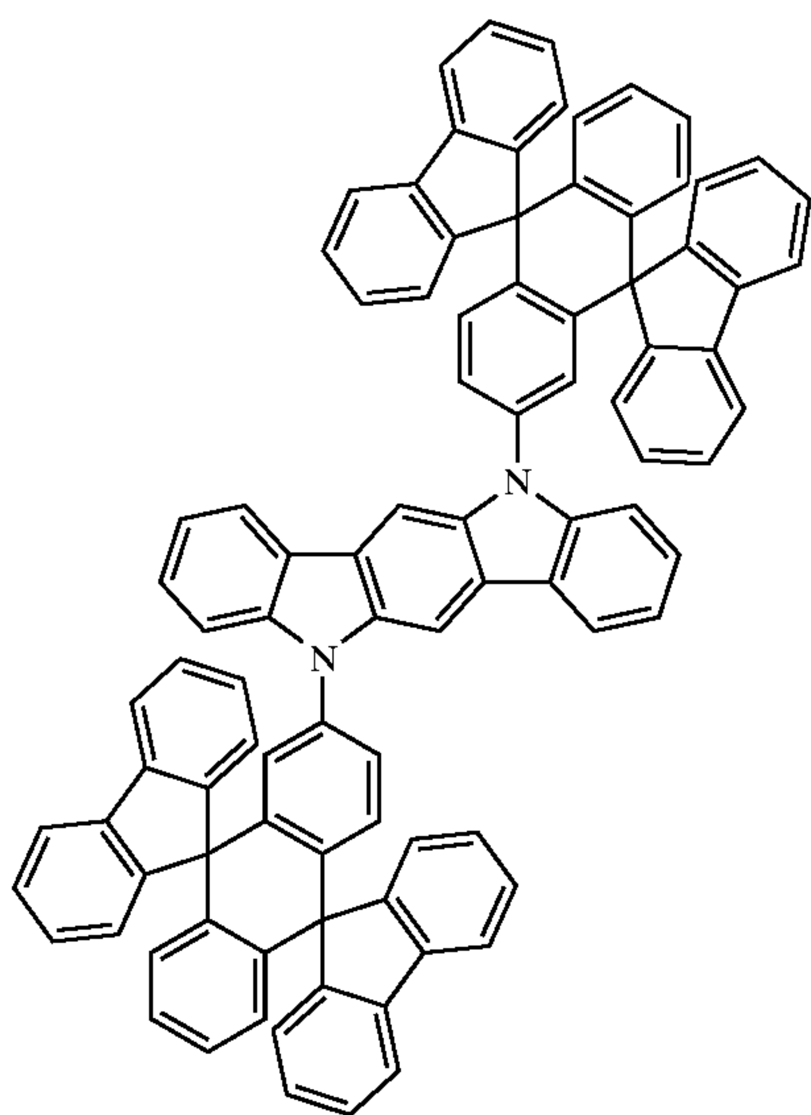
Chemical Compound 405
