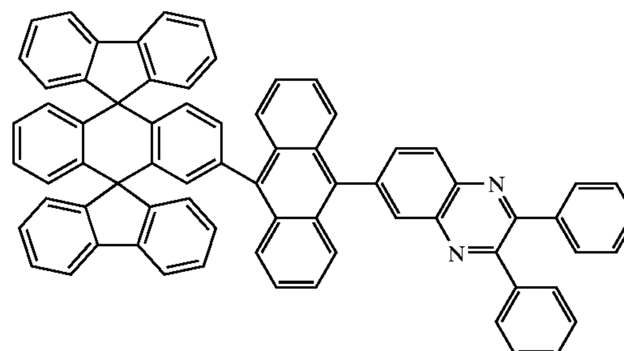
Chemical Compound 203
