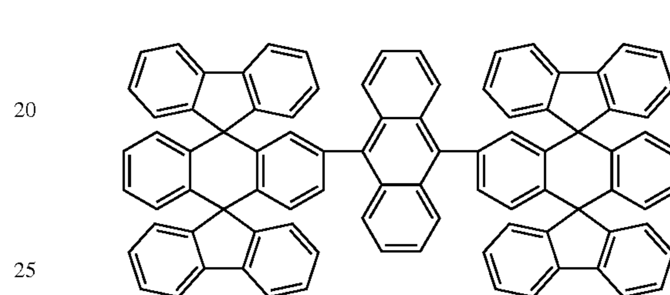
Chemical Compound 102
