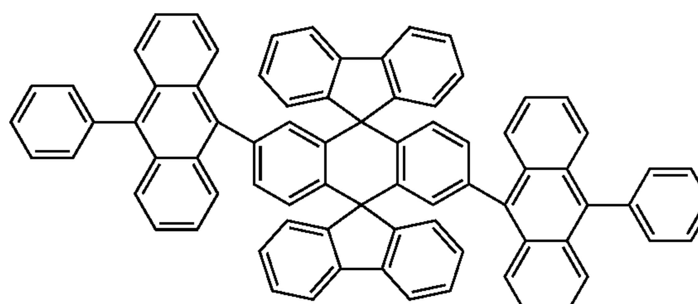
Chemical Compound 114
