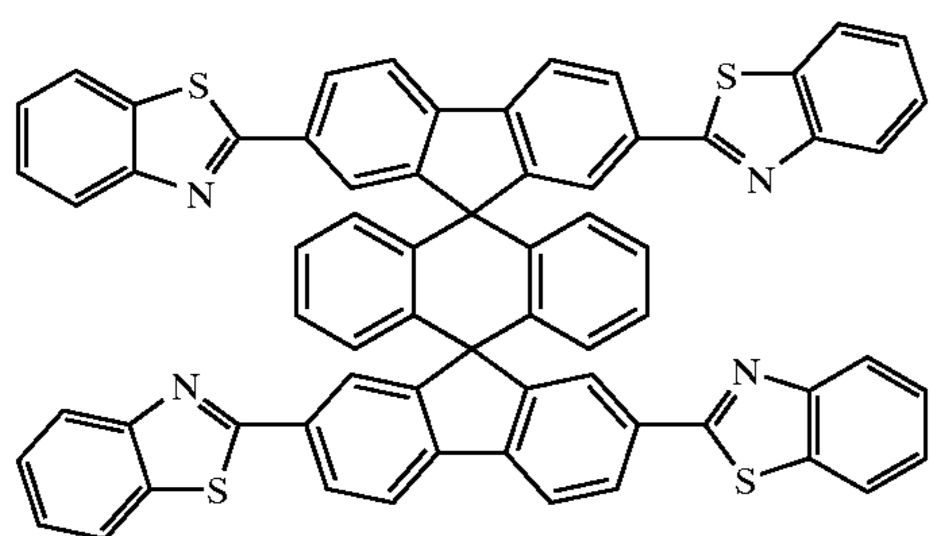
Chemical Compound 218
