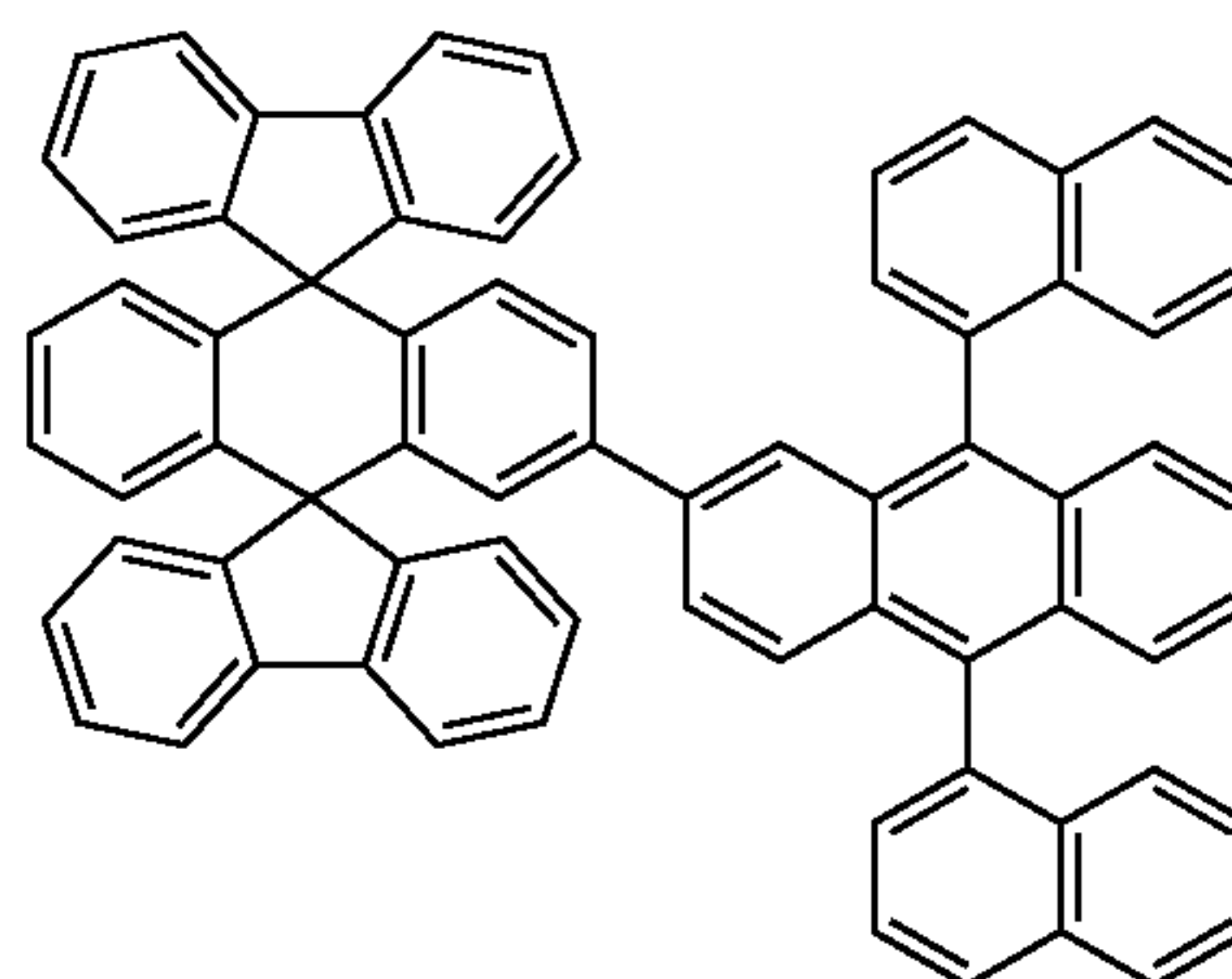
Chemical Compound 120
