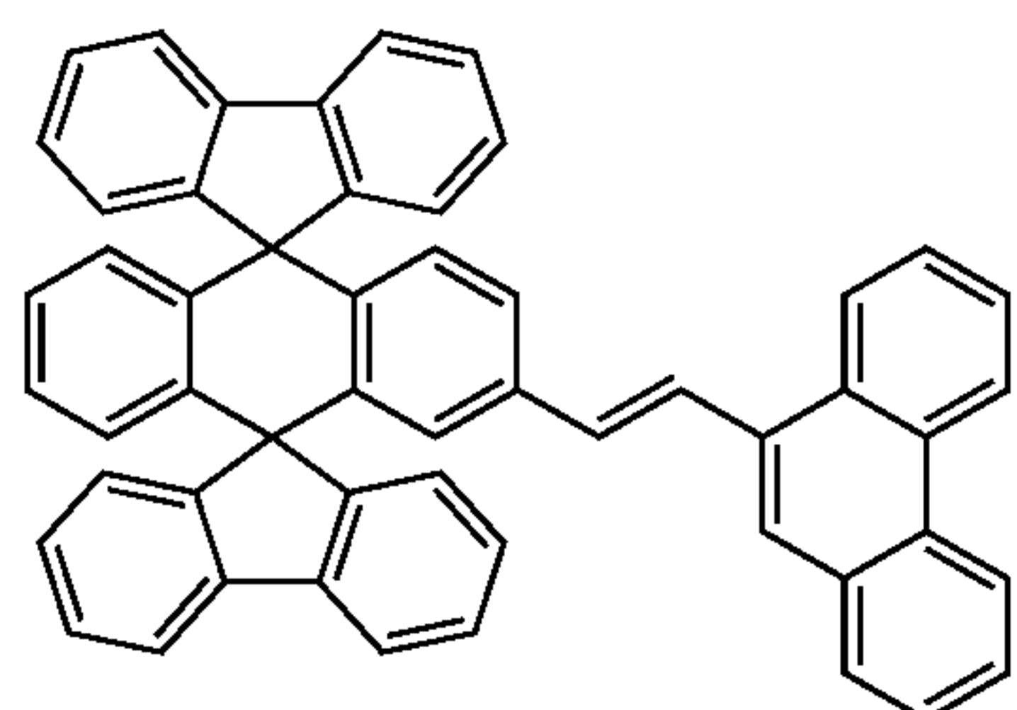
Chemical Compound 104
