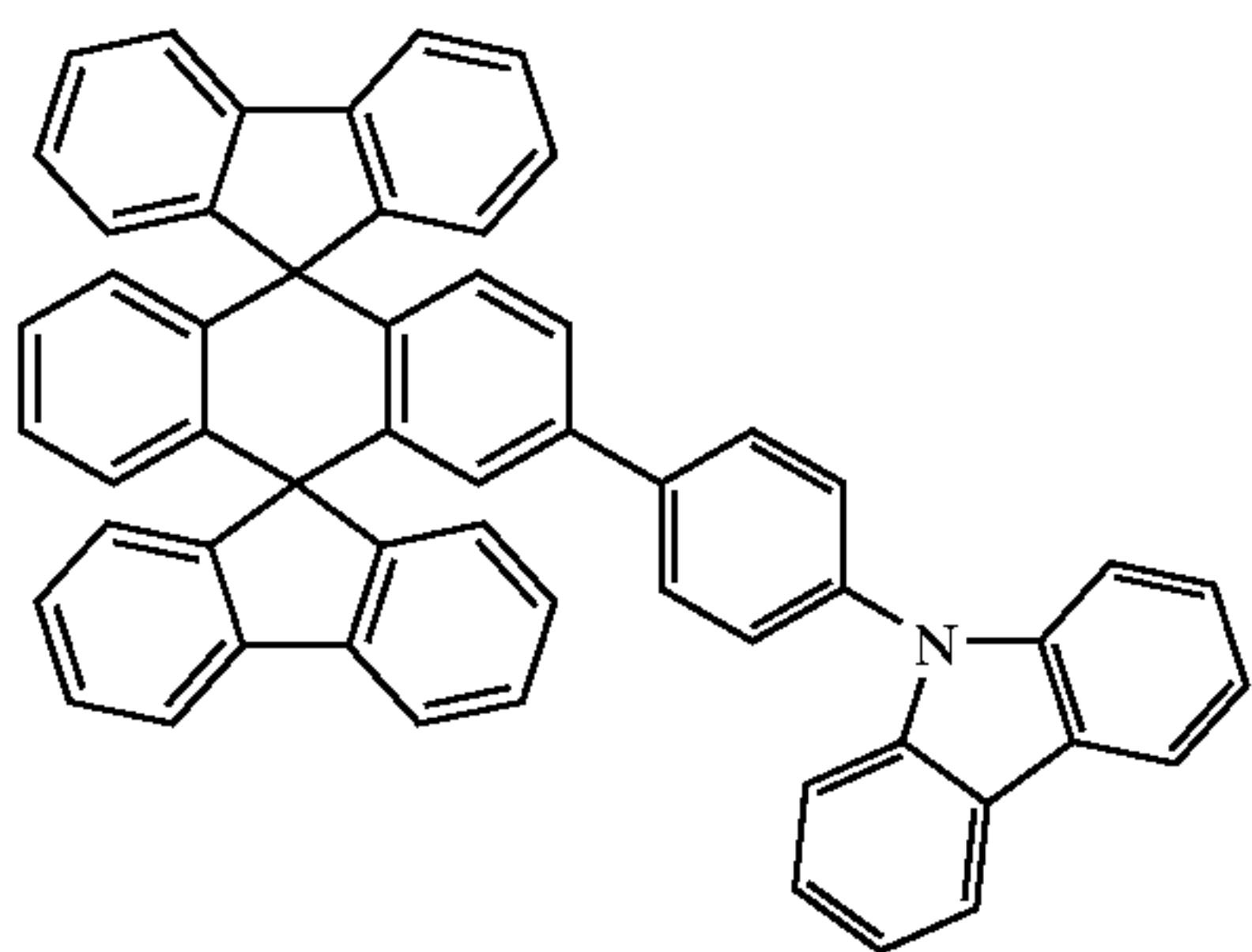
Chemical Compound 406
