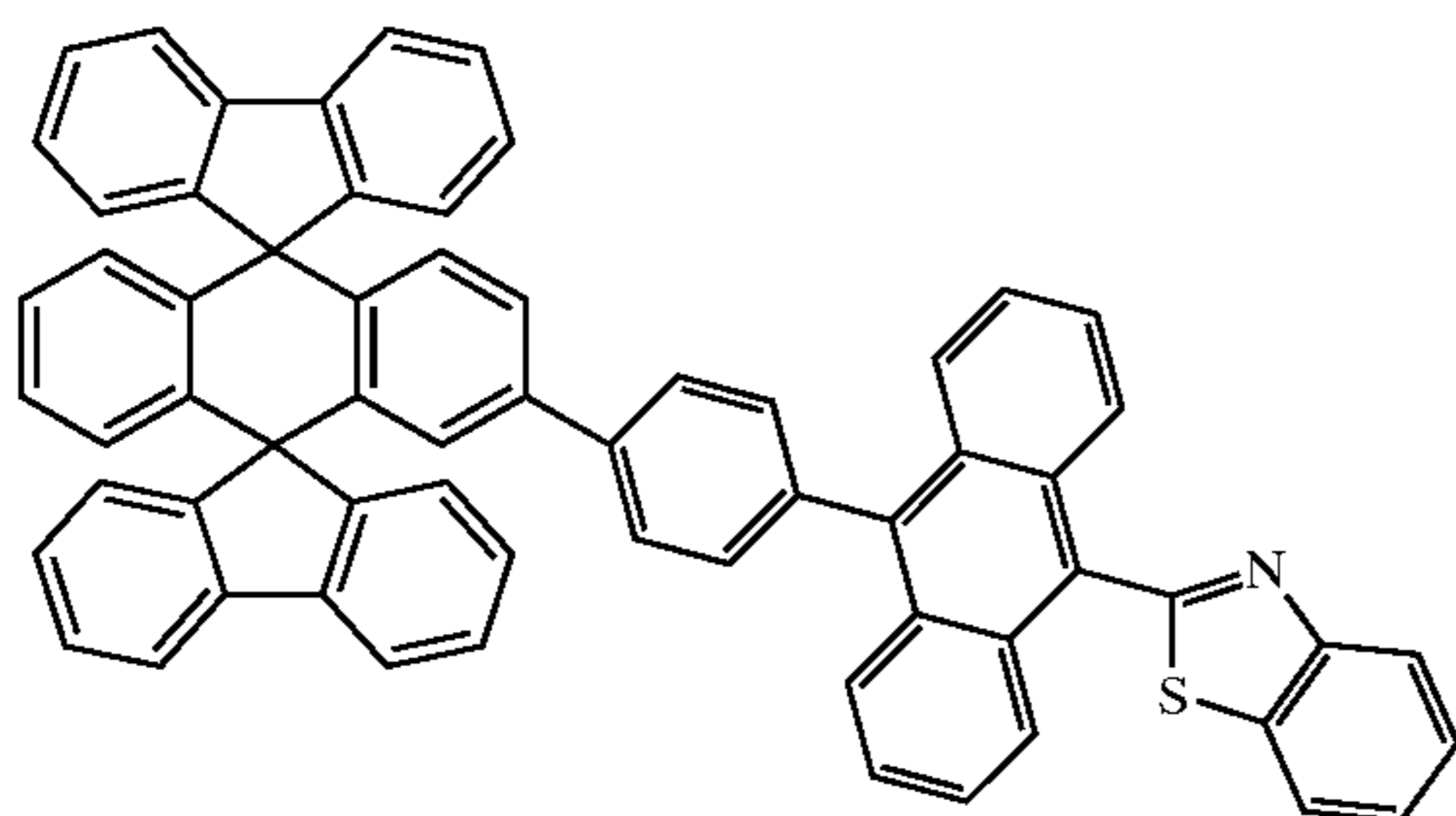
Chemical Compound 216
