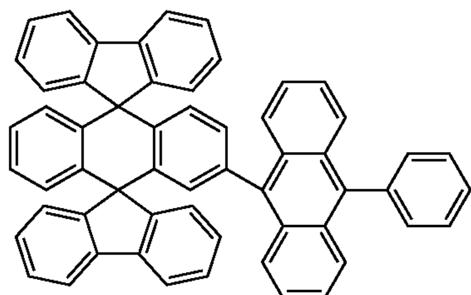
Chemical Compound 109
