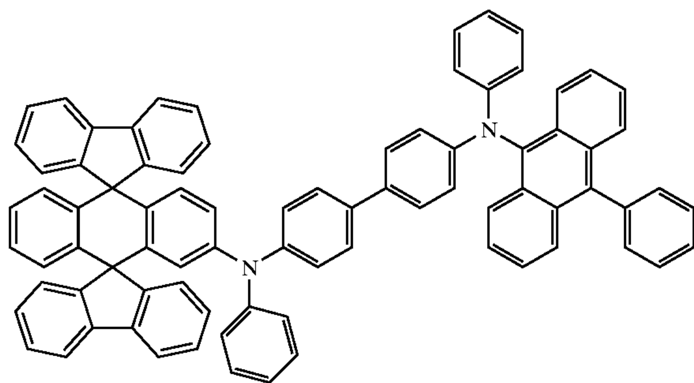
Chemical Compound 408
