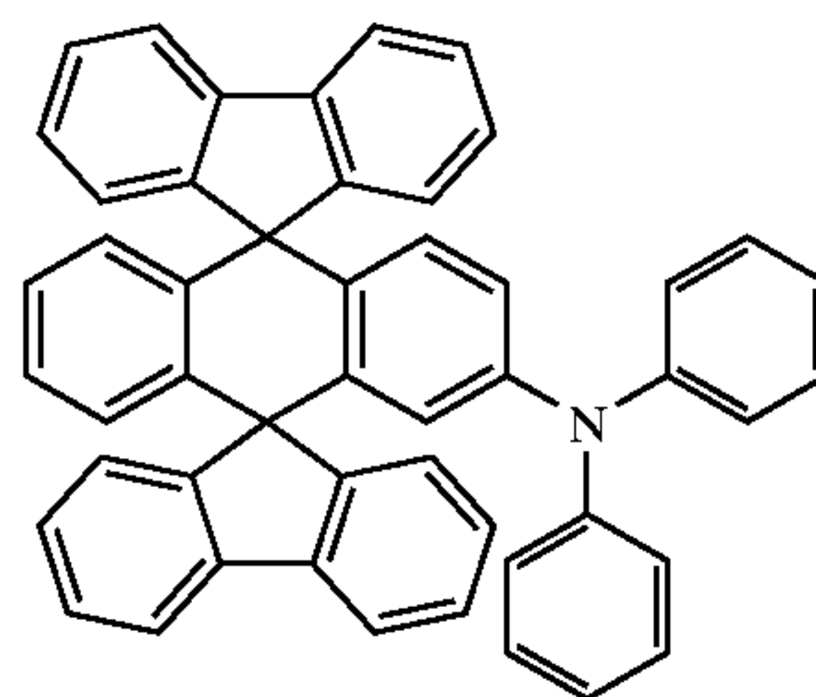
Chemical Compound 300
