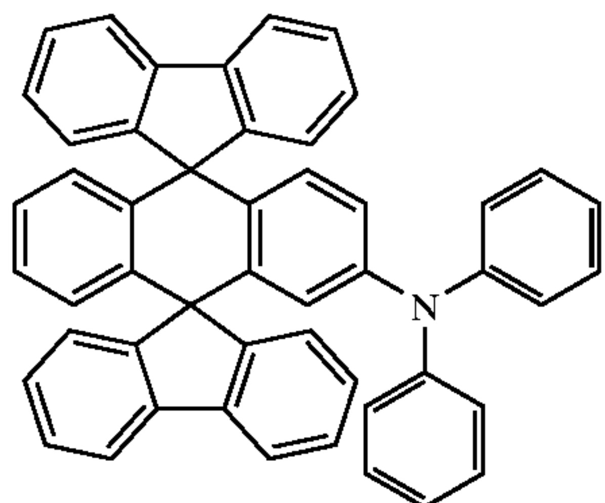
Chemical Compound 300
