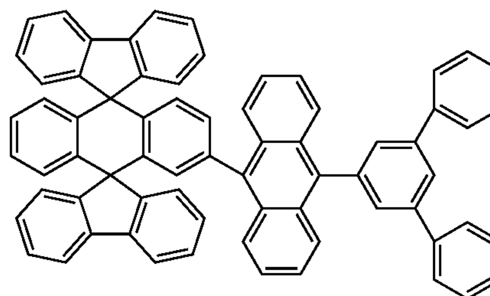
Chemical Compound 113
