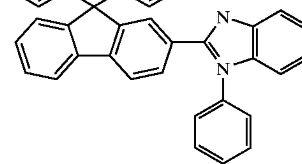
Chemical Compound 221
