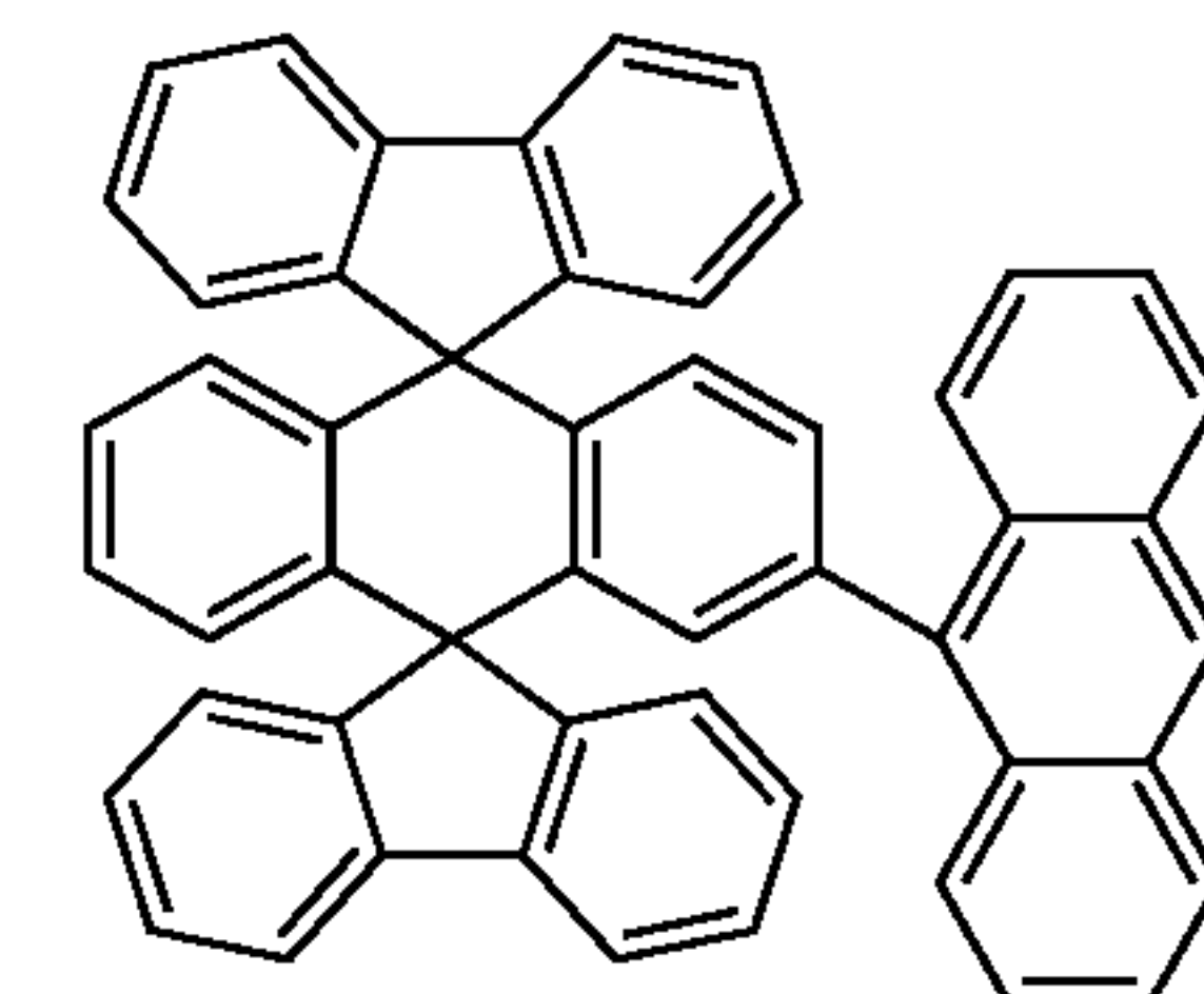
Chemical Compound 9
