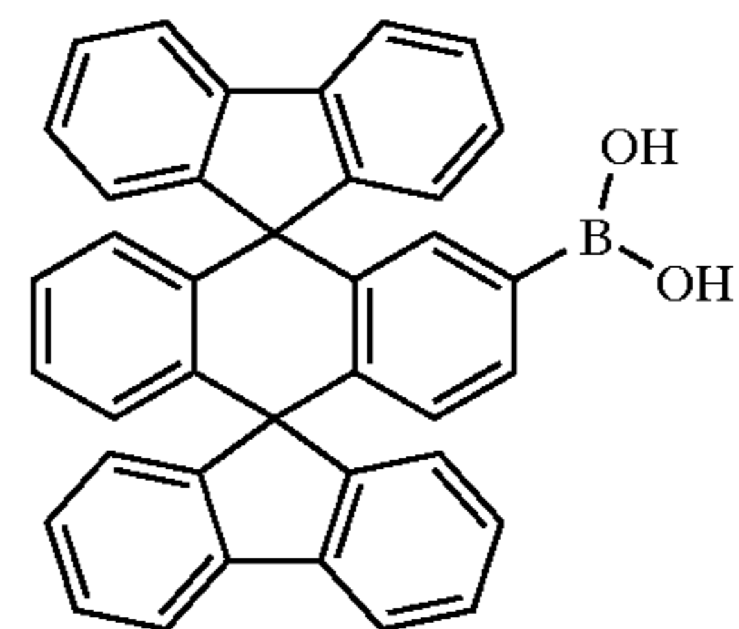
Chemical Compound 8
