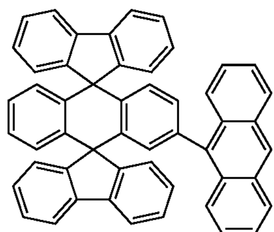
Chemical Compound 9
