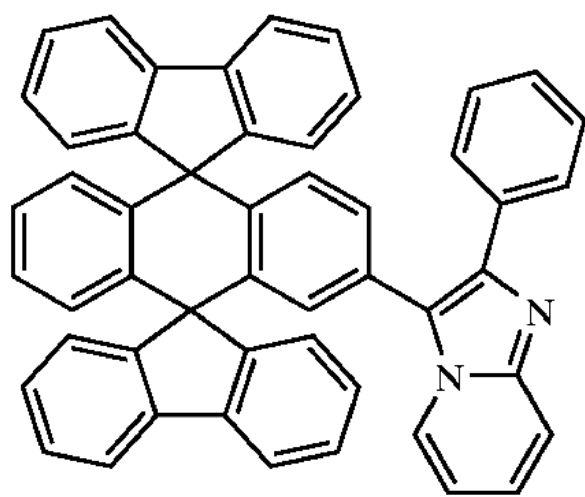
Chemical compound 412
