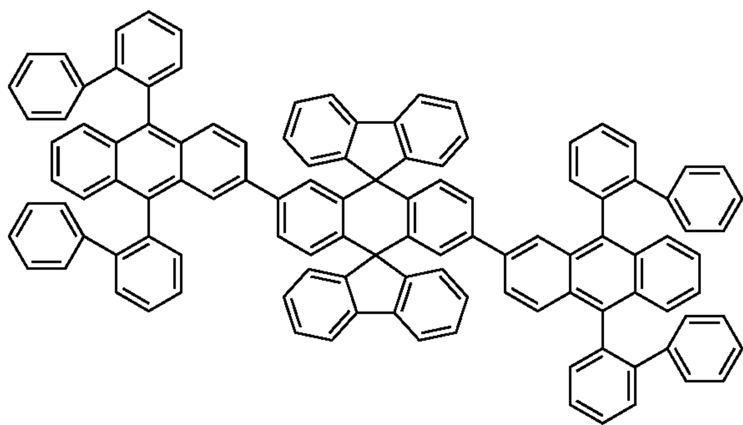
Chemical Compound 121
