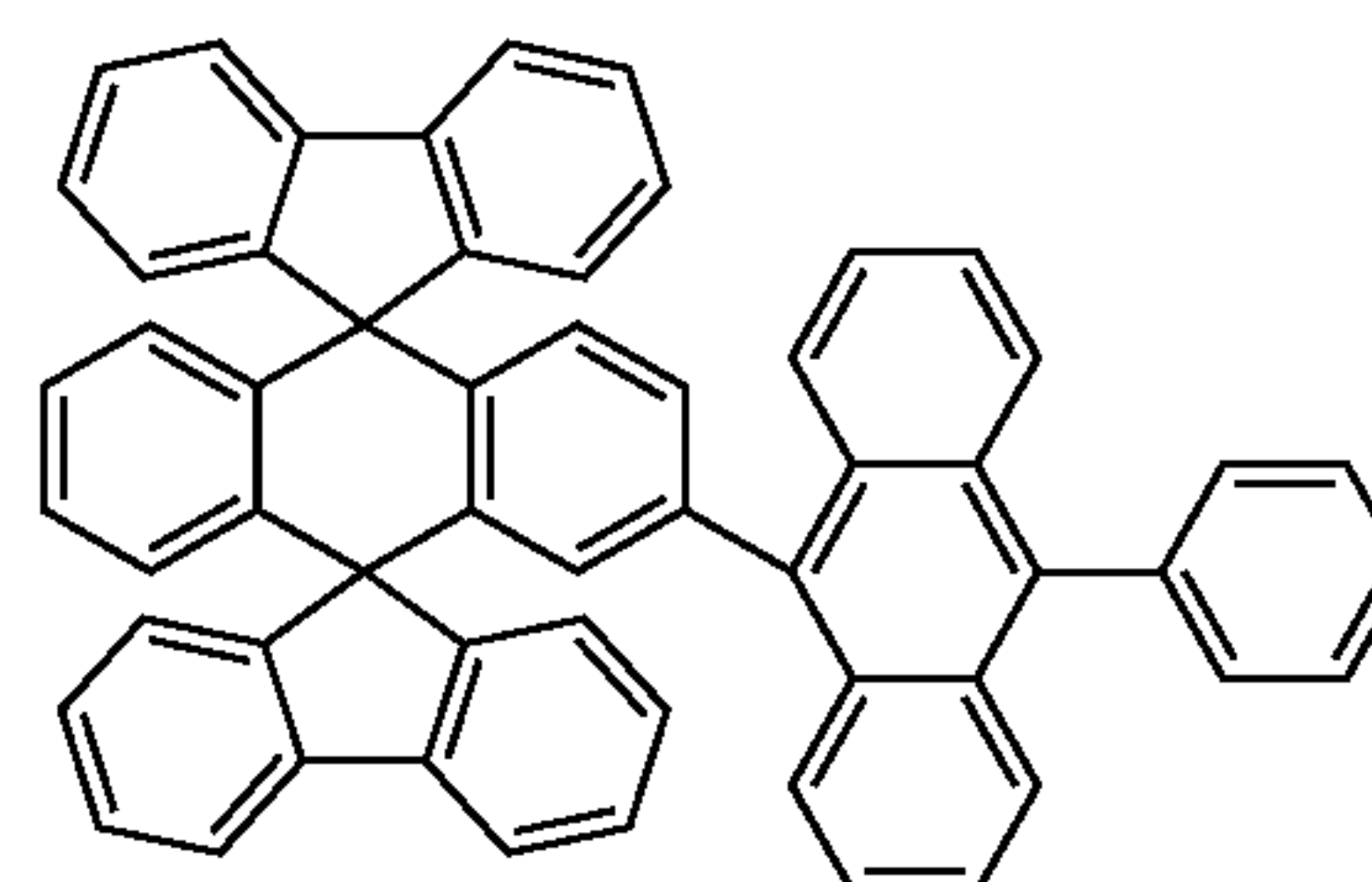
Chemical Compound 109
