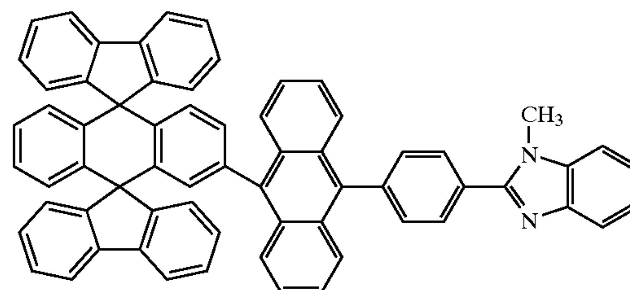
Chemical Compound 208
