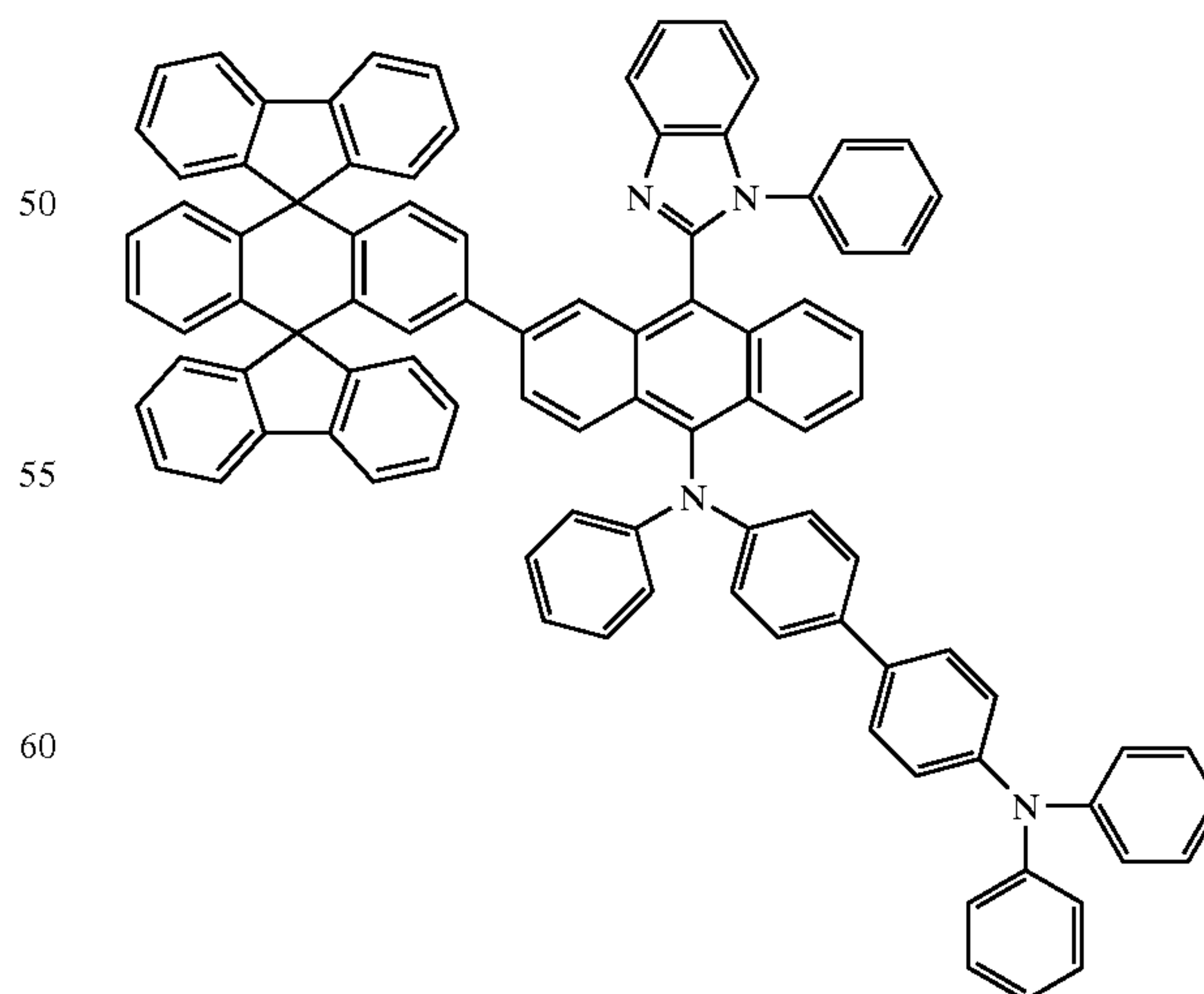
Chemical Compound 125
