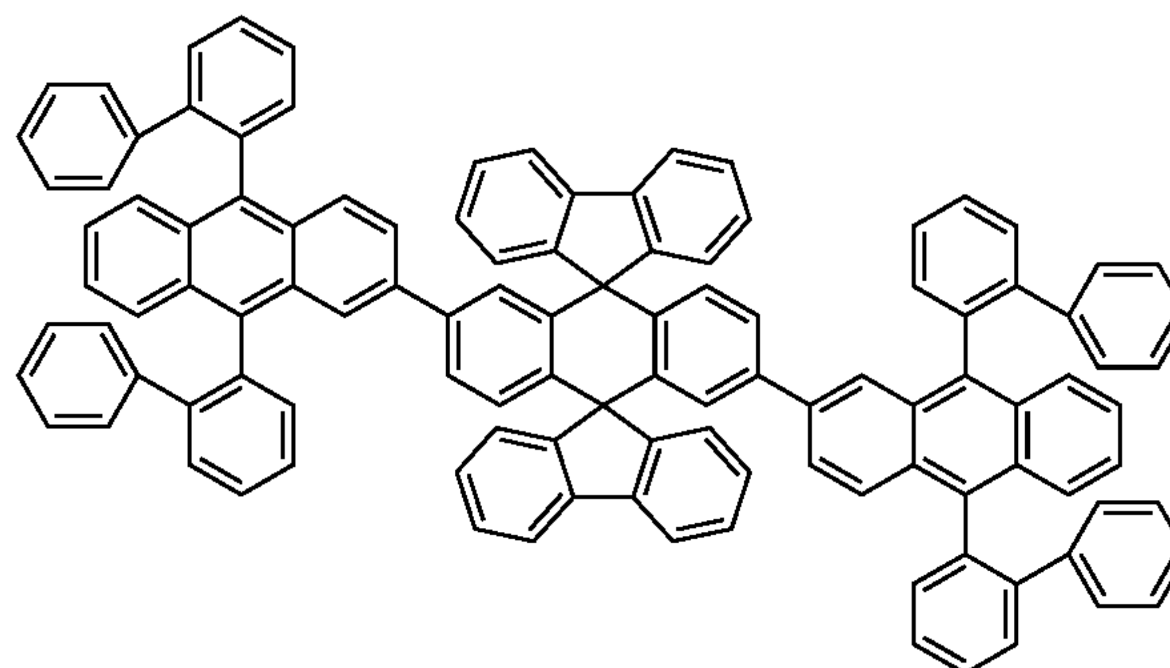
Chemical Compound 121
