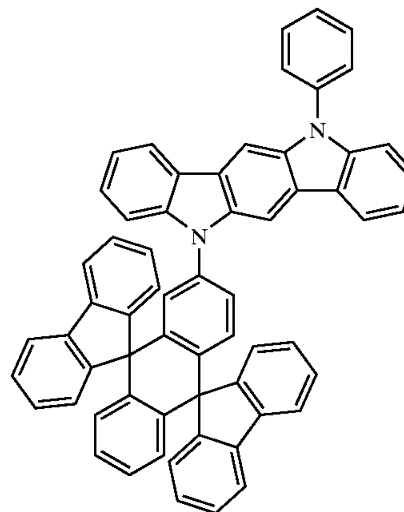
Chemical Compound 410
