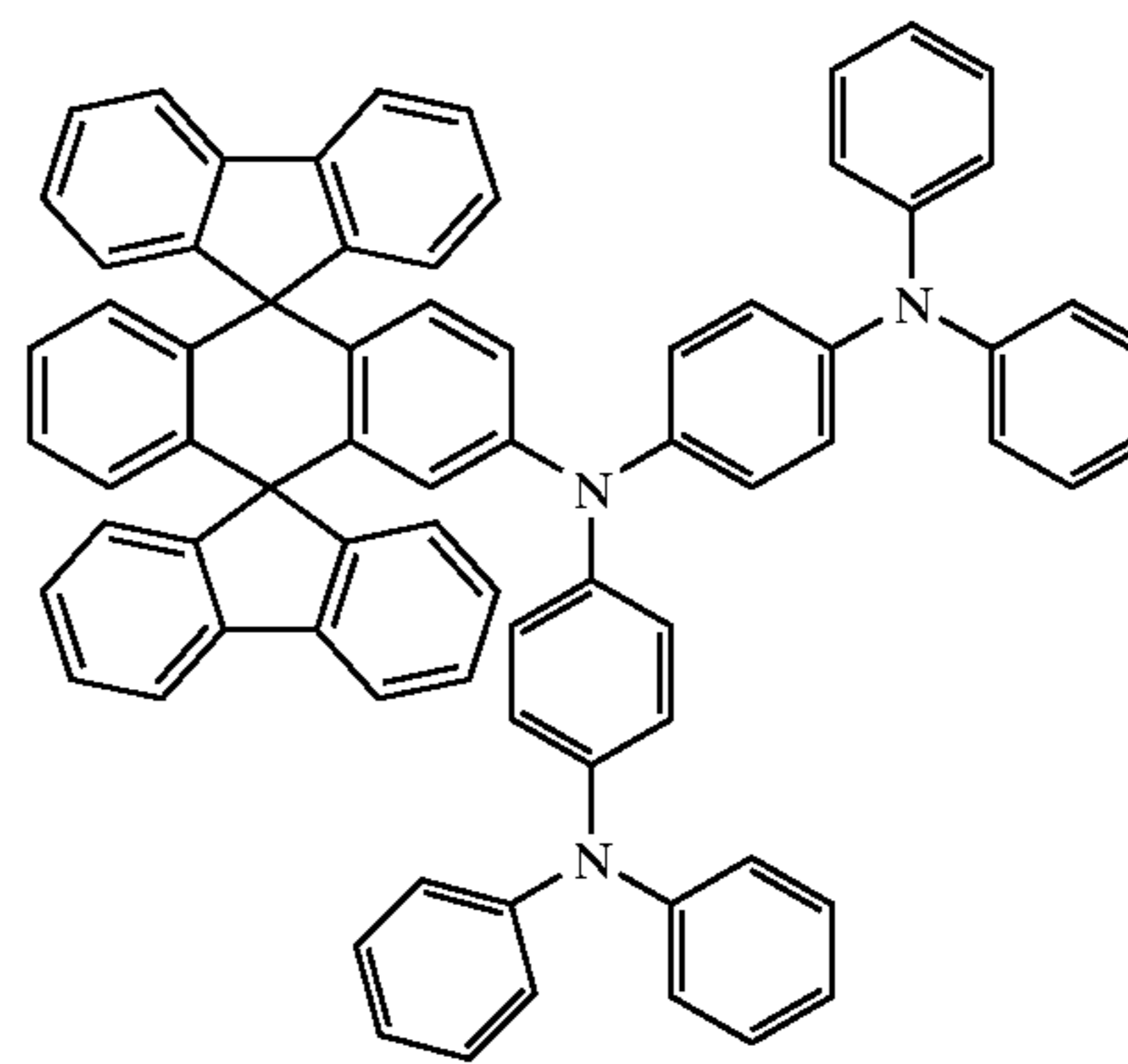
Chemical Compound 308
