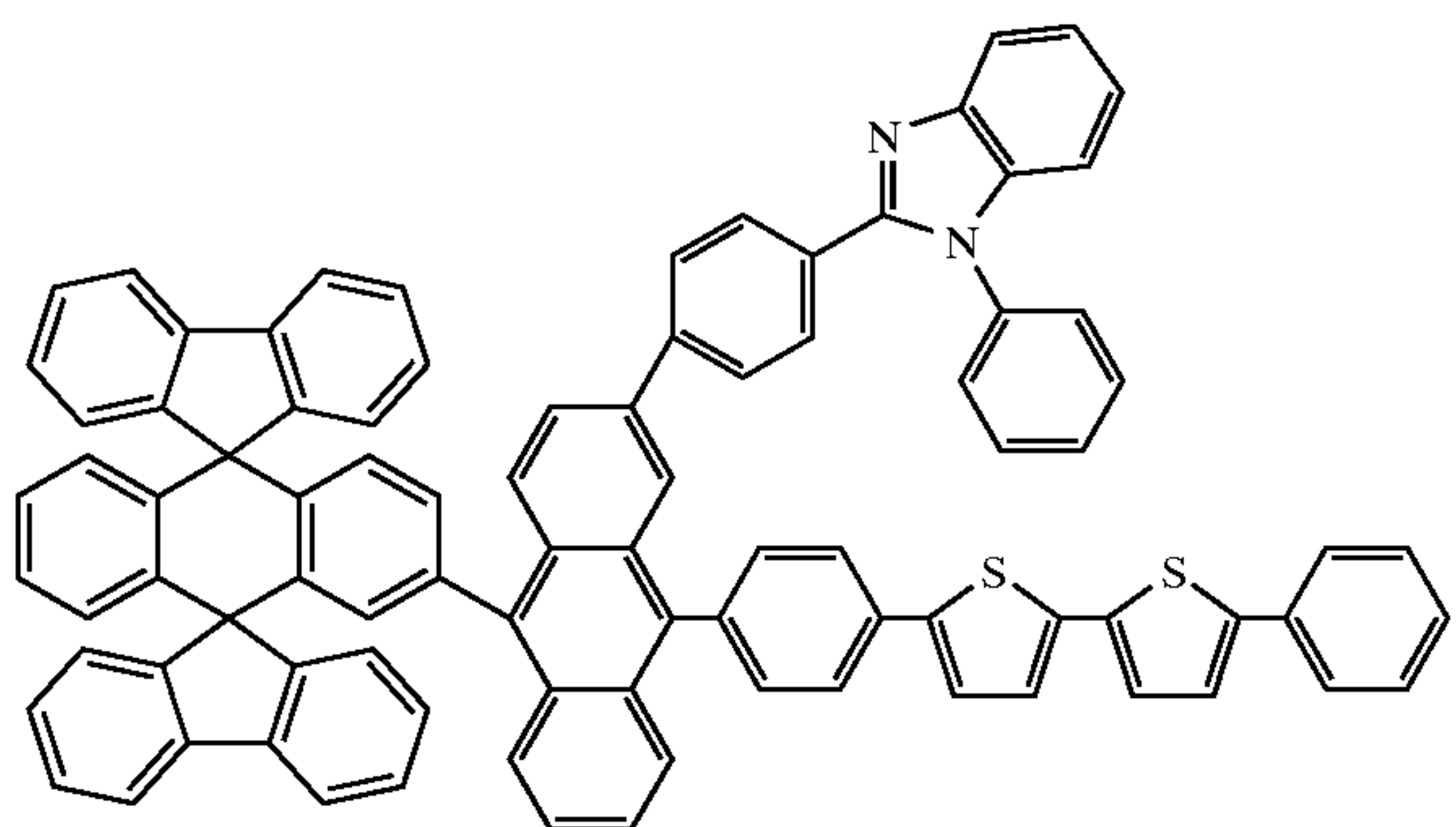
Chemical Compound 132
