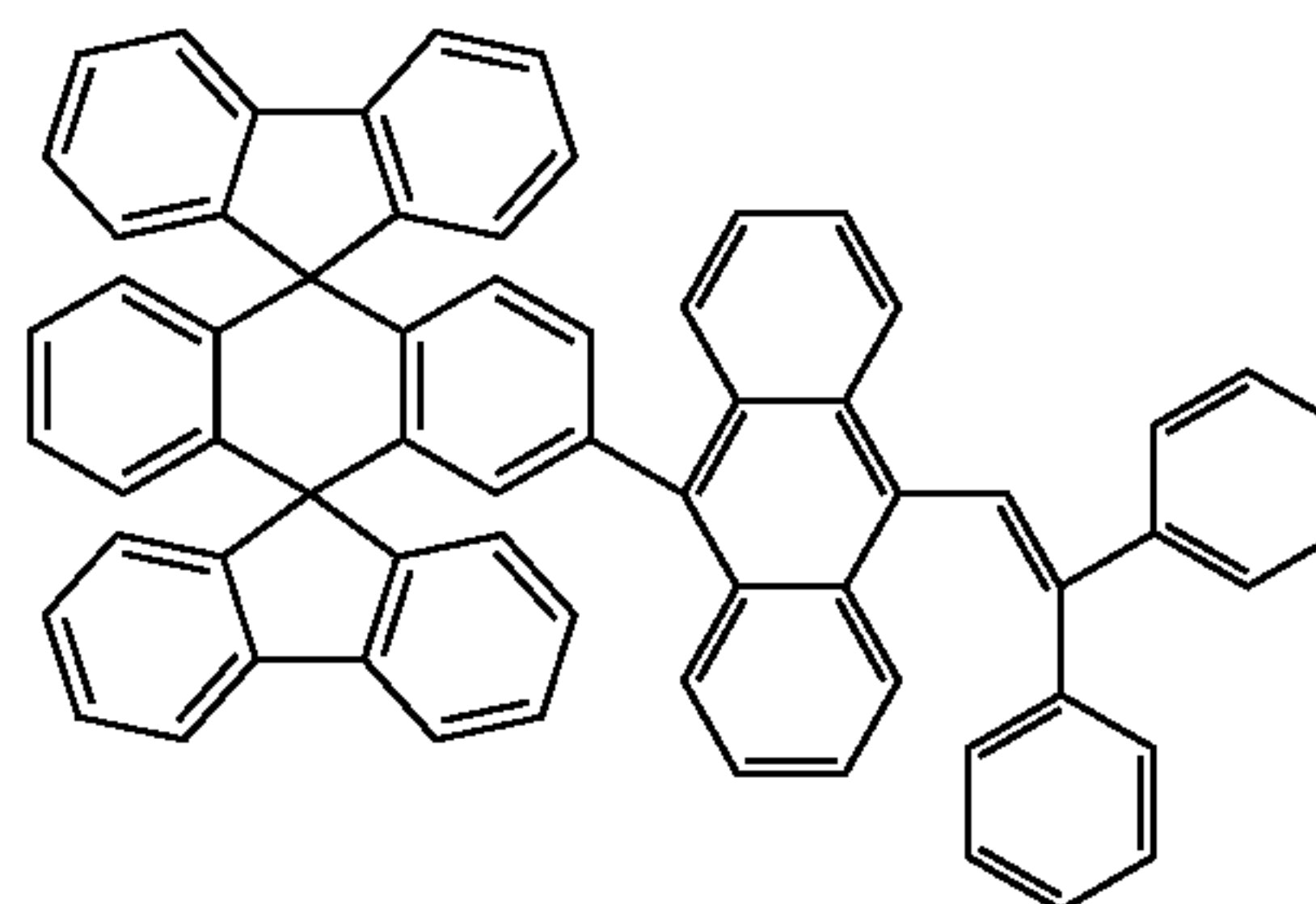
Chemical Compound 137
