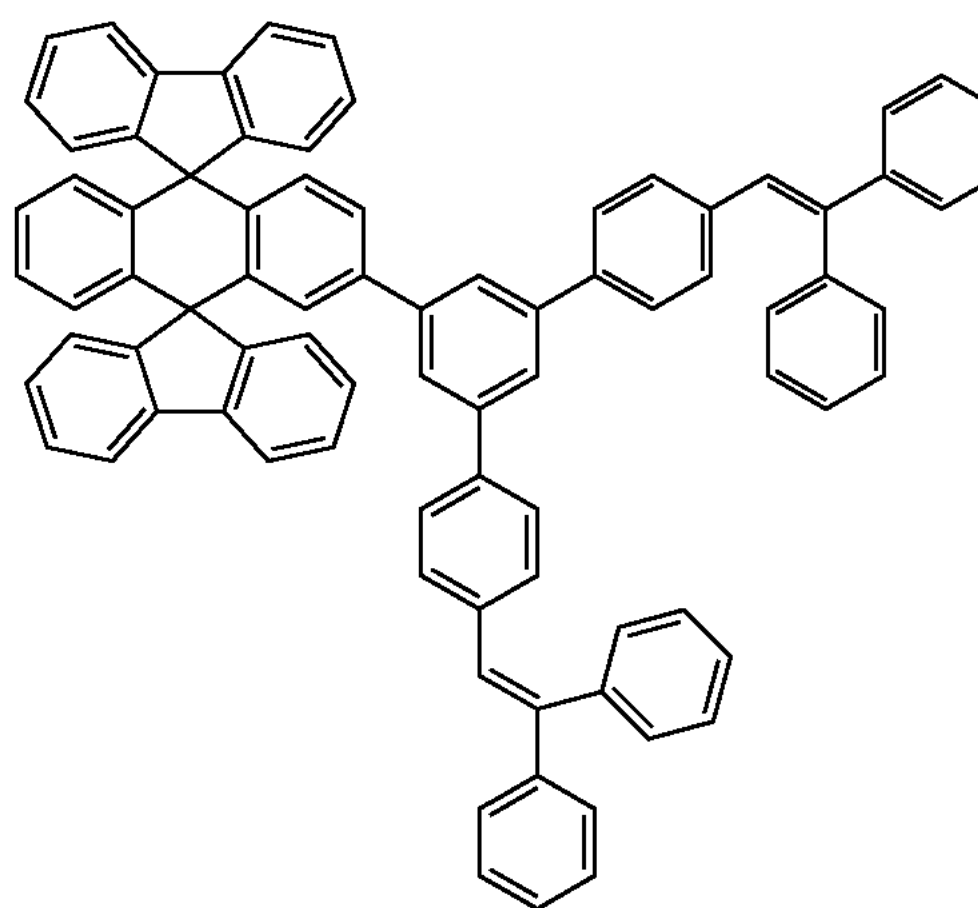
Chemical Compound 108
