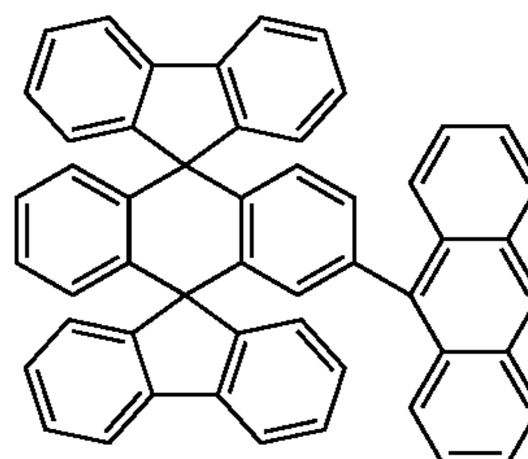
Chemical Compound 9
