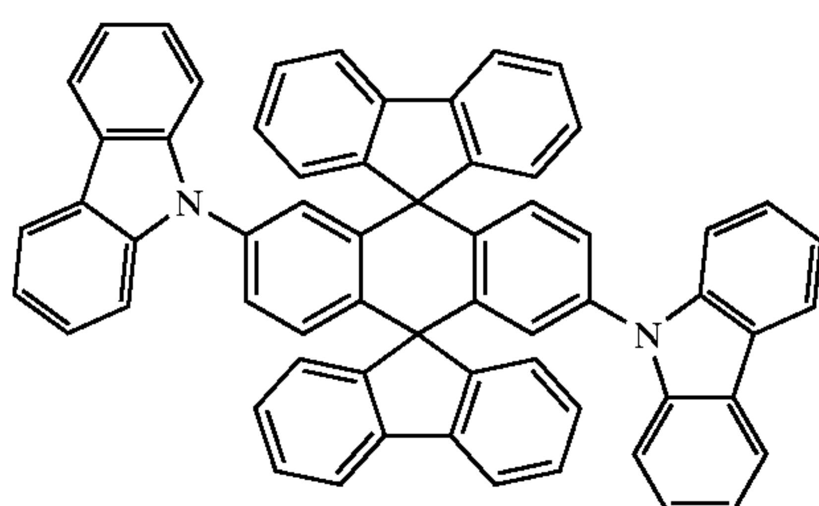
Chemical Compound 407
