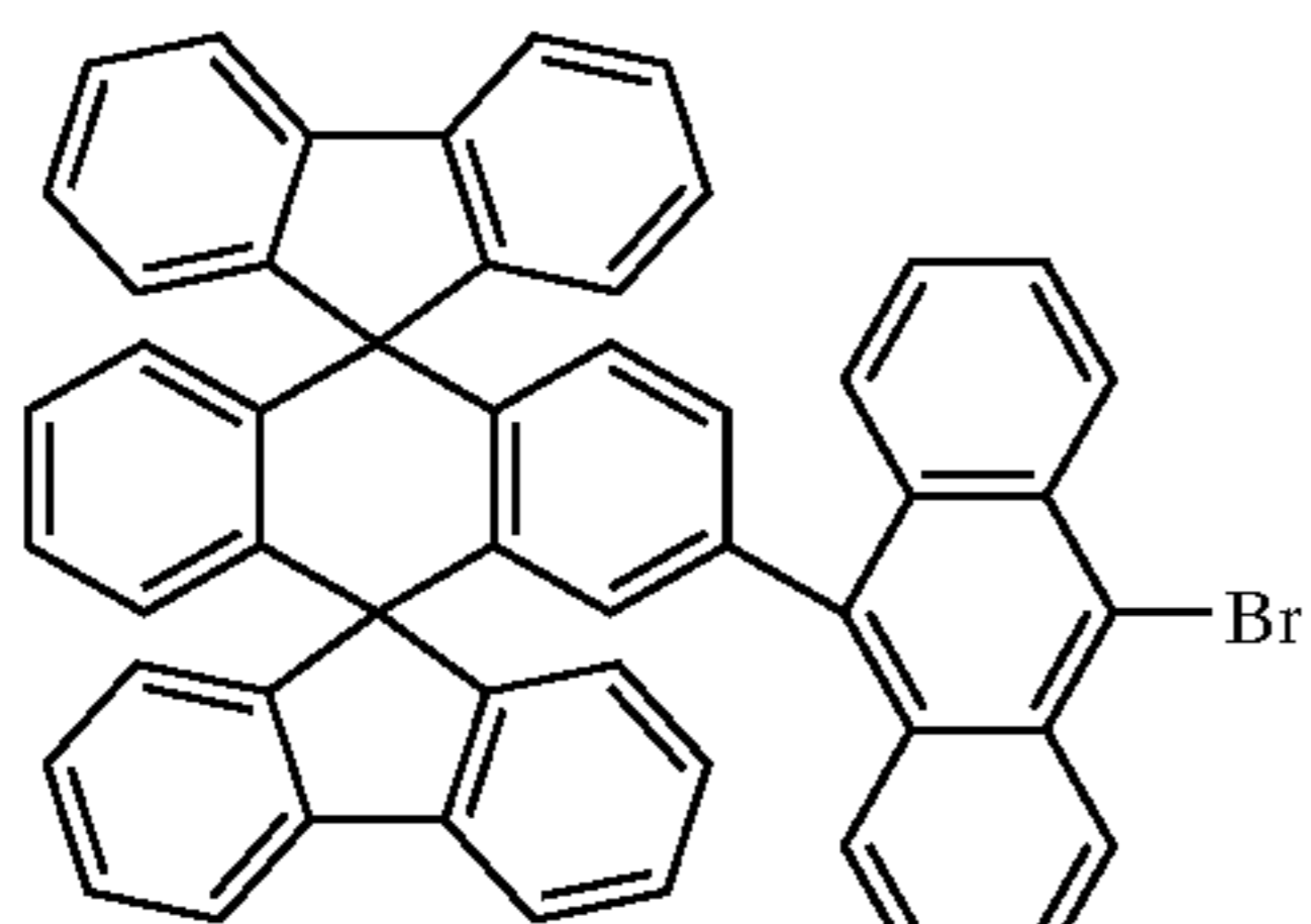
Chemical Compound 5
