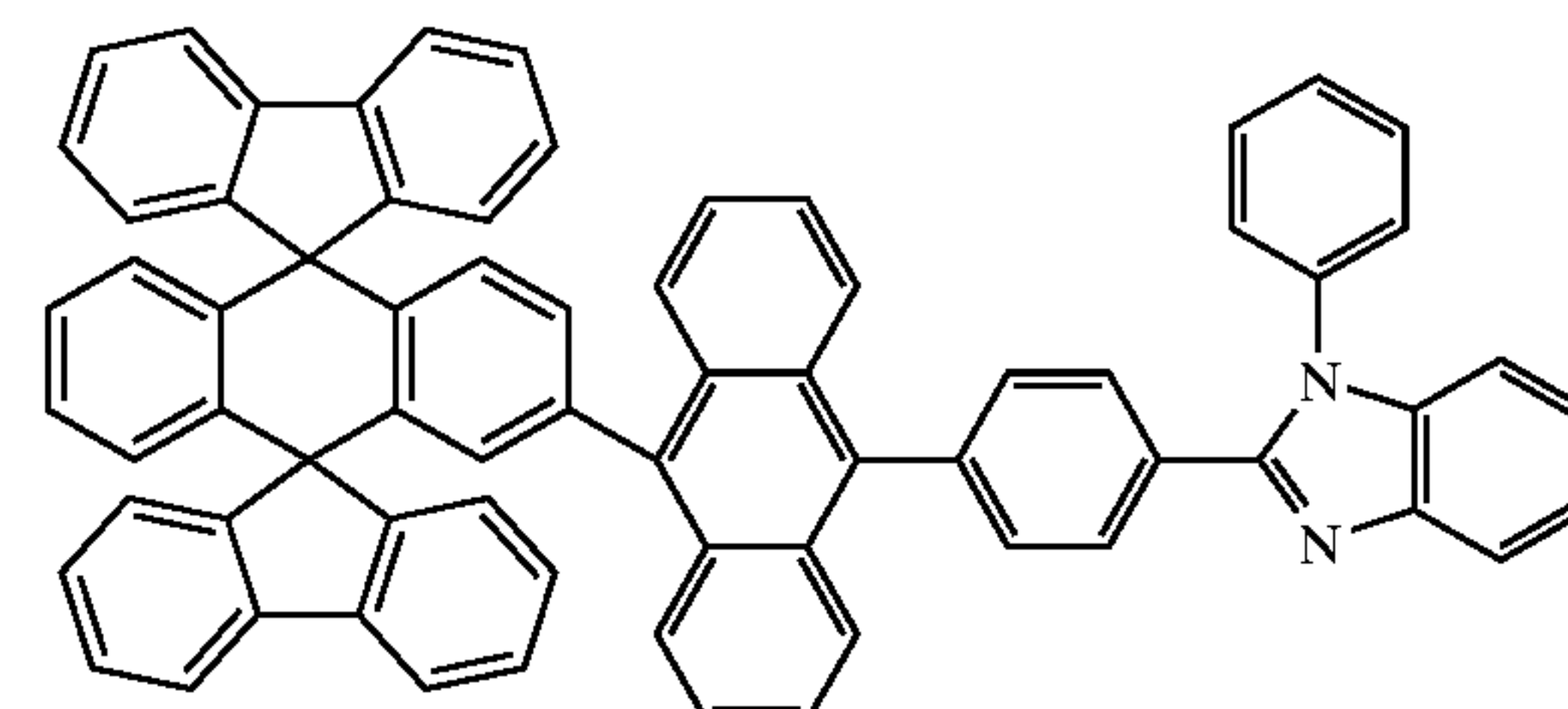
Chemical Compound 204
