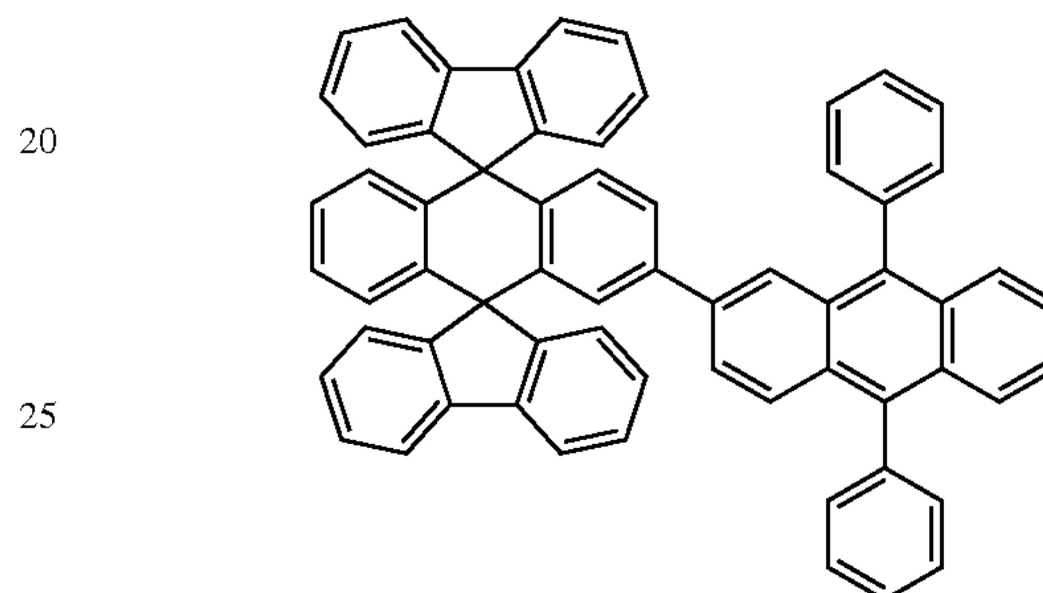
Chemical Compound 116
