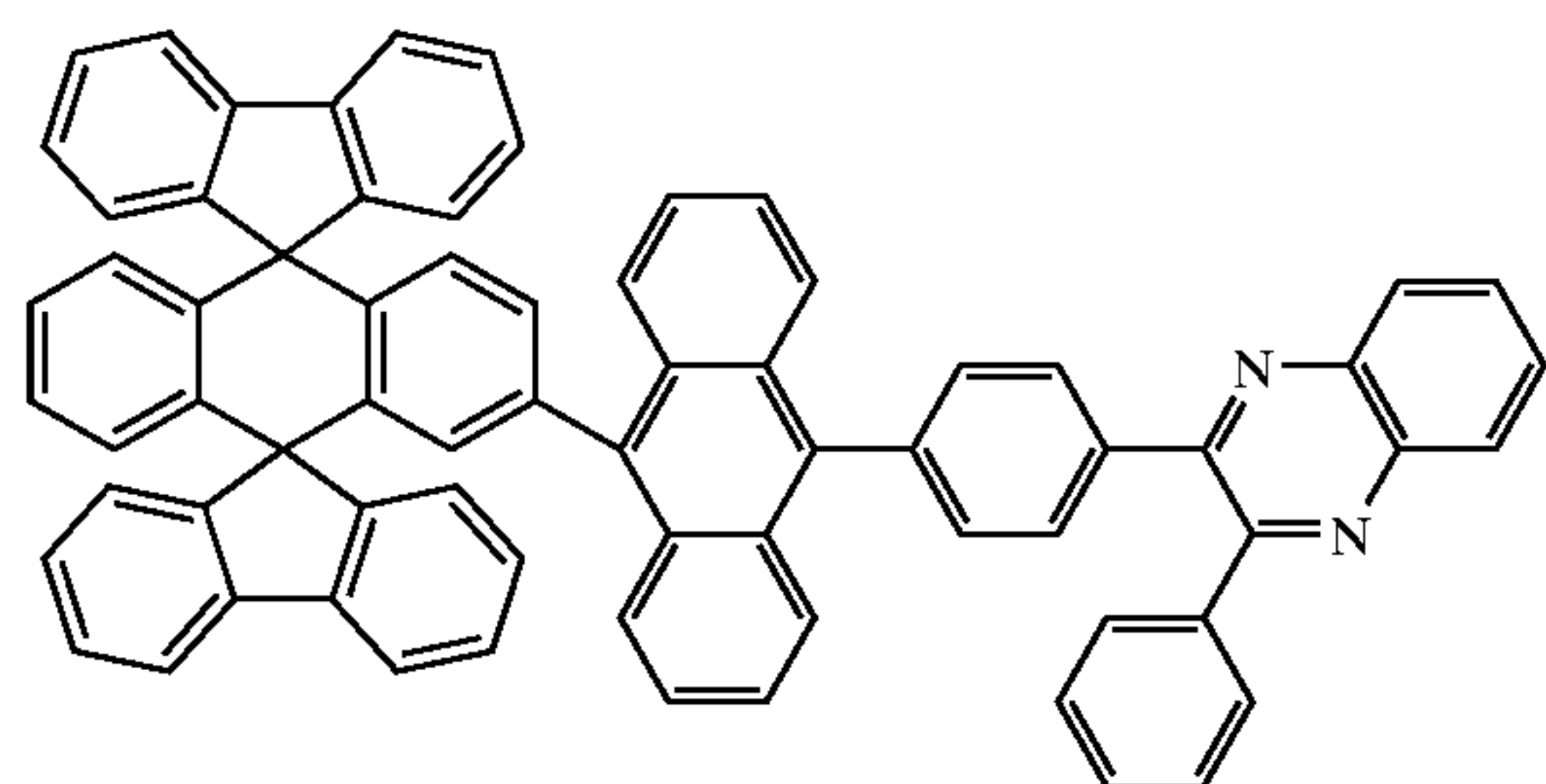
Chemical Compound 209
