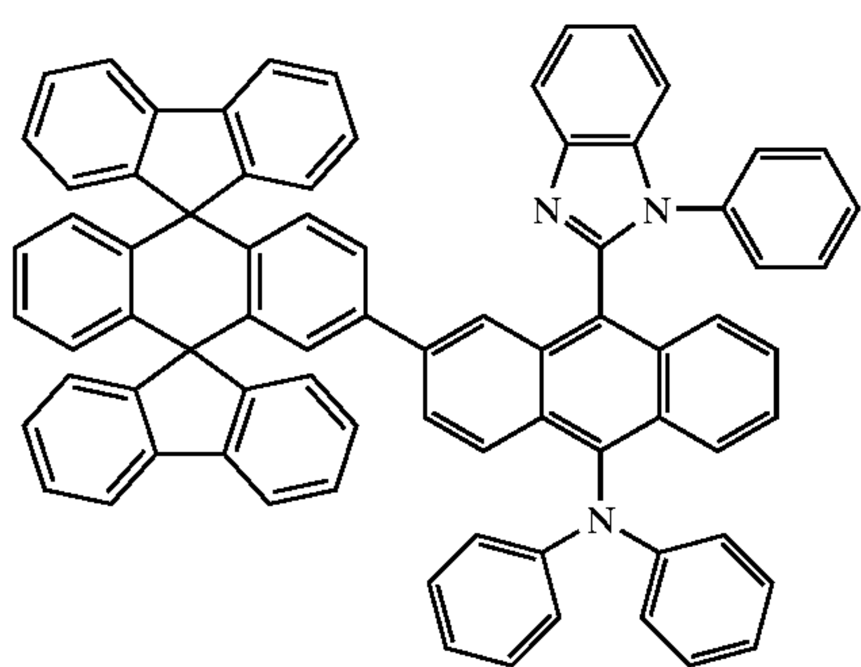
Chemical Compound 127
