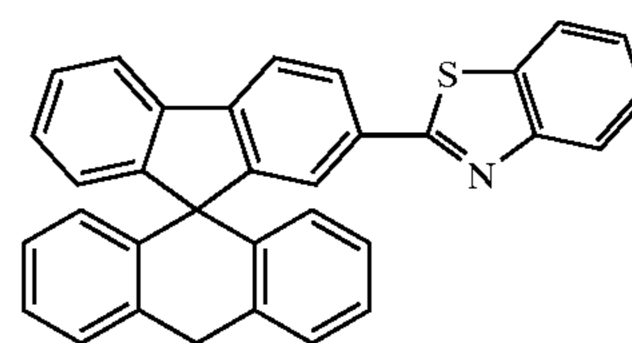
Chemical Compound 219
