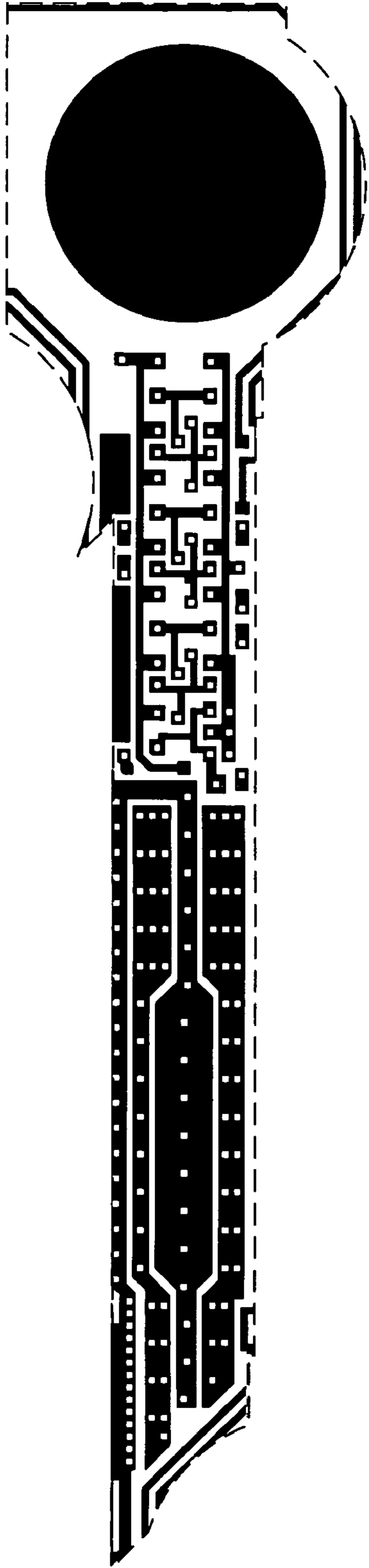
Metal 1 mask
