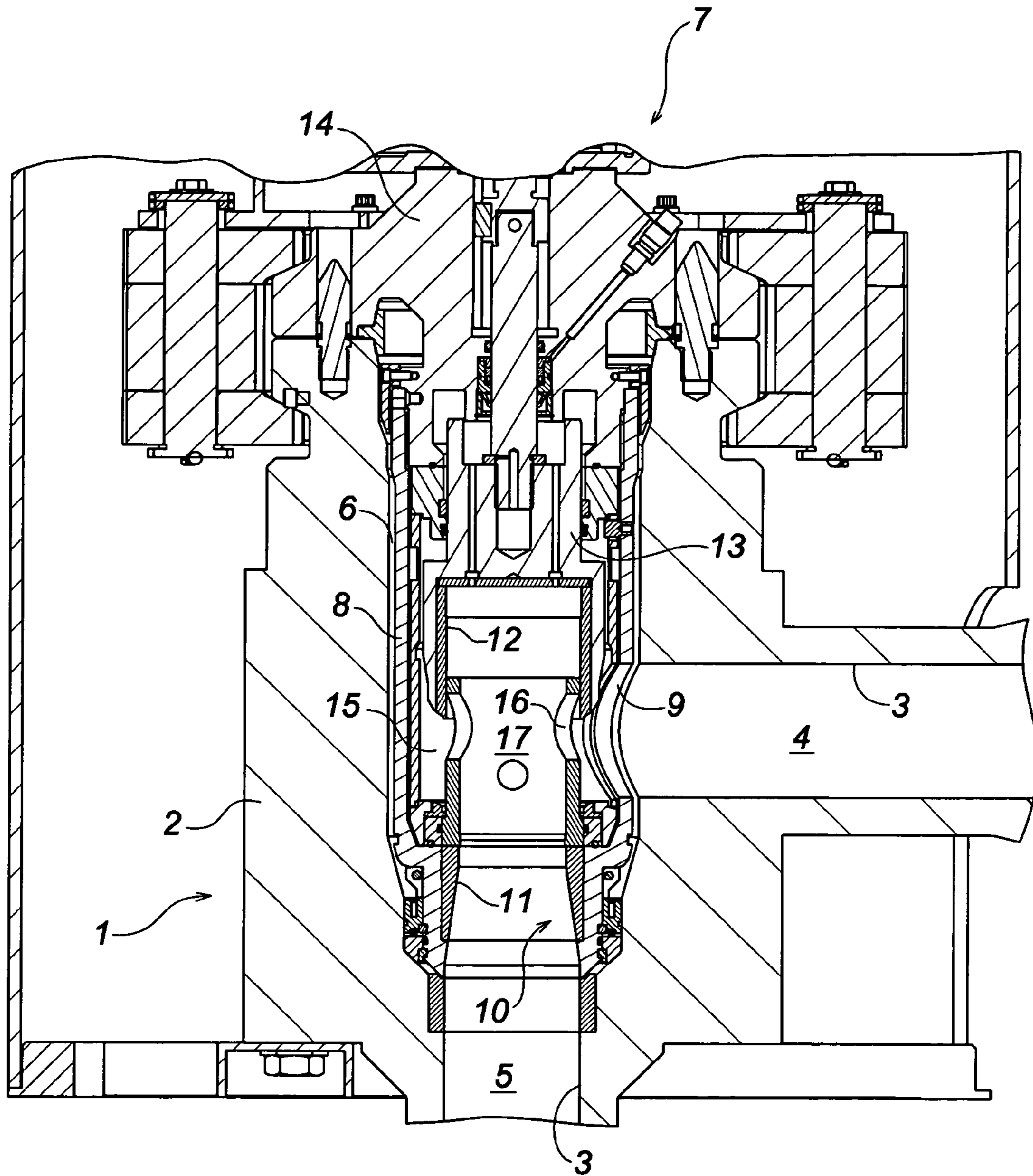
FIG. 1 (Prior Art)
