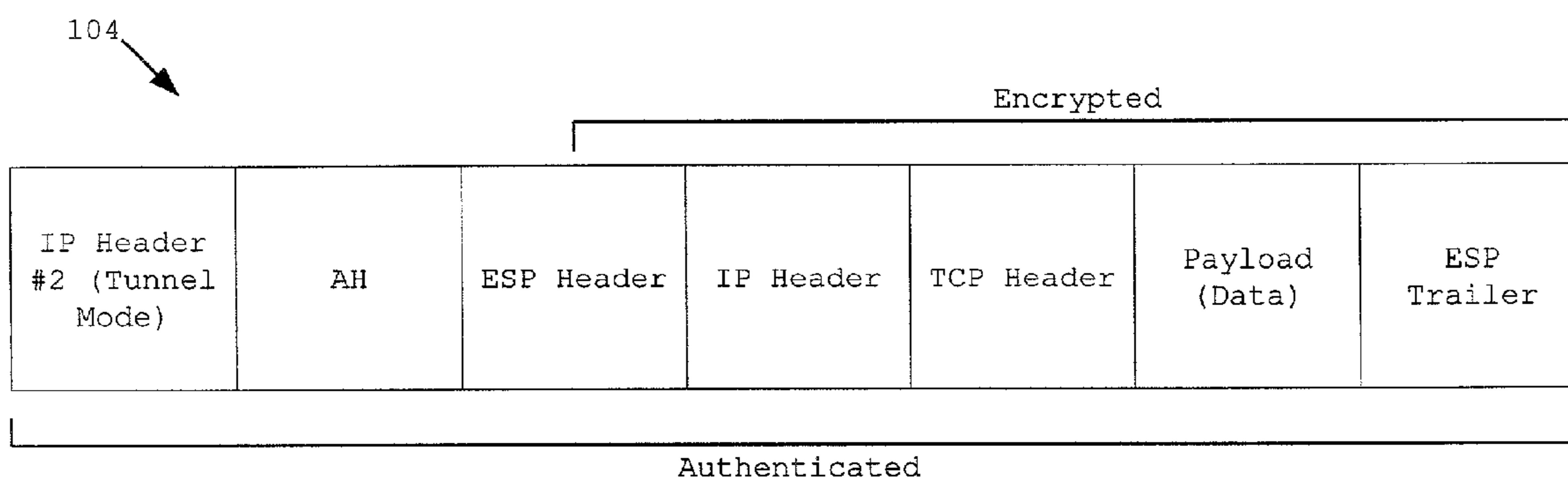
FIG. 1C (PRIOR ART)
