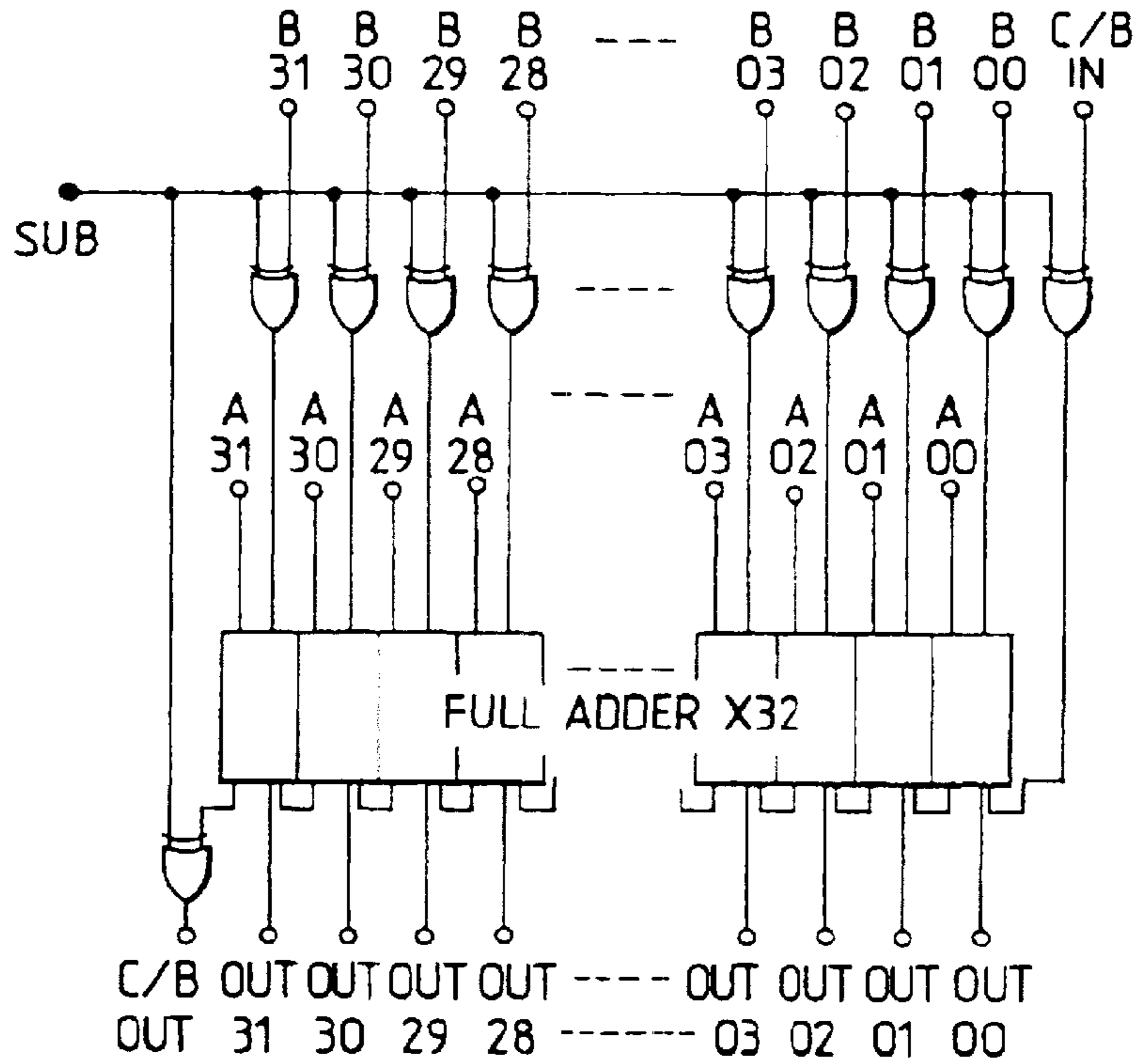
(a) ARITHMETIC LOGIC OPERATION CIRCUIT
