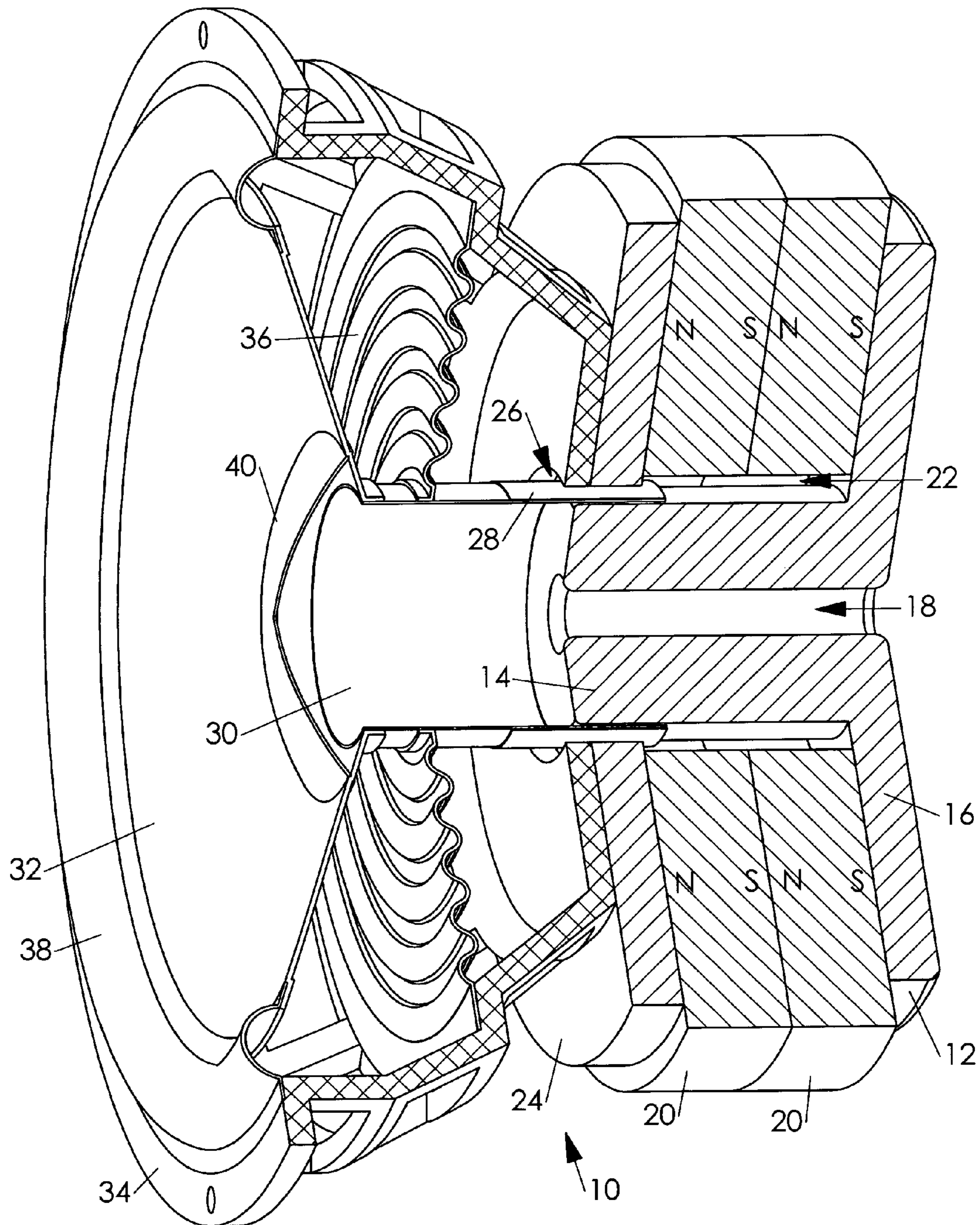
FIG. 1 - prior art
