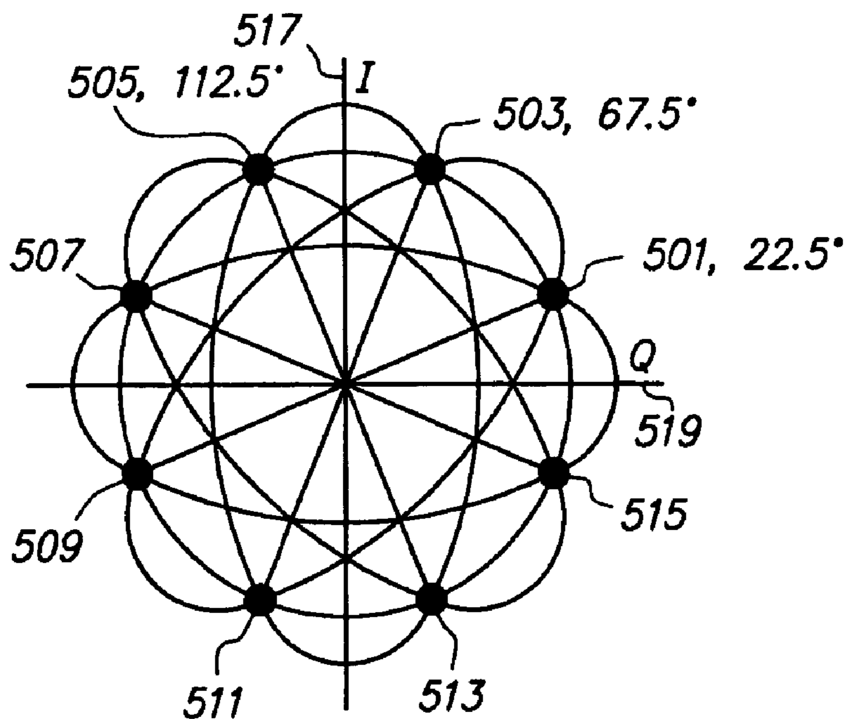
\pi/4 DQPSK Signal Trajectory
