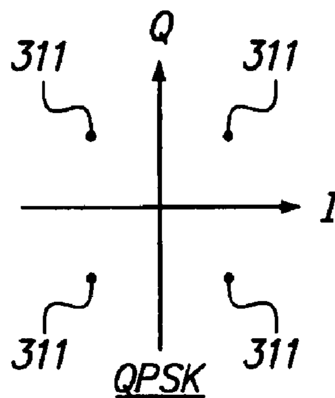
FIG. 3C (Prior Art)
