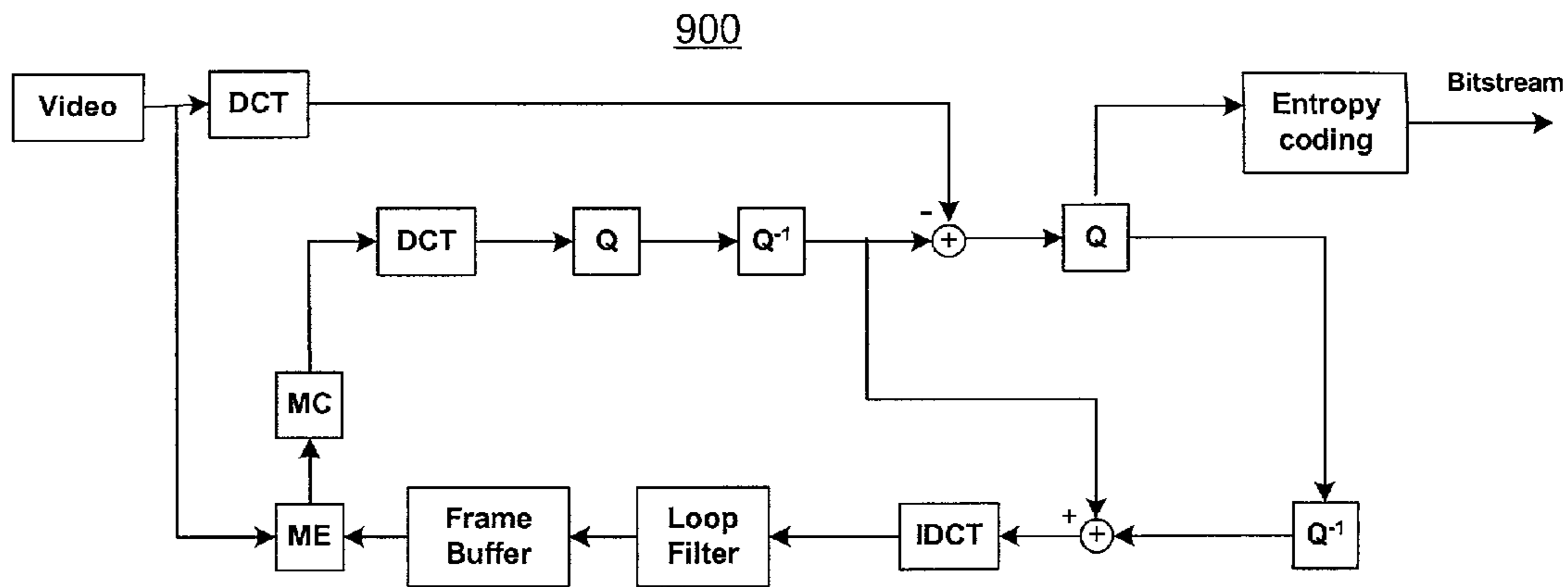
Fig. 9 (Prior Art)
