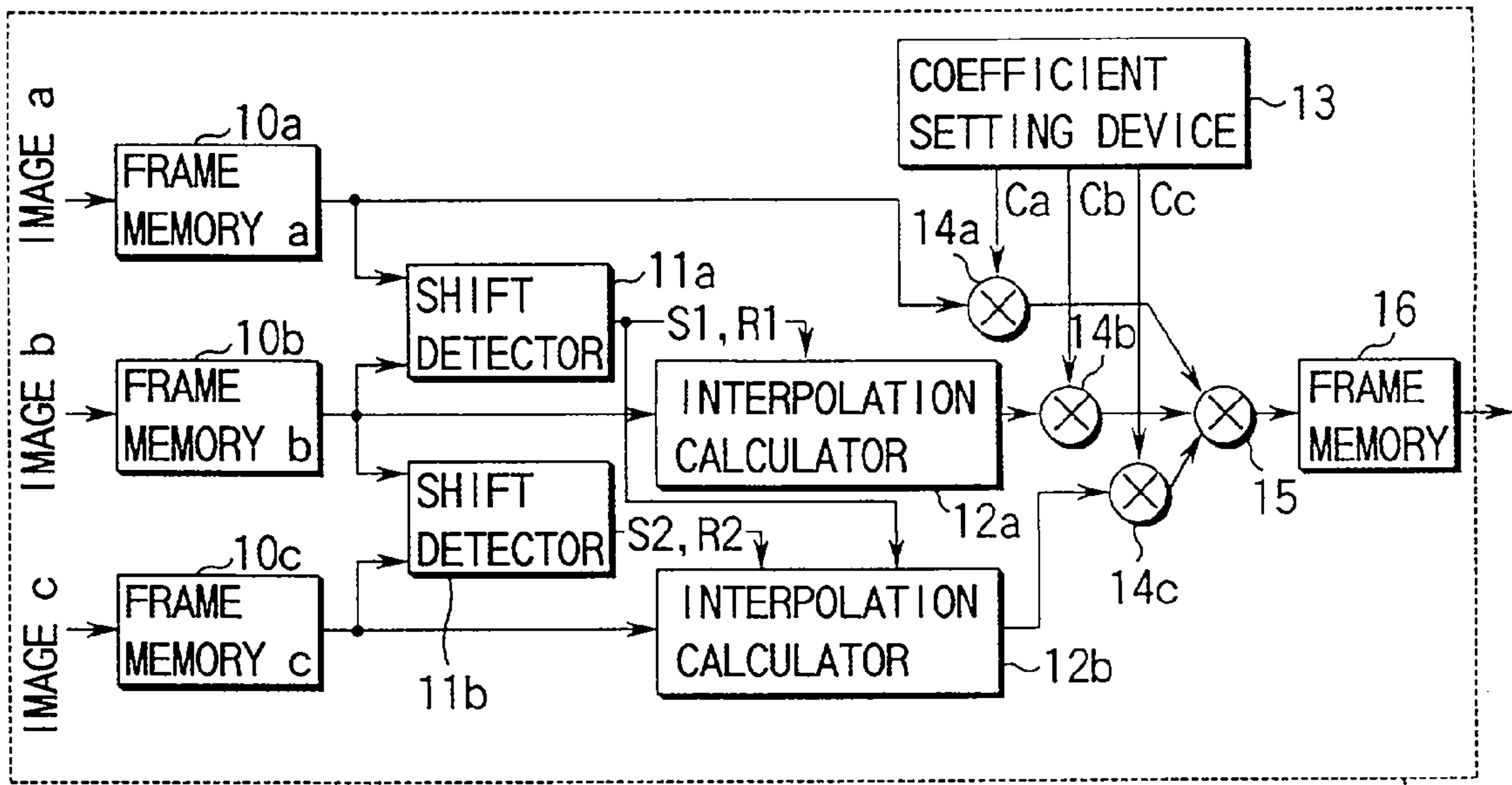
FIG. 19 PRIOR ART
