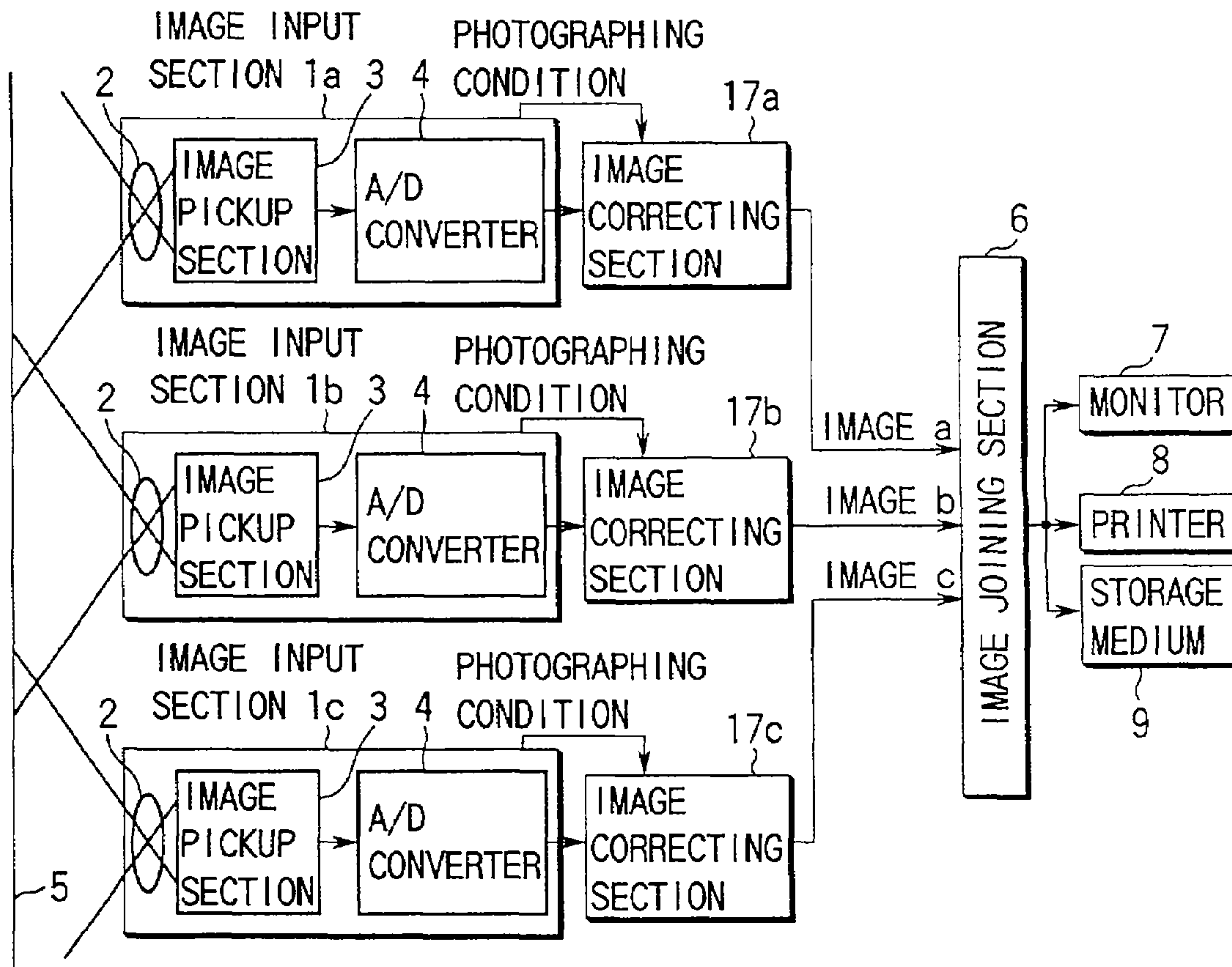
FIG. 18 PRIOR ART
