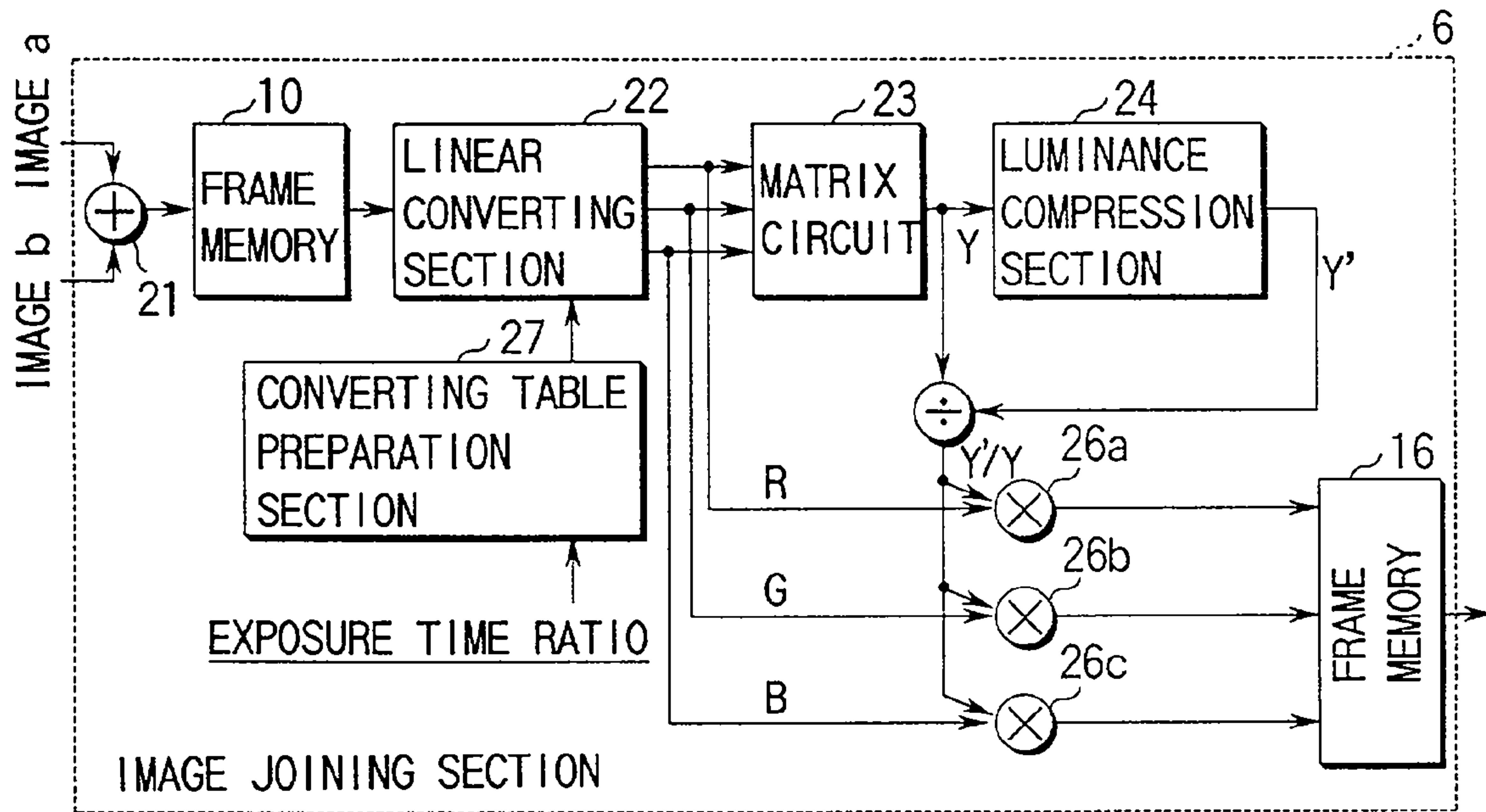
FIG. 22 PRIOR ART
