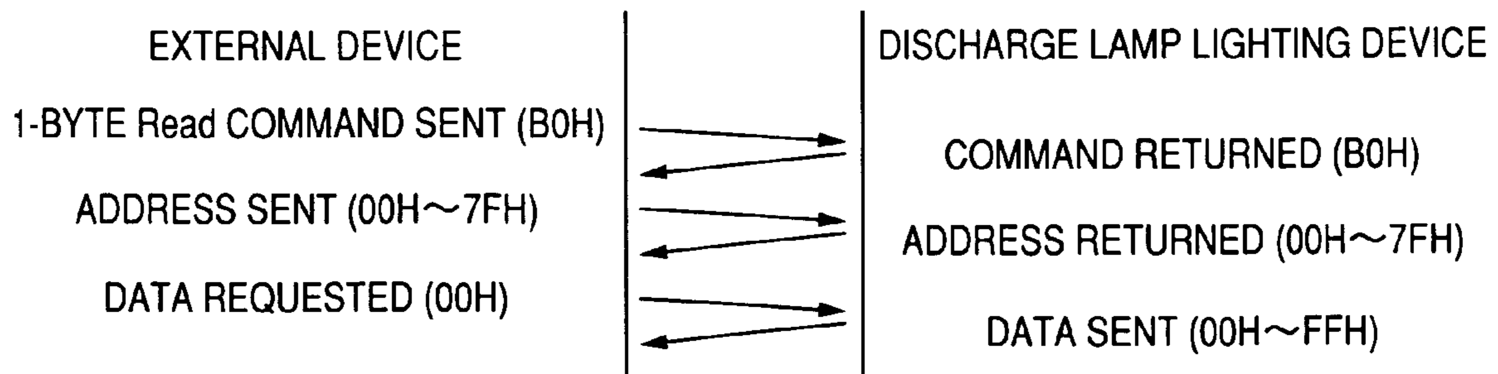
EEPROM DATA READING COMMAND (1-BYTE)
