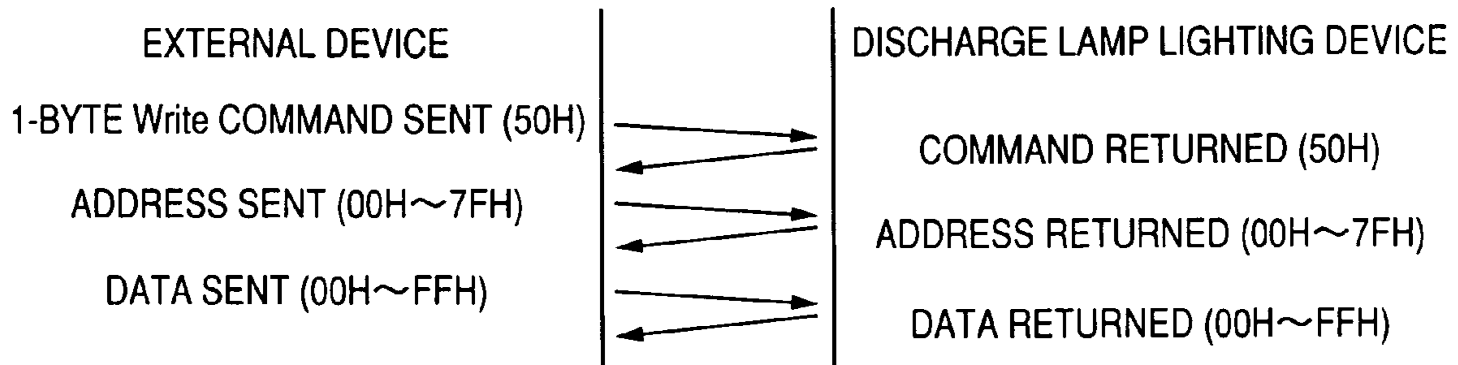
EEPROM DATA WRITING COMMAND (1-BYTE)
