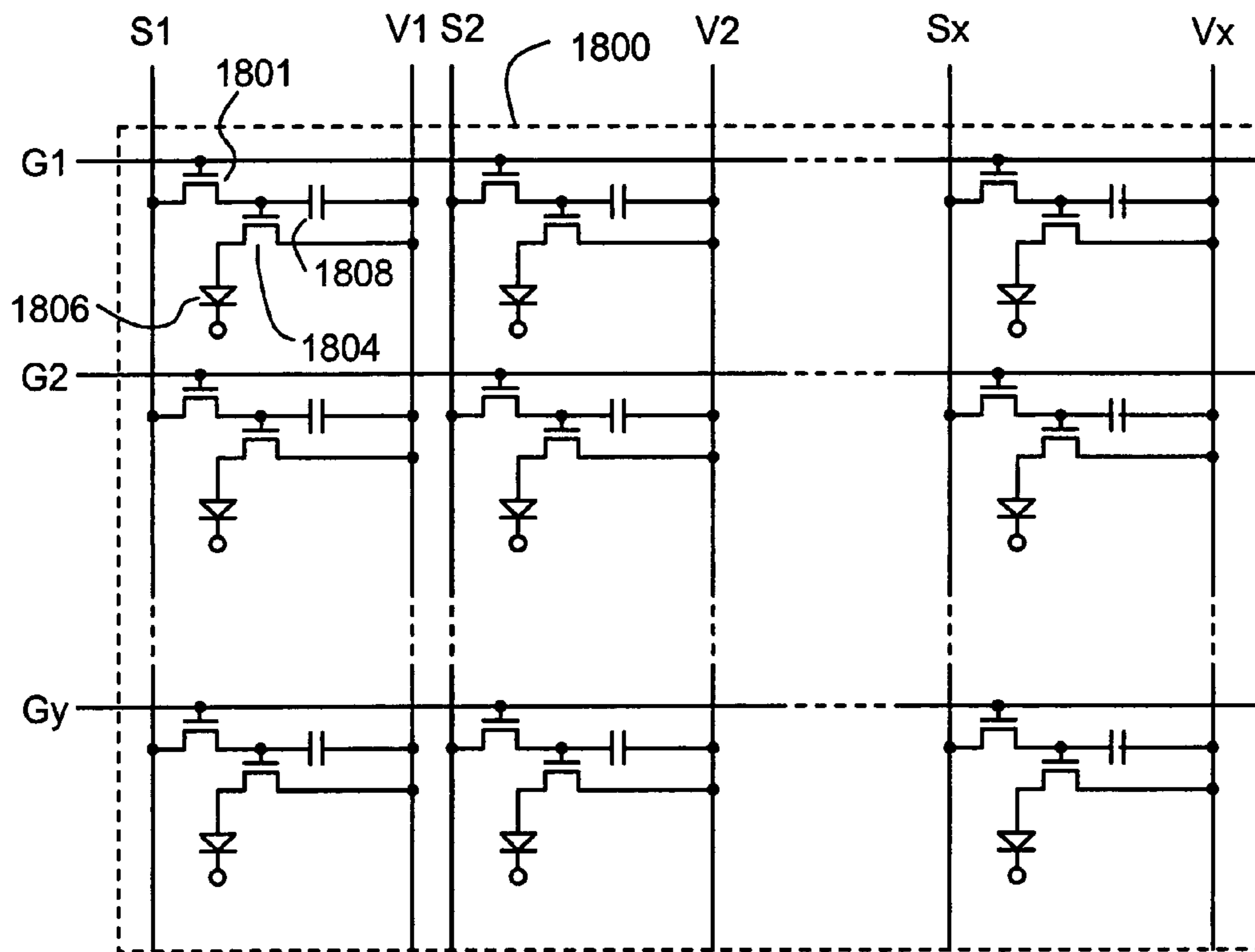
FIG. 25 PRIOR ART
