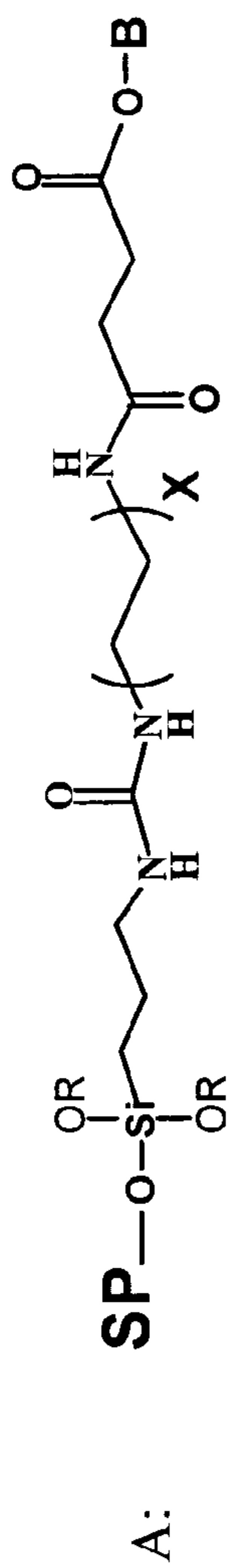
Figure 8. General Chemical formulae for Spacers
