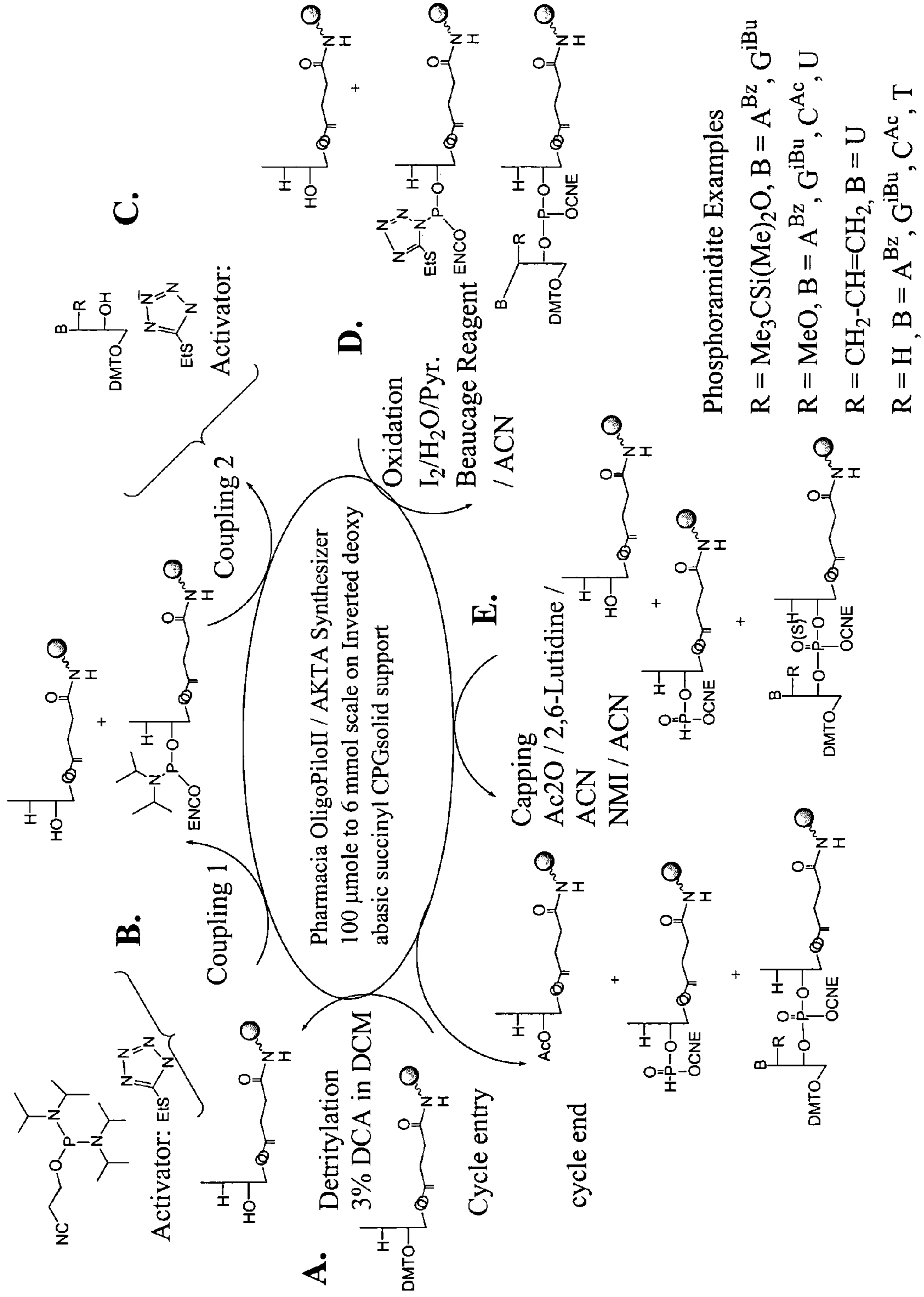
Figure 11: Chemical Synthesis of Oligonucleotides, in situ Phosphoramidite
