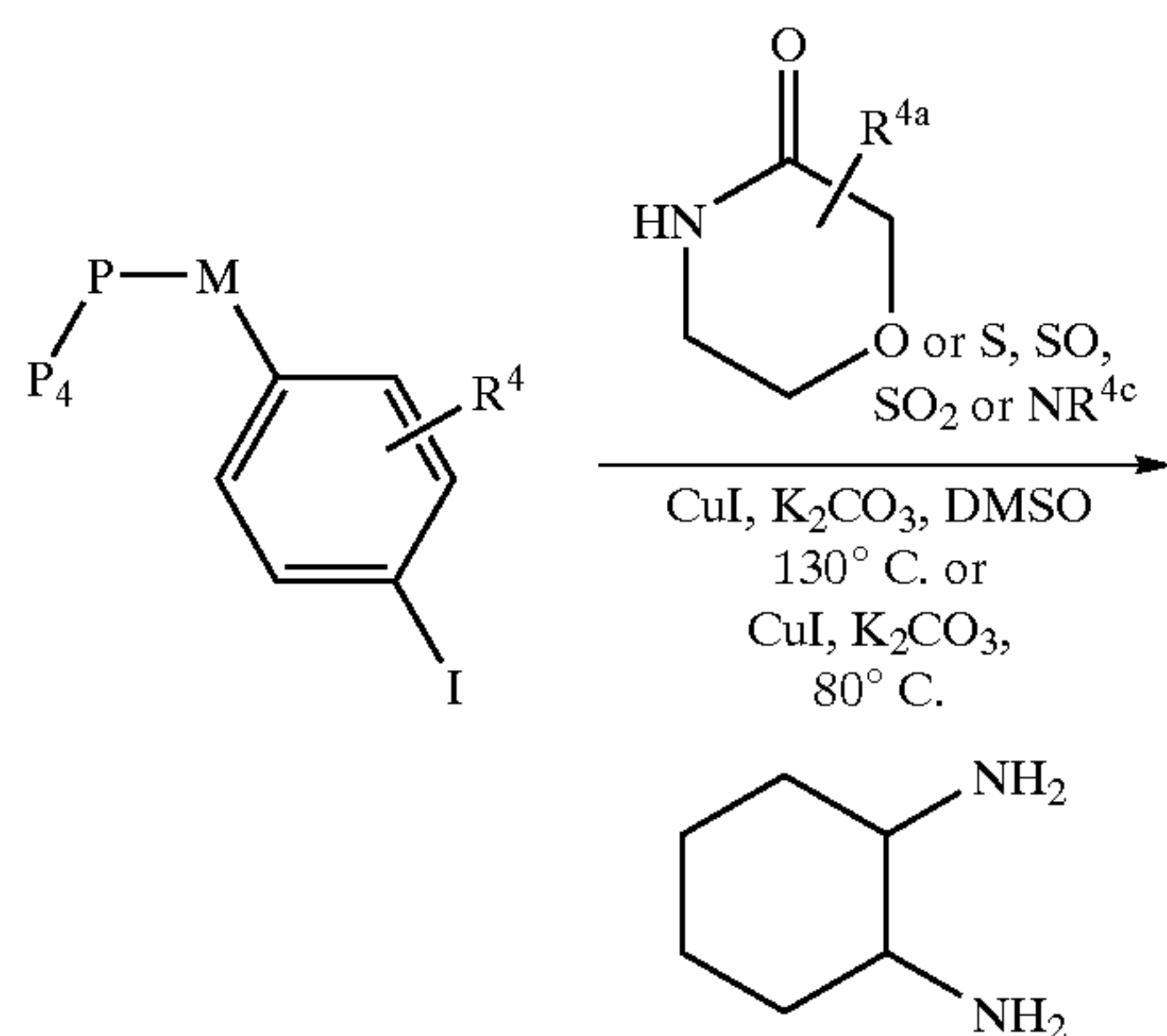
Scheme 11
