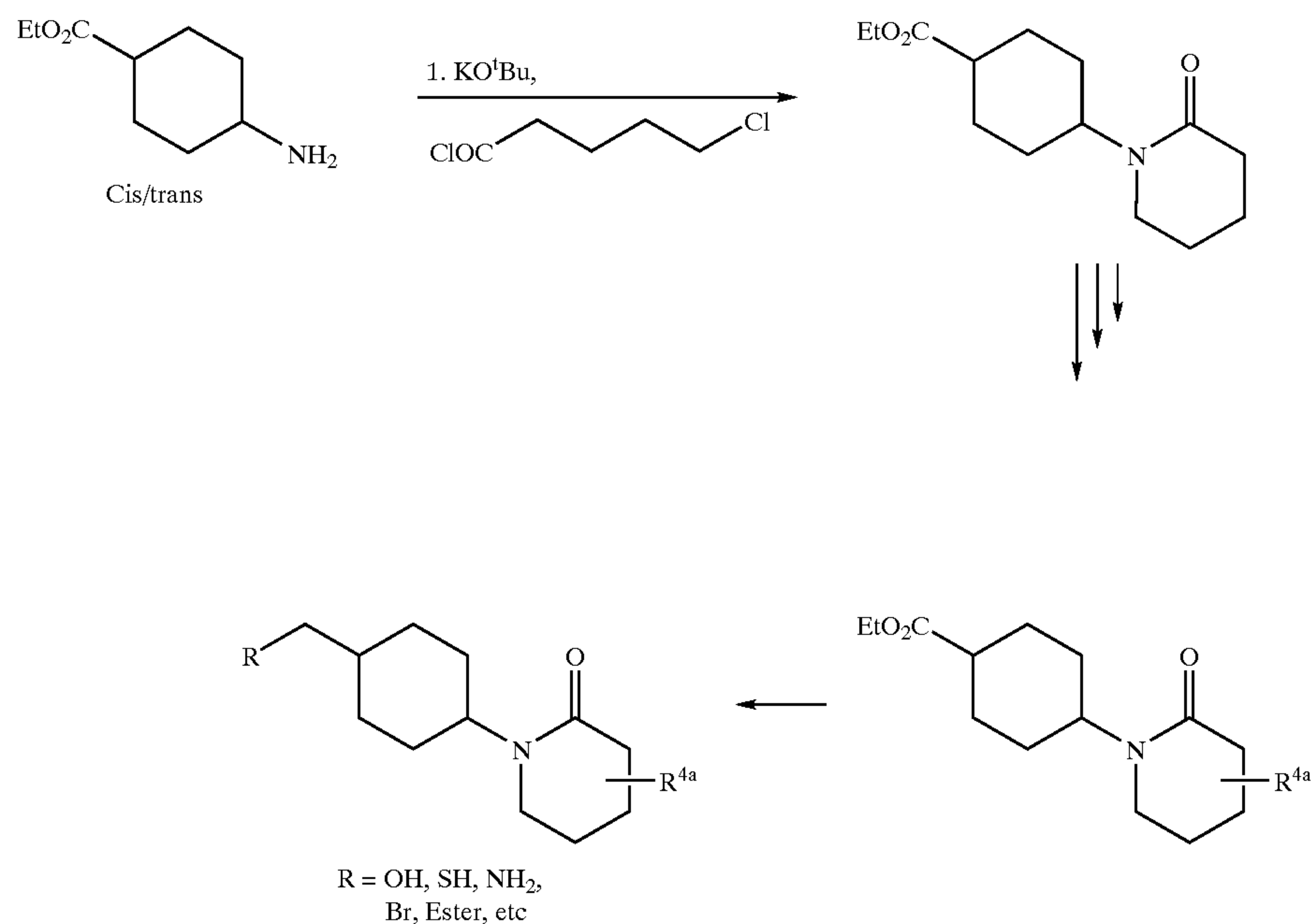
Scheme 9
