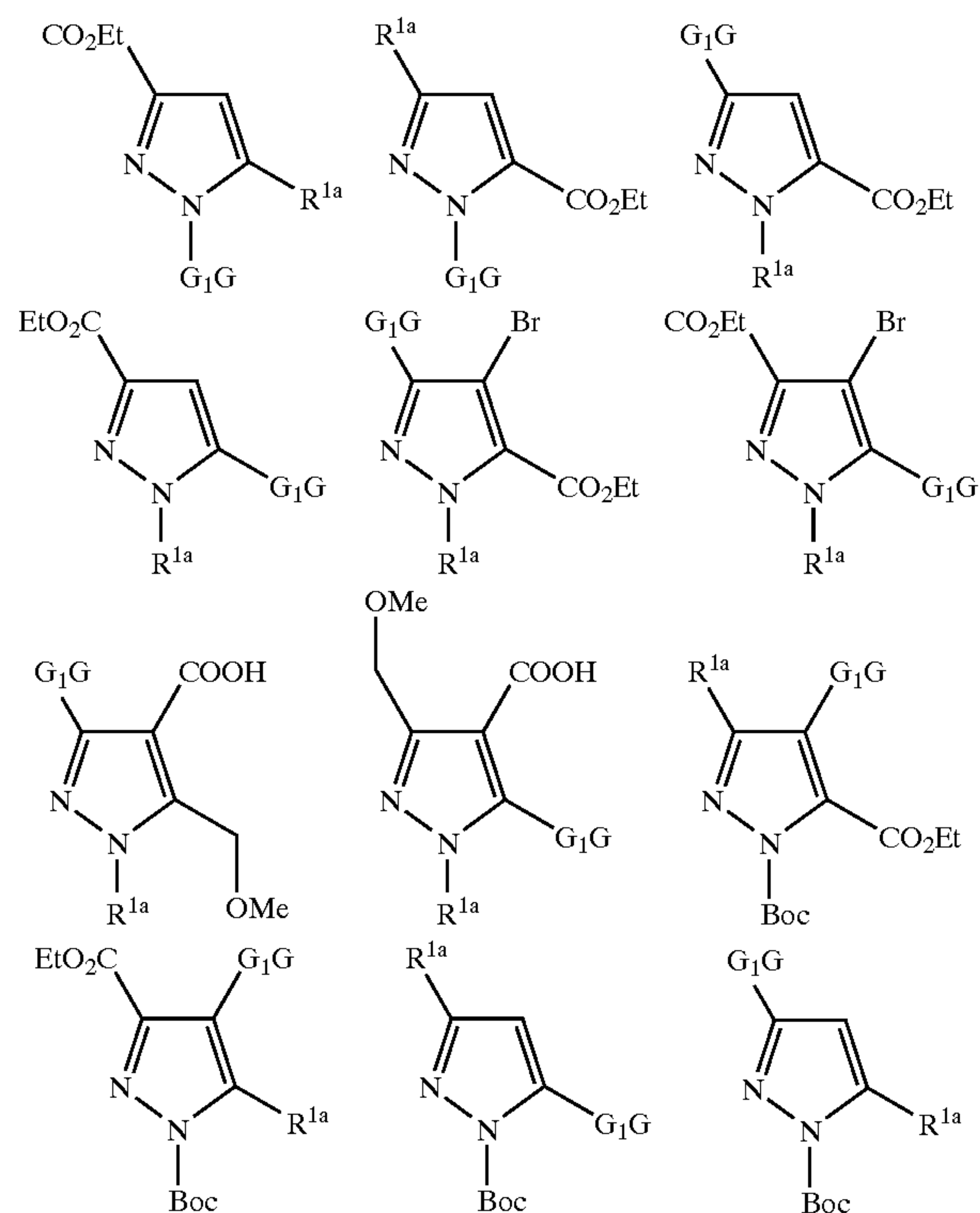
Scheme 16
