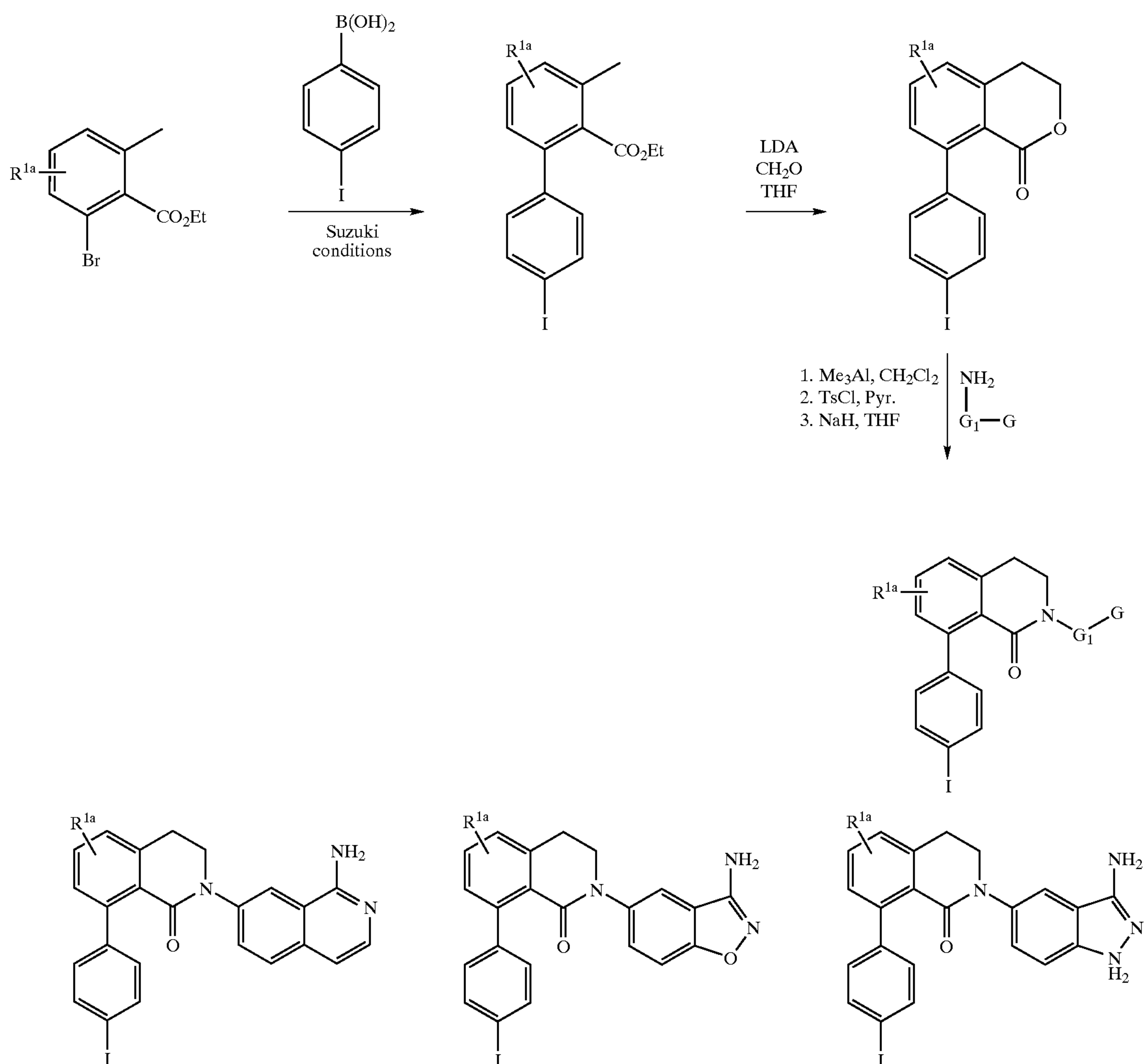
Scheme 26
