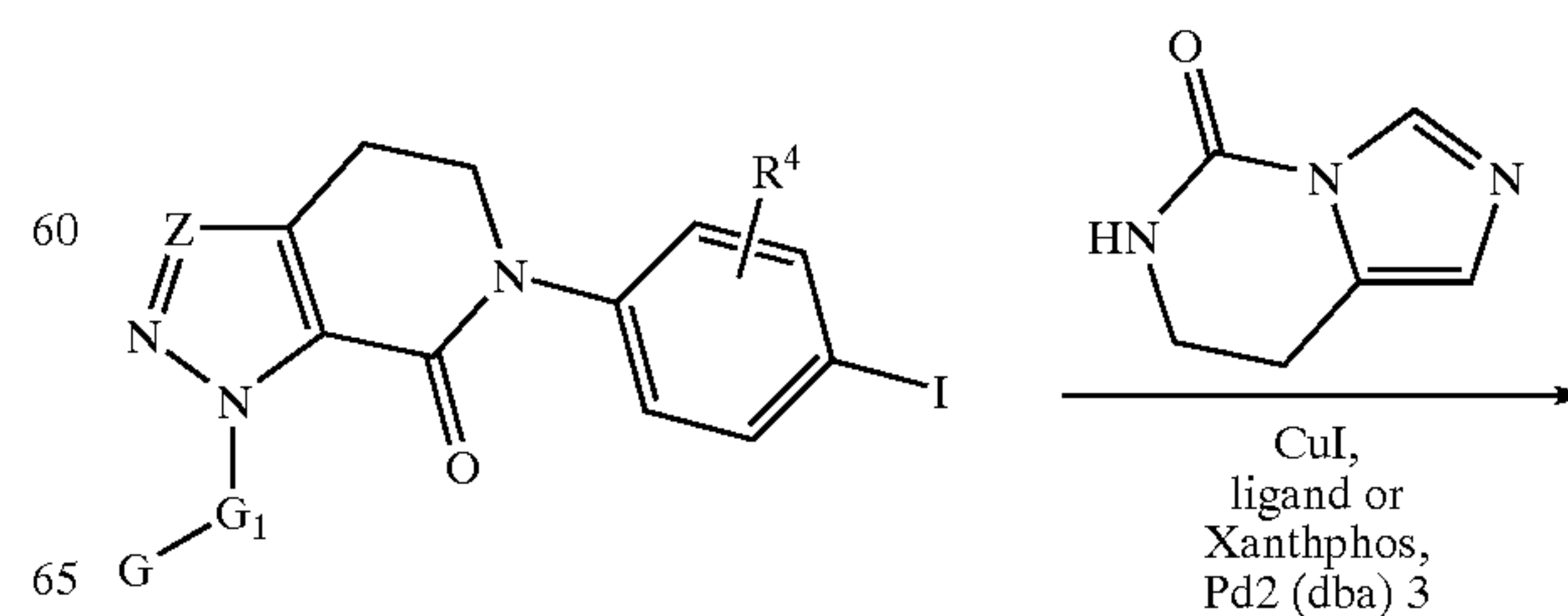
Scheme 13
