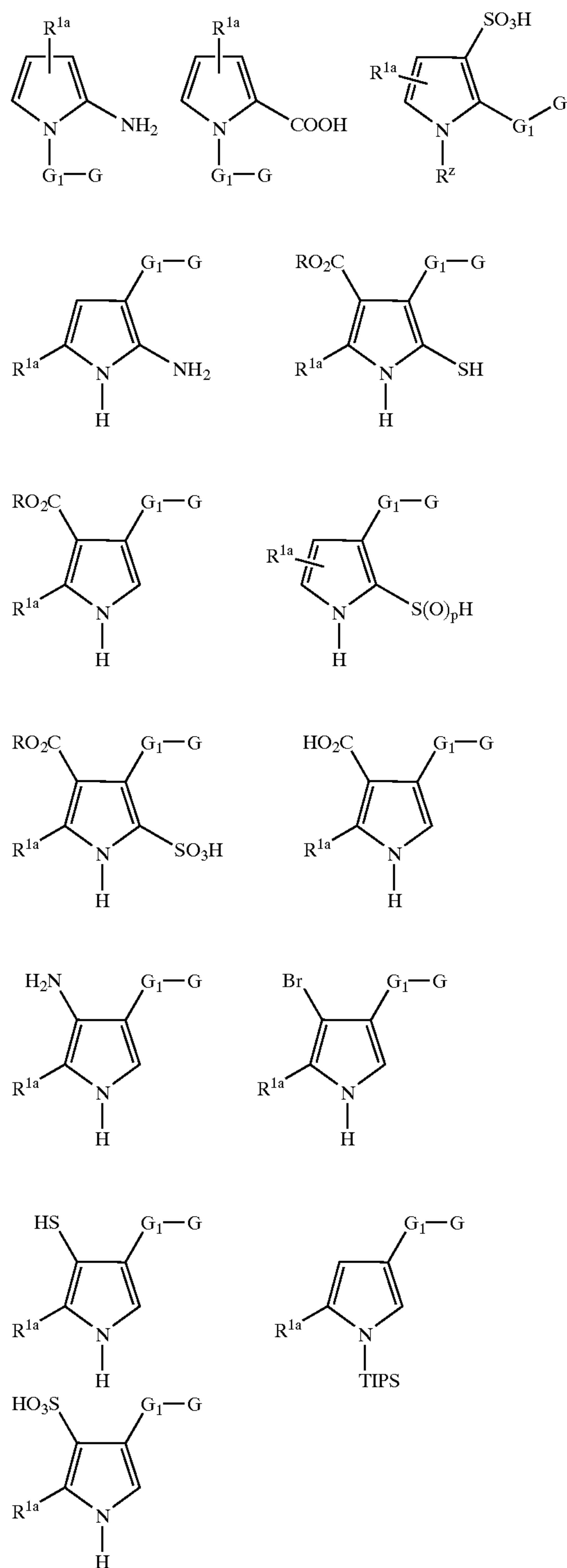
Scheme 14
