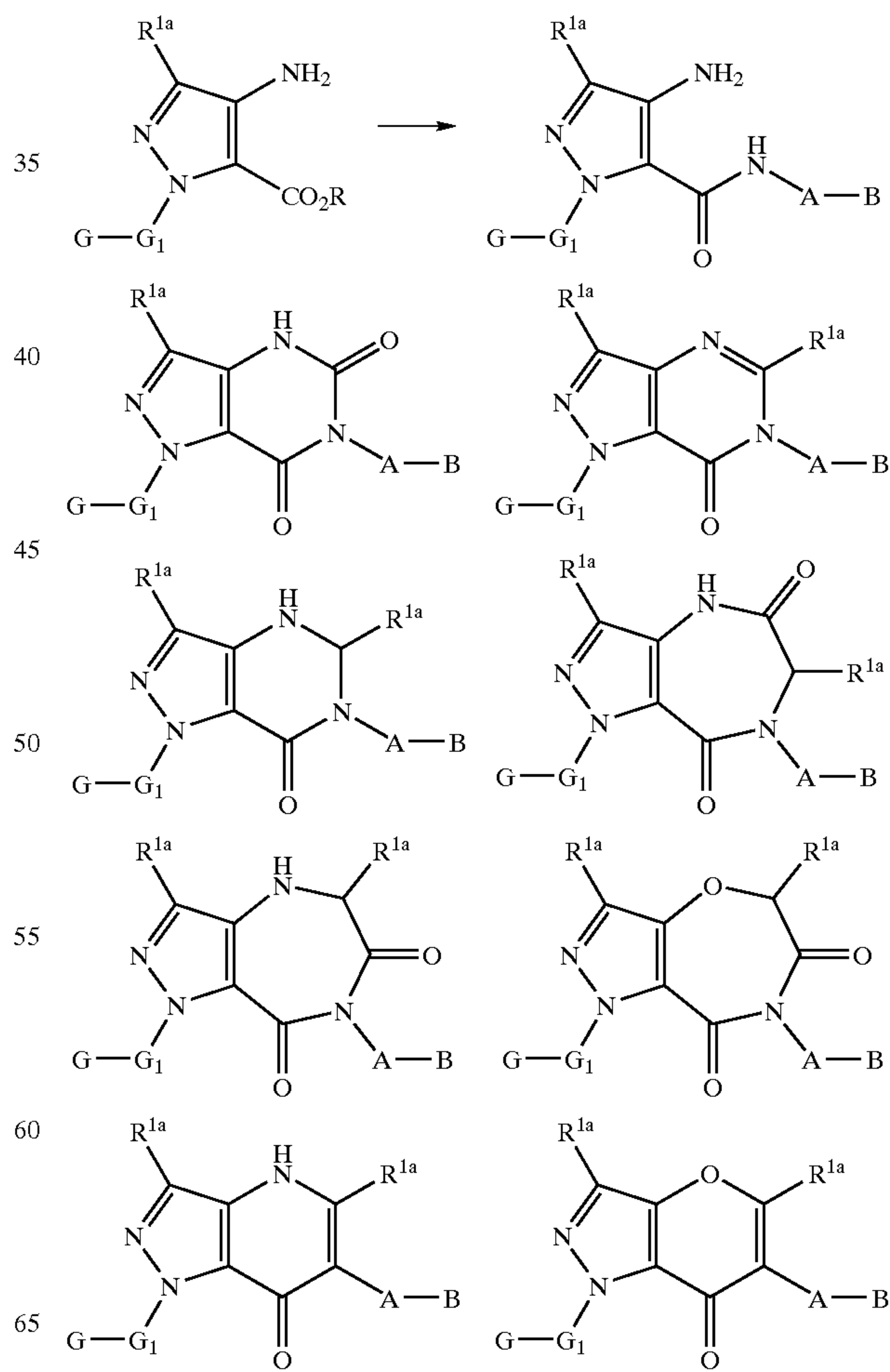
Scheme 18
