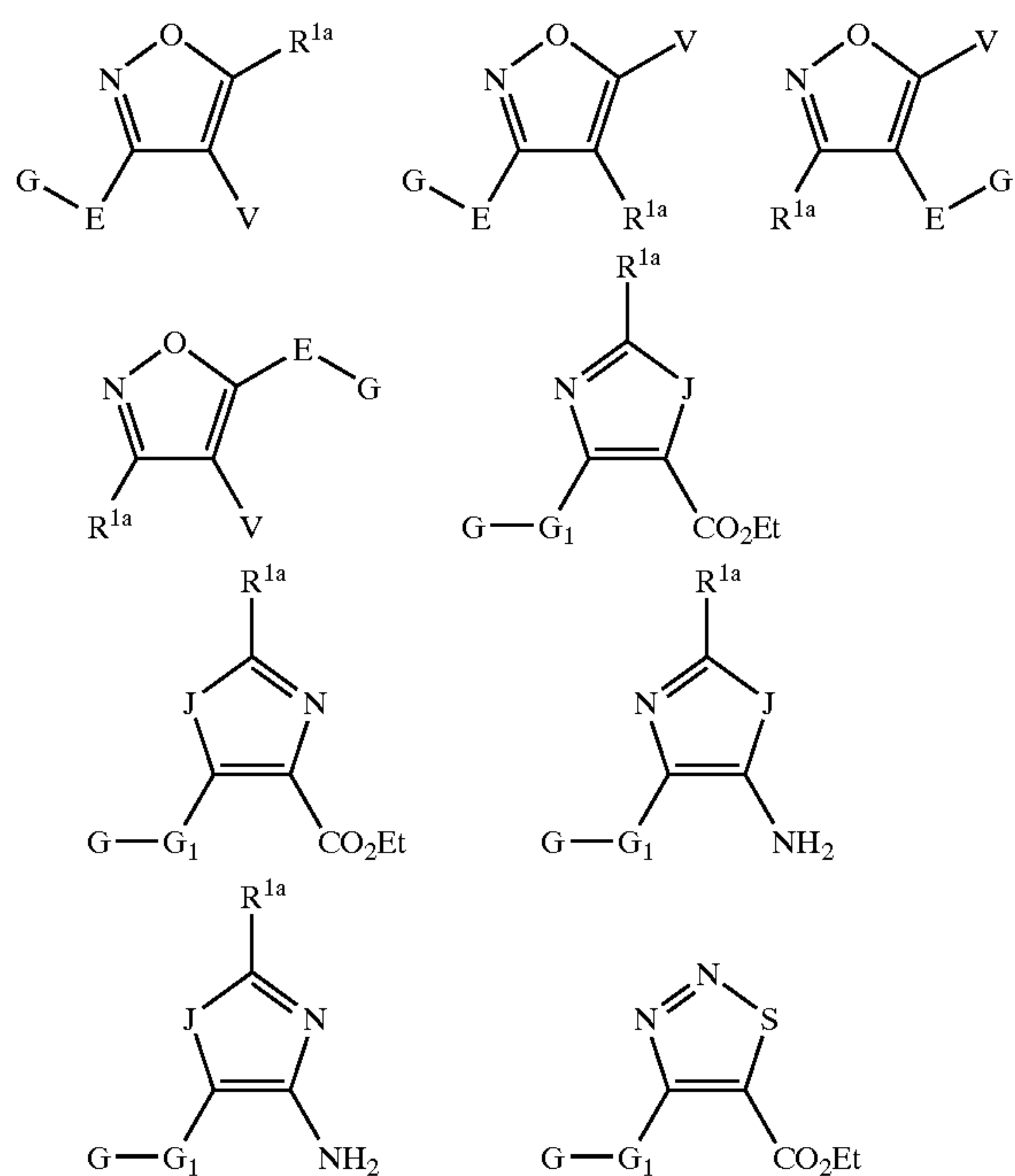
Scheme 17
