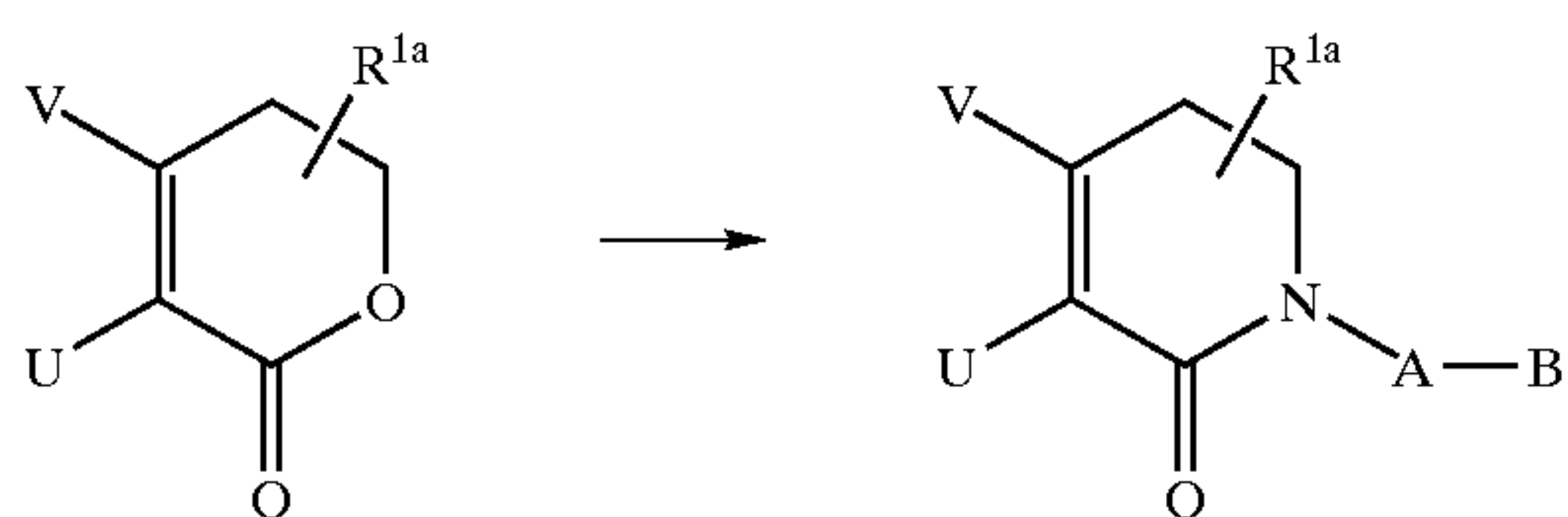
Scheme 19
