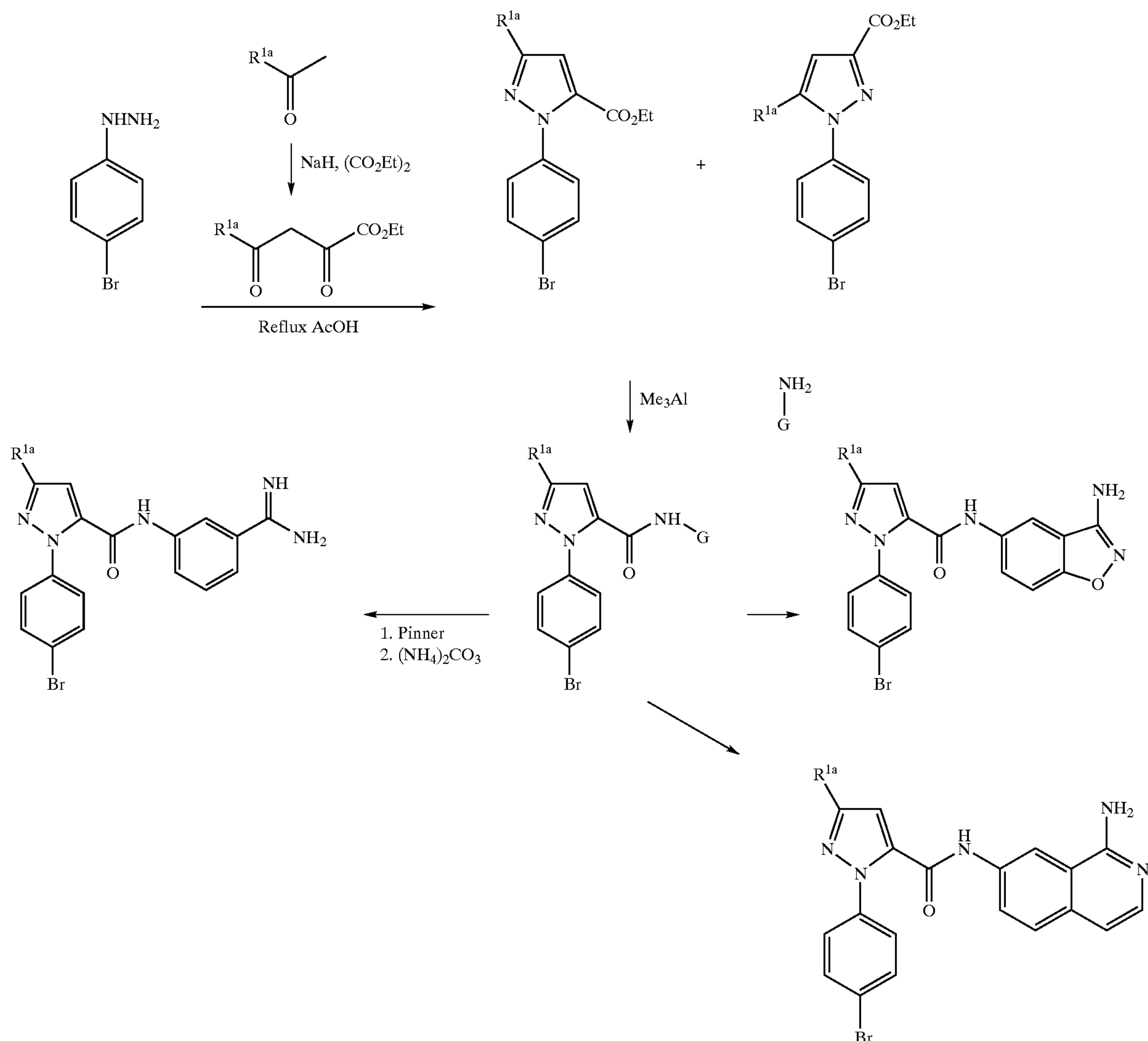
Scheme 22
