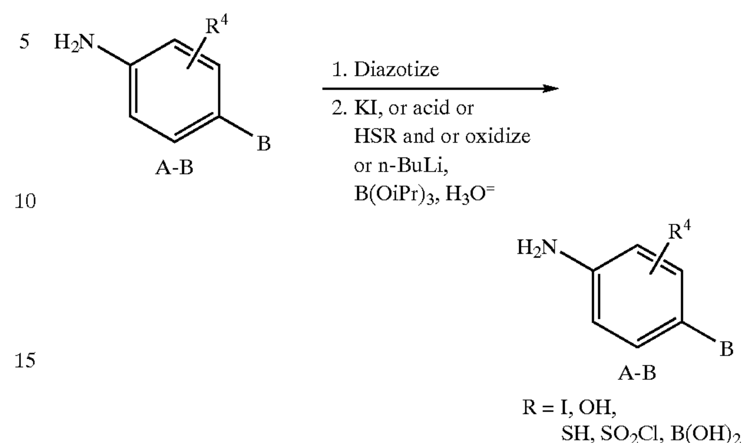
Scheme 6
