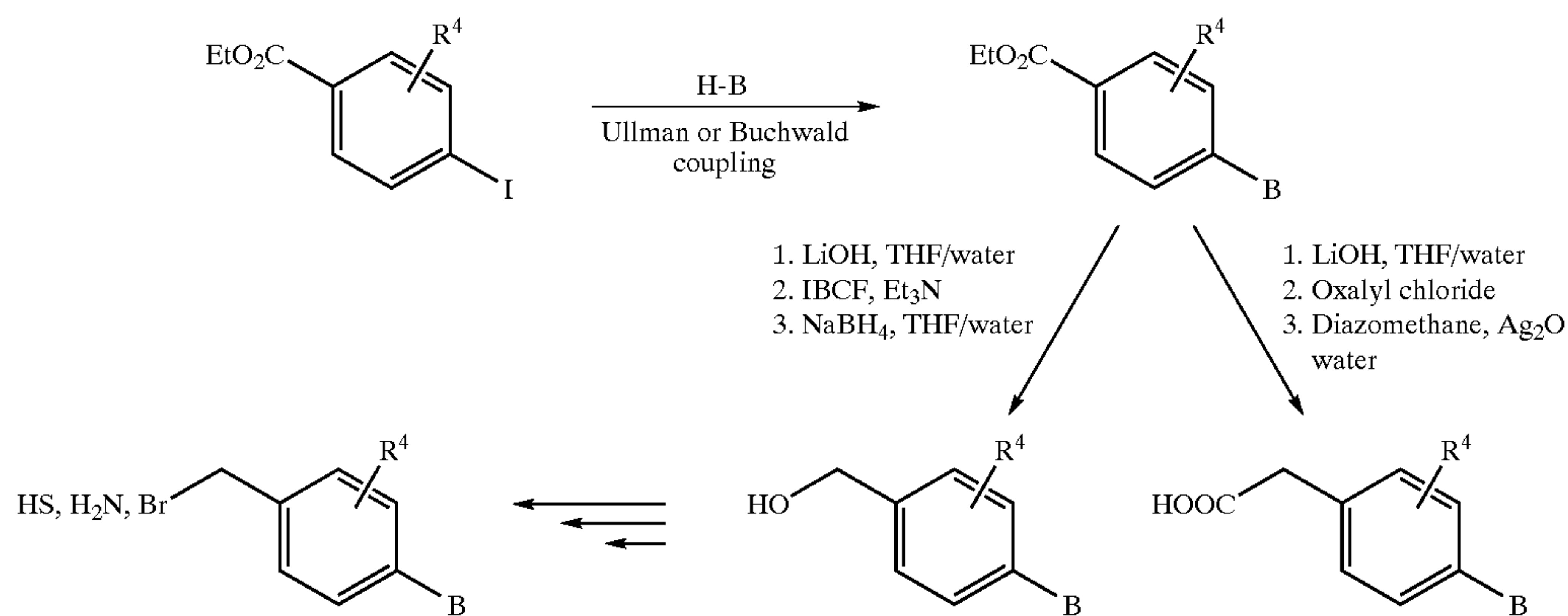
Scheme 7
