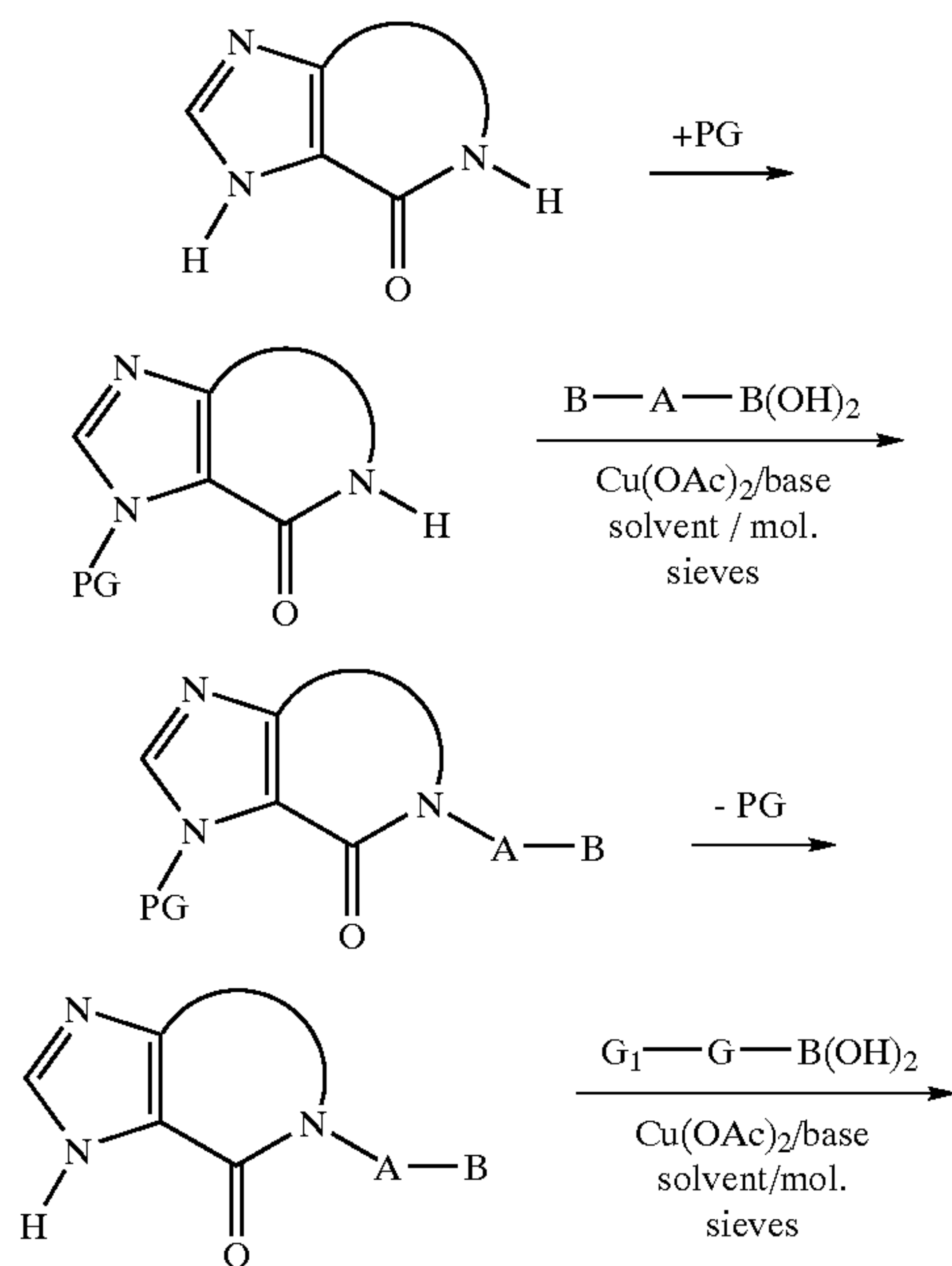
Scheme 21
