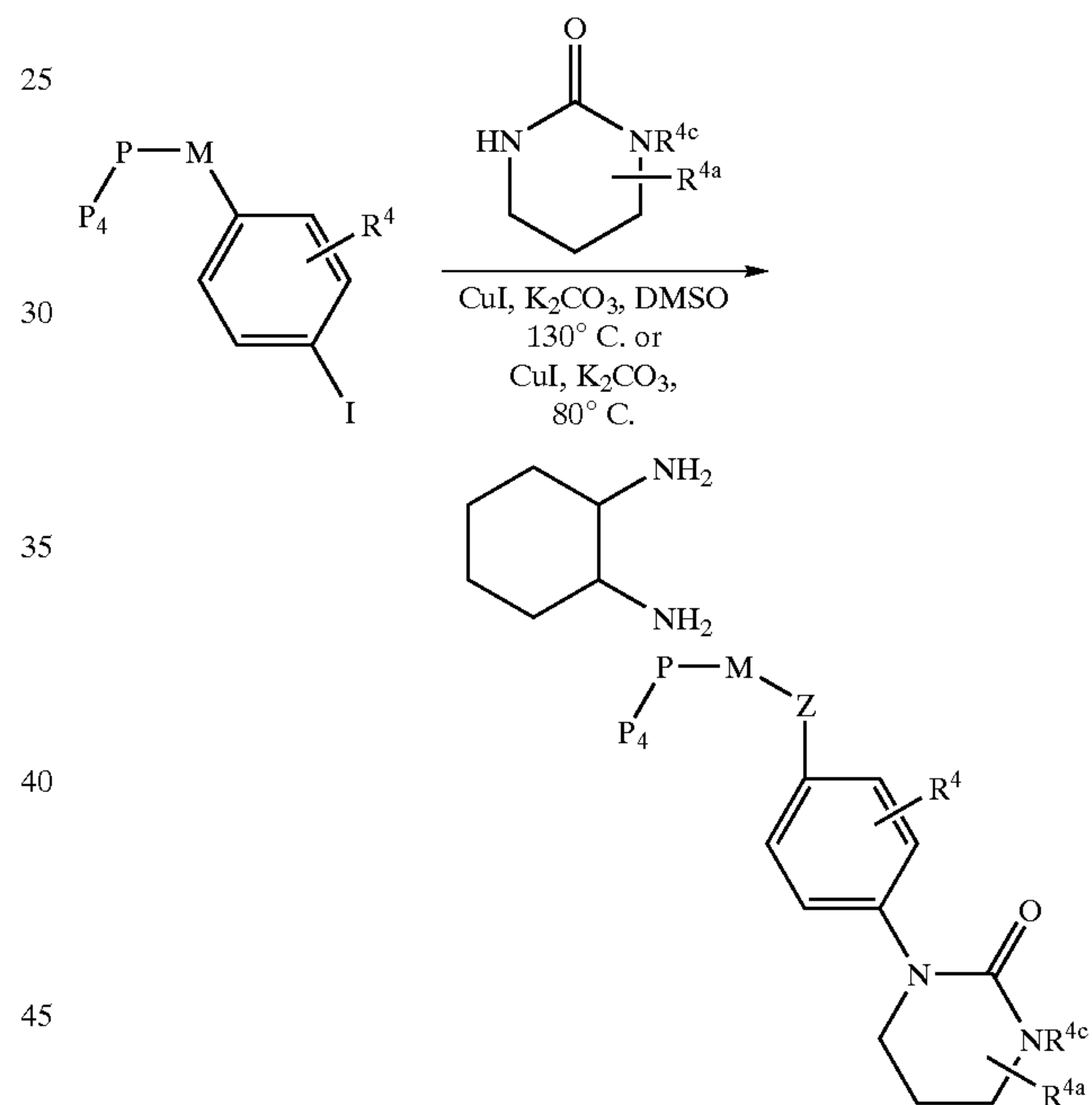
Scheme 12
