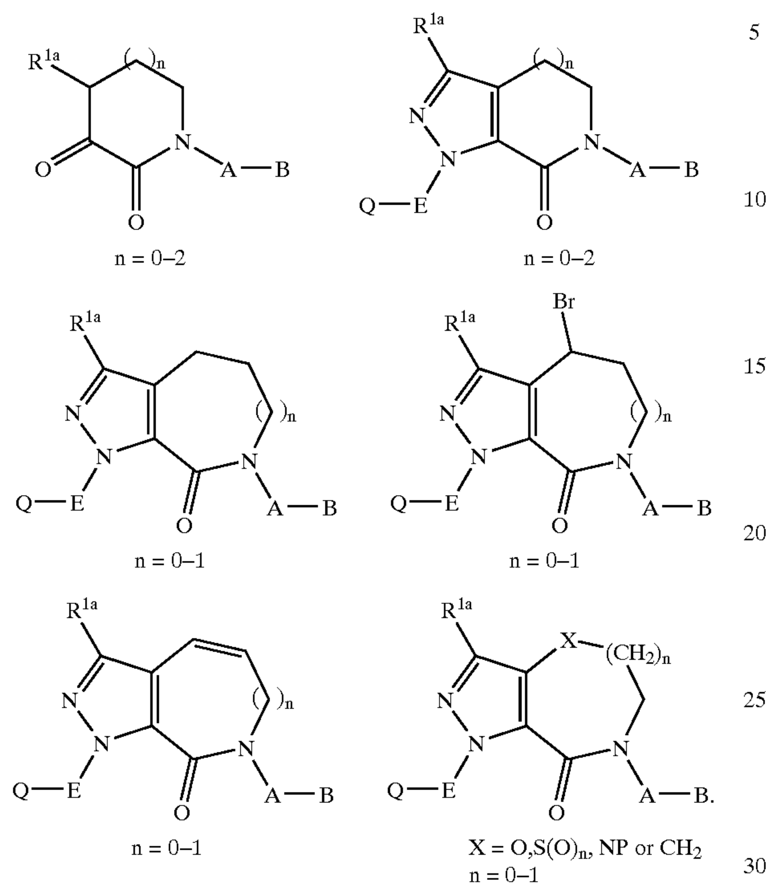
Scheme 20
