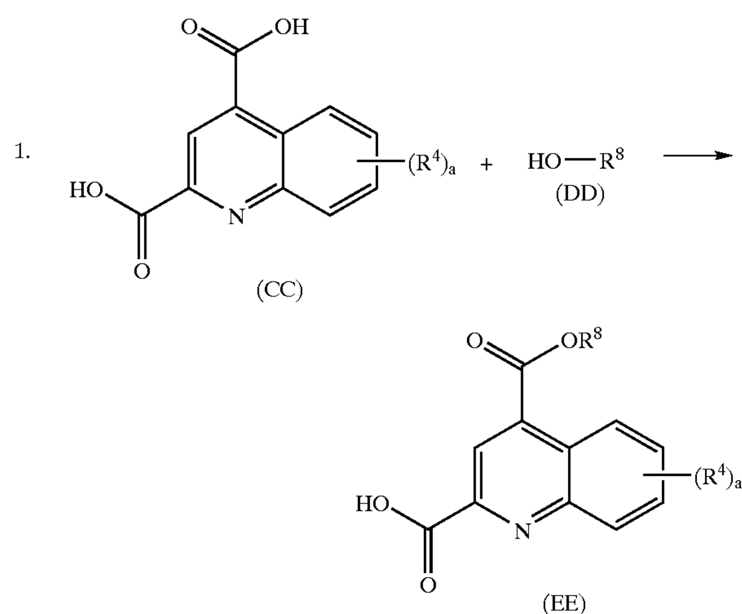
REACTION SCHEME 13
