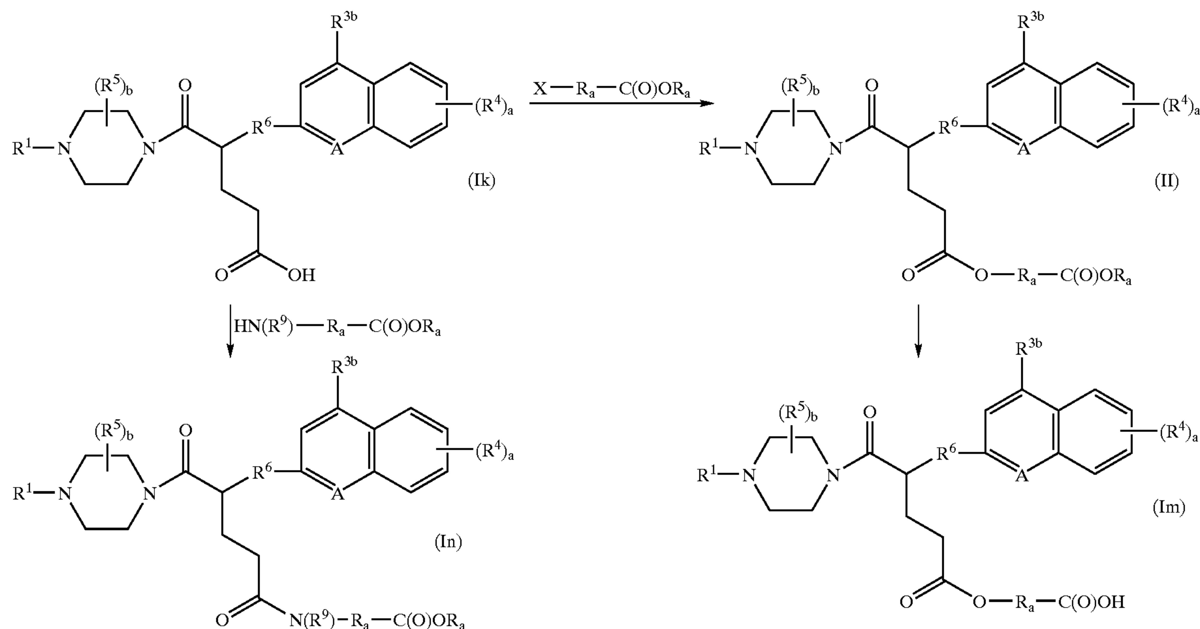
REACTION SCHEME 7
