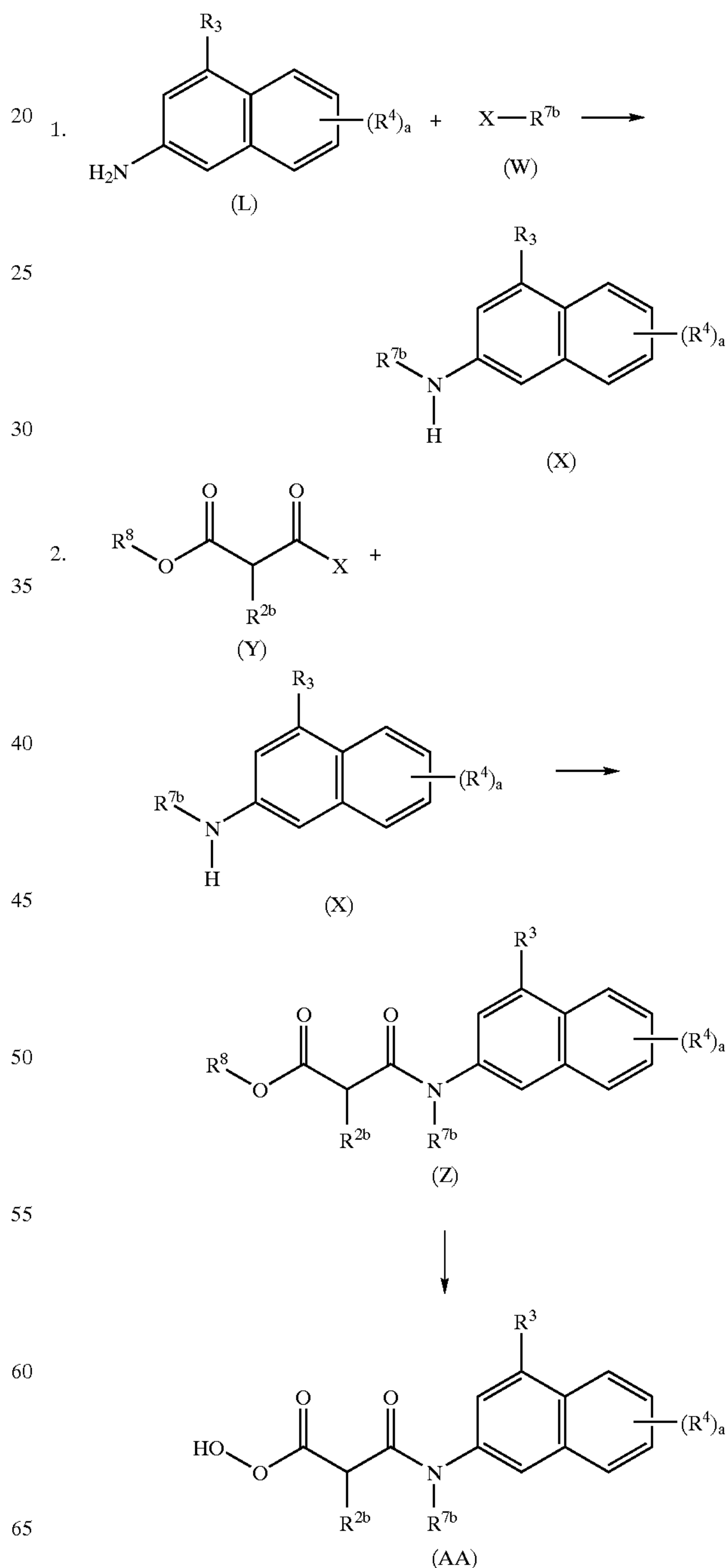
REACTION SCHEME 11
