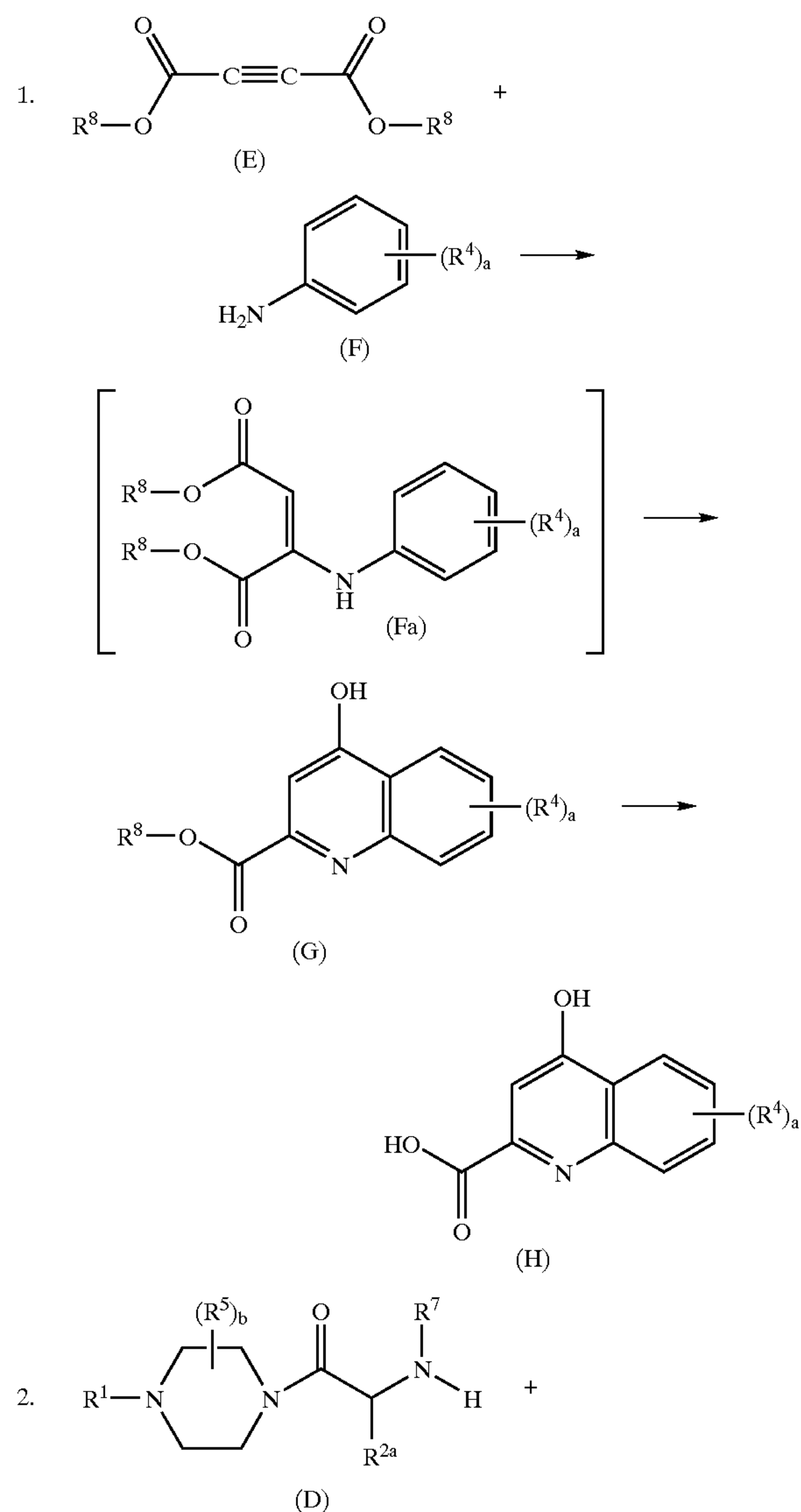
REACTION SCHEME 2
