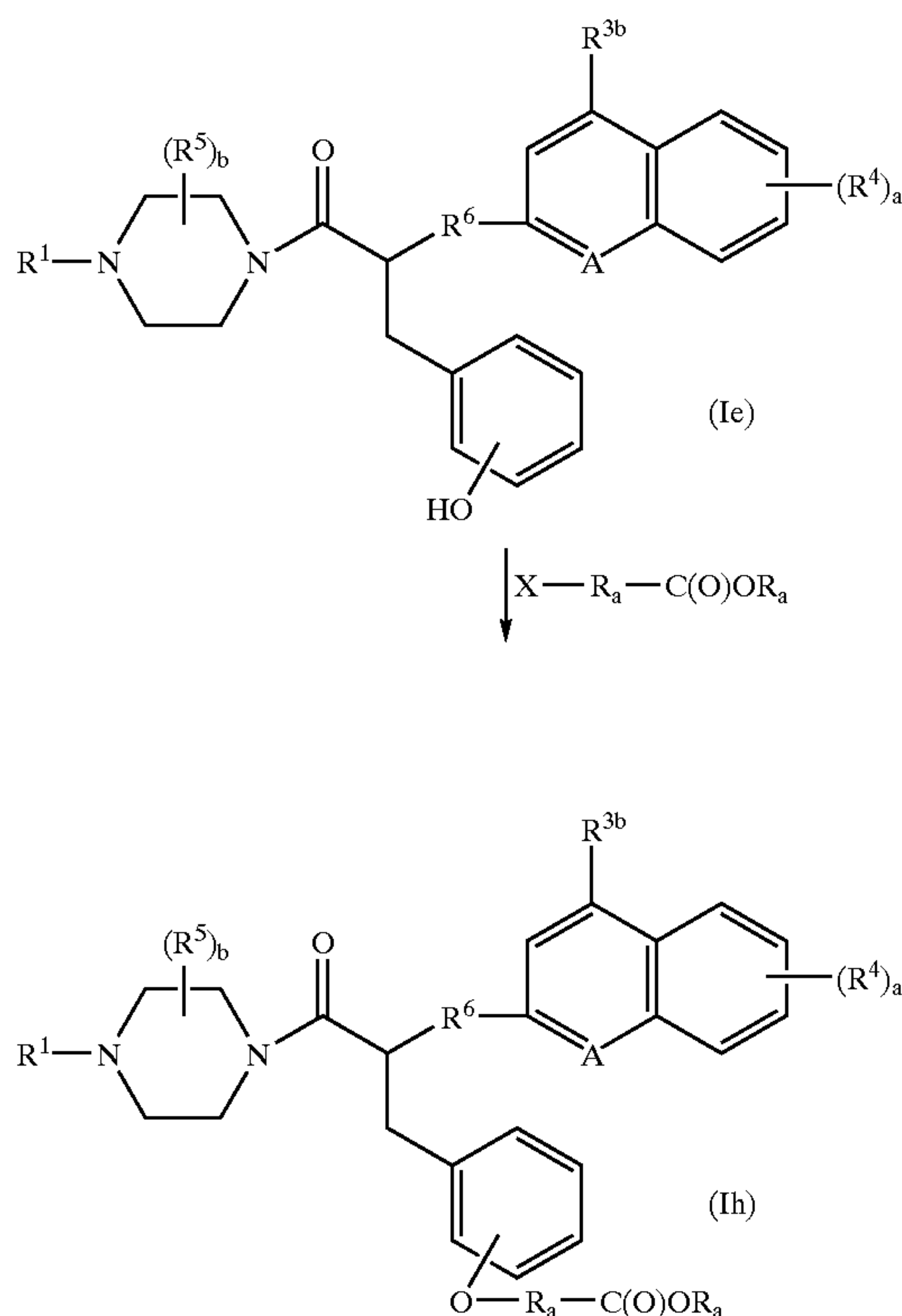
REACTION SCHEME 5
