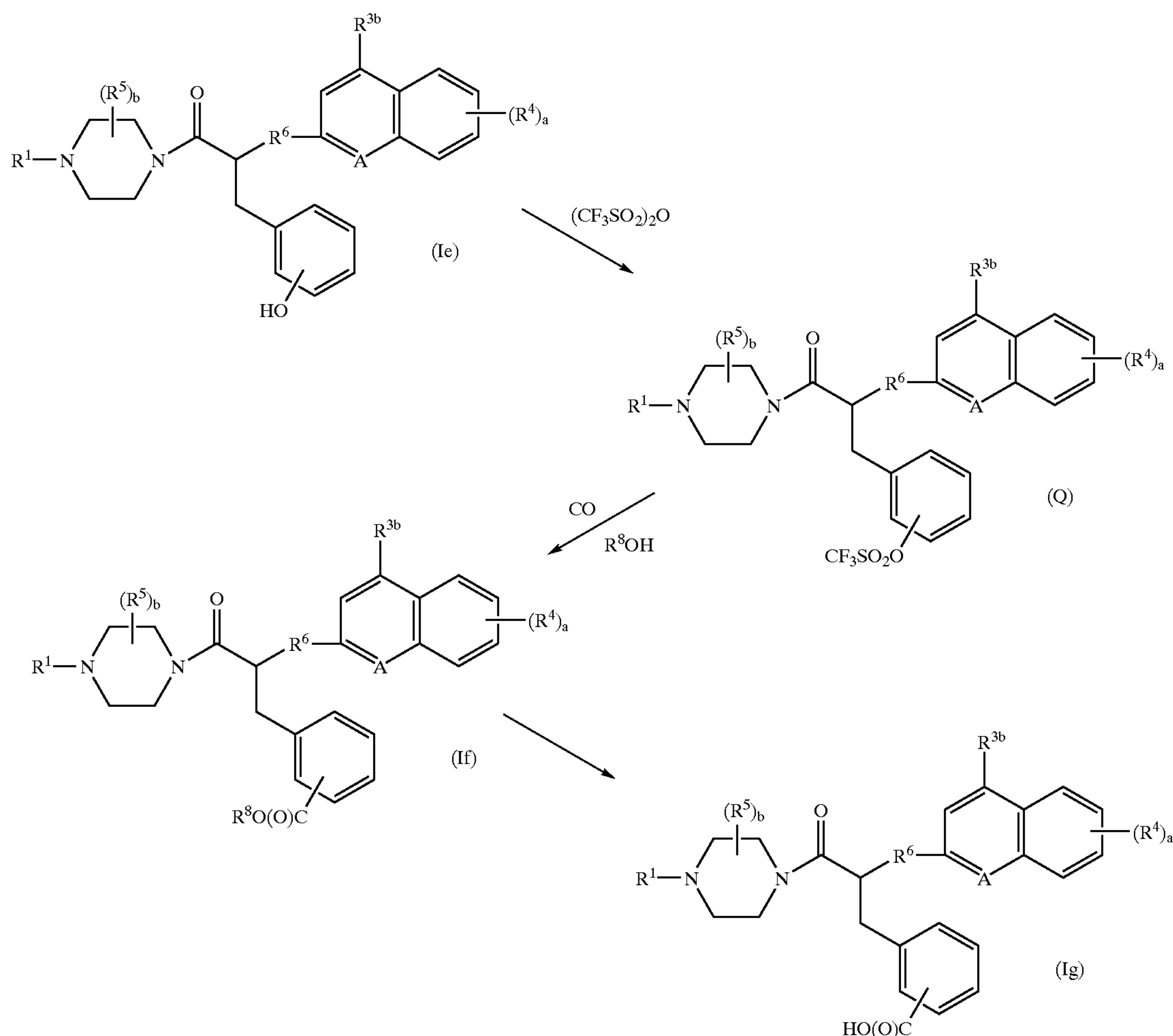
REACTION SCHEME 4
