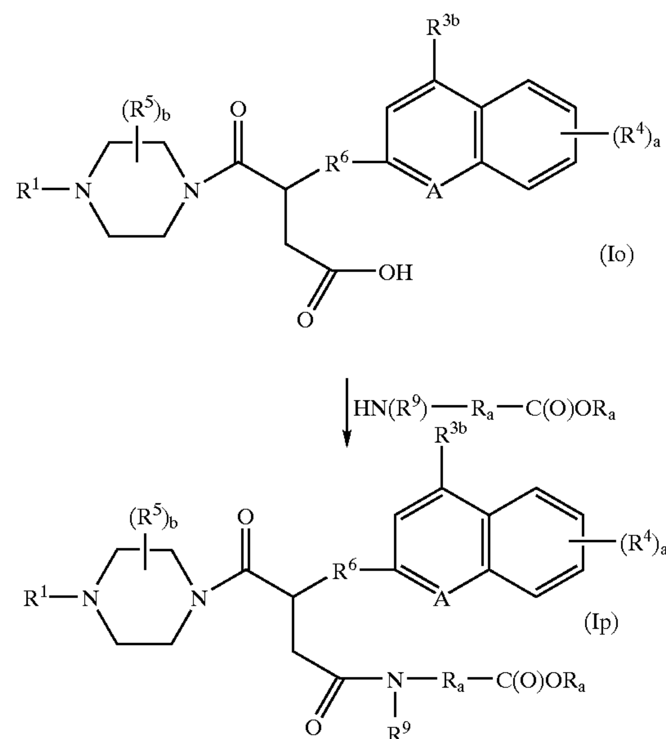
REACTION SCHEME 8
