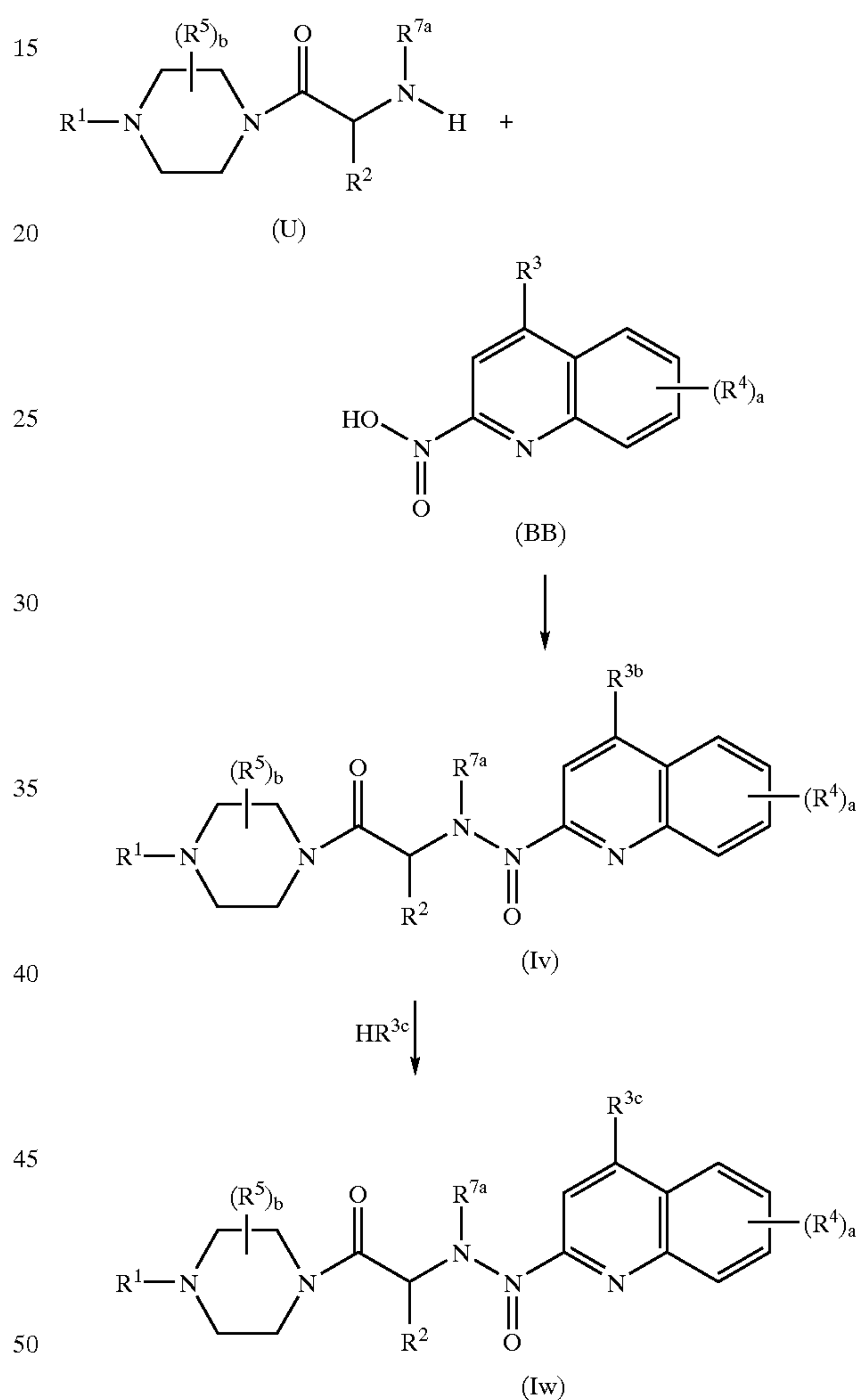
REACTION SCHEME 12
