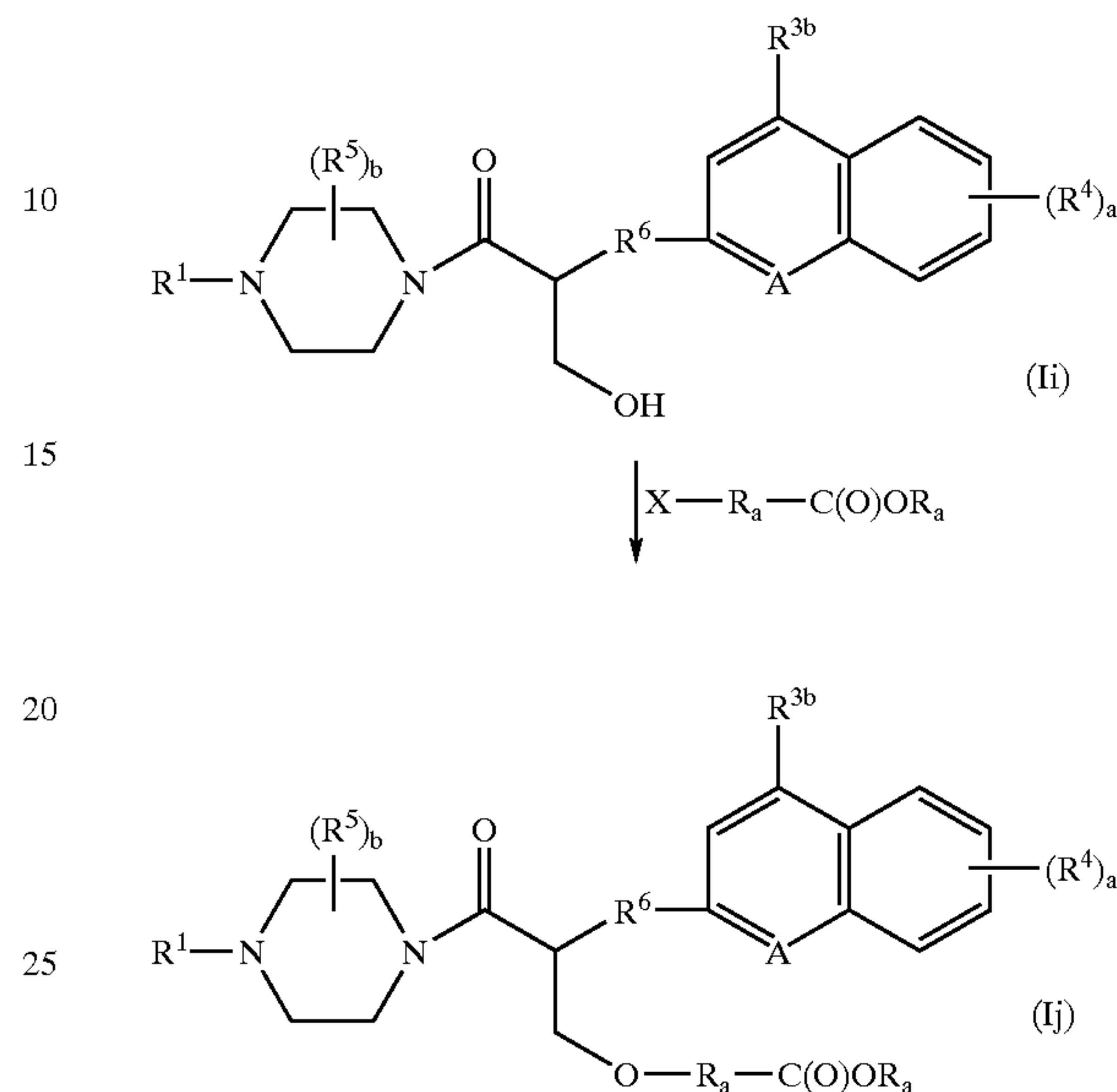
REACTION SCHEME 6
