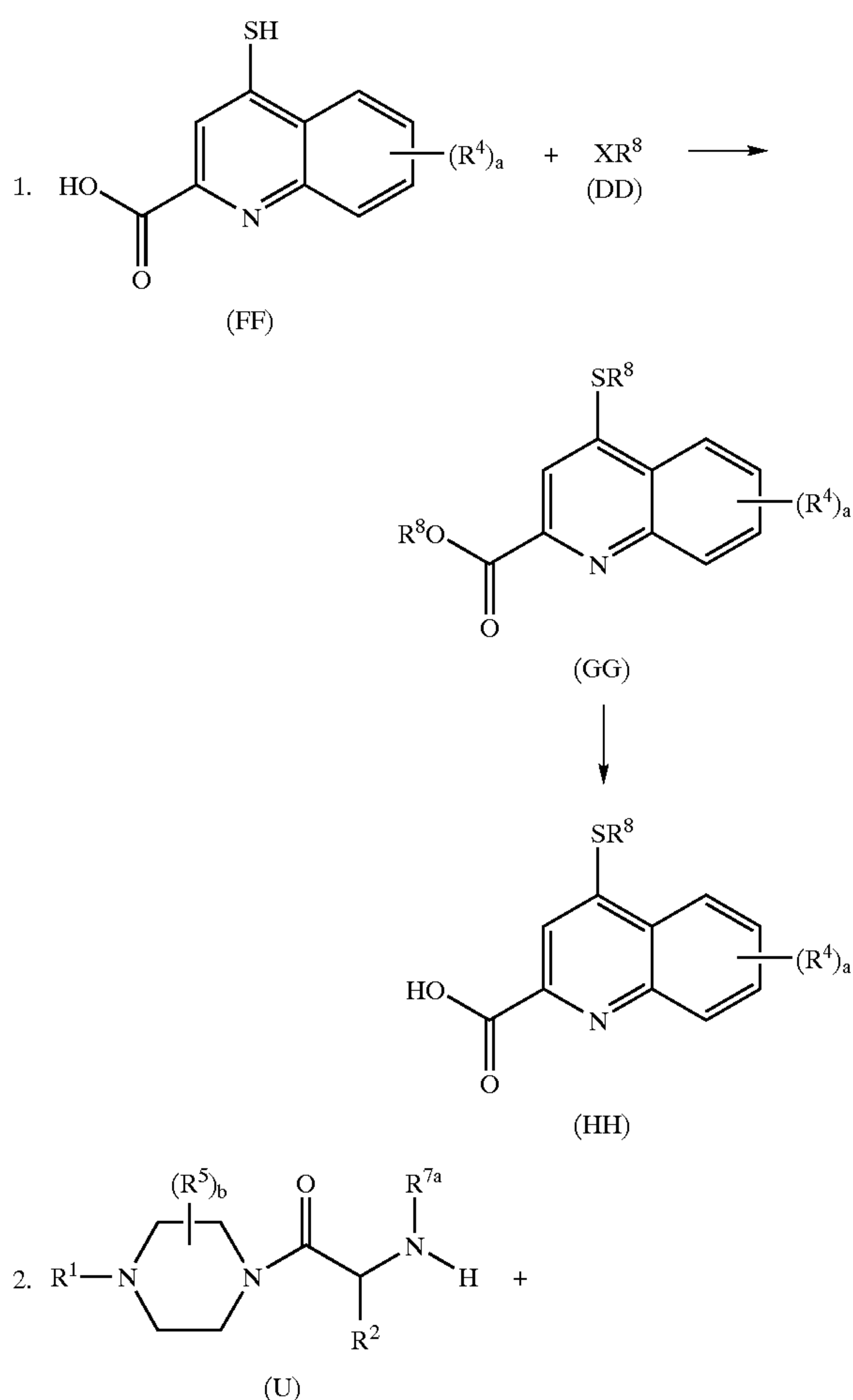
REACTION SCHEME 14
