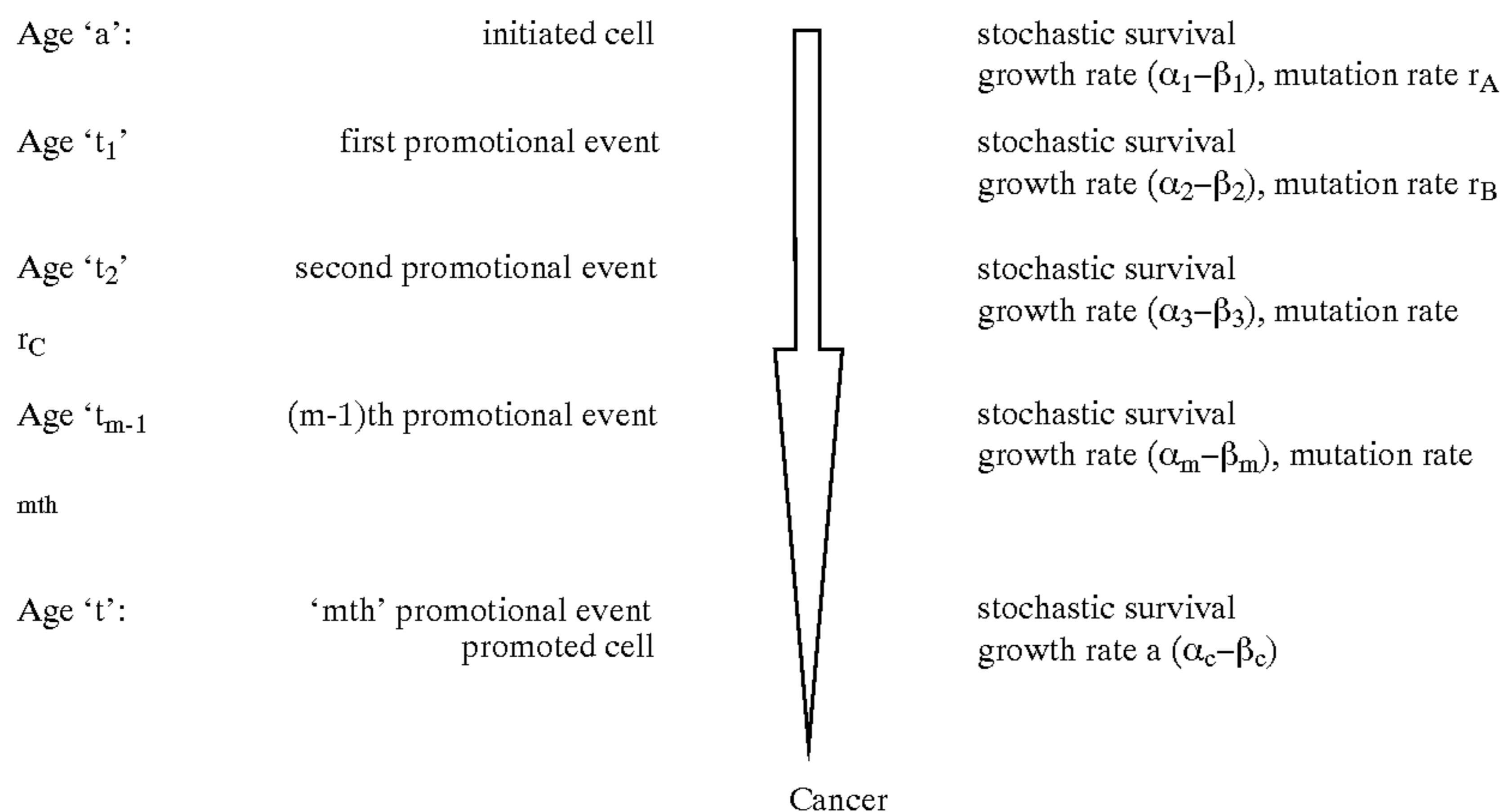
FIG. 16. Diagram of promotion for 'm' necessary events
