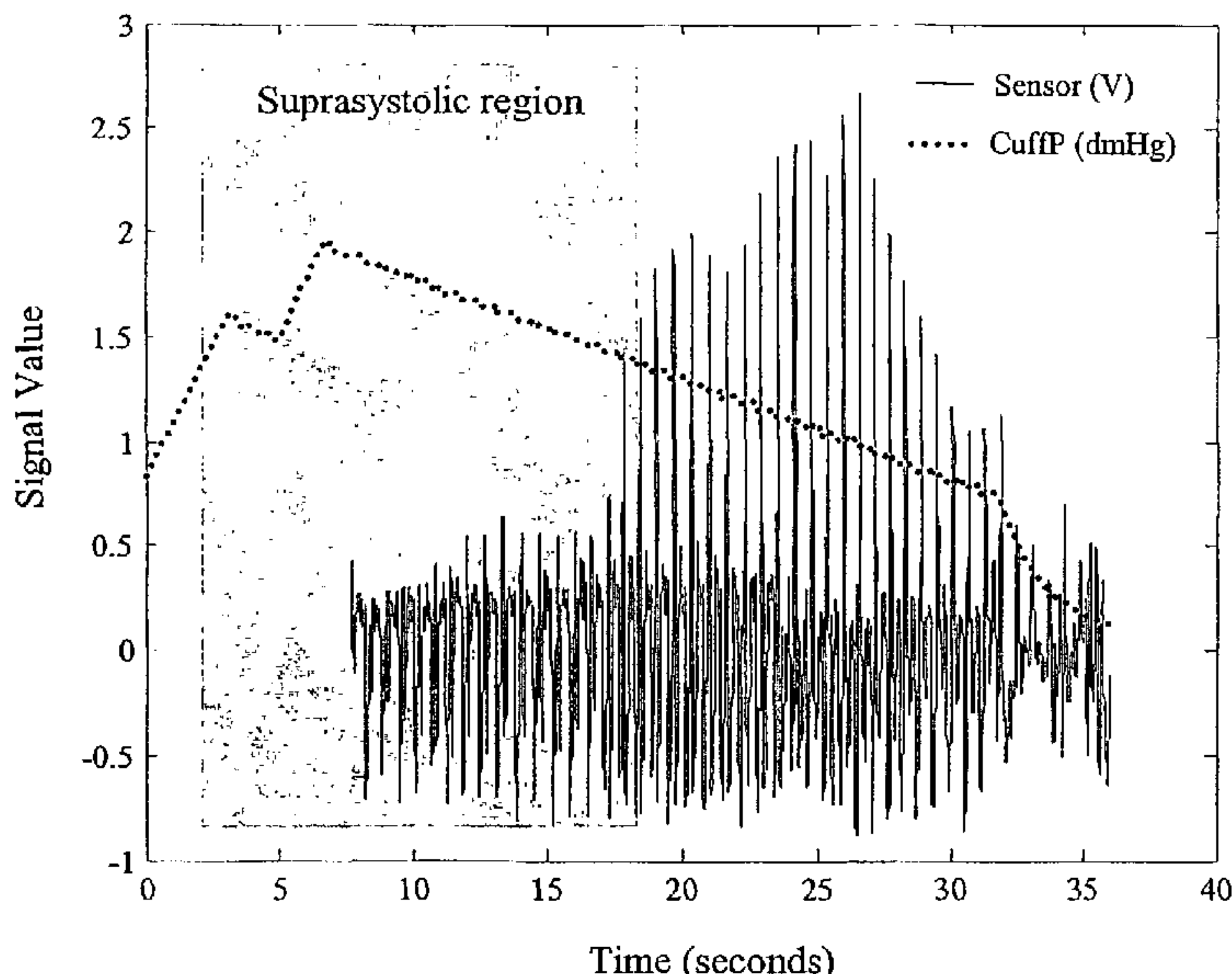
Typical signal from piezoelectric sensor
