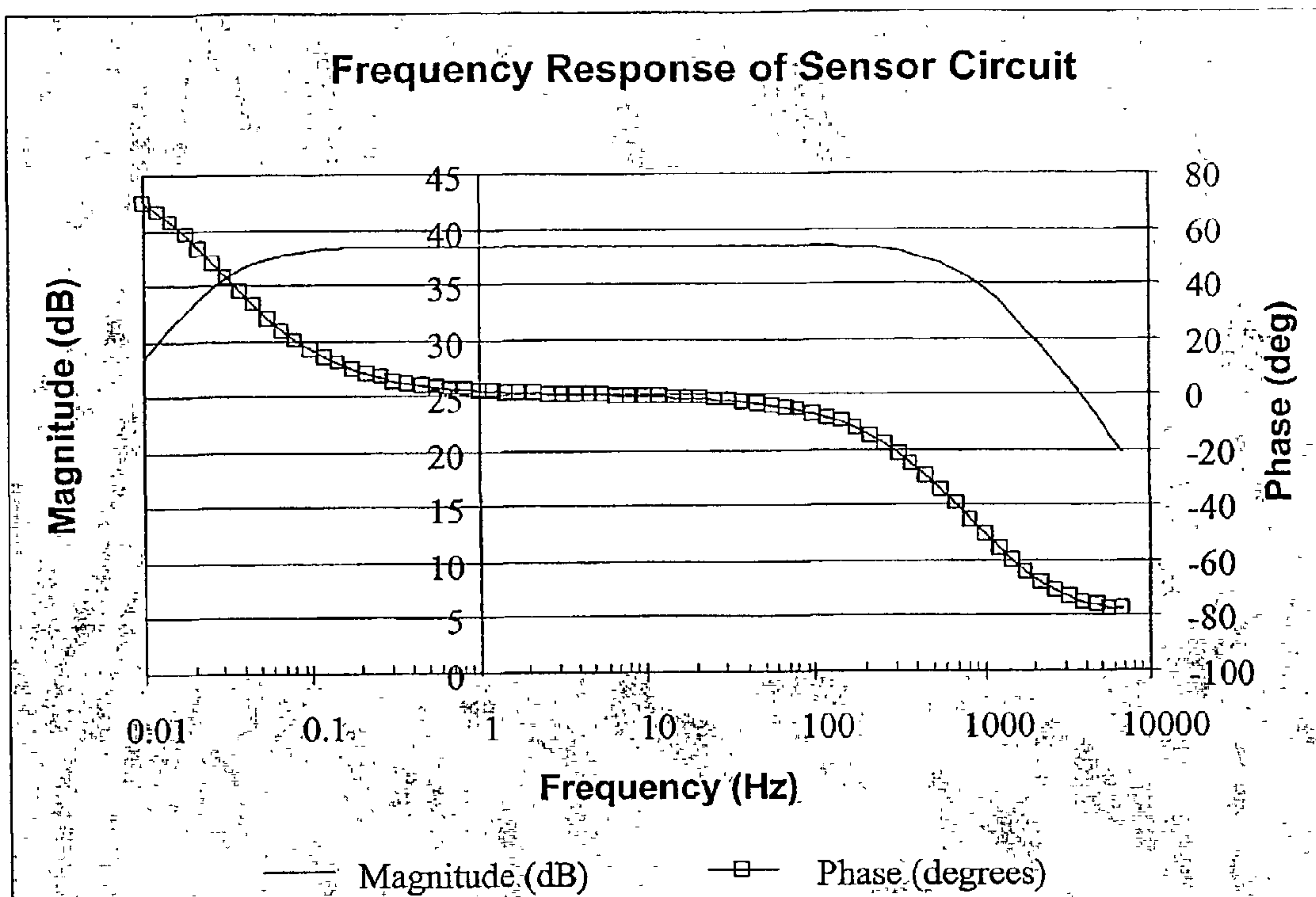
Figure 6: Frequency response of sensor
