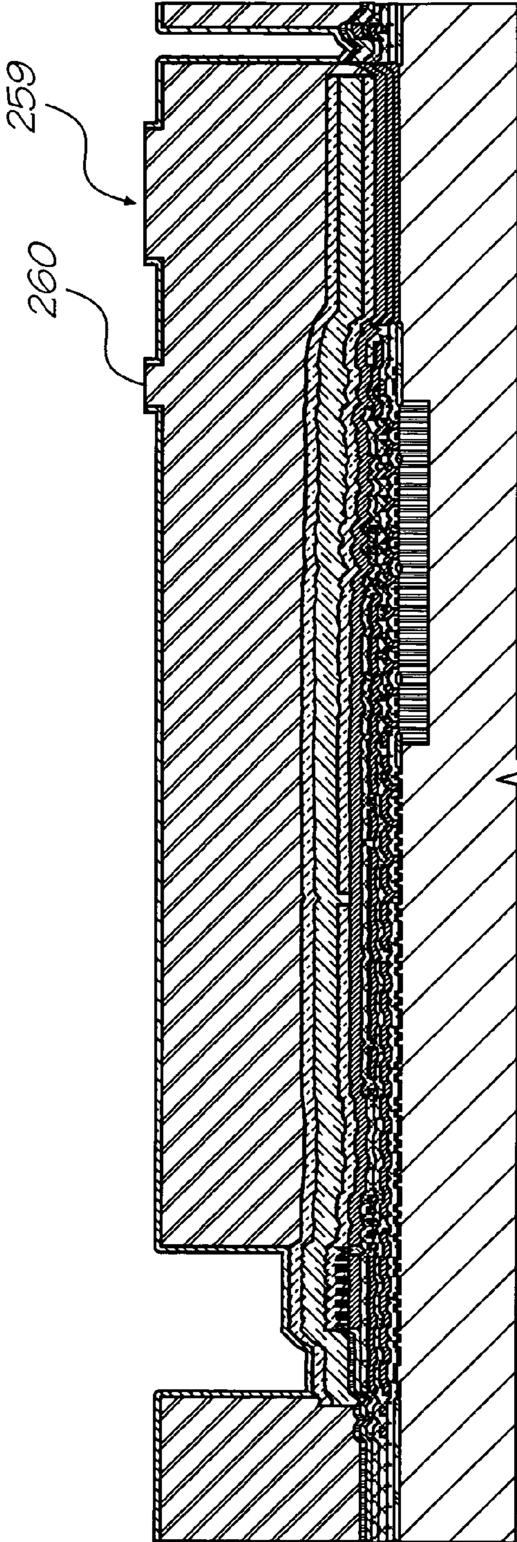
Form self-aligned nozzles using CMP
