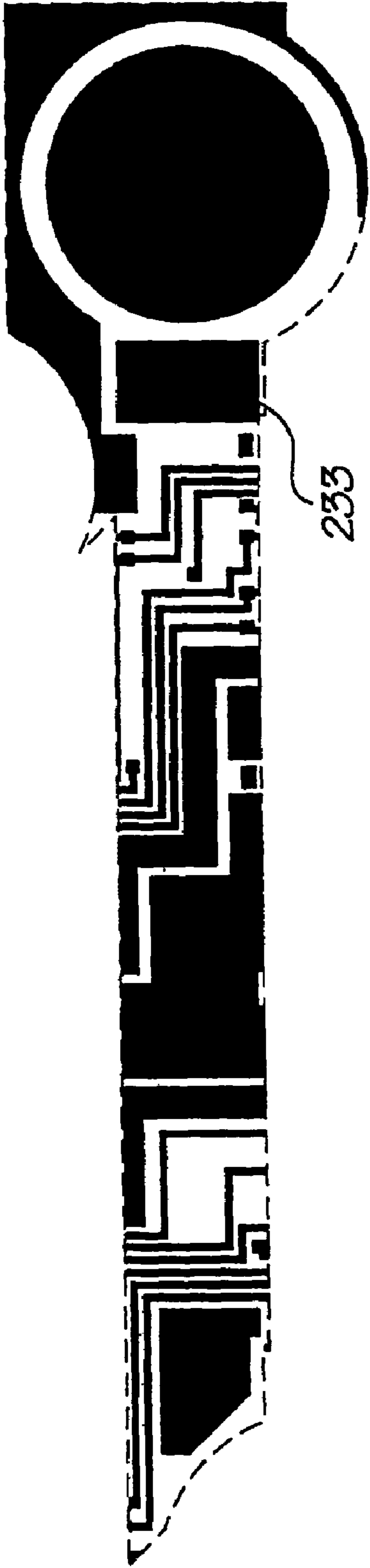
Metal 2 mask
