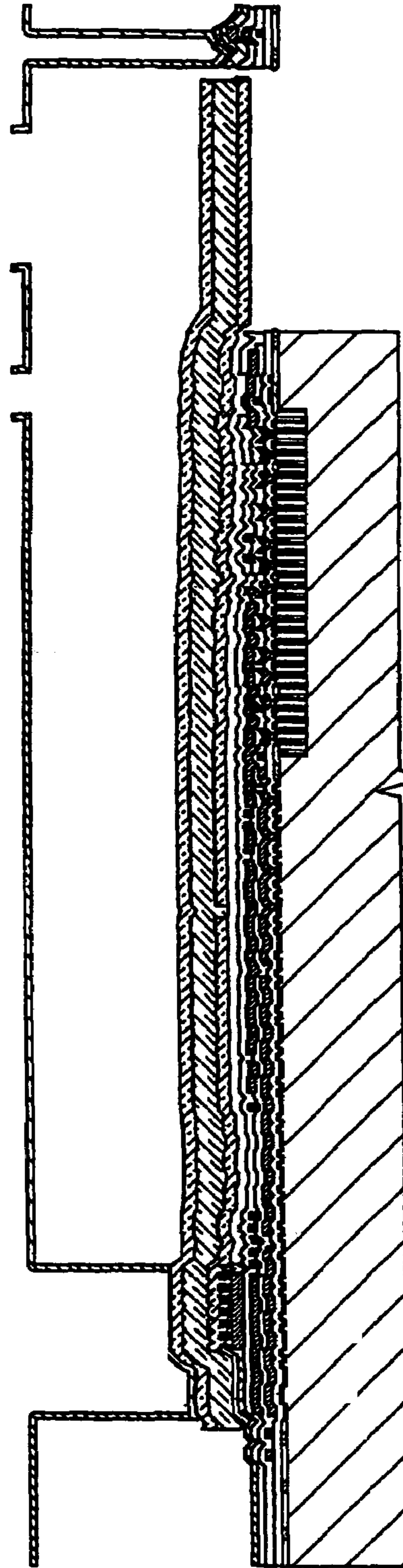
Detach from wafer blank, etch sacrificial material
