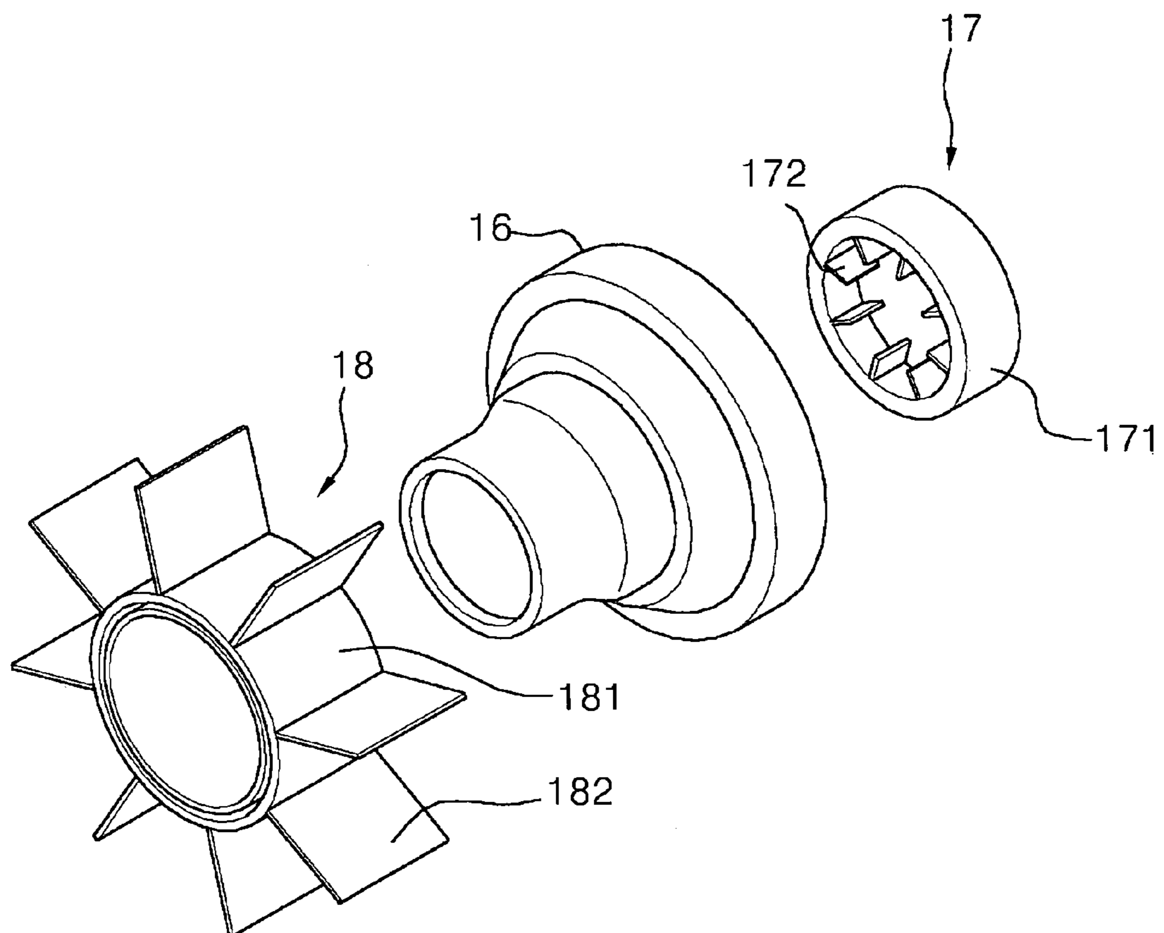
FIG. 2 PRIOR ART
