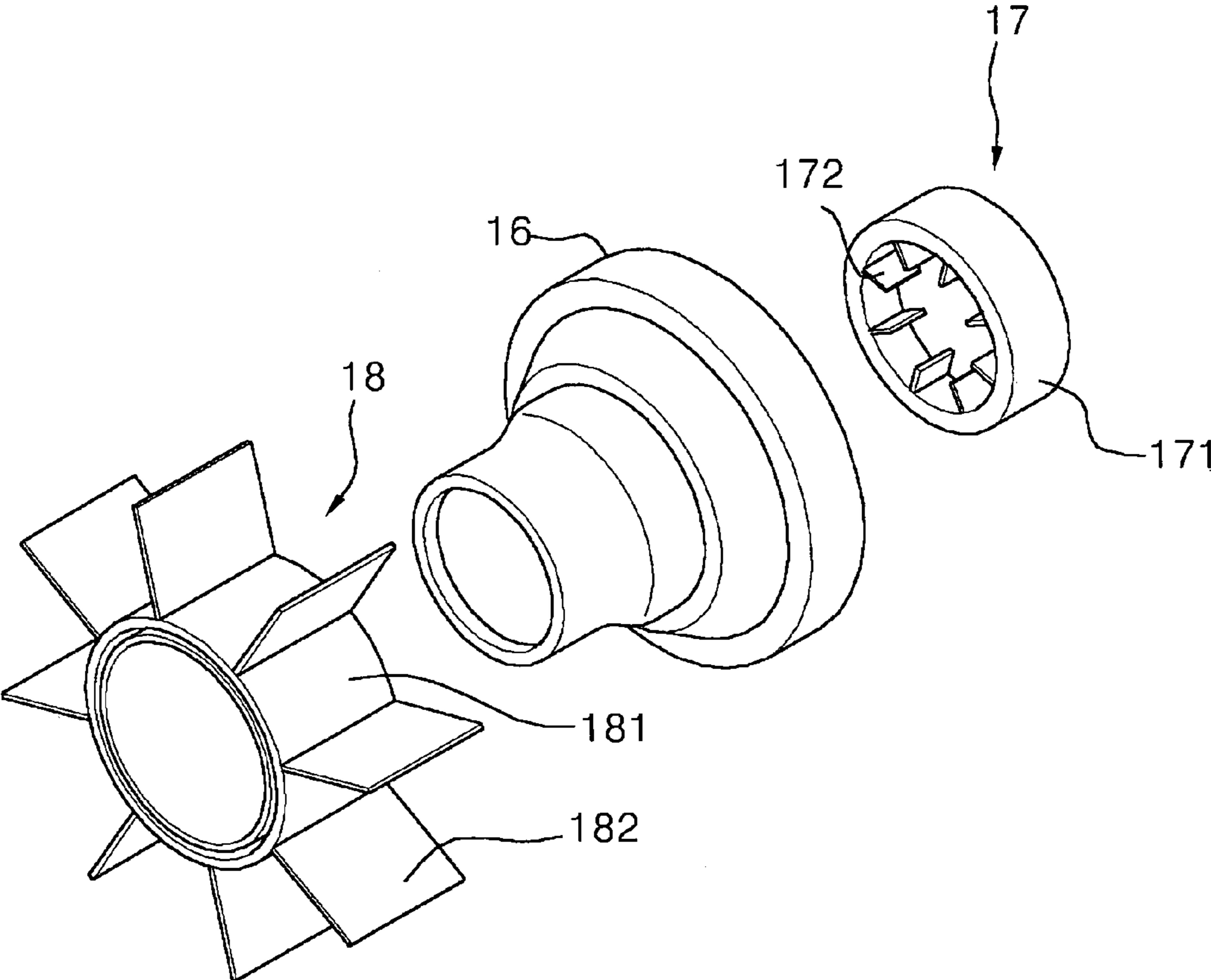
FIG. 2 PRIOR ART
