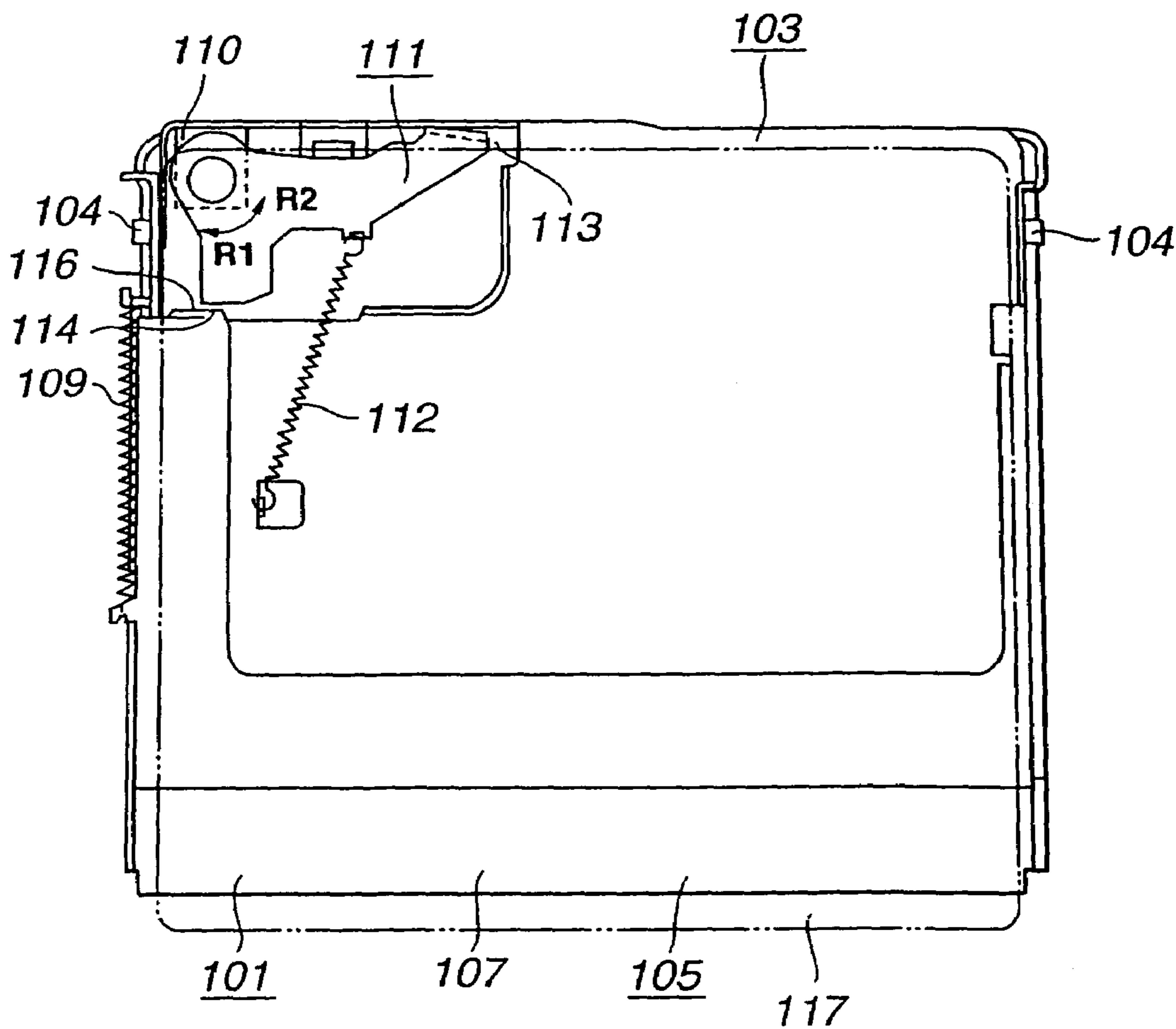
FIG. 3 (PRIOR ART)
