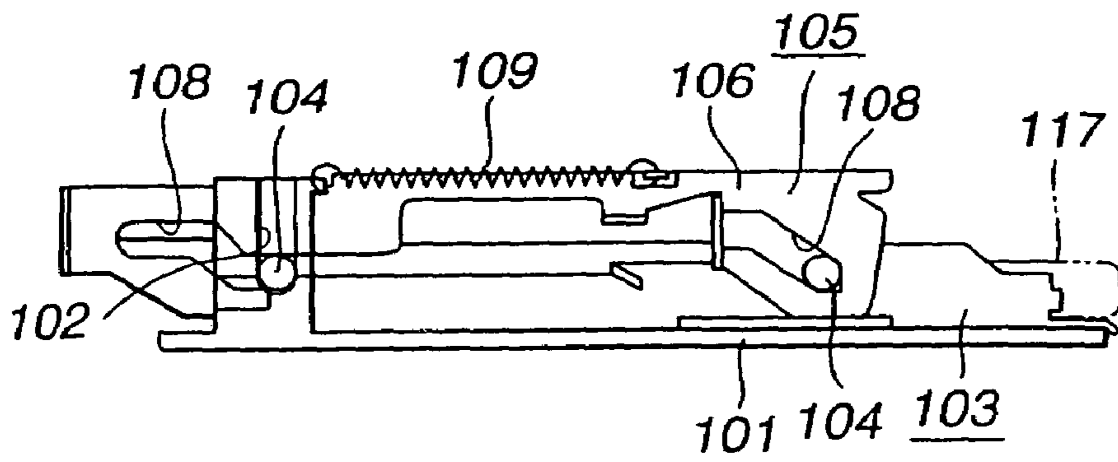
FIG. 5 (PRIOR ART)
