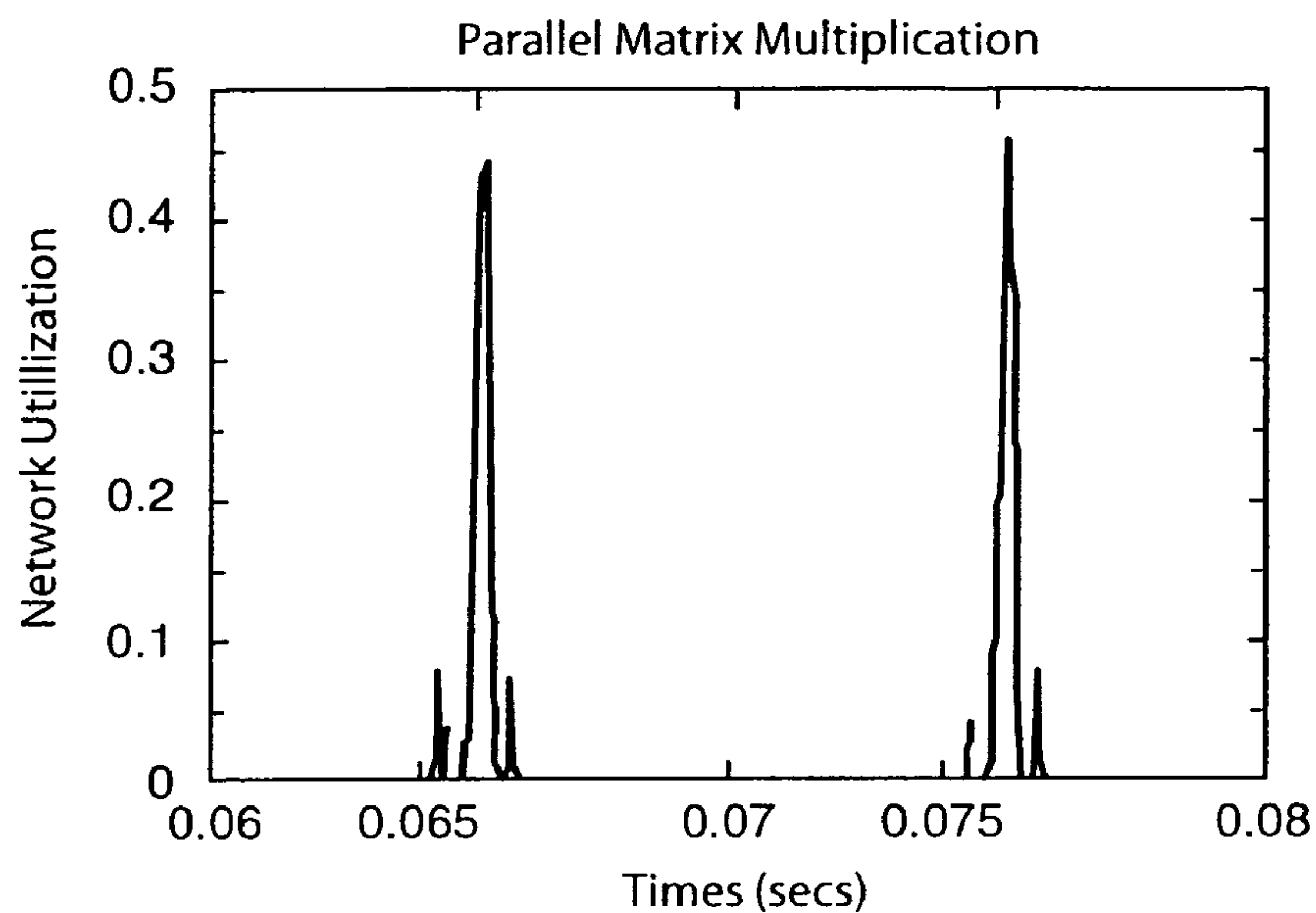
Fig. 2C (Prior Art)
