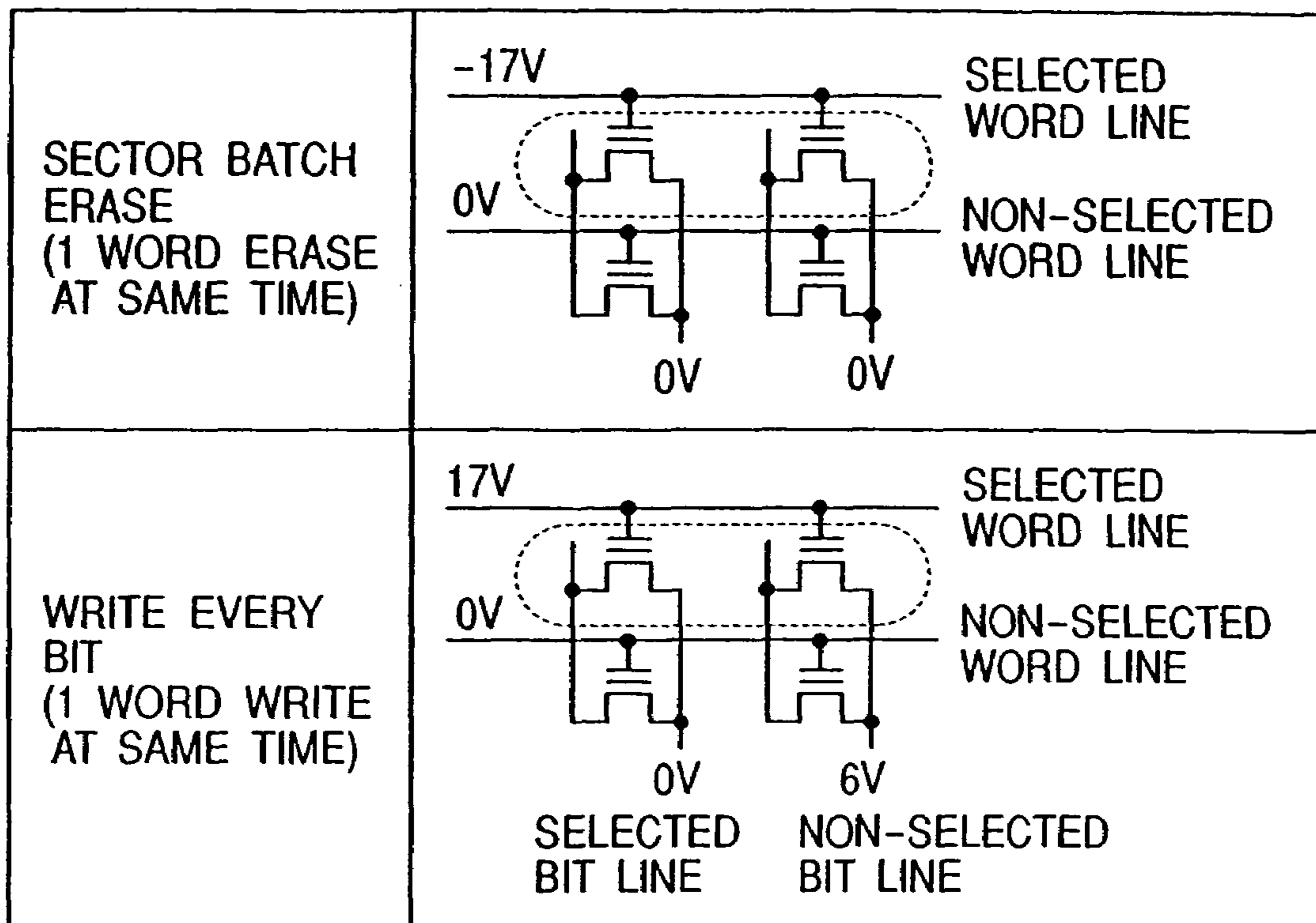
OPERATION VOLTAGE
