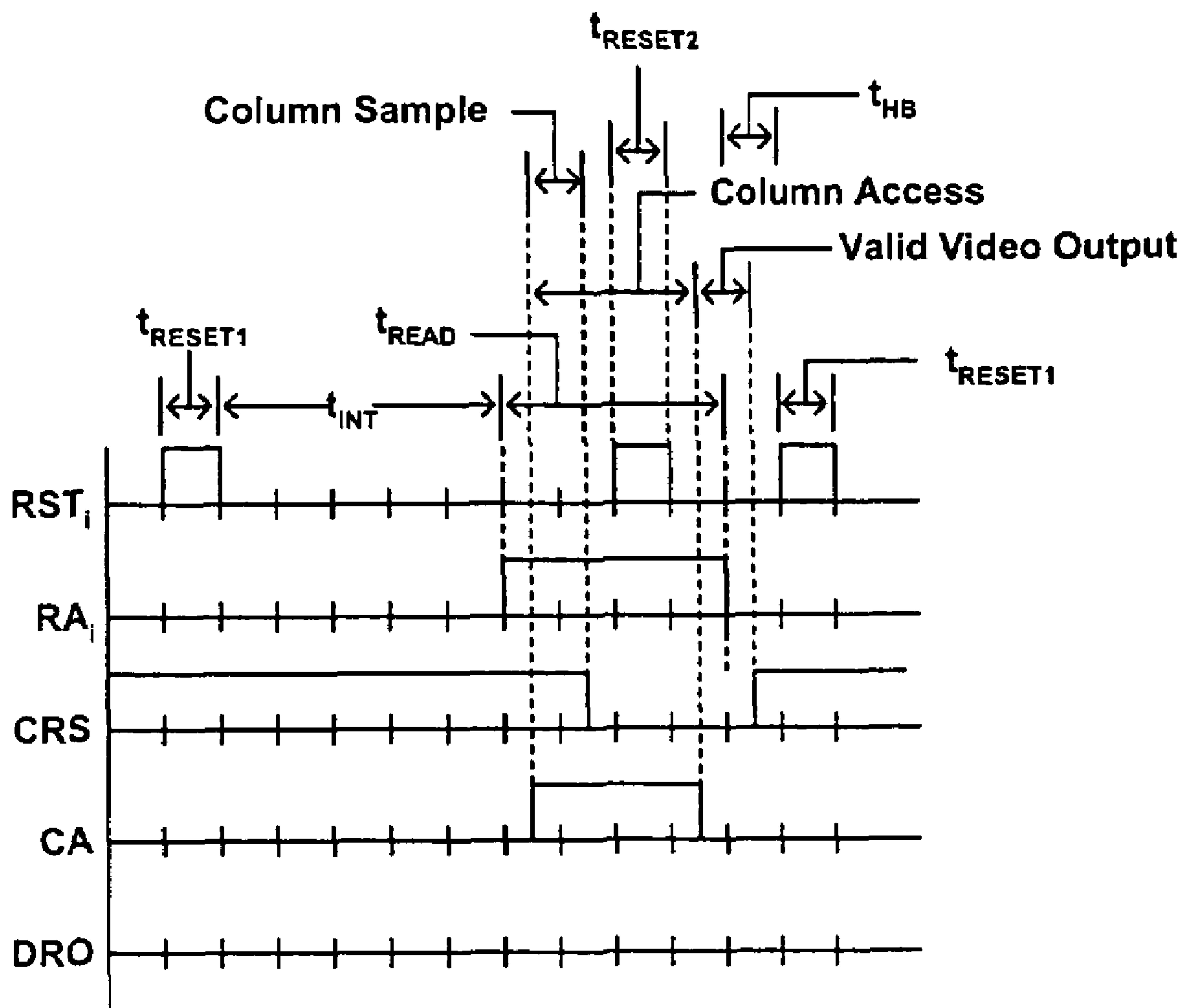
Figure 4 (PRIOR ART)
