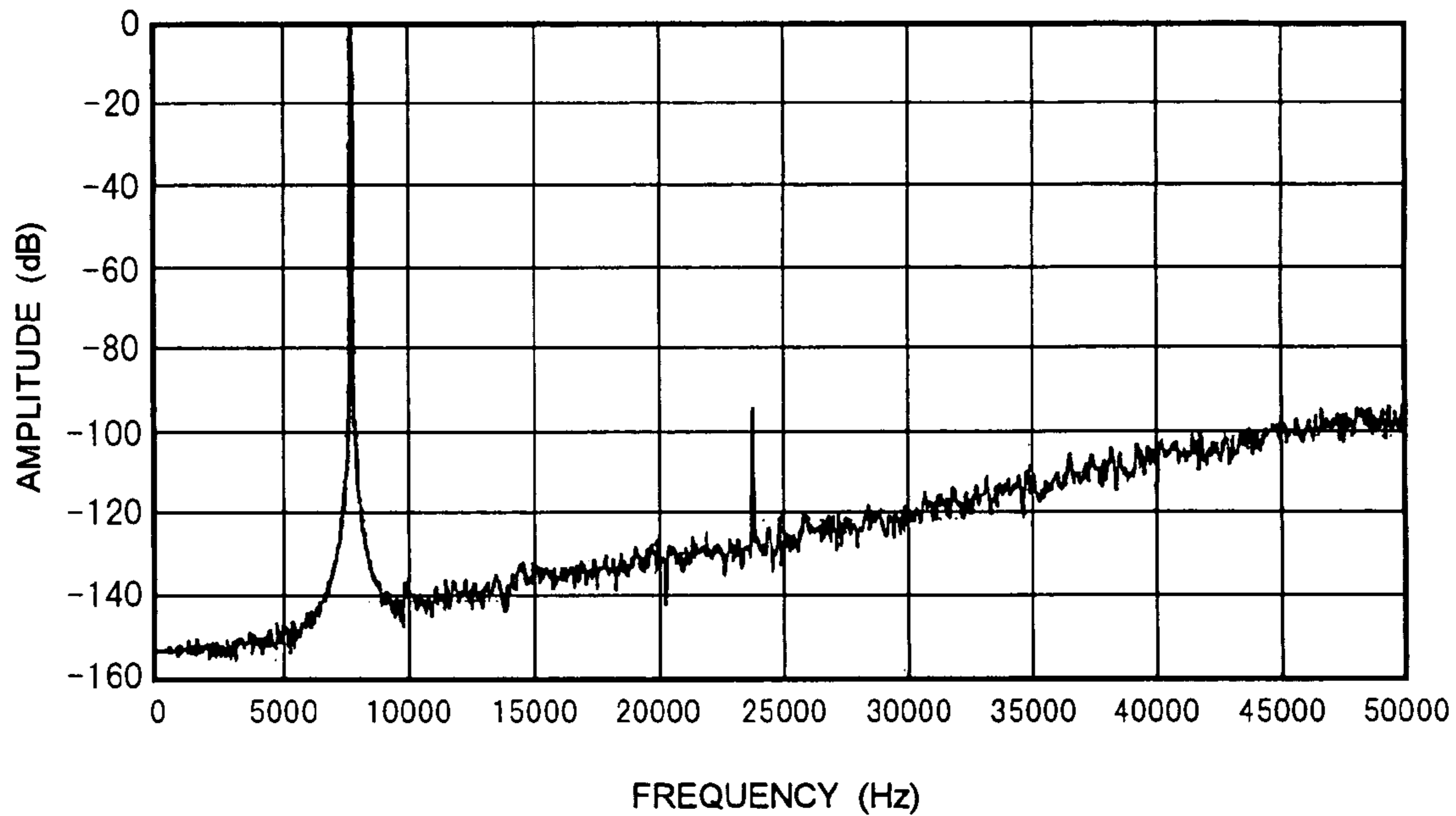
SPECTRUM OF PWM USING ONLY X - SERIES
