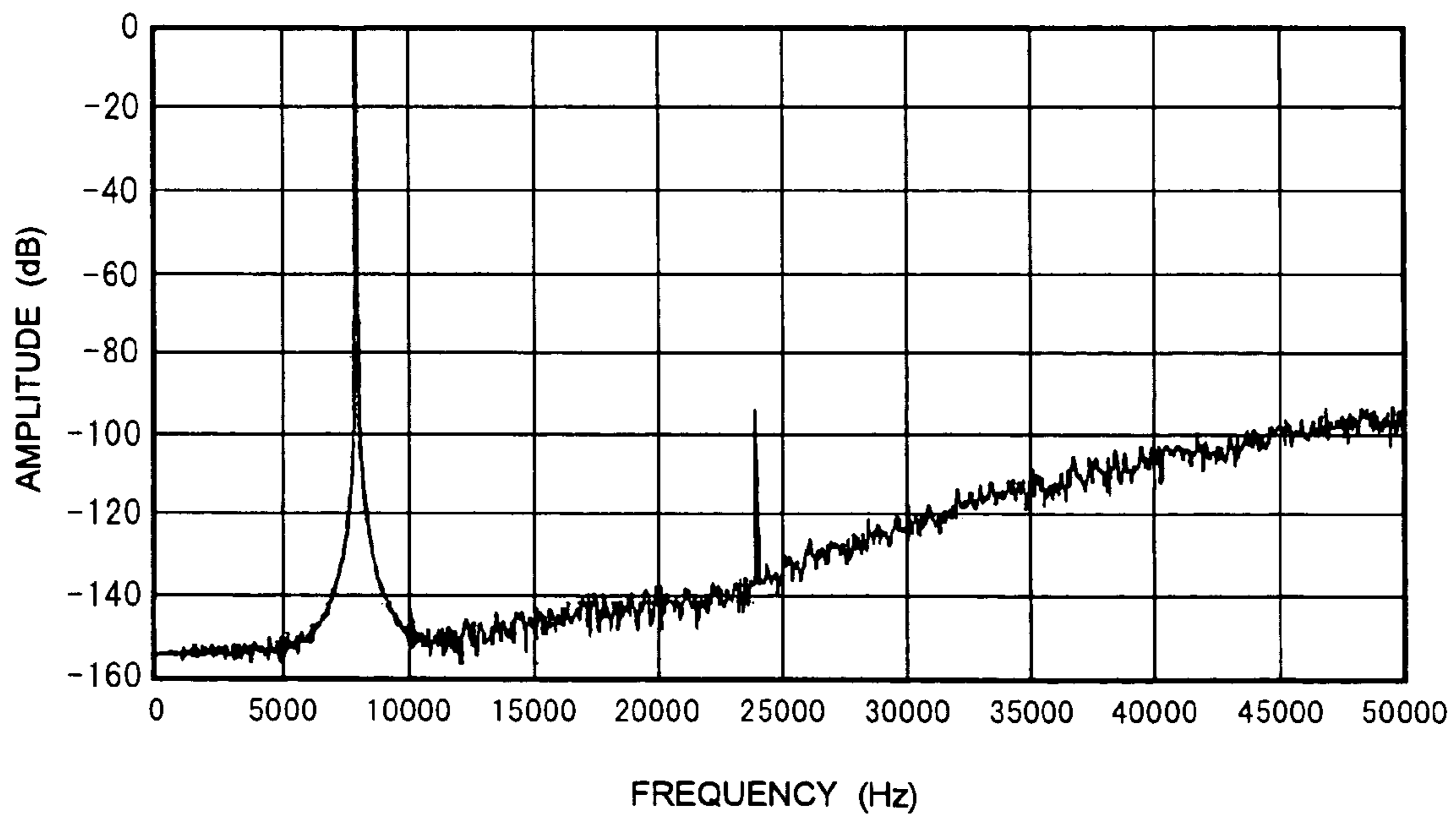
SPECTRUM OF PWM USING X - SERIES AND Y - SERIES
