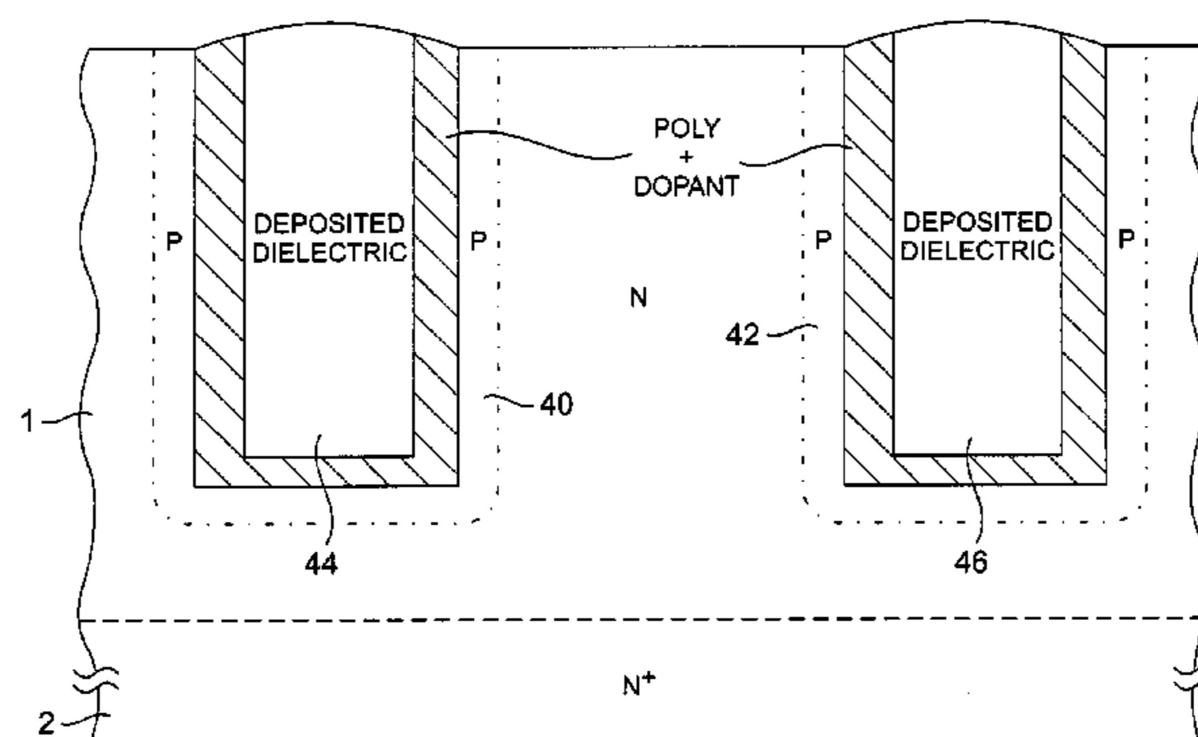
A DOPING PROFILE THAT WAS DIFFUSED FROM A TRENCH CONTAINING DOPED POLYCRYSTALLINE SILICON AS WELL AS DEPOSITED DIELECTRIC
