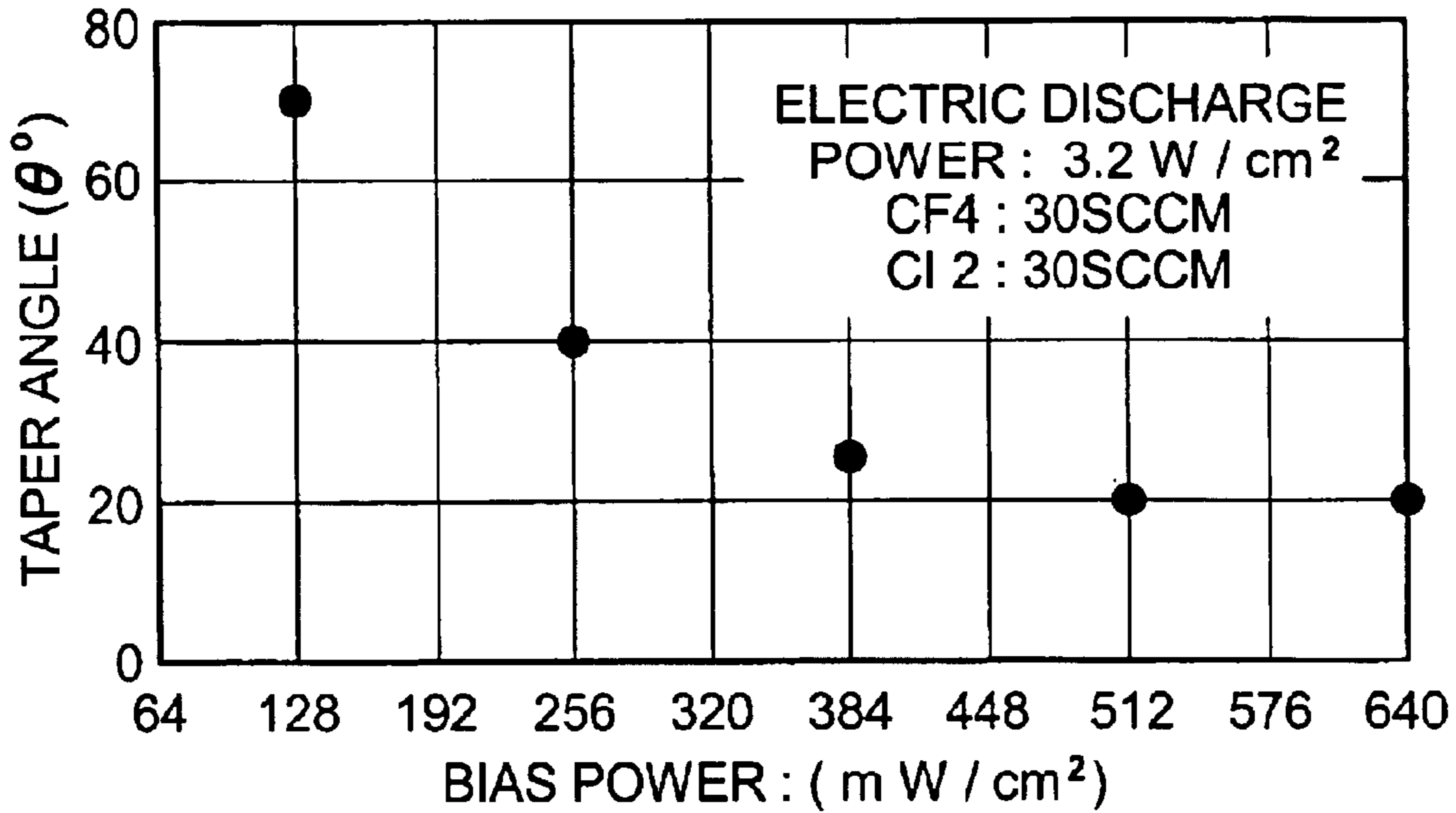
DEPENDENCE OF TAPER ANGLE ON BIAS POWER
