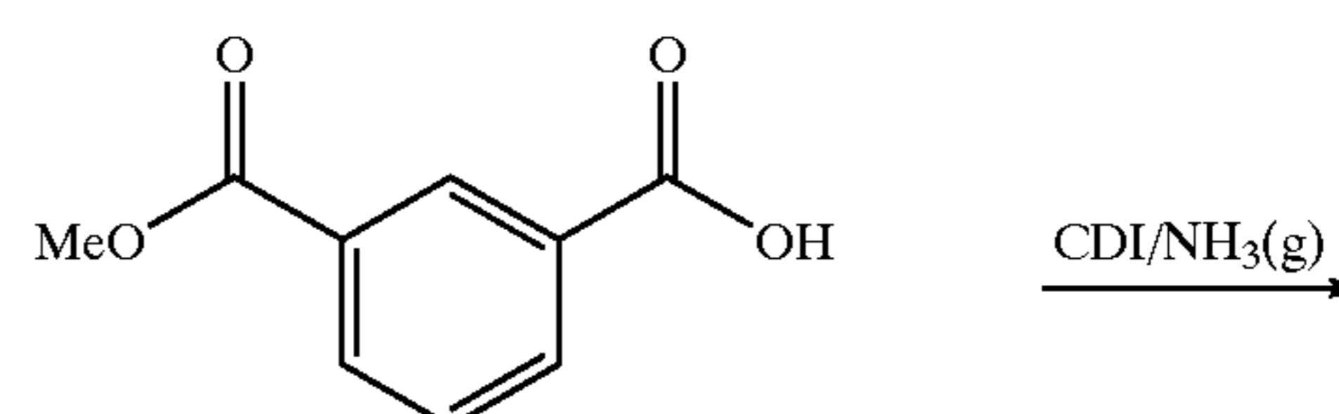
Scheme IVC
