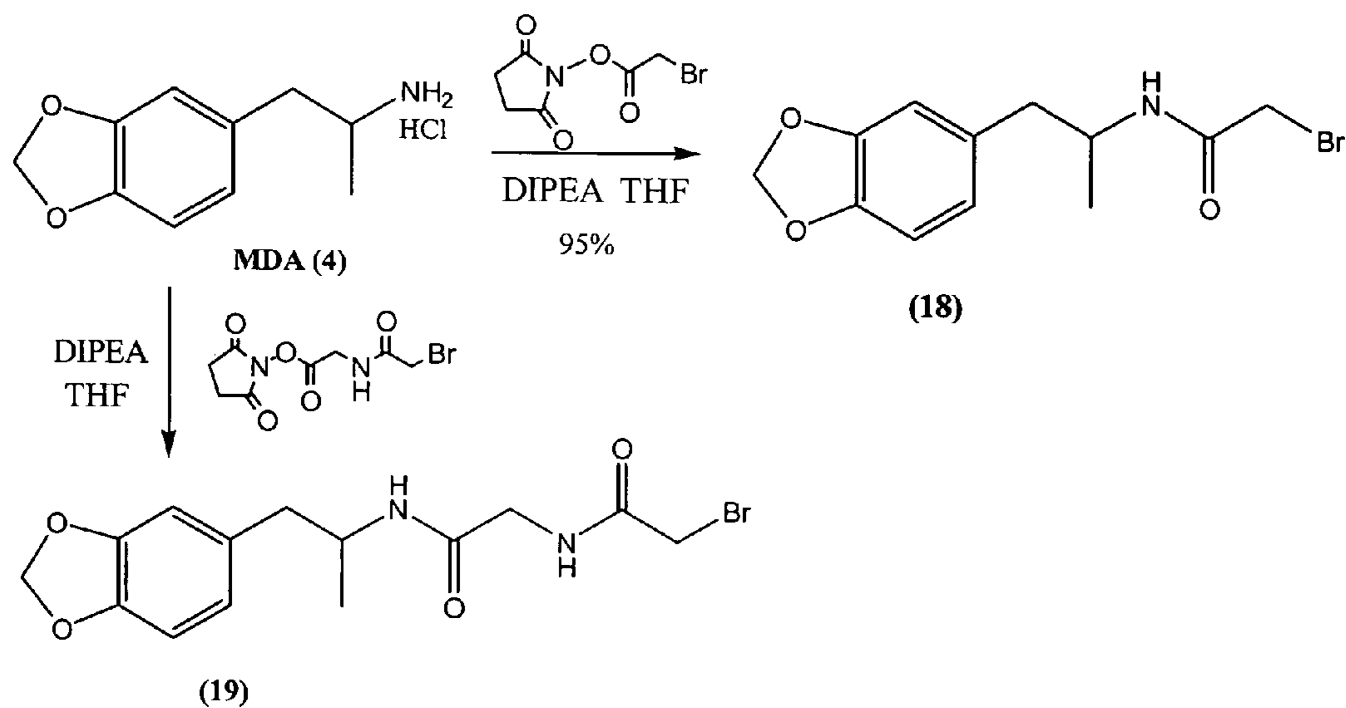
Figure 4B. Synthesis of MDA Hapten (20)
