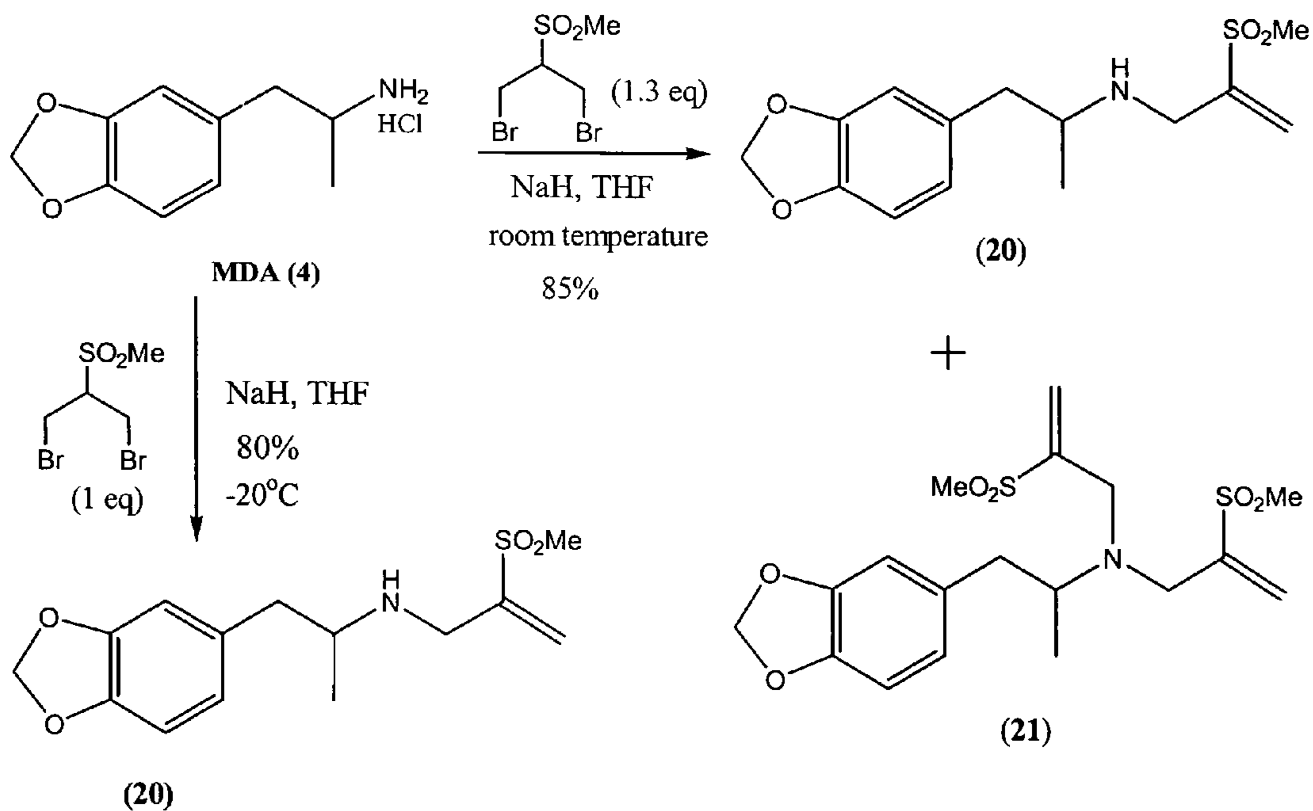
Figure 4B. Synthesis of MDA Hapten (20)
