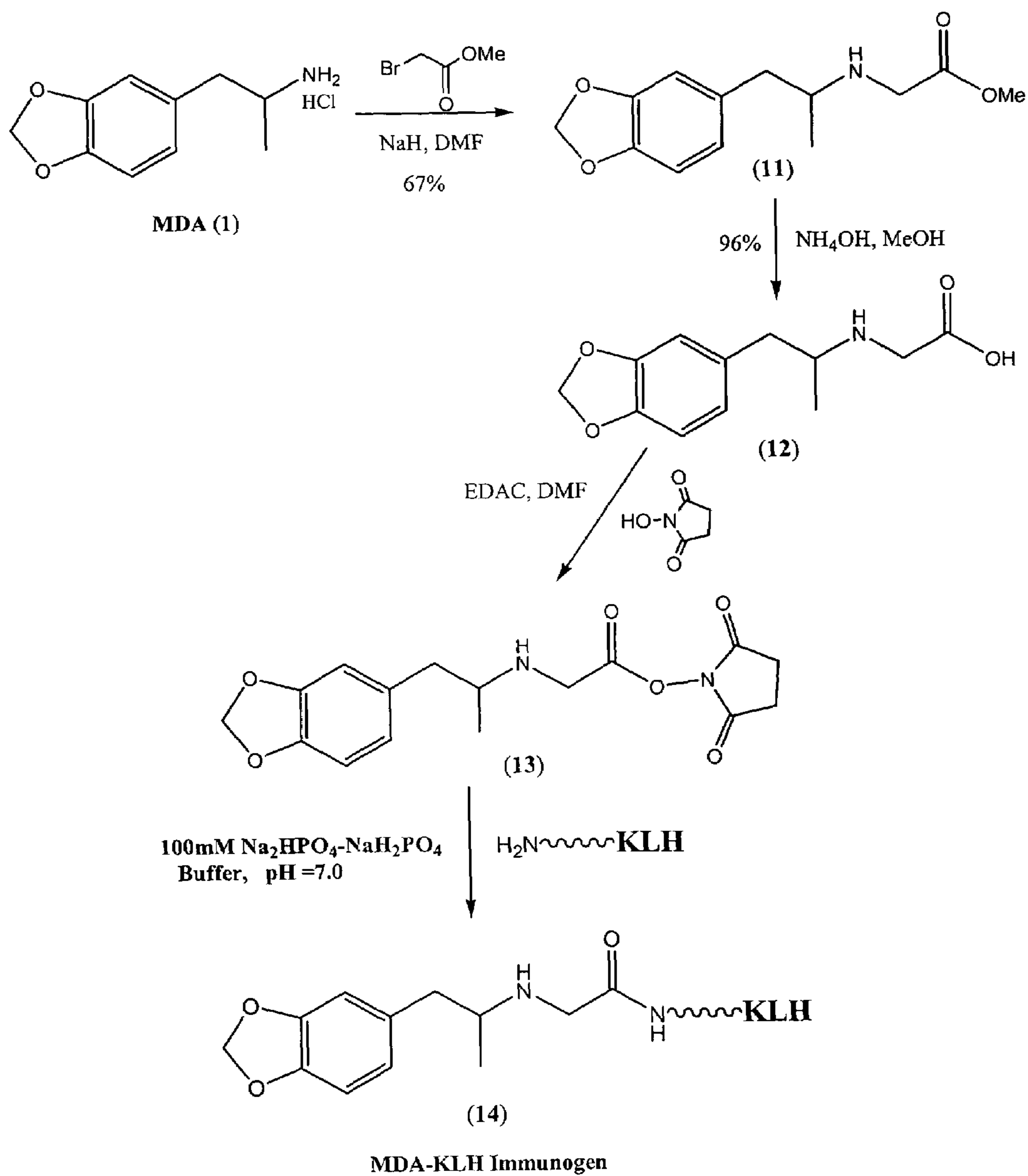
Figure 2. Synthesis of MDA-KLH Immunogen (14)
