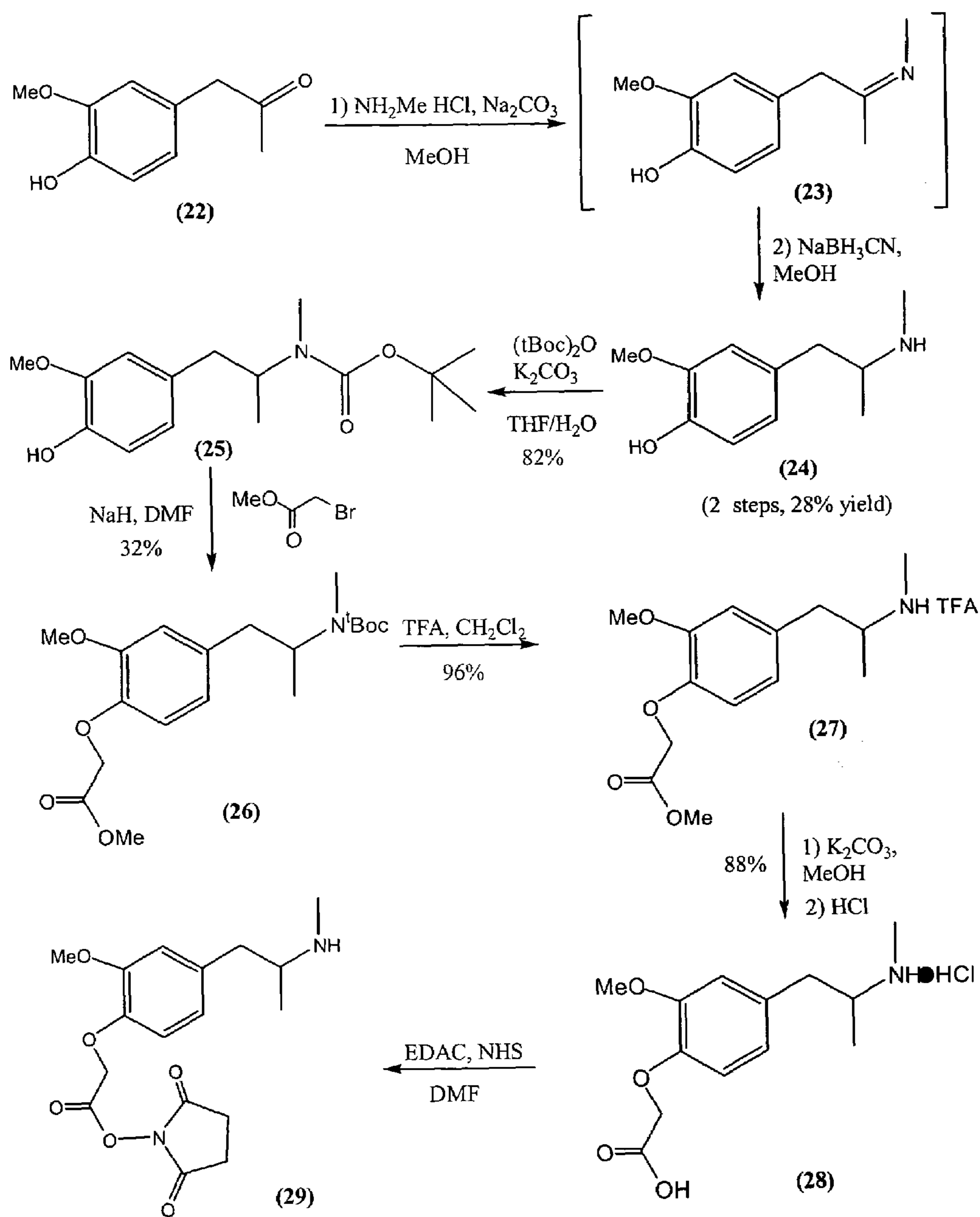
Figure 5. Synthesis of HMMA Intermediate (29) for Immunogen (30)
