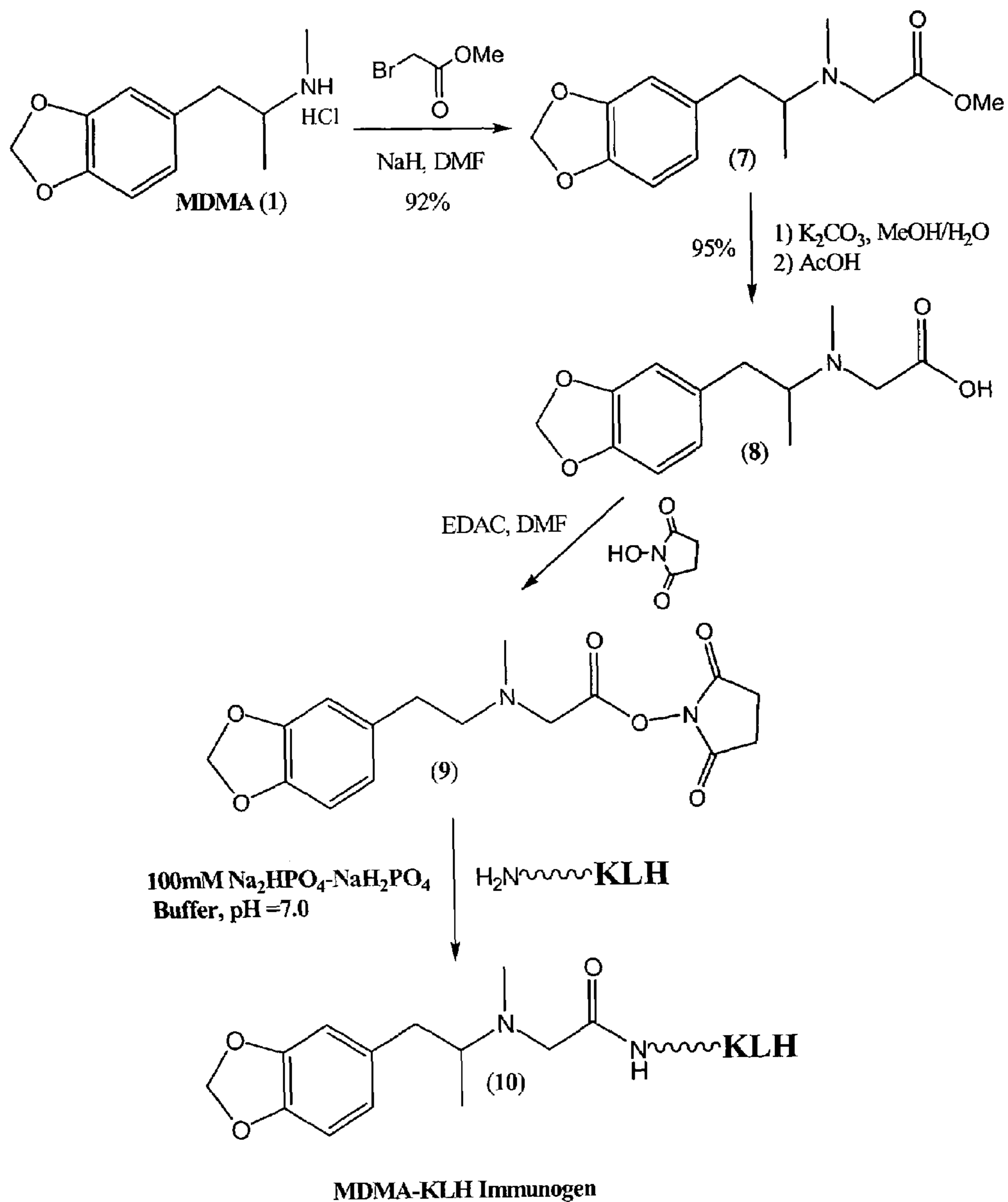
Figure 1. Synthesis of MDMA-KLH Immunogen (10)
