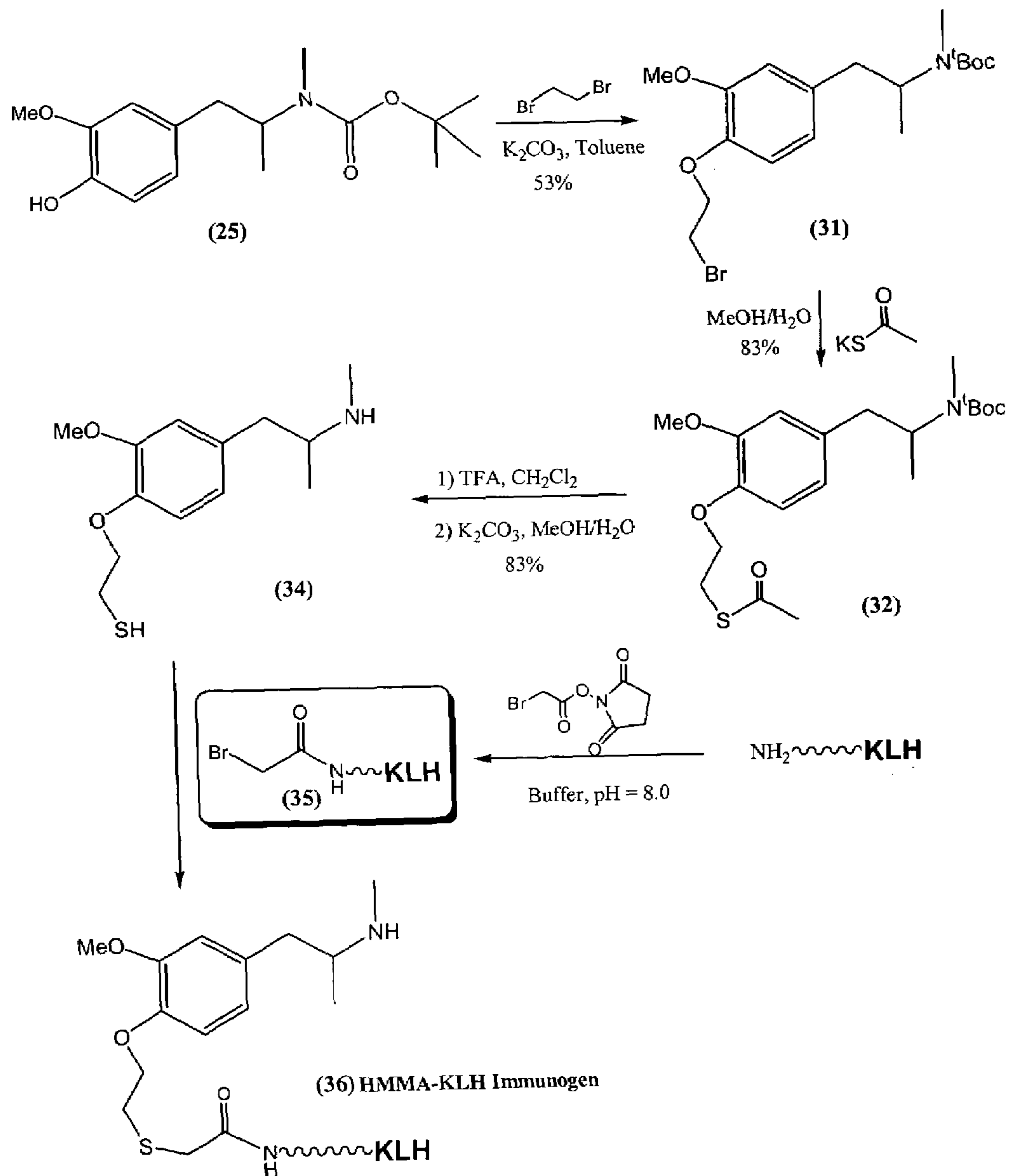
Figure 7. Synthesis of HMMA-KLH Immunogen (36)
