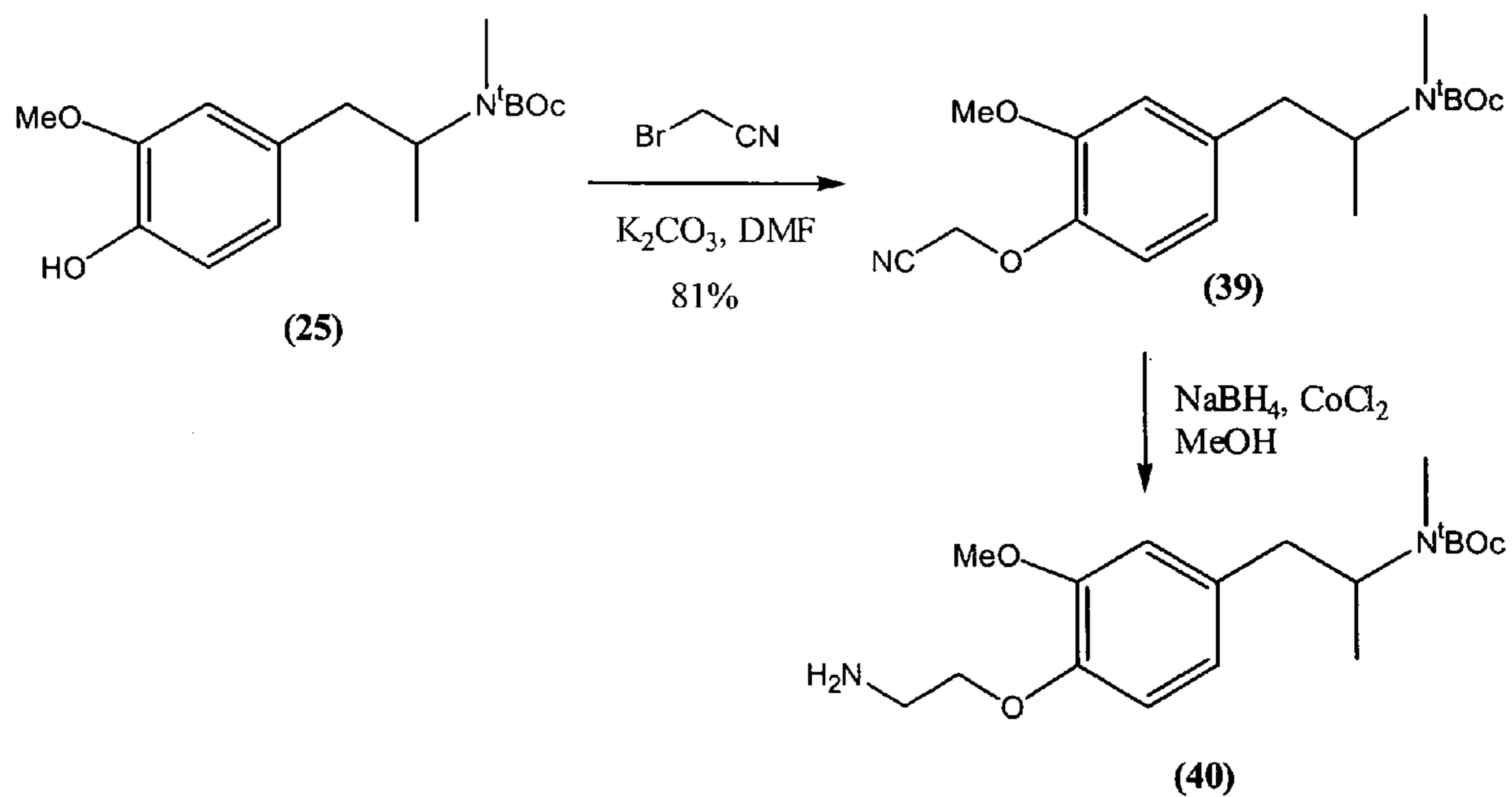
Figure 8B. Synthesis of MDMA Hapten Intermediate (40)
