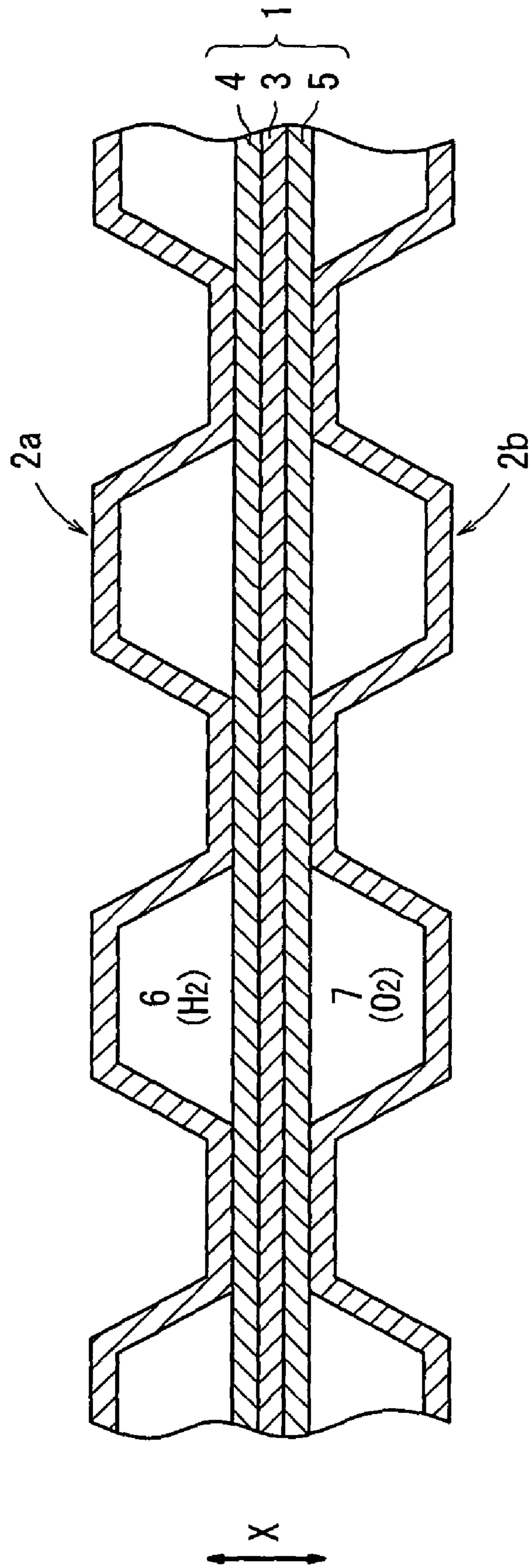
FIG. 17 PRIOR ART
