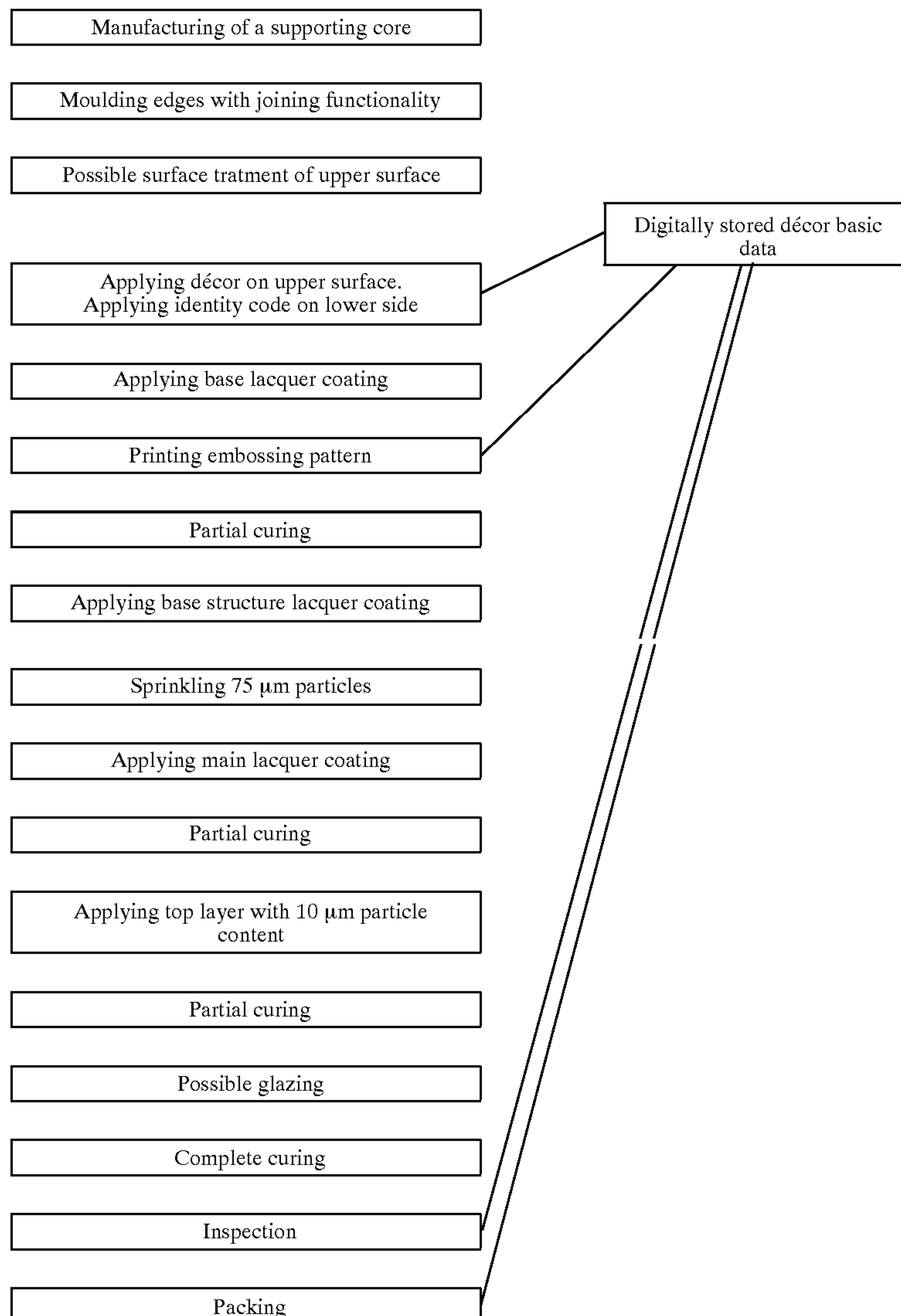
Process scheme 1.
