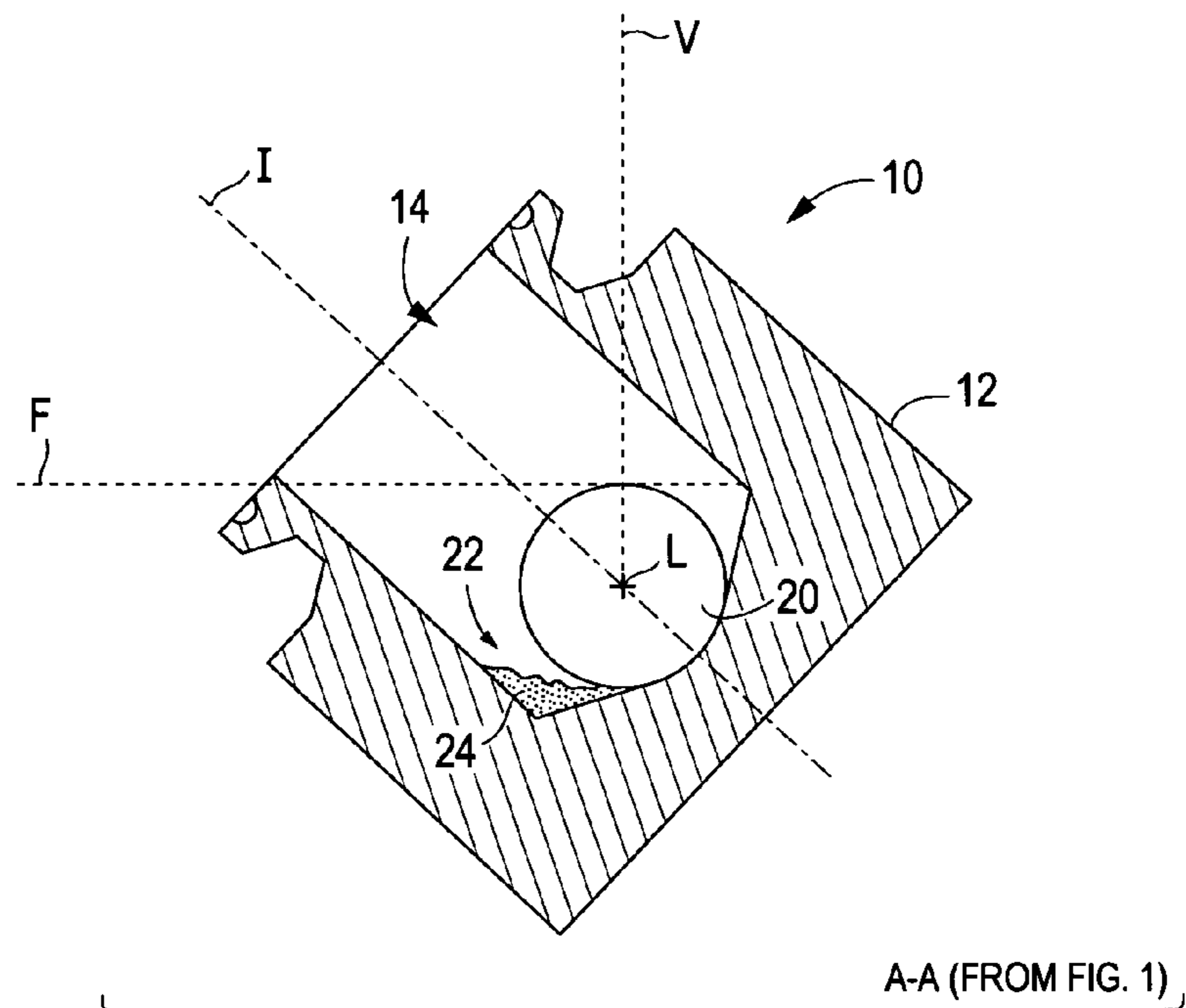
FIG. 2 PRIOR ART
