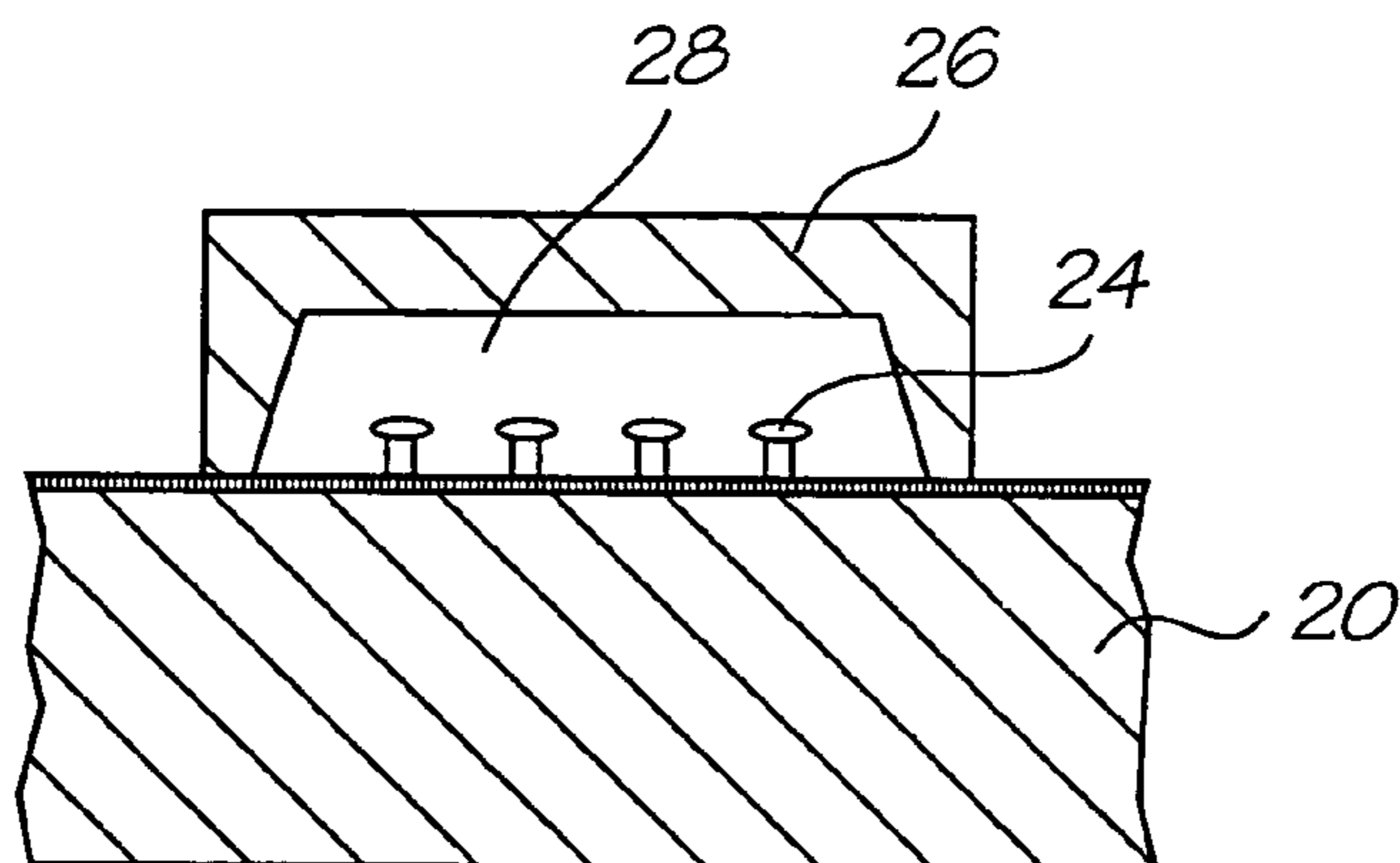
FIG. 3 (Prior Art)
