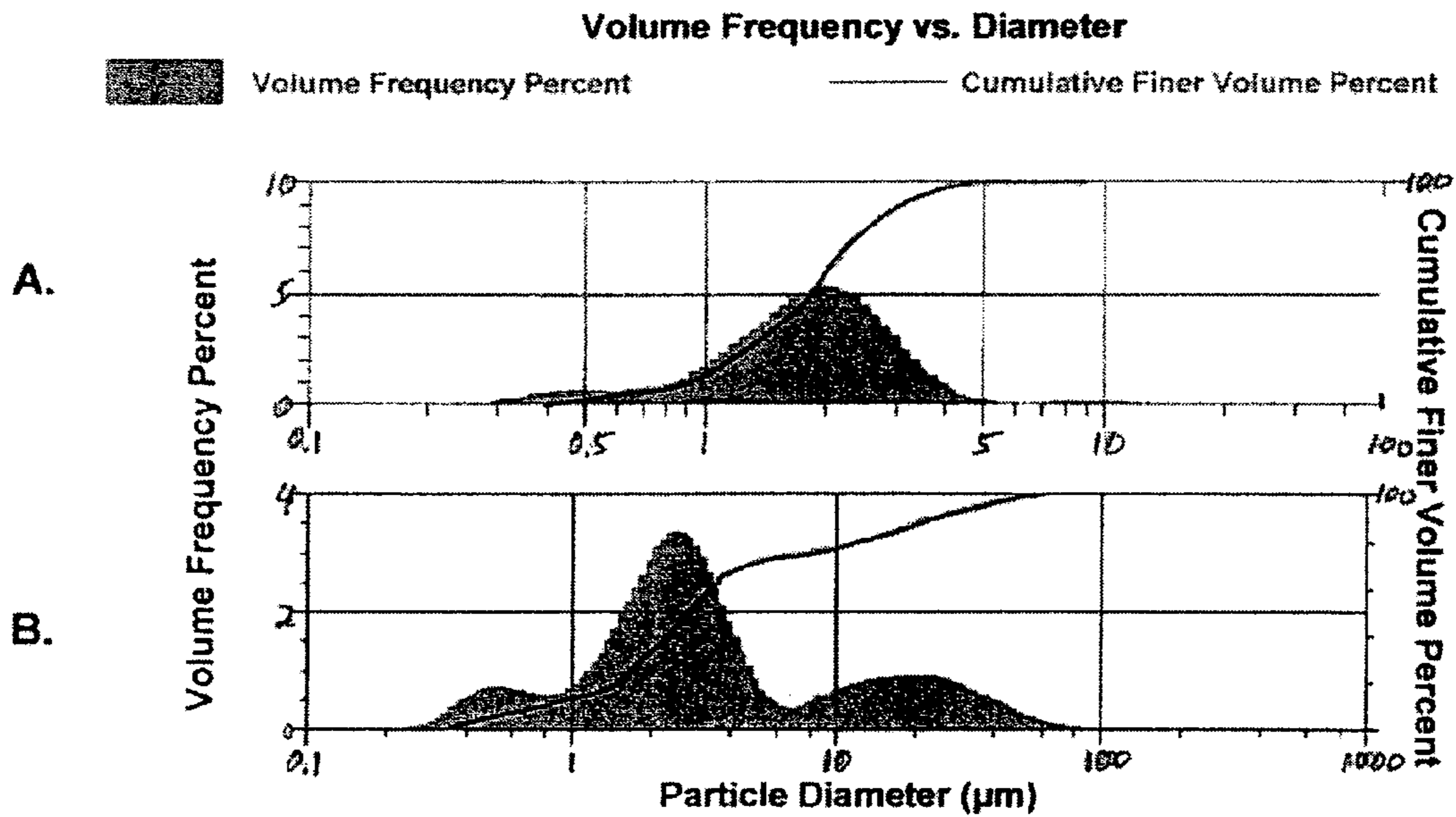
Figure 15 Resonance Disintegration (RD) of Standard Reference Carbon Black N660 Dispersed in Isopropanol. A. Before RD, B. After RD.
