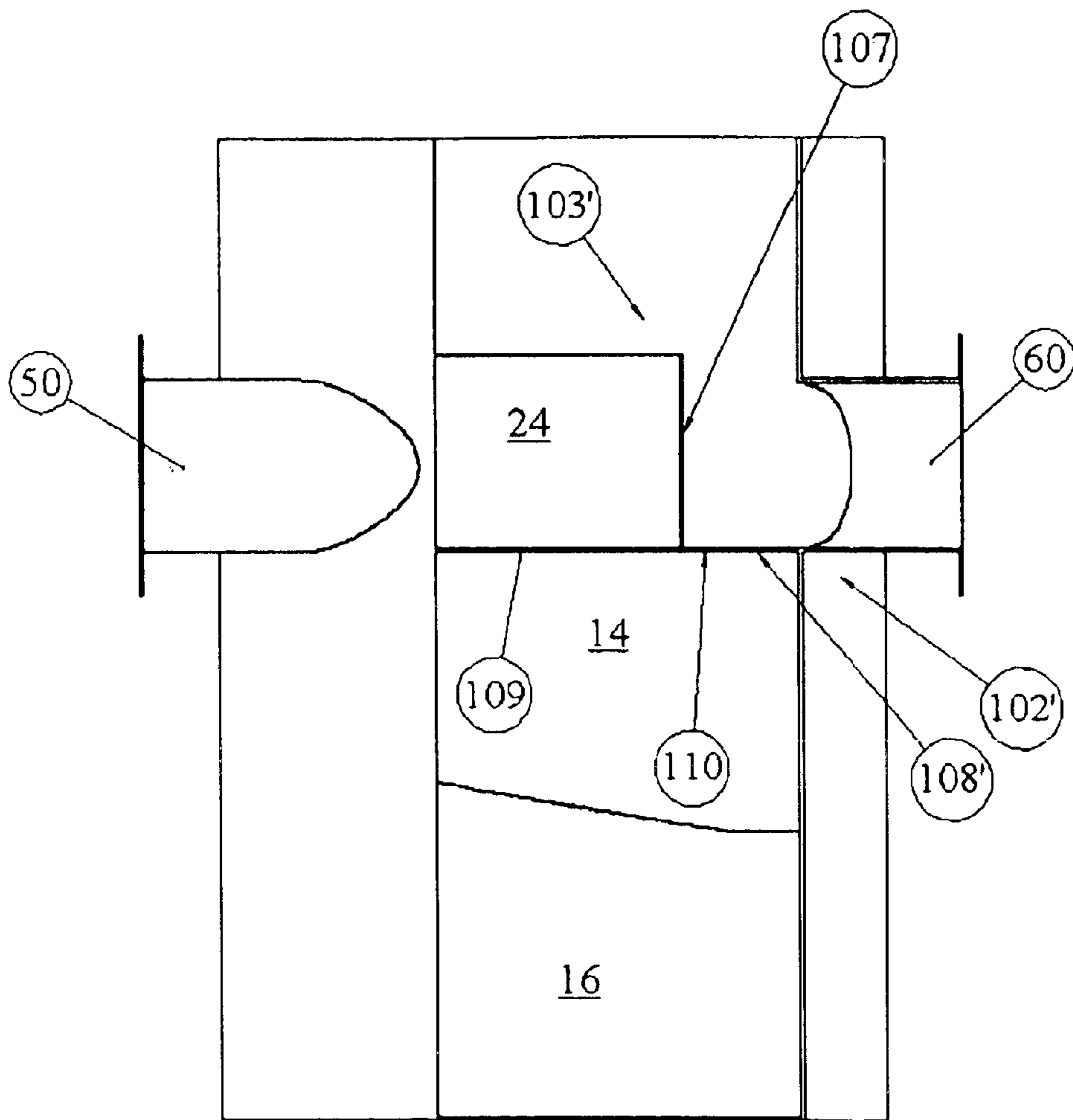
FIG. 10C (VIEW E-E)
