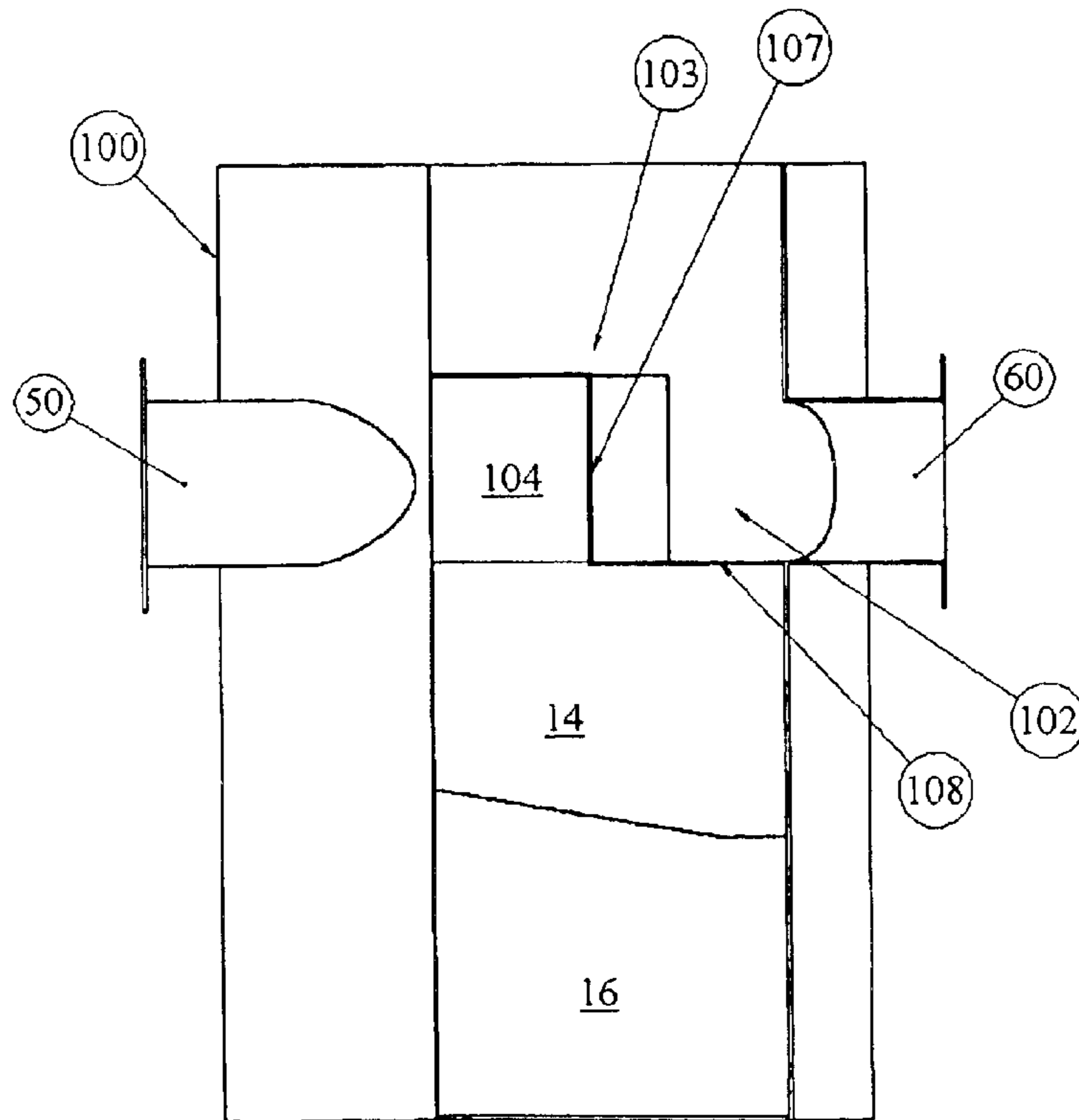
FIG. 9C (VIEW D-D)
