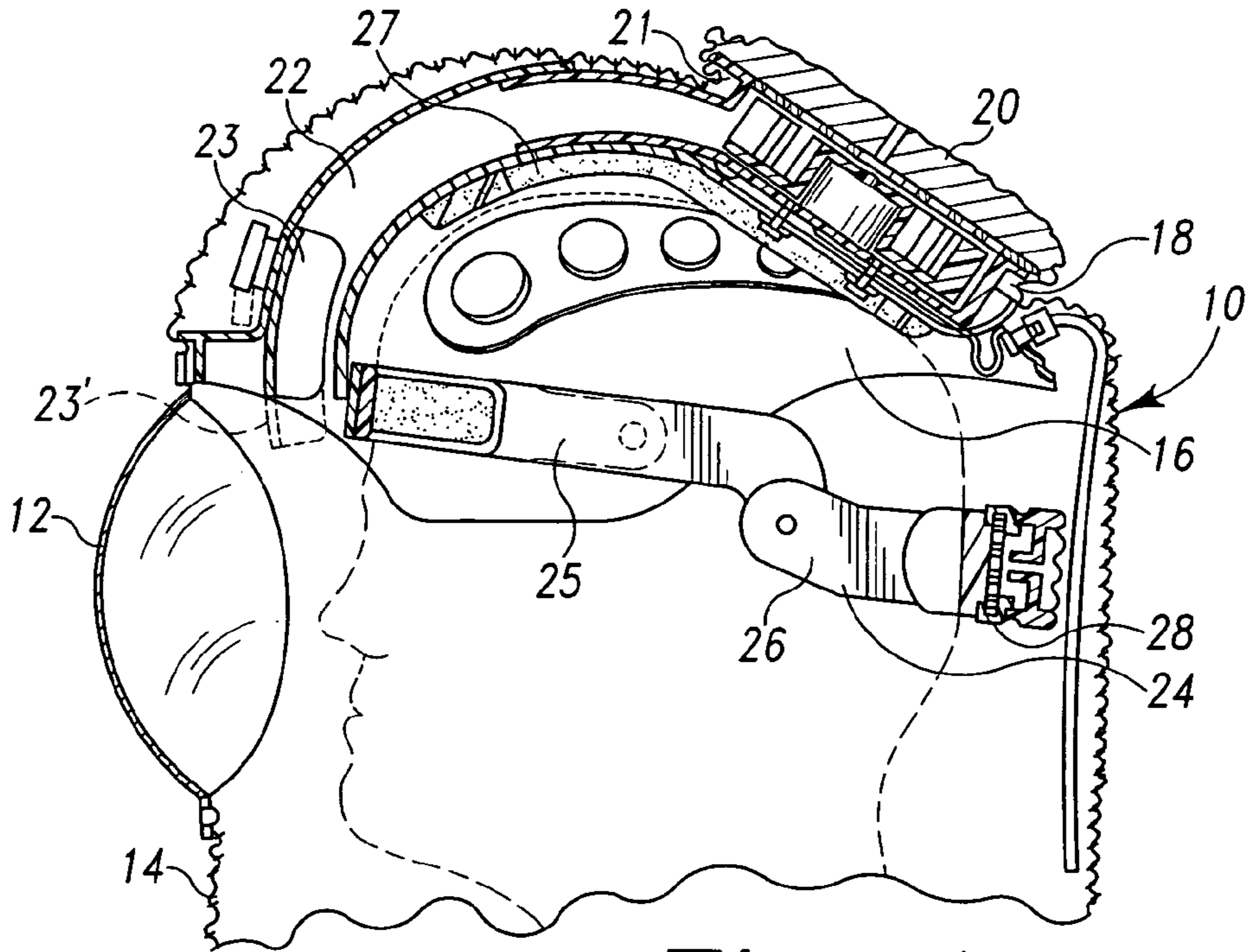
Fig. 1 (Prior Art)
