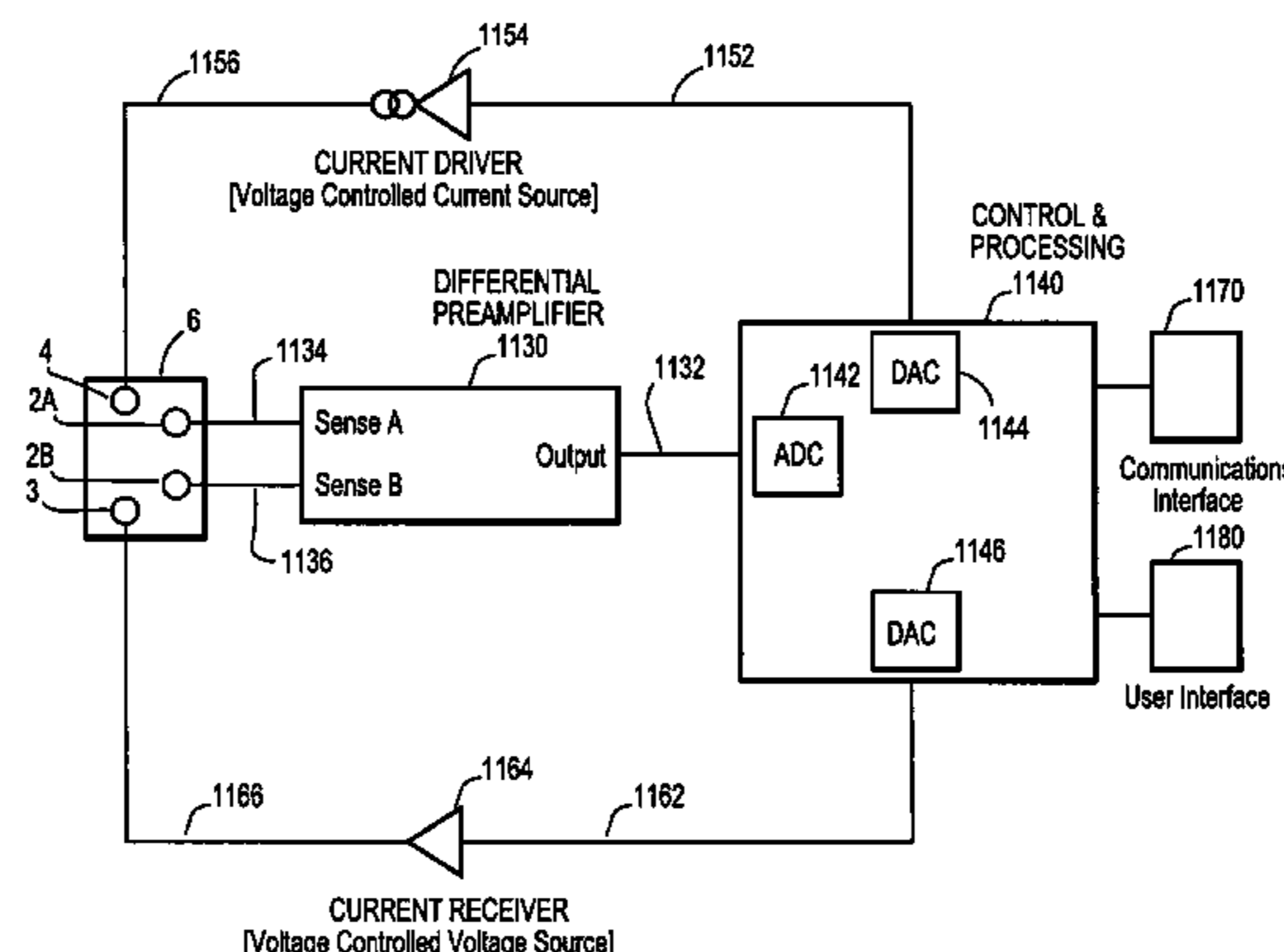
Galvanodynamic Test System
