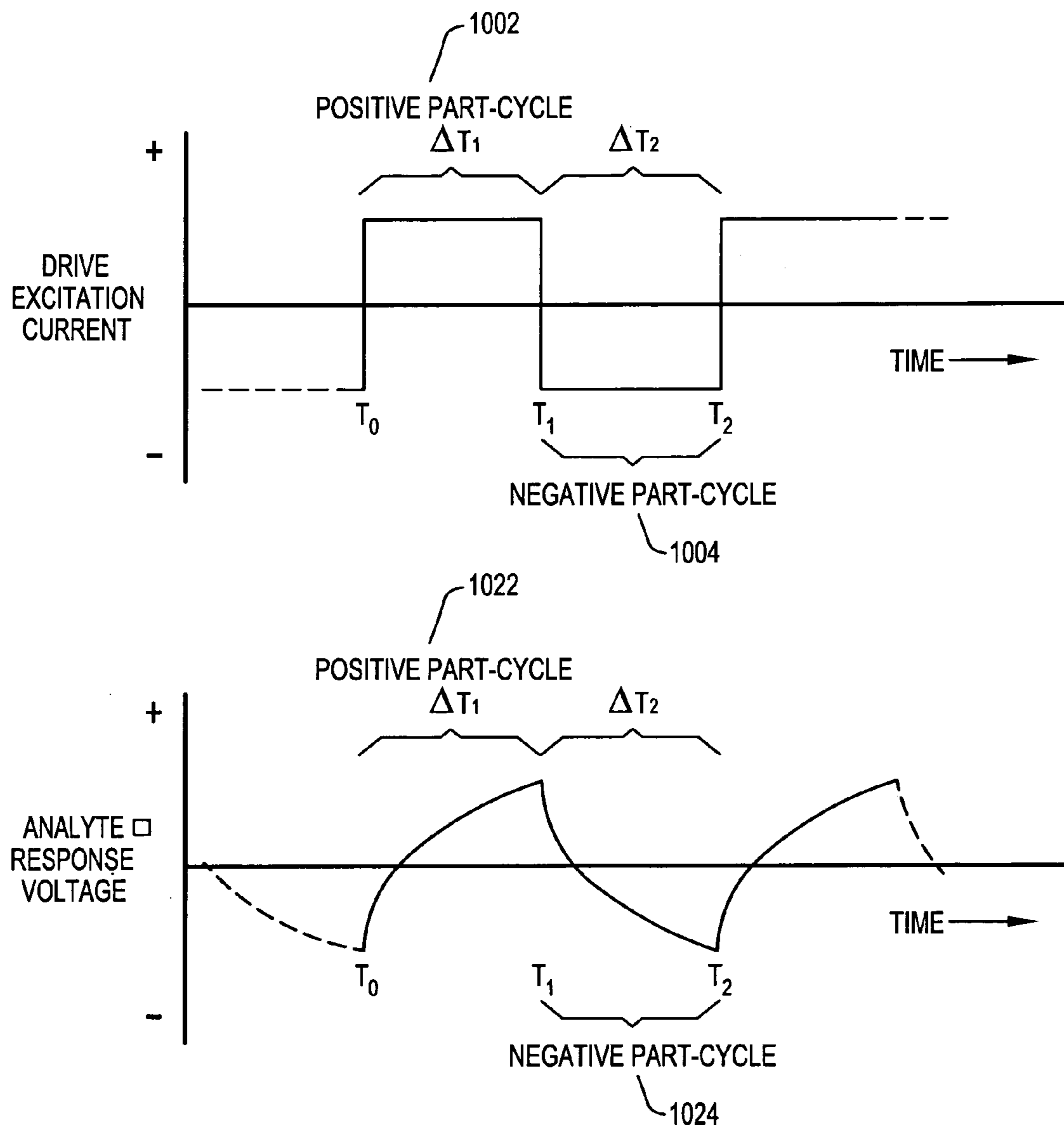
FIG. 10 Excitation and Response Waveforms
