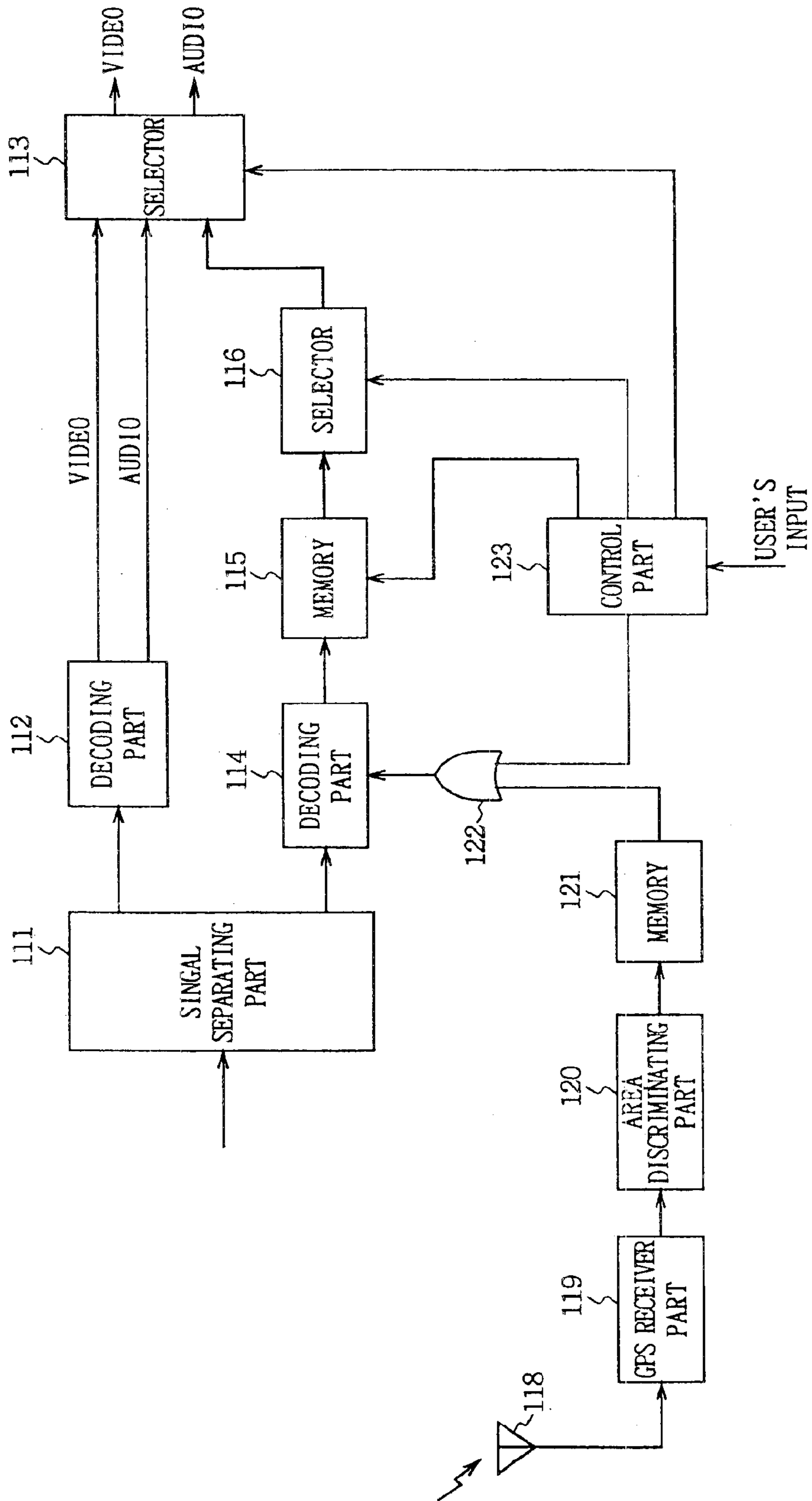
ISDB RECEIVER
