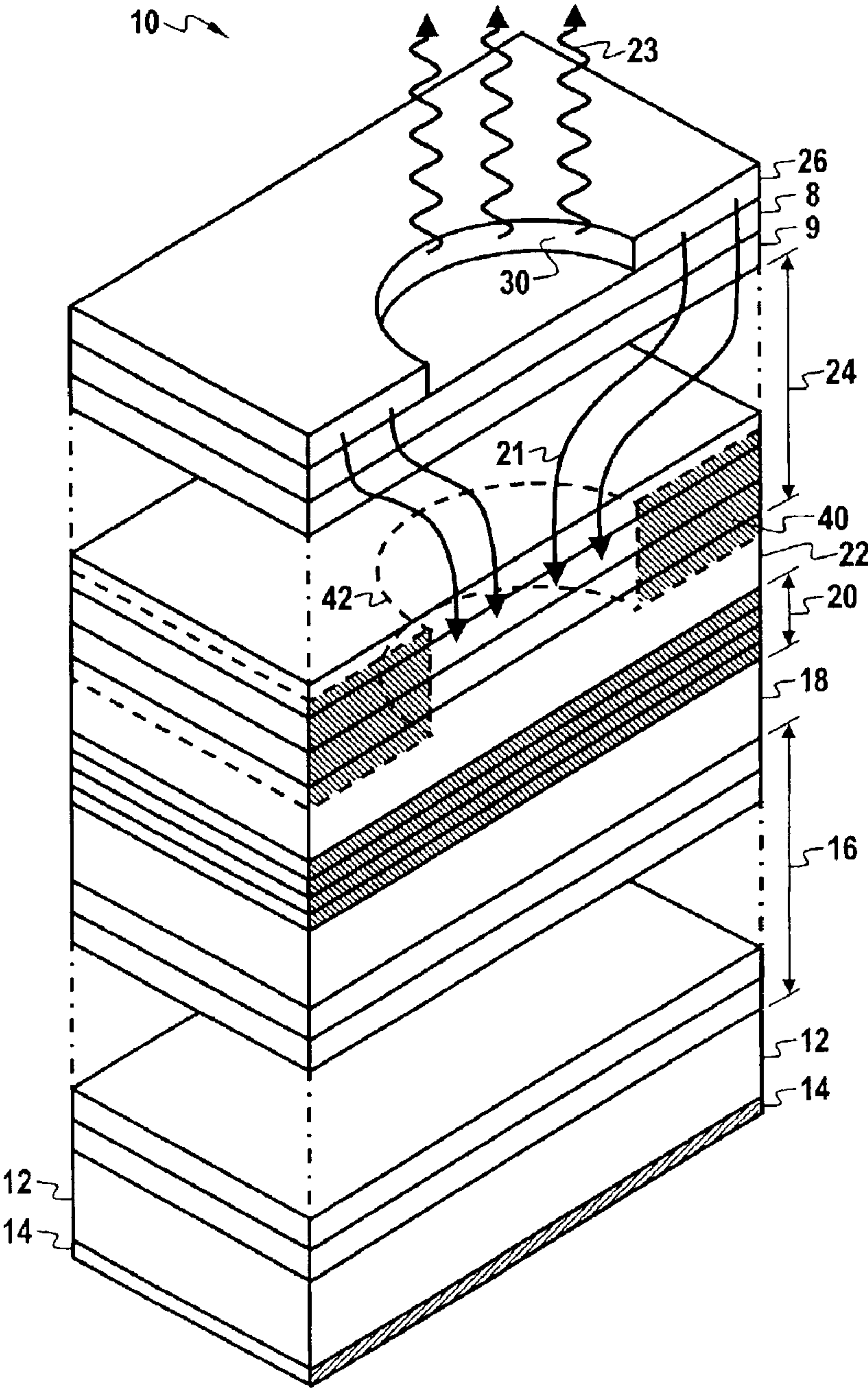
Figure 1 (Prior Art)
