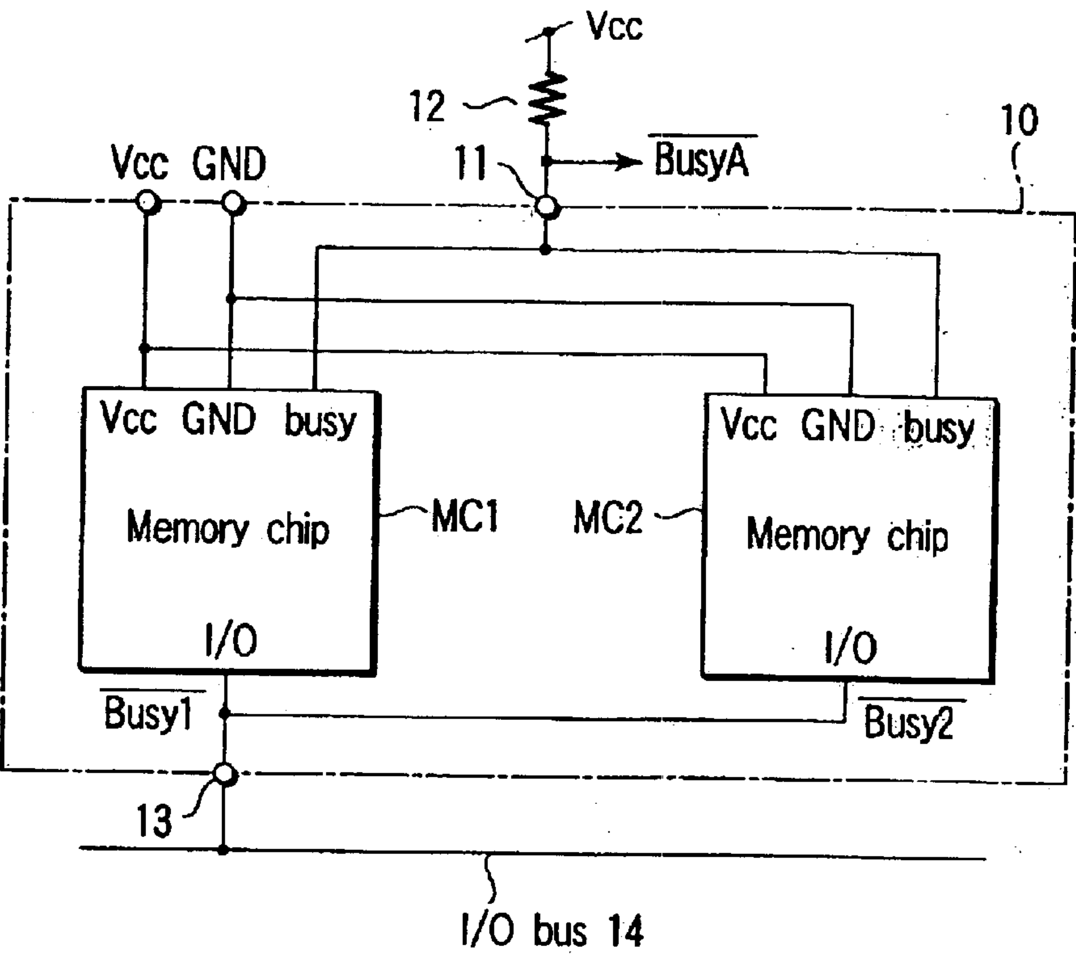
FIG. 1 PRIOR ART
