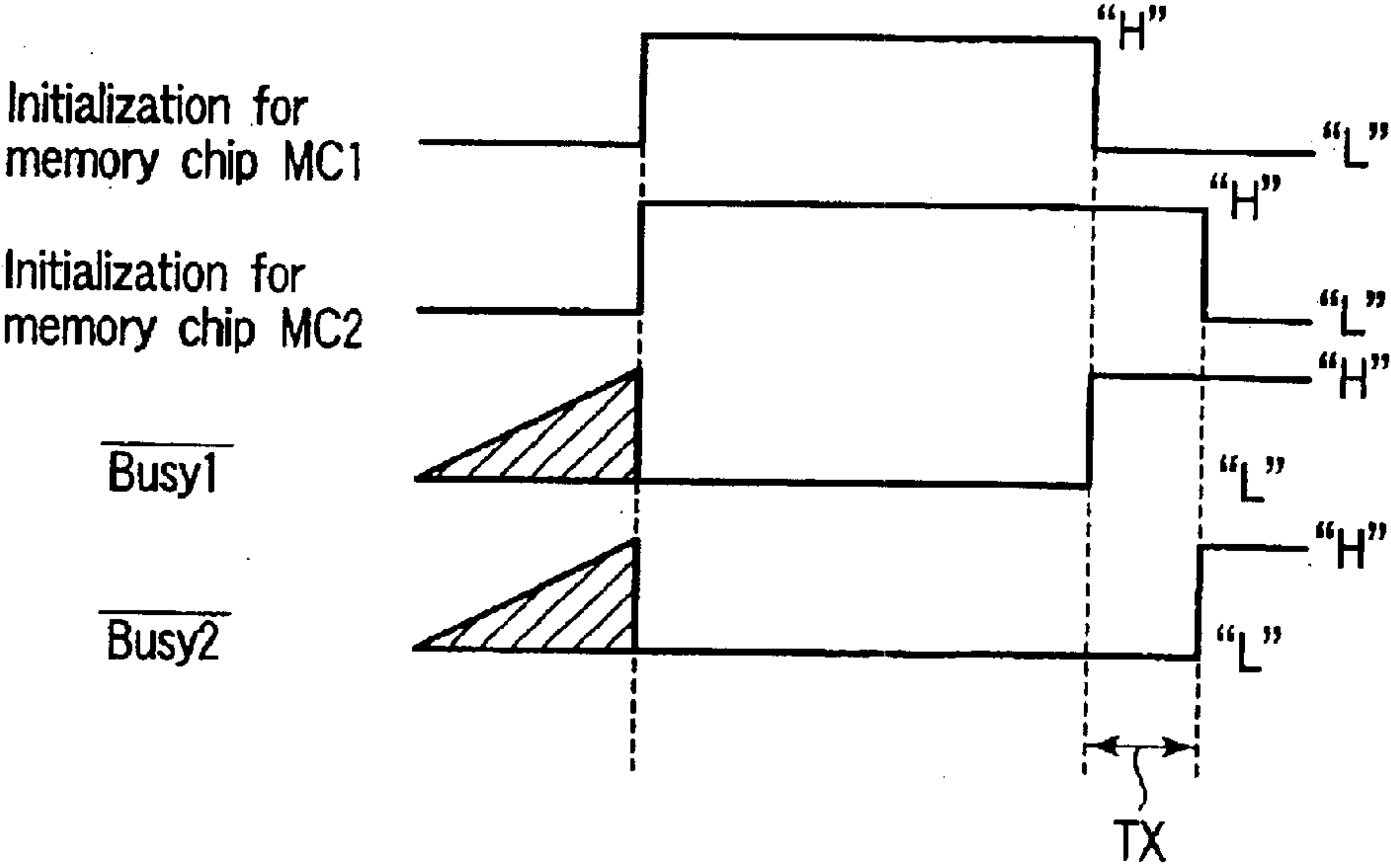
FIG. 2 PRIOR ART
