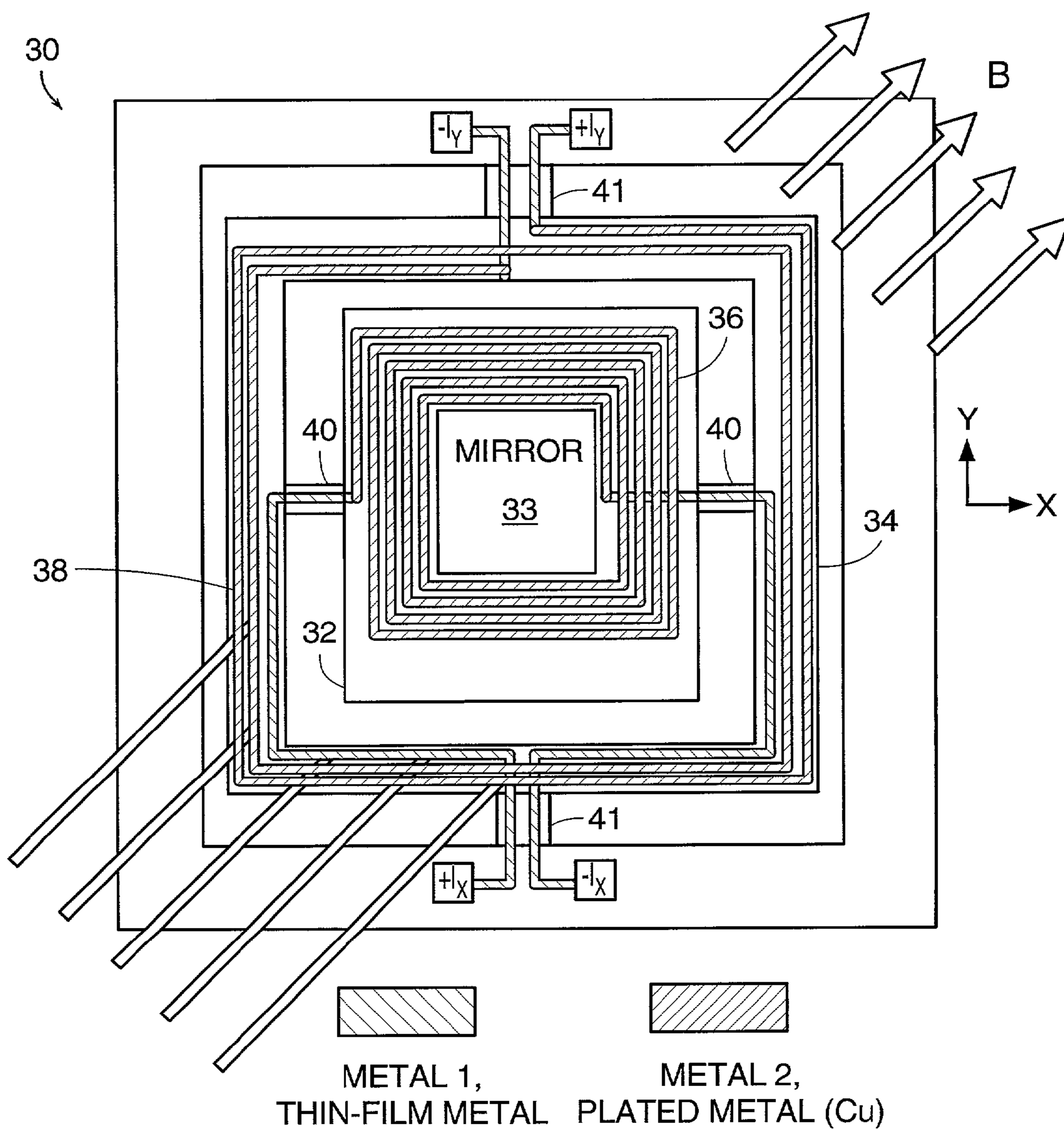
FIG. 2 PRIOR ART
