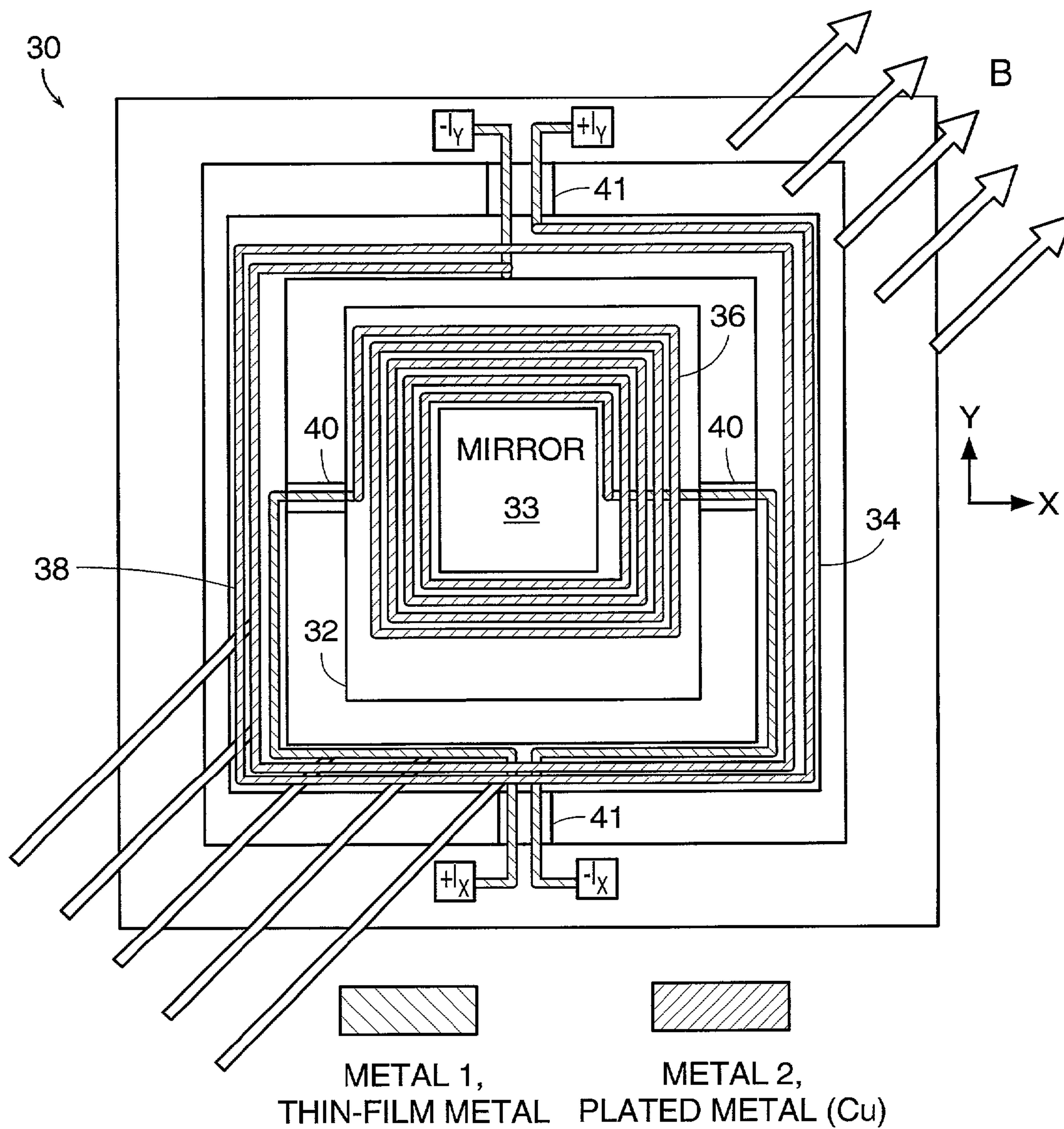
FIG. 2 PRIOR ART
