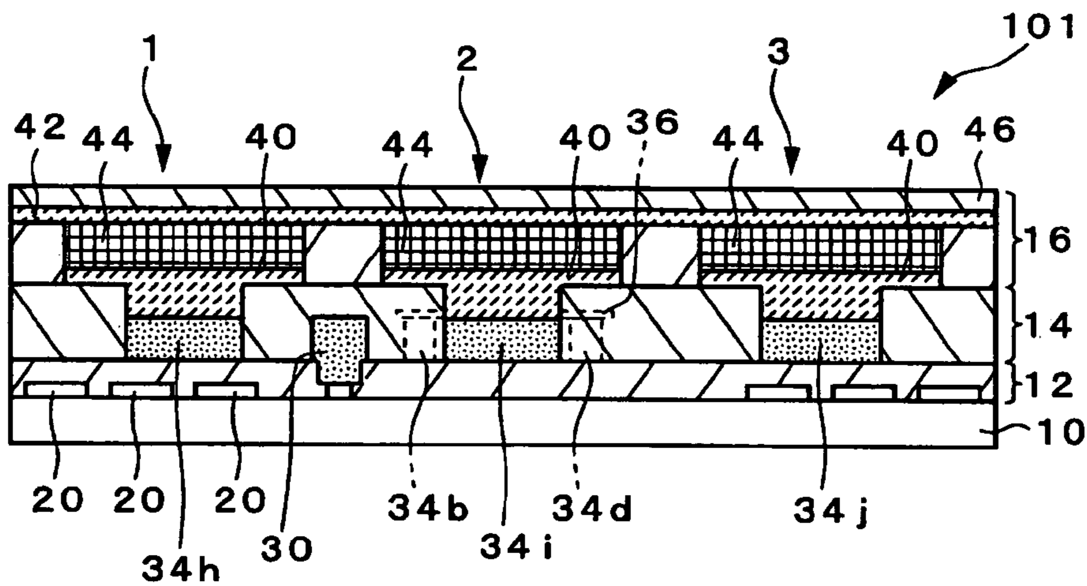
Sectional view taken along line B-B'
