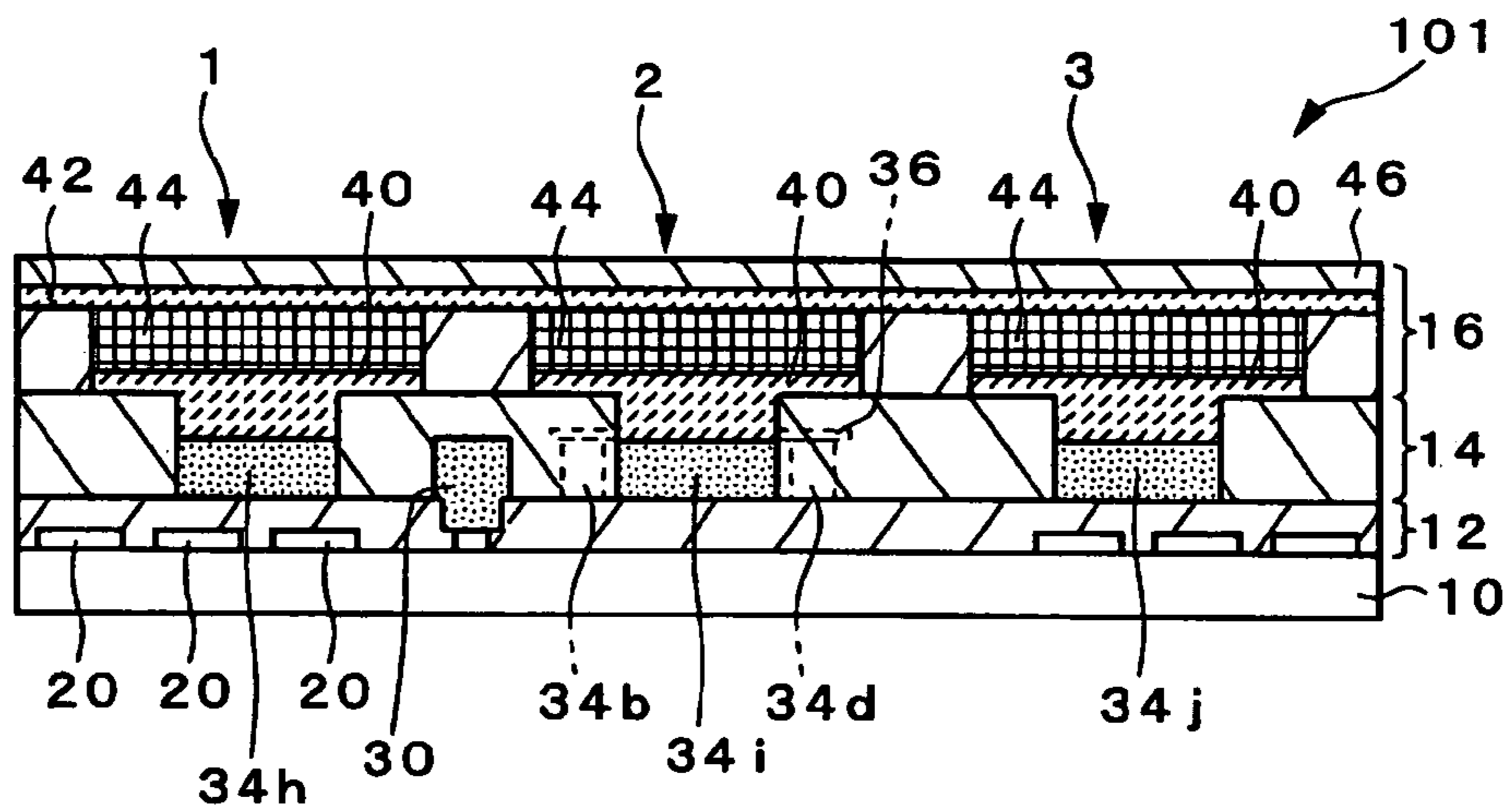
Sectional view taken along line B-B'
