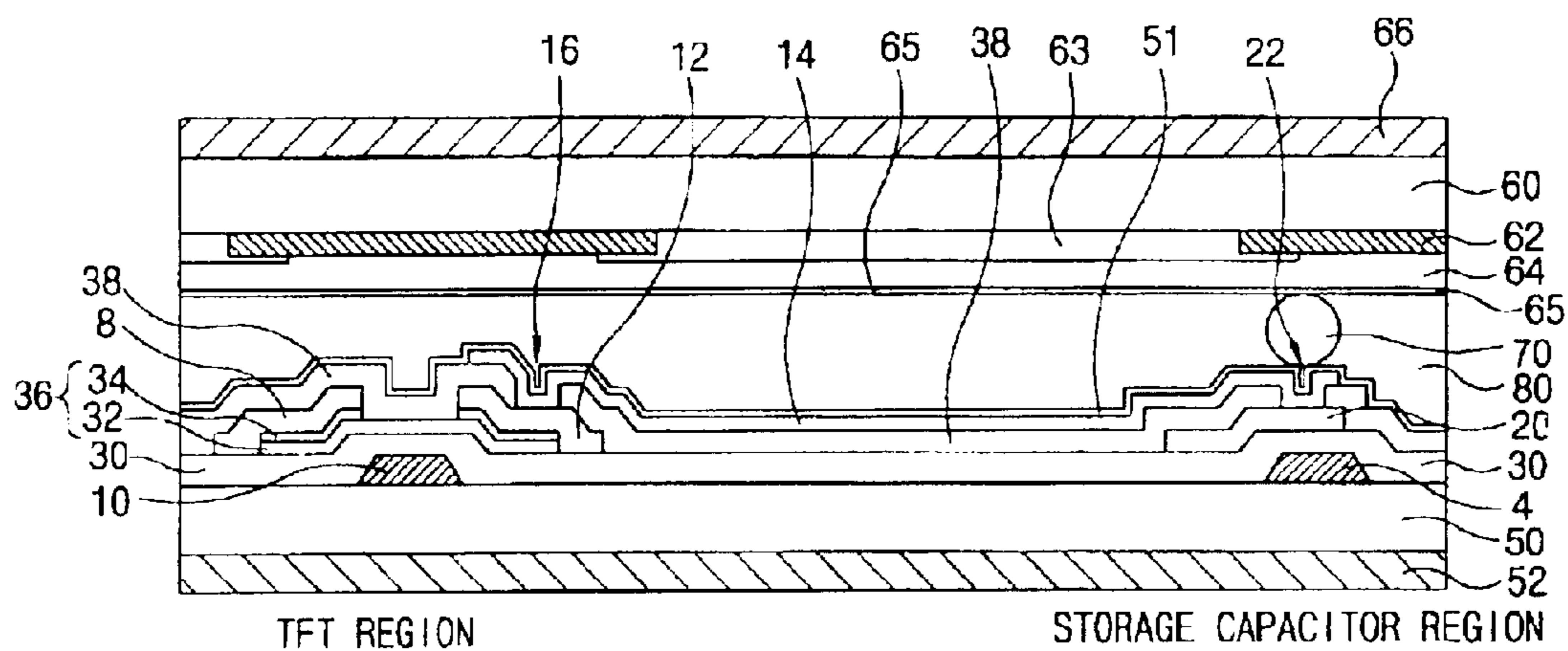
FIG. 2 CONVENTIONAL ART
