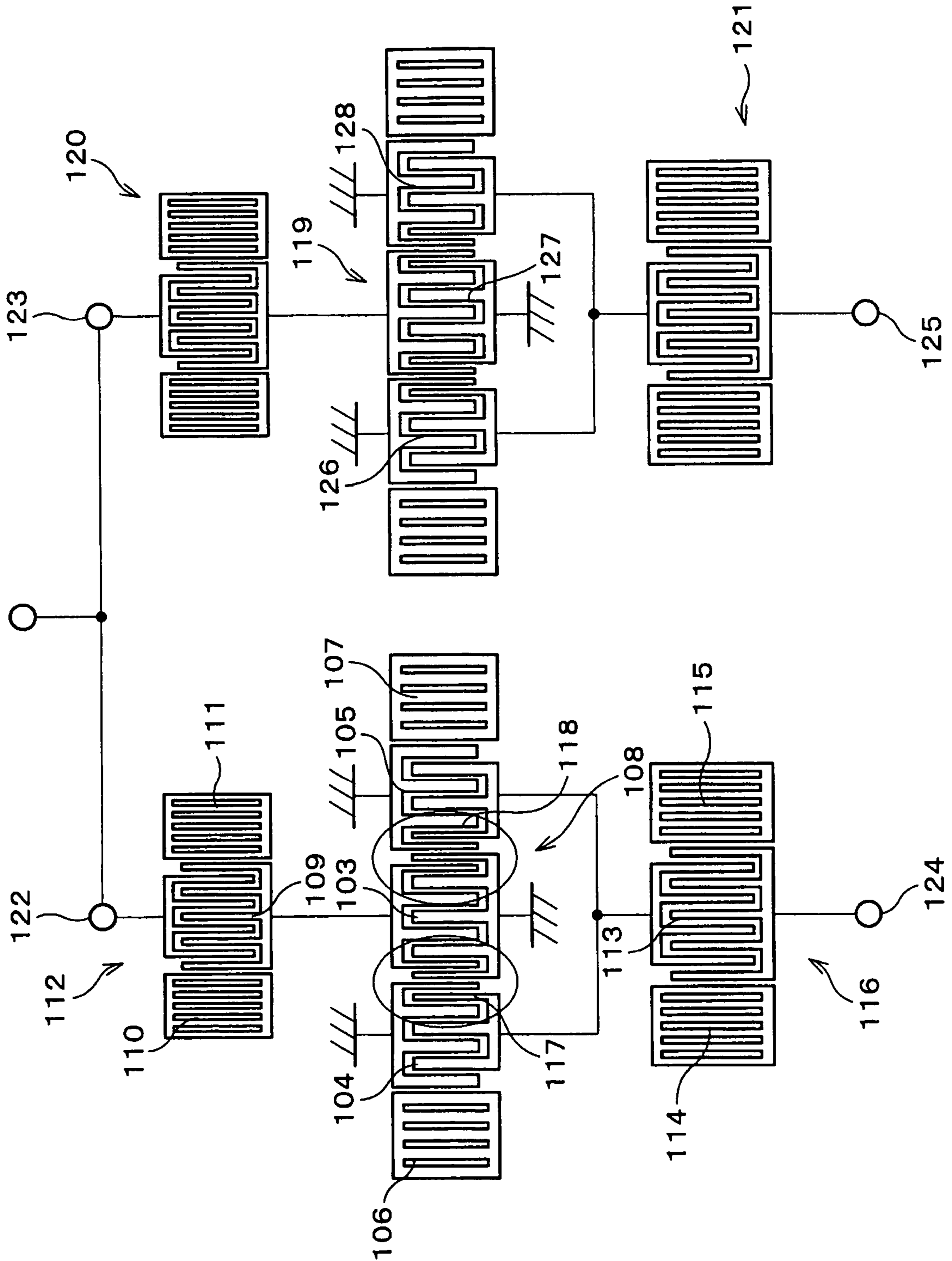
FIG. 2 PRIOR ART
