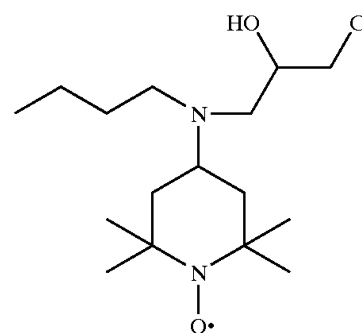
N-Butyl-N-(2-hydroxy-3-chloro)propyl-1-oxyl-2,2,6,6-tetramethyl-4-aminopiperidine
