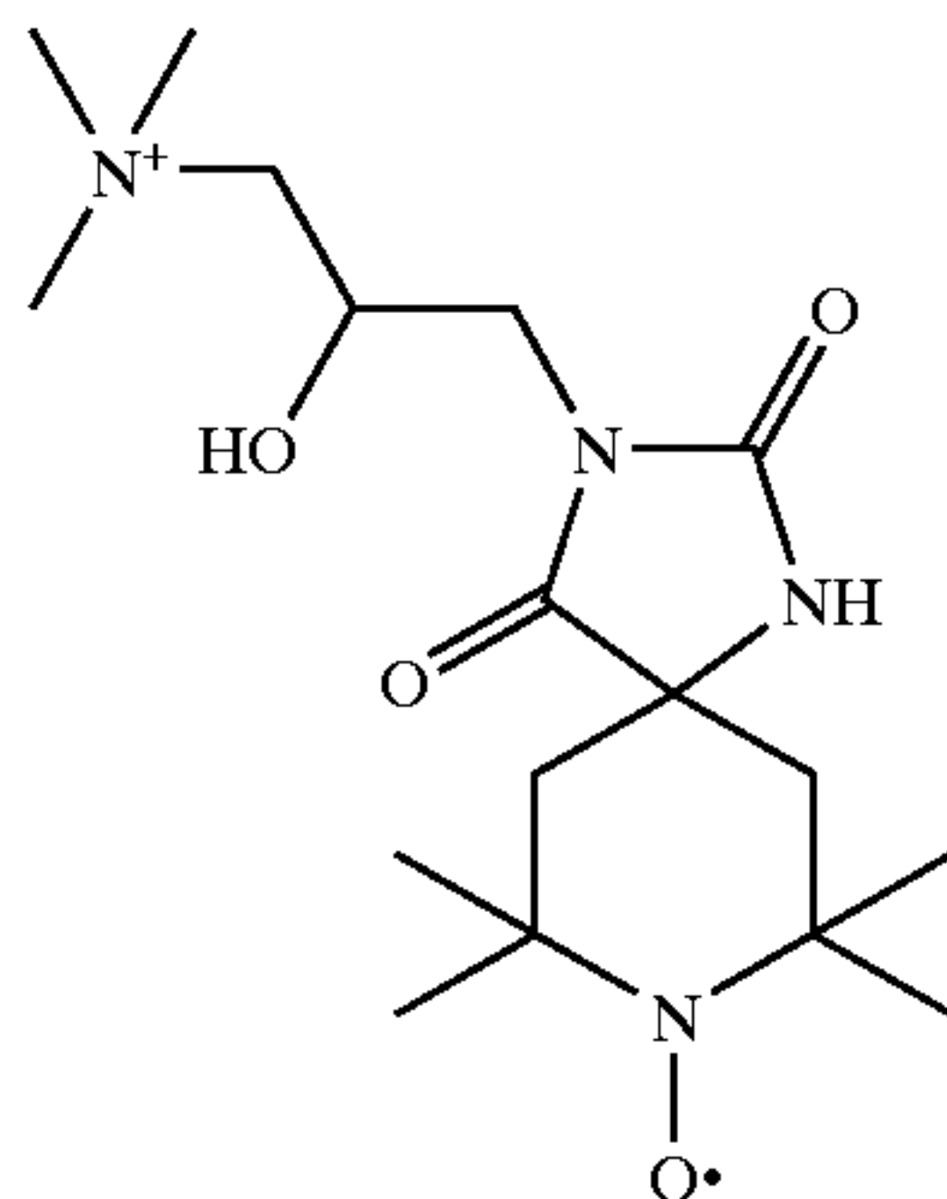
[2-Hydroxy-3-(8-oxyl-7,7,9,9-tetramethyl-2,4-dioxo-1,3,8-triaza-spiro[4.5]dec-3-yl)-propyl]-trimethylammonium chloride
