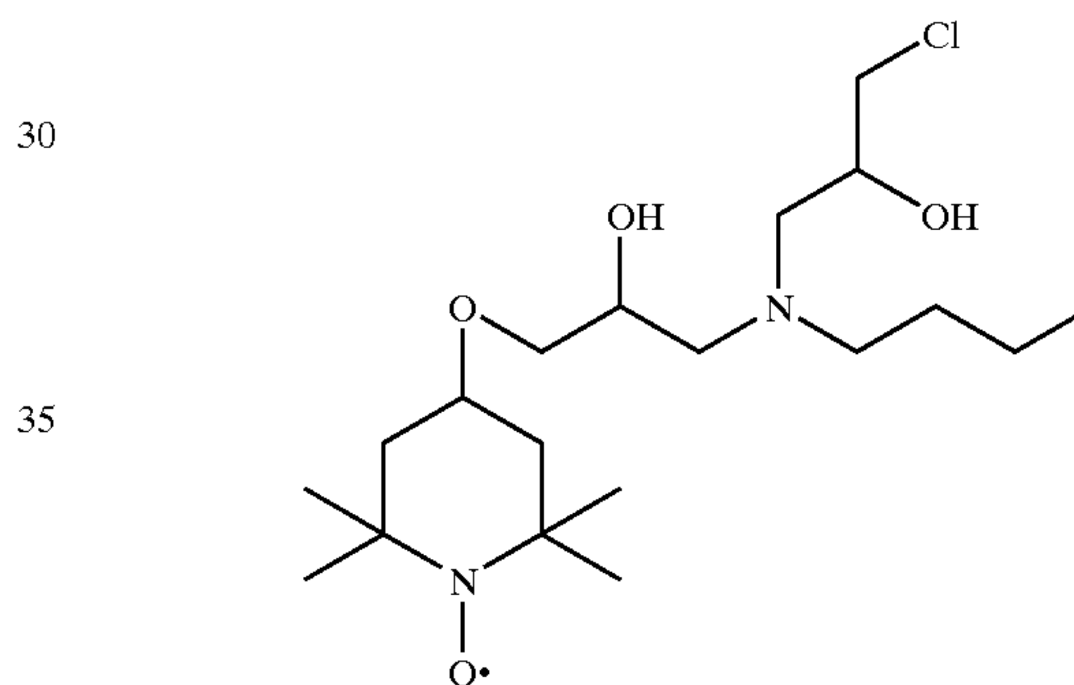
4-{3-[Butyl-(3-chloro-2-hydroxy-propyl)-amino]-2-hydroxy-propoxy}-2,2,6,6-tetramethyl-piperidin-1-oxyl
