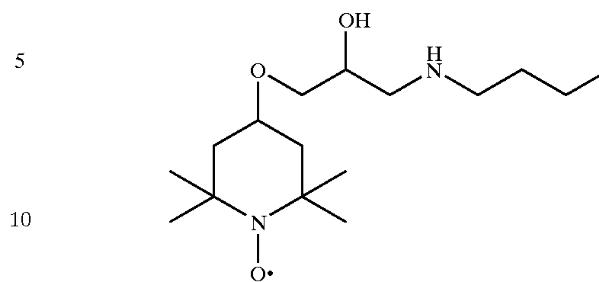
4-(3-Butylamino-2-hydroxy-propoxy)-2,2,6,6-tetramethyl-piperidin-1-oxyl
