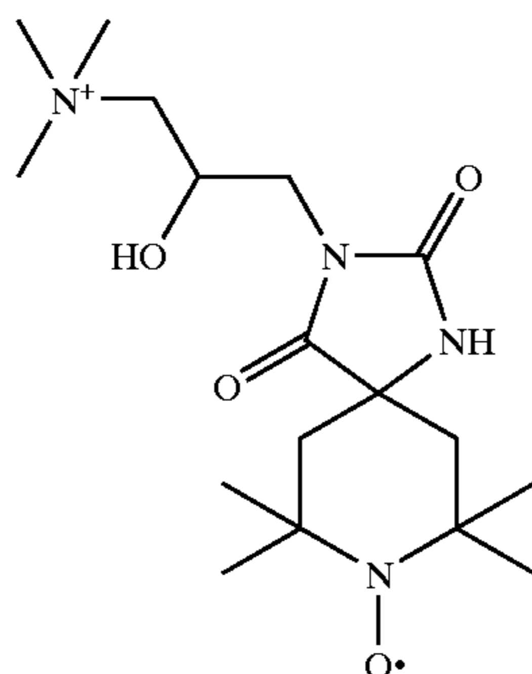
[2-Hydroxy-3-(8-oxyl-7,7,9,9-tetramethyl-2,4-dioxo- 1,3,8-triaza-spiro[4.5]dec-3-yl)-propyl]-trimethyl- ammonium chloride
