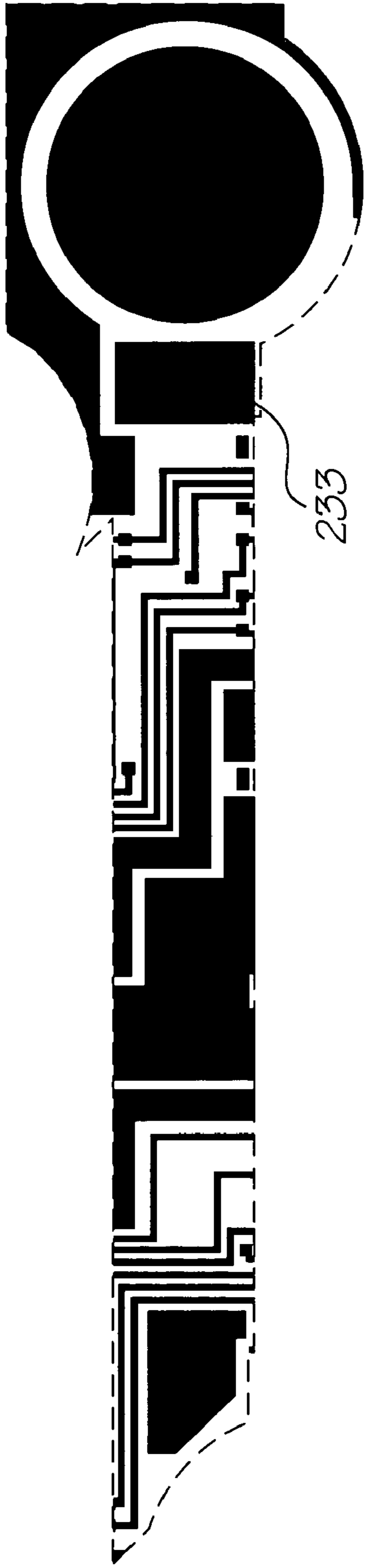
Metal 2 mask
