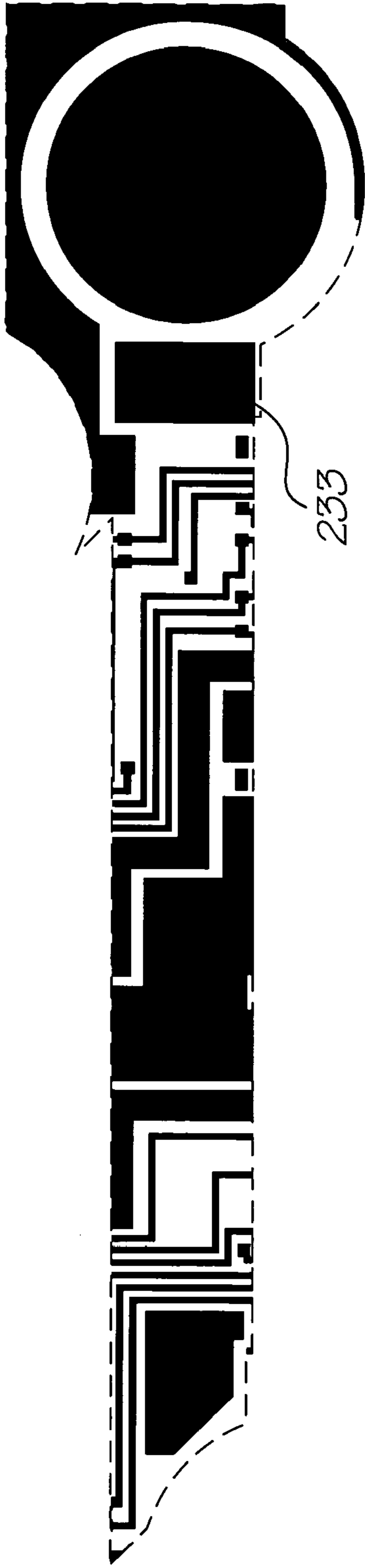
Metal 2 mask
