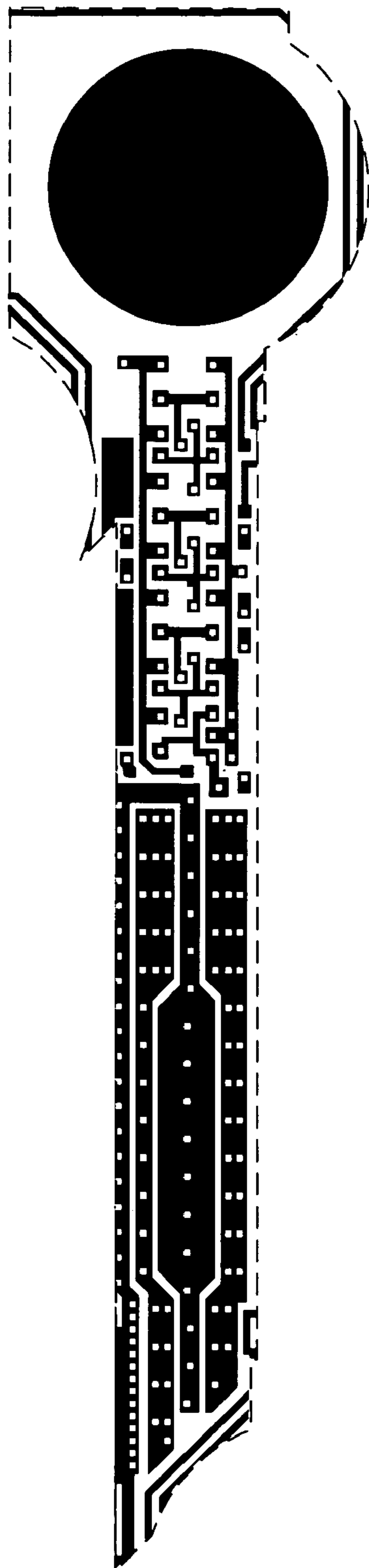
Metal 1 mask
