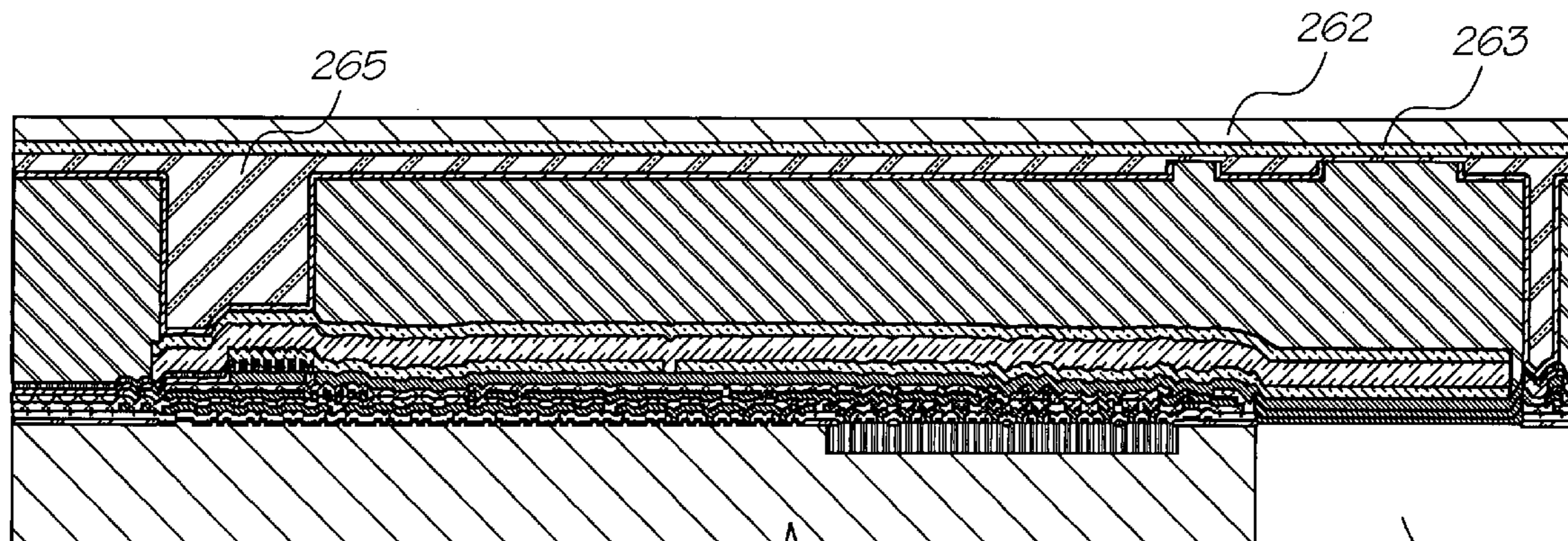
Mount on wafer blank, back-etch inlets
