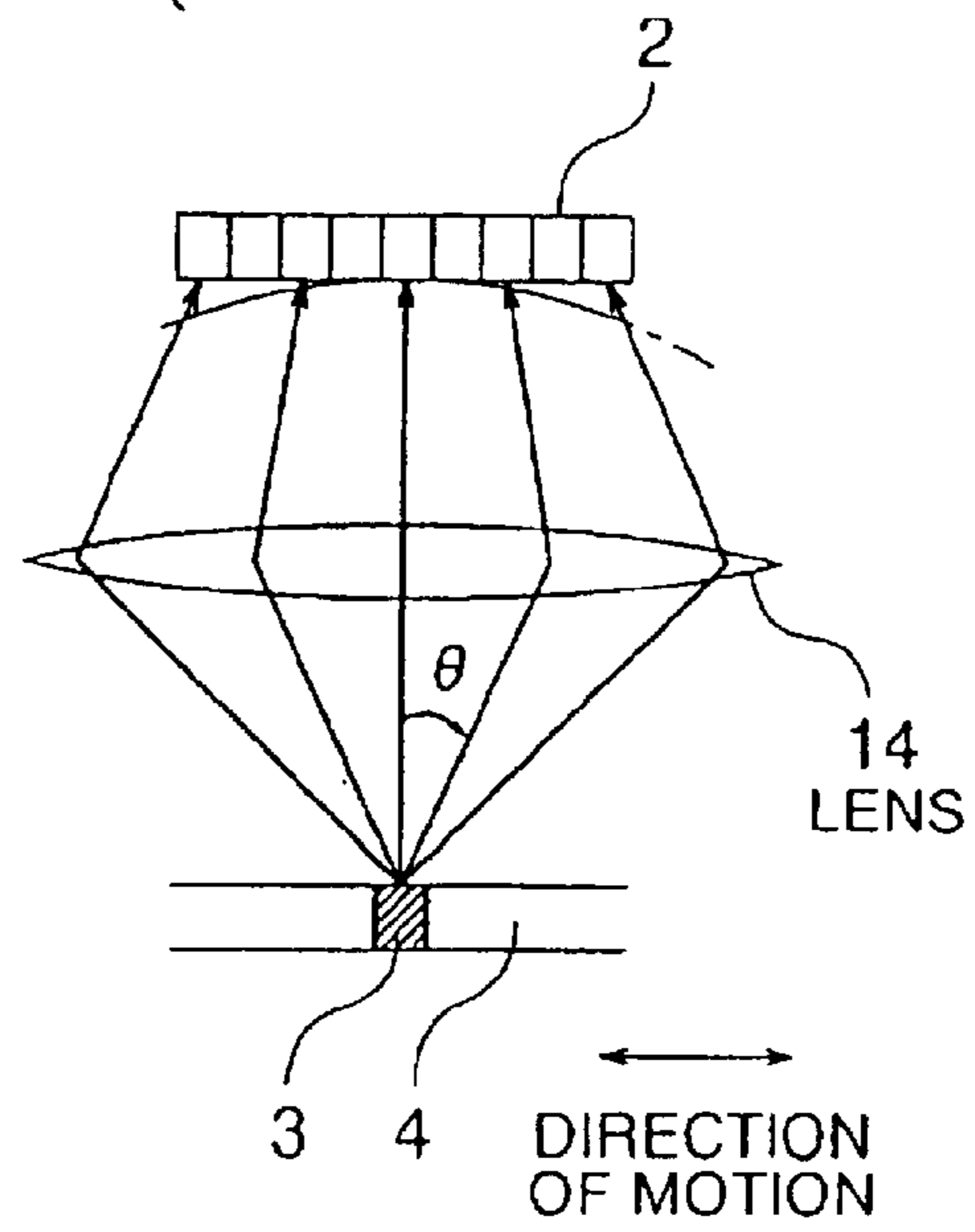
FIG. 9B (PRIOR ART)
