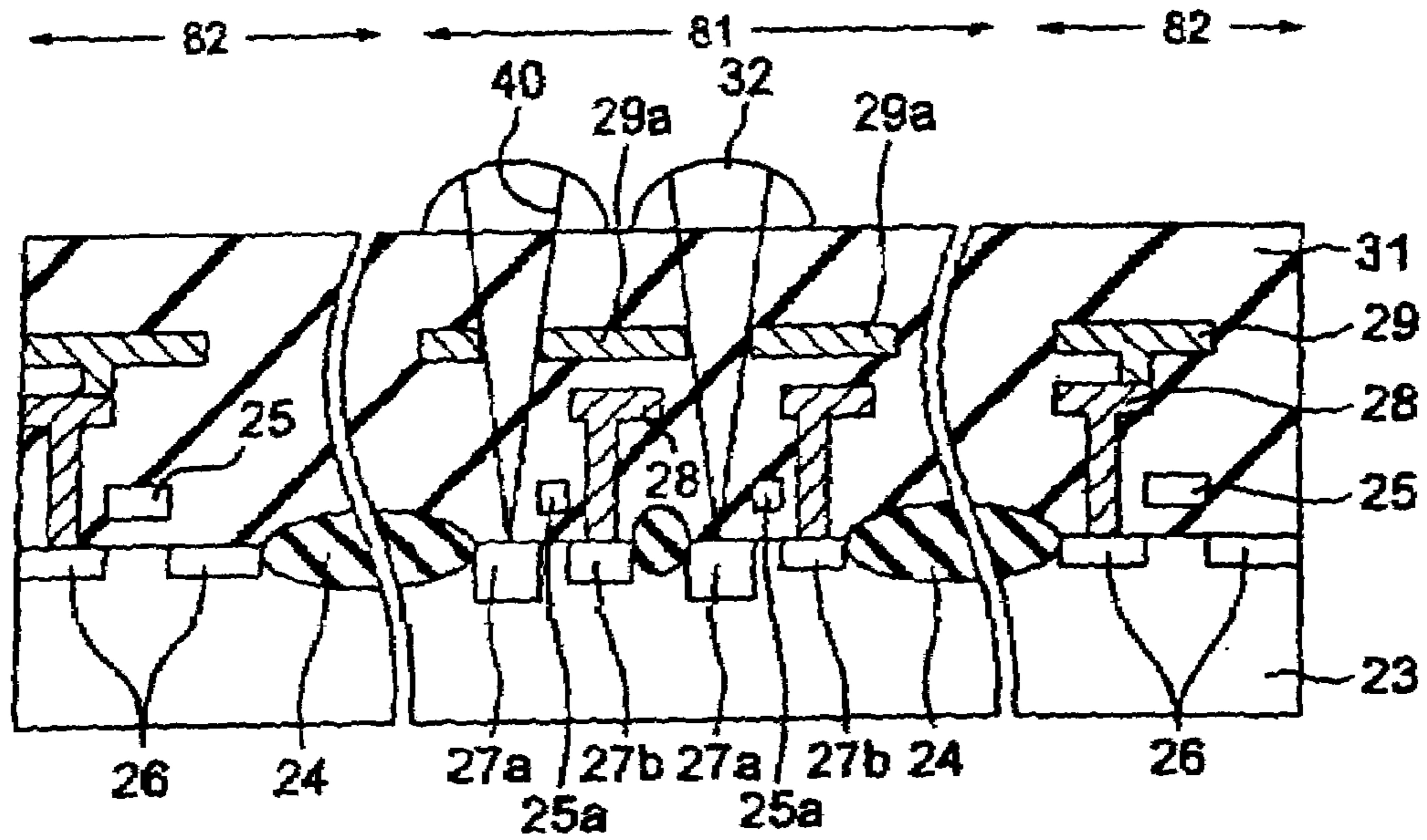
FIG. 16 PRIOR ART
