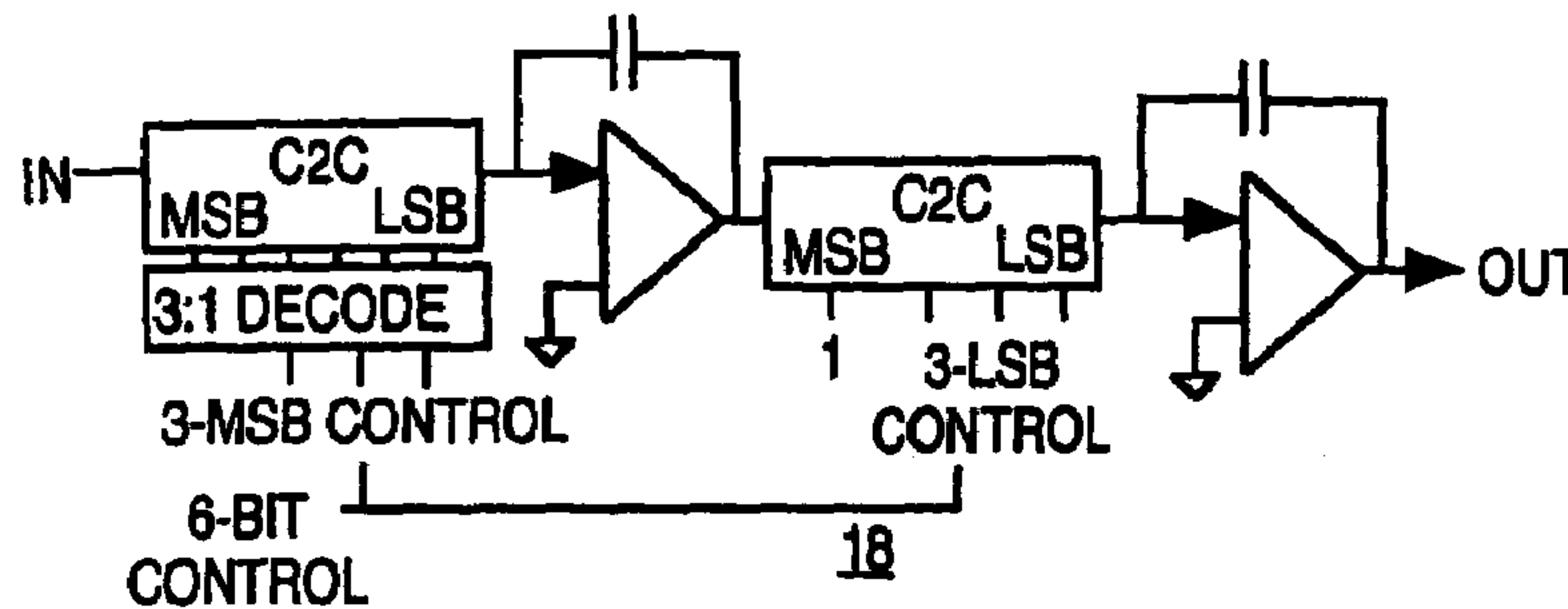
CASCADED TGC STAGES TECHNIQUE
