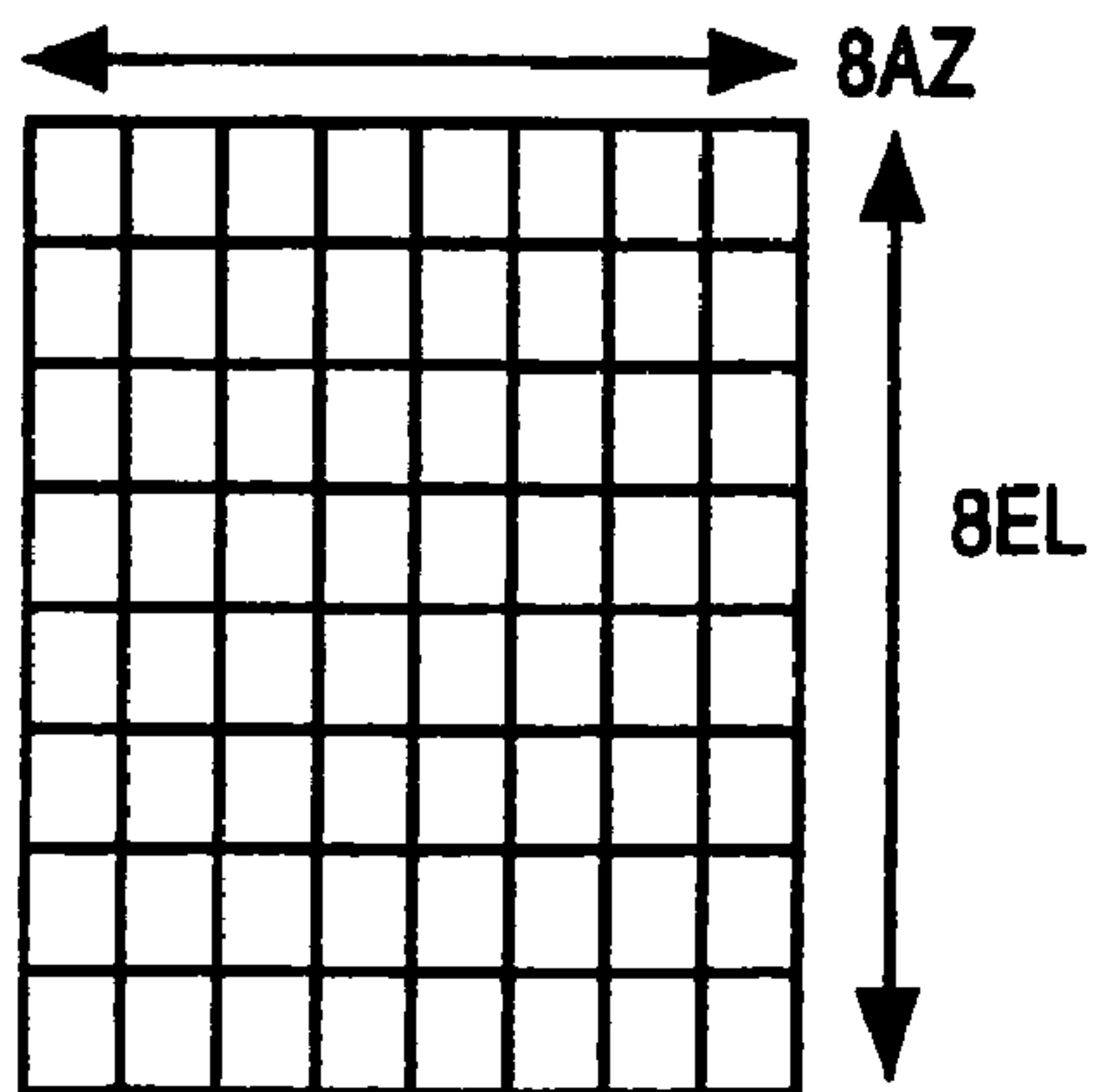
NORMAL BEAMFORMER
